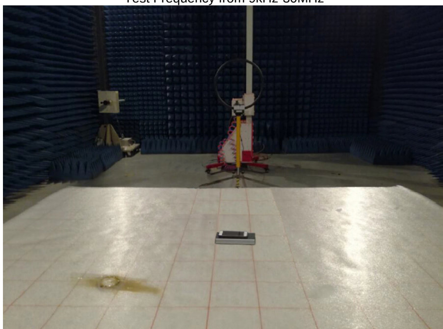
Radiated Spurious Emission Test Frequency from 9kHz-30MHz
