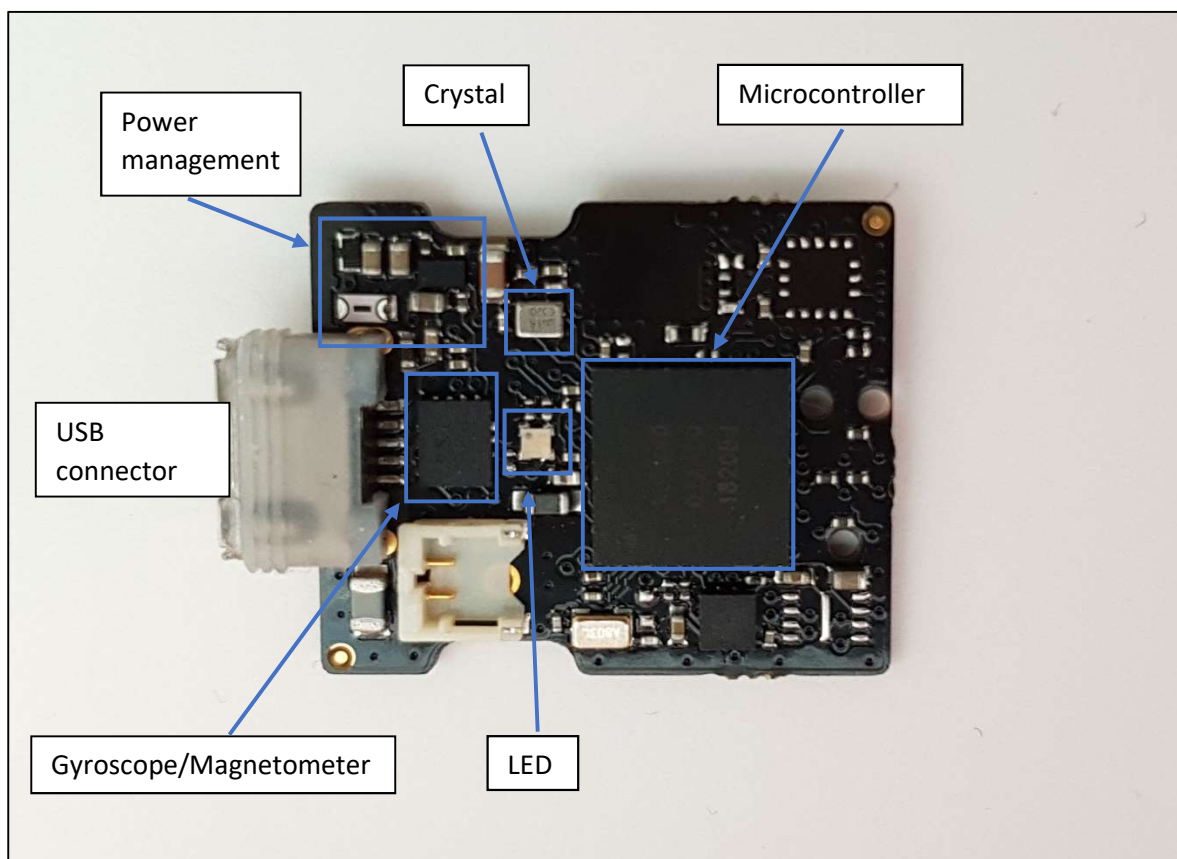
Figure 4. Main parts.
