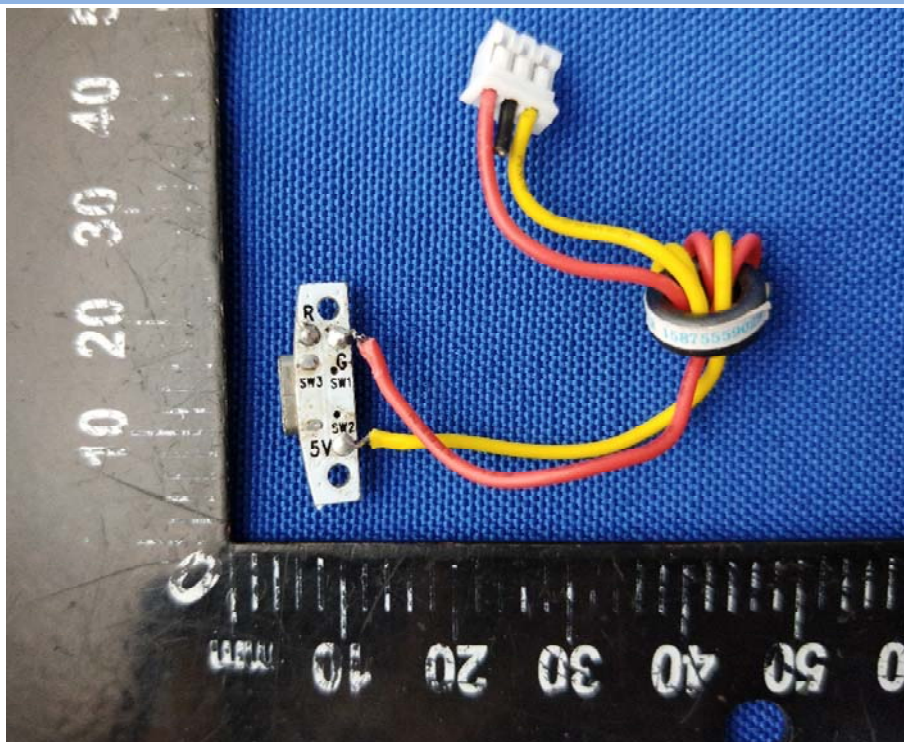
MAIN BOARD TOP VIEW
