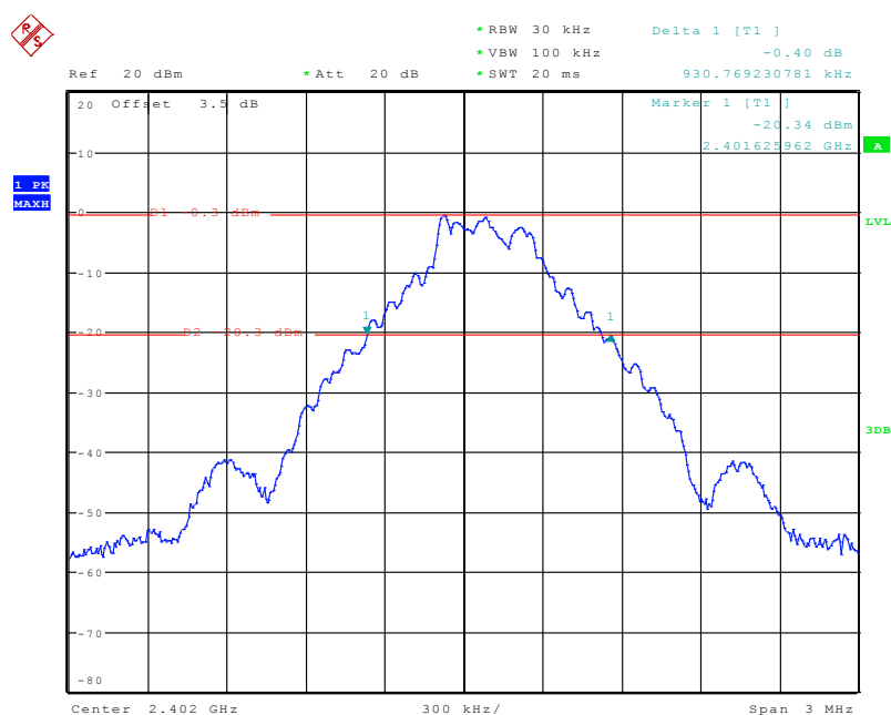
BDR (GFSK): Low Channel
