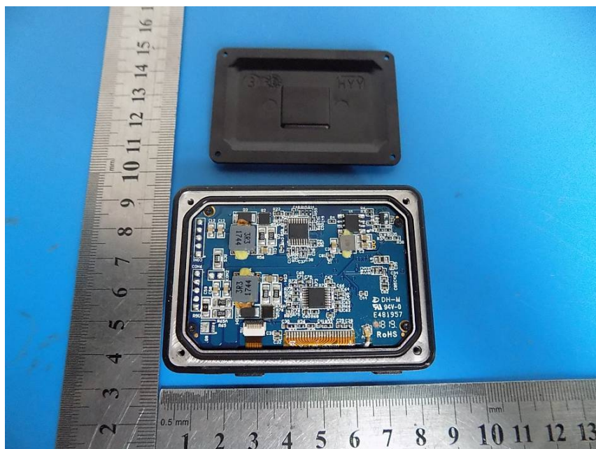
Uncover-2
