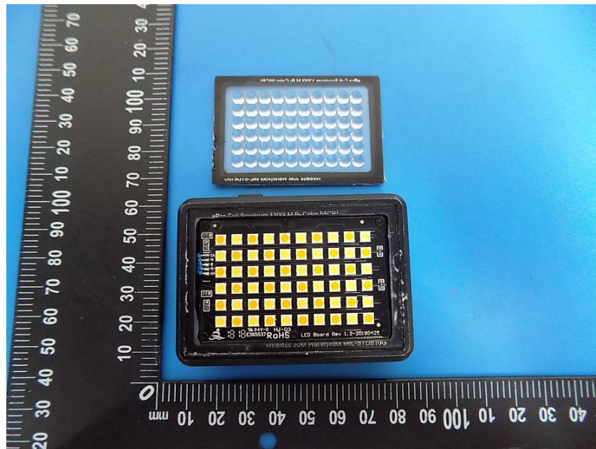
LED board front
