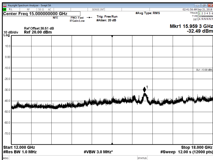
Antenna A - LTE Modulation QPSK - Channel M
