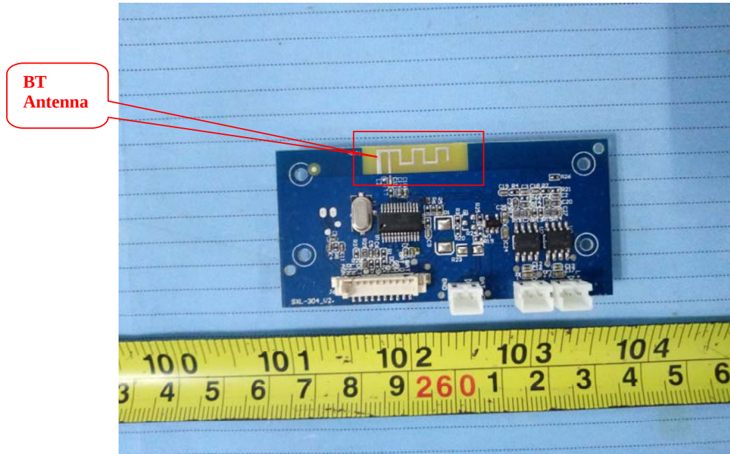
EUT – Mainboard 1 Top View
