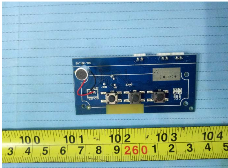
EUT – Mainboard 1 Bottom View
