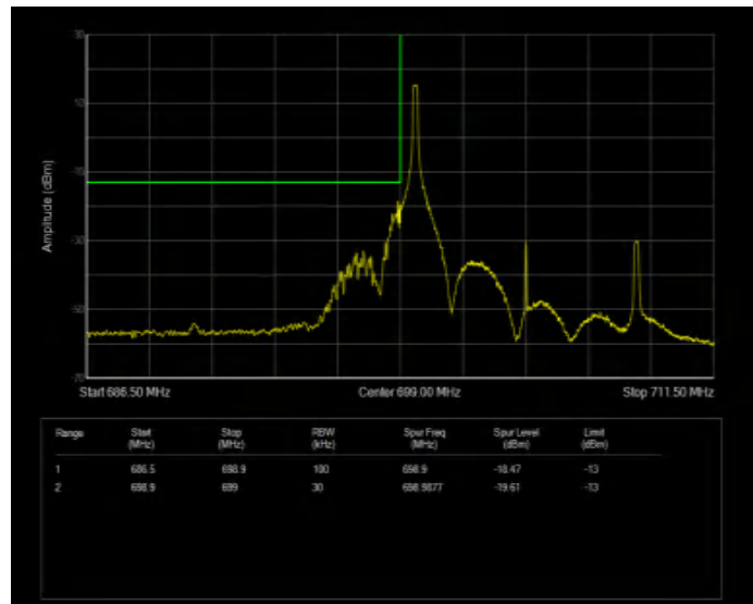
Band12 QPSK BW=10MHz Channel=23060 RB Size=1 Position=#Max Extended
