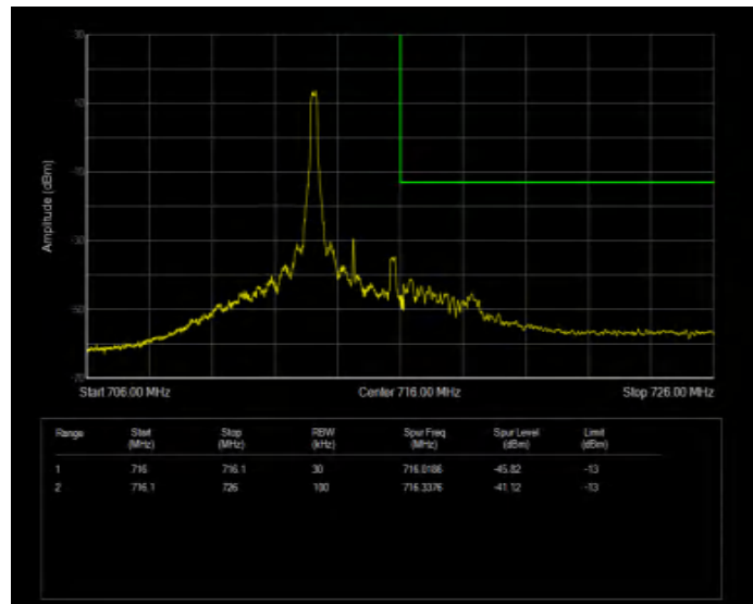
Band12 16QAM BW=3MHz Channel=23165 RB Size=1 Position=#Max Extended
