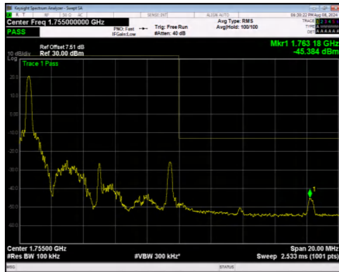
Band4 QPSK BW=10MHz Channel=20350 RB Size=1 Position=#Max Extended
