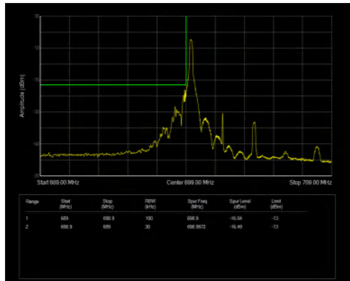
Band12 QPSK BW=5MHz Channel=23035 RB Size=1 Position=#Max Extended
