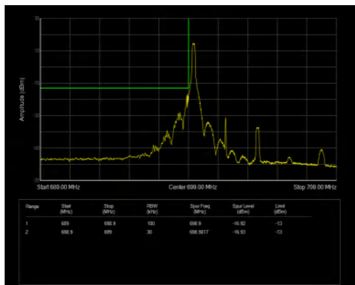
Band12 16QAM BW=5MHz Channel=23035 RB Size=1 Position=#Max Extended
