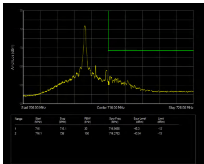
Band12 QPSK BW=3MHz Channel=23165 RB Size=1 Position=#Max Extended
