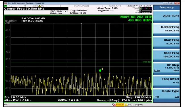
Band41_15MHz_QPSK_40740_1RB#74_0.009~0.15_0.00 9~0.15
