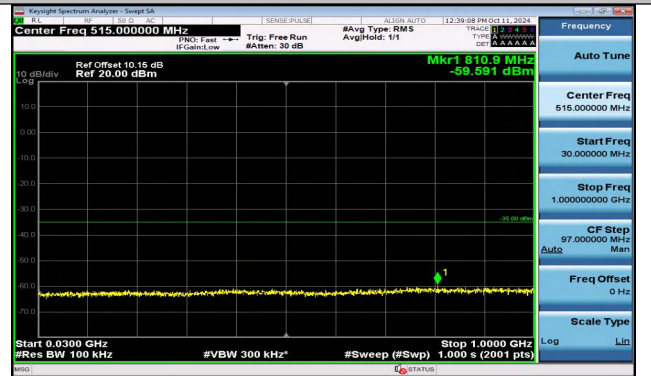
Band41_15MHz_QPSK_40740_1RB#74_30~1000_30~10 00
