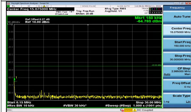
Band41_15MHz_QPSK_40740_1RB#74_0.15~30_0.15~3 0
