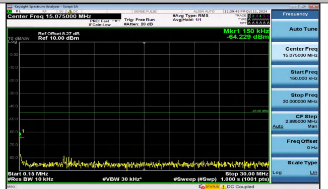
Band41_15MHz_16QAM_40740_1RB#74_0.15~30_0.15~3 30
