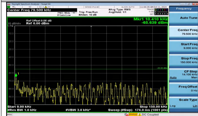
Band41_5MHz_QPSK_40740_1RB#24_0.009~0.15_0.009~0.15
