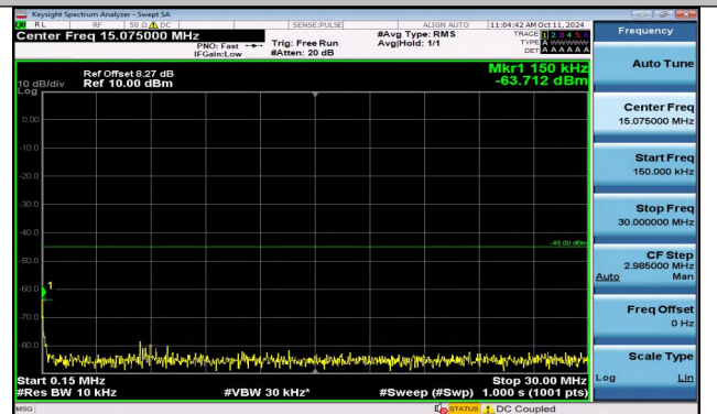
Band41_5MHz_QPSK_40740_1RB#24_0.15~30_0.15~30
