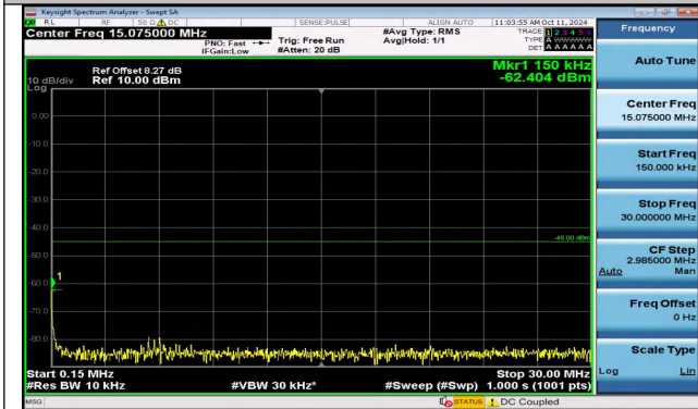
Band41_5MHz_16QAM_40740_1RB#0_0.15~30_0.15~30
