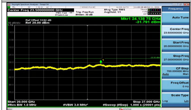
Band41_5MHz_QPSK_40265_1RB#24_20000~27000_20
