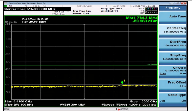
Band41_5MHz_16QAM_40740_1RB#0_30~1000_30~1000
