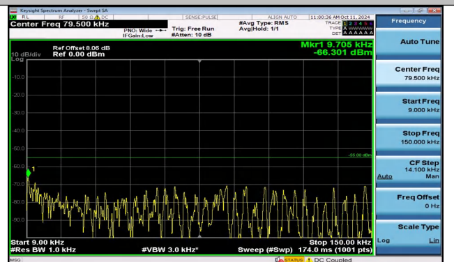
Band41_5MHz_16QAM_40265_1RB#24_0.009~0.15_0.00
