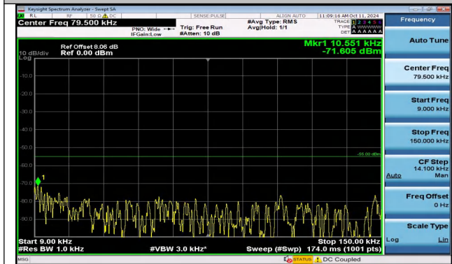
Band41_5MHz_QPSK_41215_1RB#24_0.009~0.15_0.009~0.15
