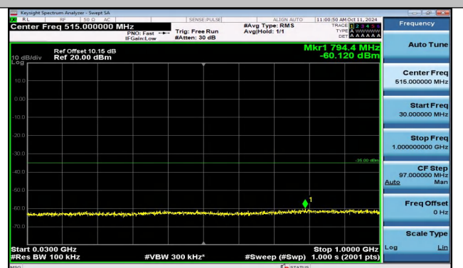
Band41_5MHz_16QAM_40265_1RB#24_30~1000_30~10
