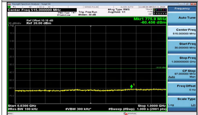
Band41_5MHz_QPSK_40265_1RB#24_30~1000_30~100
