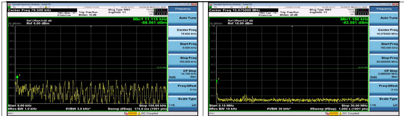
Band41_5MHz_QPSK_40265_1RB#24_0.009~0.15_0.009 ~0.15
