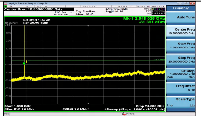
Band38_20MHz_QPSK_38150_1RB#99_1000~20000_10 00~20000
