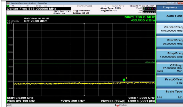
Band38_20MHz_QPSK_38150_1RB#99_30~1000_30~10 00
