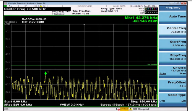
Band38_20MHz_16QAM_38150_1RB#99_0.009~0.15_0.0 09~0.15
