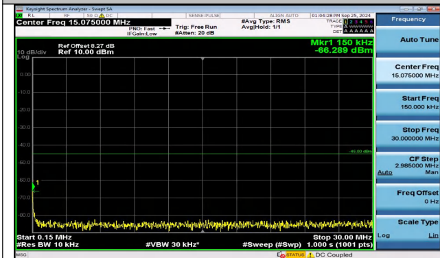
Band38_20MHz_16QAM_38150_1RB#99_0.15~30_0.15~ 30
