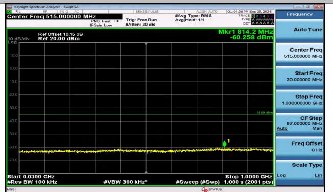
Band38_20MHz_16QAM_38150_1RB#99_30~1000_30~1 000
