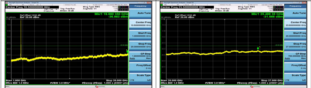
Band38_15MHz_QPSK_38000_1RB#0_1000~20000_100 0~20000
