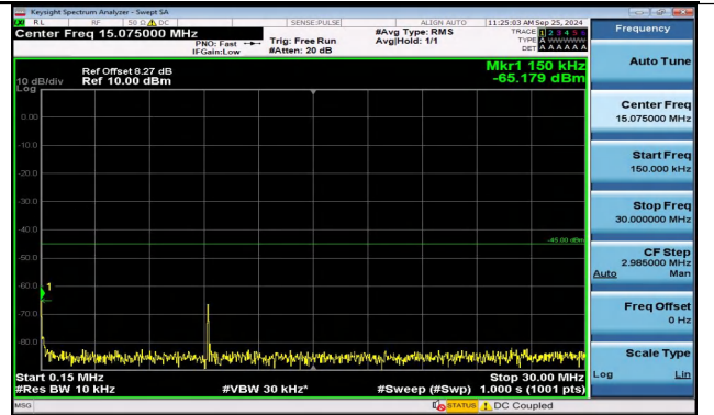
Band38_10MHz_QPSK_37800_1RB#0_0.15~30_0.15~30
