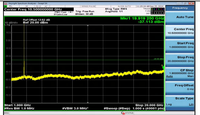
Band38_10MHz_QPSK_37800_1RB#0_1000~20000_100 0~20000
