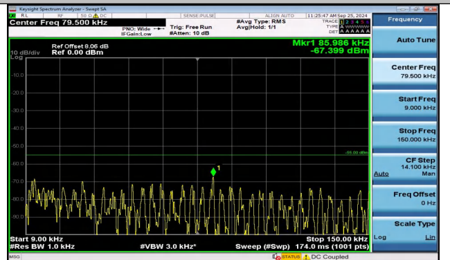
Band38_10MHz_16QAM_37800_1RB#0_0.009~0.15_0.00 9~0.15
