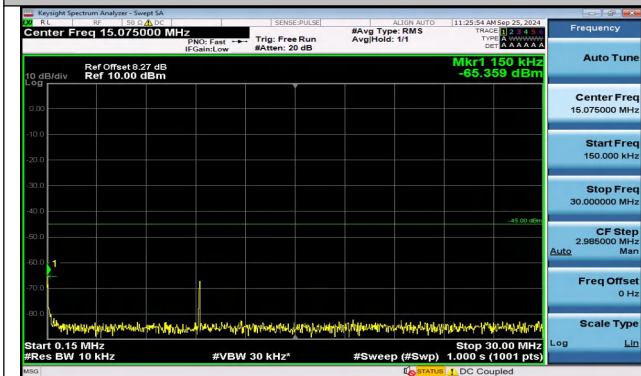
Band38_10MHz_16QAM_37800_1RB#0_0.15~30_0.15~3 0
