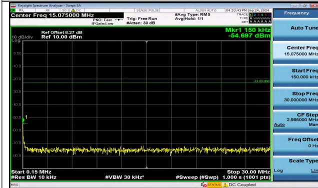
Band5_10MHz_QPSK_20525_50RB#0_0.15~30_0.15~30
