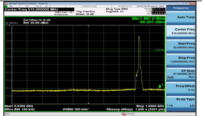
Band5_10MHz_QPSK_20525_50RB#0_30~1000_30~1000
