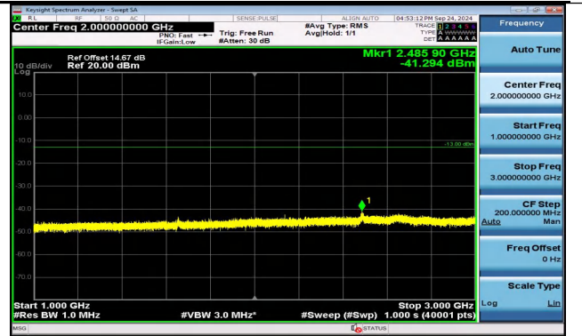
Band5_10MHz_QPSK_20450_50RB#0_1000~3000_1000~ 3000
