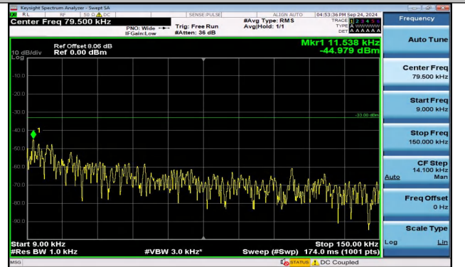
Band5_10MHz_QPSK_20525_50RB#0_0.009~0.15_0.009 ~0.15
