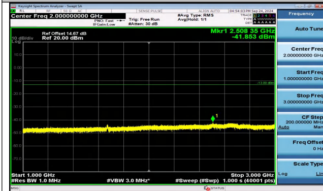
Band5_10MHz_QPSK_20525_50RB#0_1000~3000_1000~ ~3000
