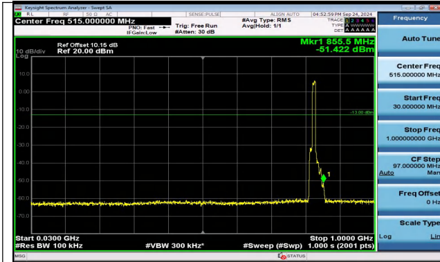
Band5_10MHz_QPSK_20450_50RB#0_30~1000_30~100 0
