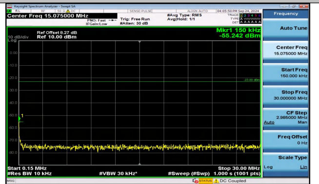
Band5_5MHz_QPSK_20525_25RB#0_0.15~30_0.15~30
