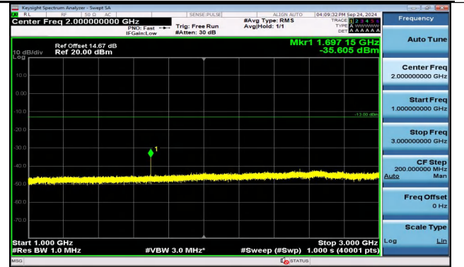
Band5_5MHz_QPSK_20625_1RB#24_1000~3000_1000~3000
