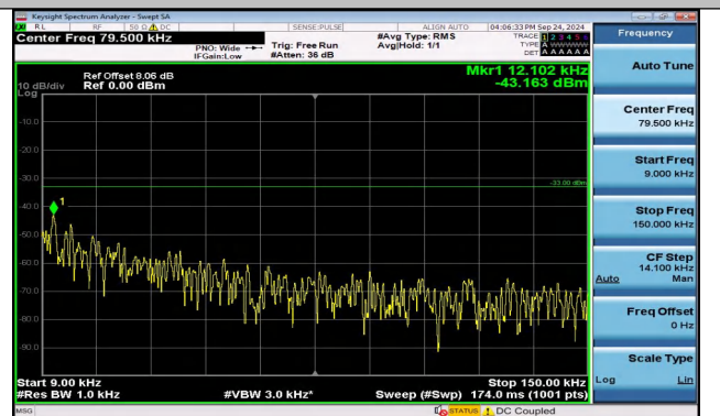
Band5_5MHz_16QAM_20525_25RB#0_0.009~0.15_0.009 ~0.15
