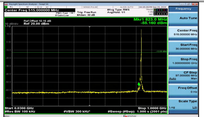
Band5_5MHz_16QAM_20525_1RB#24_30~1000_30~1000
