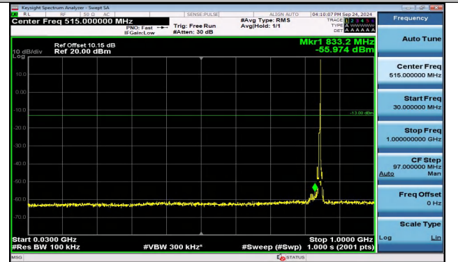
Band5_5MHz_16QAM_20625_1RB#24_30~1000_30~1000
