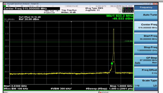
Band5_5MHz_16QAM_20625_25RB#0_30~1000_30~1000
