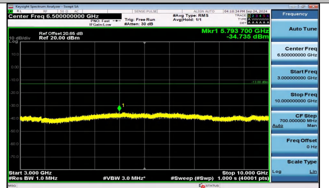
Band5_5MHz_16QAM_20625_1RB#24_3000~10000_3000~10000
