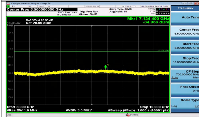
Band5_5MHz_QPSK_20625_1RB#24_3000~10000_3000~10000
