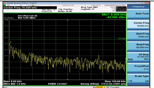
Band5_5MHz_16QAM_20525_1RB#24_0.009~0.15_0.009~0.15
