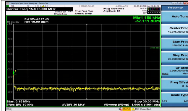
Band5_5MHz_16QAM_20525_1RB#0_0.15~30_0.15~30
