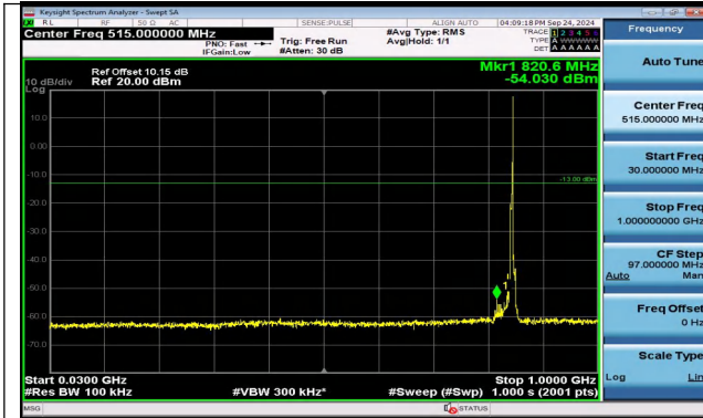
Band5_5MHz_QPSK_20625_1RB#24_30~1000_30~1000
