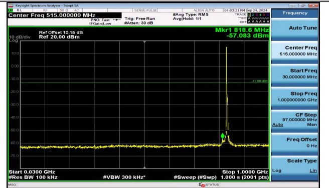
Band5_5MHz_16QAM_20525_1RB#0_30~1000_30~1000
