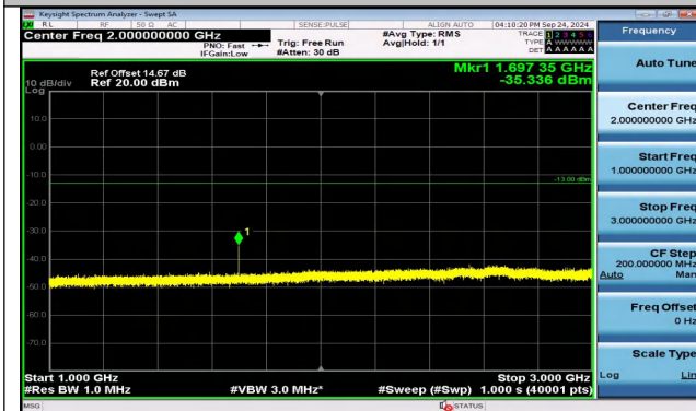
Band5_5MHz_16QAM_20625_1RB#24_1000~3000_1000~3000
