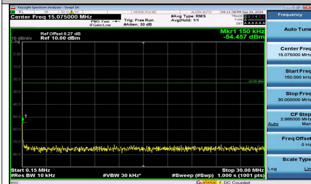
Band5_5MHz_16QAM_20625_25RB#0_0.15~30_0.15~30
