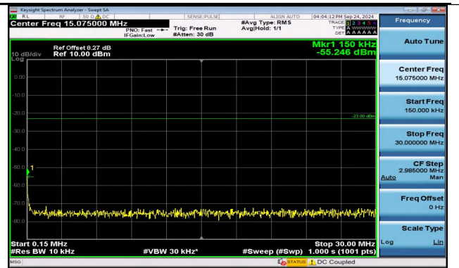
Band5_5MHz_QPSK_20525_1RB#24_0.15~30_0.15~30
