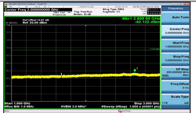
Band5_5MHz_QPSK_20525_25RB#0_1000~3000_1000~3000
