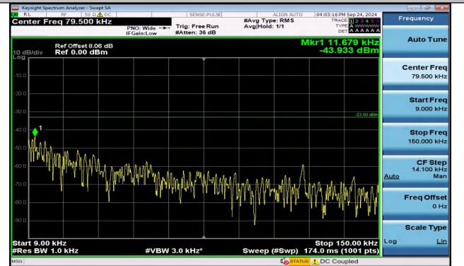
Band5_5MHz_16QAM_20525_1RB#0_0.009~0.15_0.009~0.15
