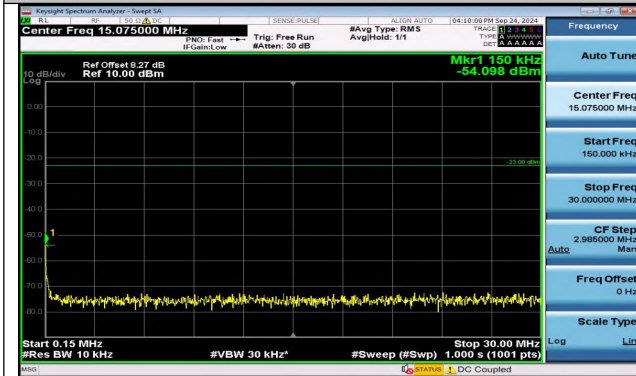
Band5_5MHz_16QAM_20625_1RB#24_0.15~30_0.15~30
