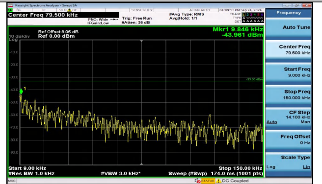
Band5_5MHz_16QAM_20625_1RB#24_0.009~0.15_0.009~0.15
