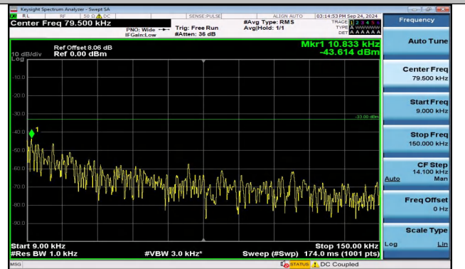
Band5_3MHz_16QAM_20525_15RB#0_0.009~0.15_0.009~0.15
