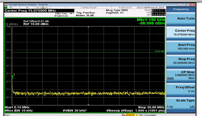
Band5_3MHz_QPSK_20525_1RB#14_0.15~30_0.15~30
