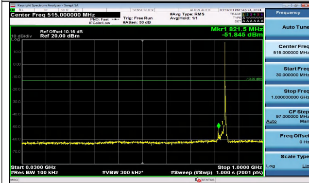
Band5_3MHz_QPSK_20635_1RB#0_30~1000_30~1000
