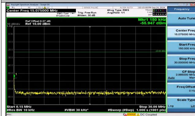
Band5_3MHz_16QAM_20525_15RB#0_0.15~30_0.15~30
