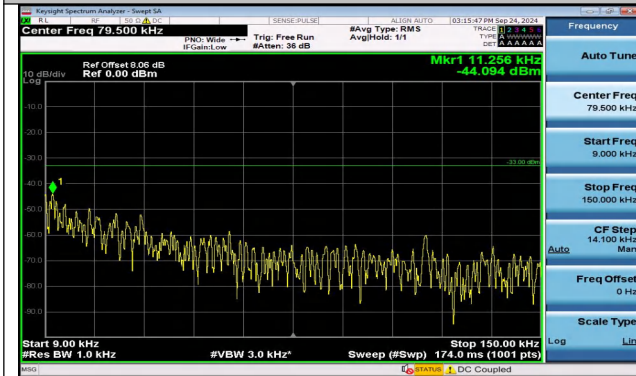
Band5_3MHz_QPSK_20635_1RB#0_0.009~0.15_0.009~ 0.15
