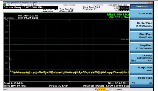
Band5_3MHz_QPSK_20525_1RB#0_0.15~30_0.15~30
