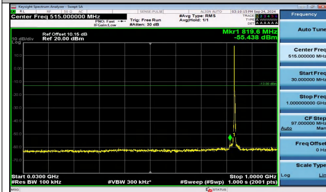
Band5_3MHz_QPSK_20525_1RB#0_30~1000_30~1000
