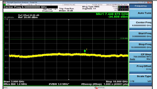
Band5_3MHz_16QAM_20525_1RB#0_3000~10000_3000~10000
