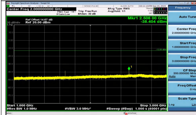
Band5_3MHz_16QAM_20525_1RB#0_1000~3000_1000~3000
