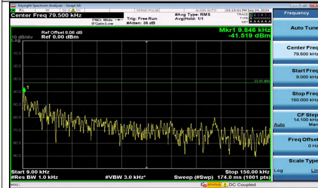
Band5_3MHz_QPSK_20525_1RB#0_0.009~0.15_0.009~0.15 0.15
