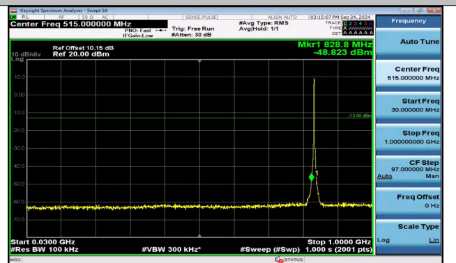
Band5_3MHz_16QAM_20525_15RB#0_30~1000_30~1000
