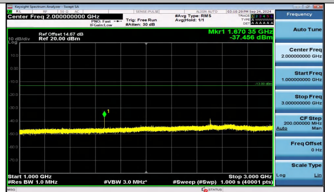
Band5_3MHz_QPSK_20525_1RB#0_1000~3000_1000~3000 00
