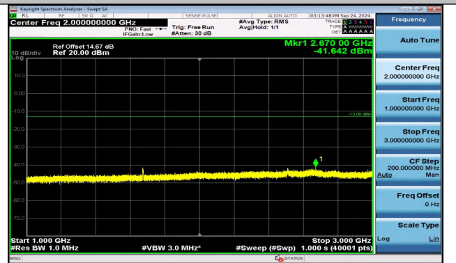
Band5_3MHz_QPSK_20525_15RB#0_1000~3000_1000~3000
