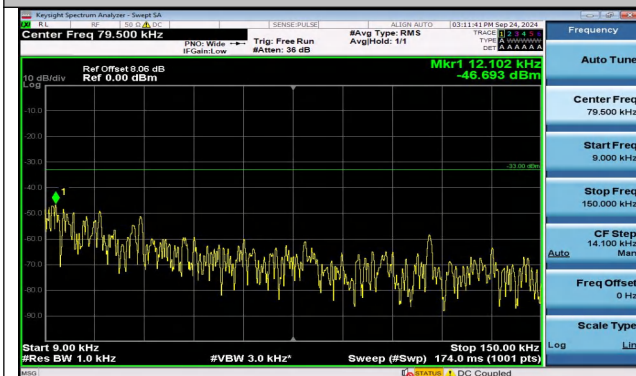
Band5_3MHz_QPSK_20525_1RB#14_0.009~0.15_0.009~0.15
