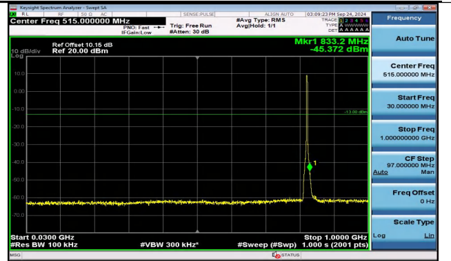
Band5_3MHz_16QAM_20415_15RB#0_30~1000_30~100 0
