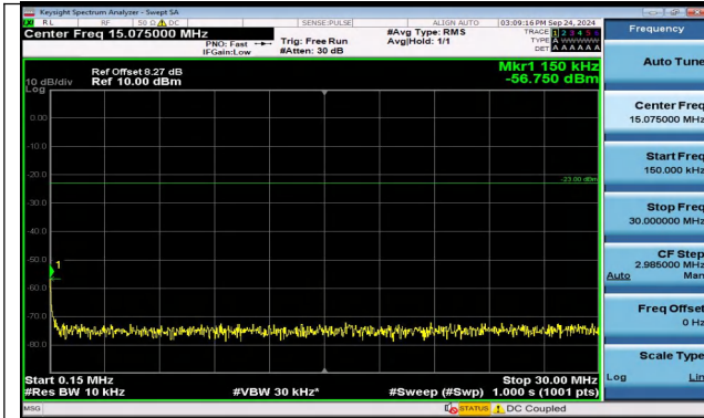
Band5_3MHz_16QAM_20415_15RB#0_0.15~30_0.15~3 0
