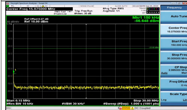
Band5_3MHz_16QAM_20525_1RB#0_0.15~30_0.15~30
