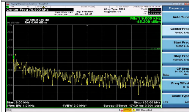
Band5_1.4MHz_QPSK_20643_1RB#5_0.009~0.15_0.009 ~0.15
