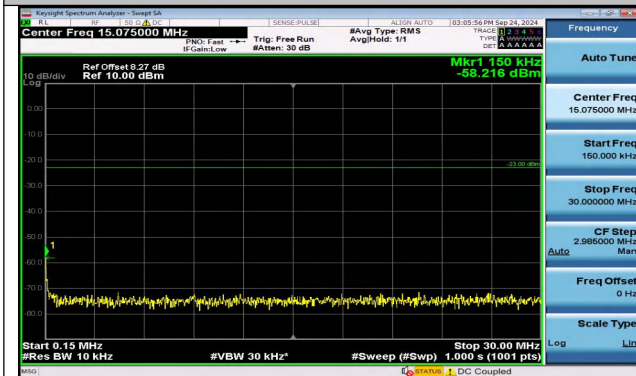
Band5_3MHz_16QAM_20415_1RB#0_0.15~30_0.15~30
