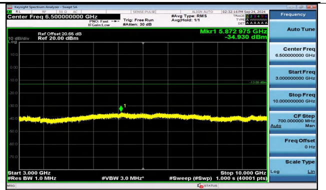
Band5_1.4MHz_16QAM_20643_1RB#0_3000~10000_300 0~10000
