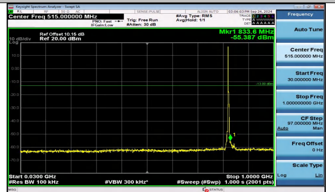
Band5_3MHz_16QAM_20415_1RB#0_30~1000_30~1000
