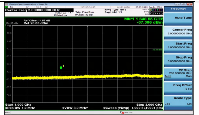
Band5_3MHz_QPSK_20415_1RB#0_1000~3000_1000~3000
