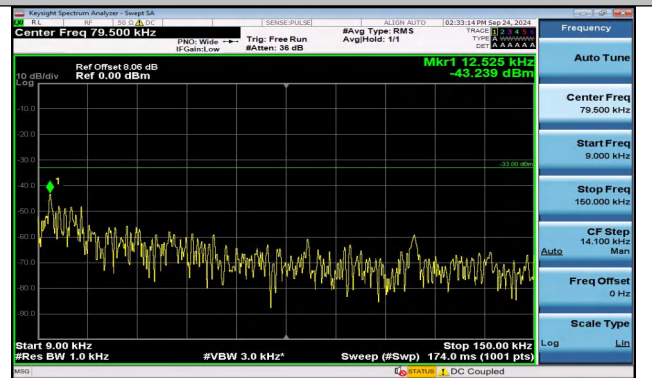
Band5_1.4MHz_16QAM_20643_1RB#5_0.009~0.15_0.009 ~0.15
