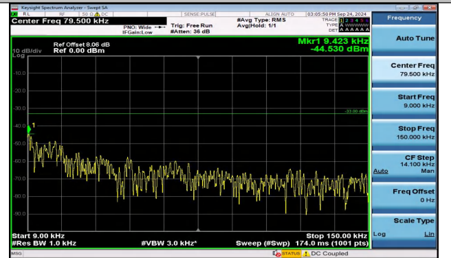
Band5_3MHz_16QAM_20415_1RB#0_0.009~0.15_0.009~0.15
