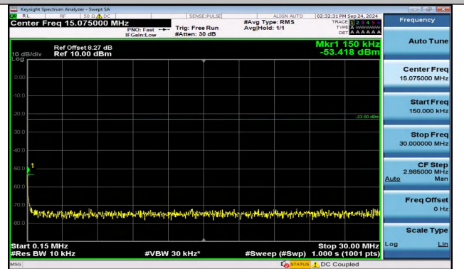
Band5_1.4MHz_QPSK_20643_1RB#5_0.15~30_0.15~30
