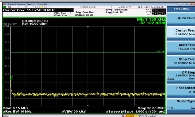
Band5_1.4MHz_16QAM_20643_1RB#0_0.15~30_0.15~30
