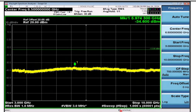
Band5_3MHz_16QAM_20415_1RB#0_3000~10000_3000~10000
