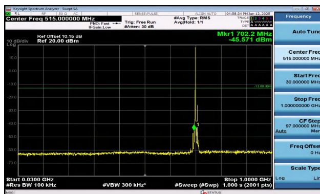
Band17-10MHz-16QAM-23800-1RB#0-30~1000-PASS
