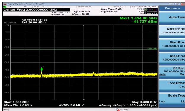
Band17-10MHz-QPSK-23800-50RB#0-1000~3000-PASS
