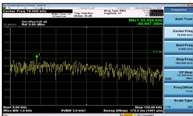
Band17-10MHz-QPSK-23800-50RB#0-0.009~0.15-PASS
