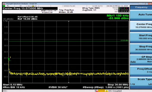
Band17-10MHz-QPSK-23800-1RB#49-0.15~30-PASS
