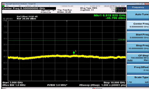
Band17-10MHz-QPSK-23800-50RB#0-3000~10000-PASS
