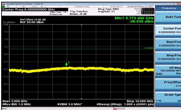
Band17-10MHz-16QAM-23790-1RB#0-3000~10000-PASS
