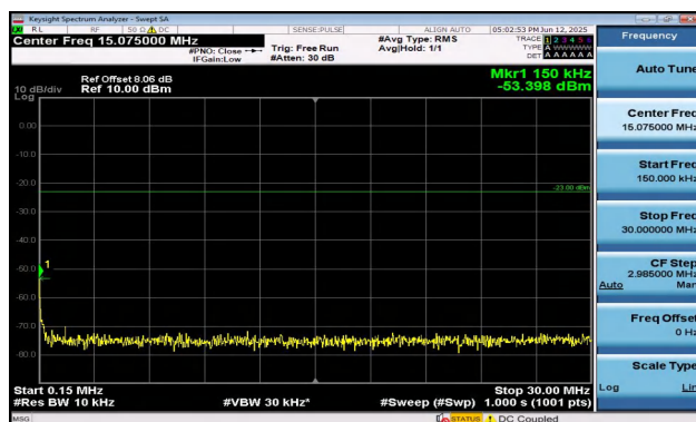
Band17-10MHz-QPSK-23800-50RB#0-0.15~30-PASS
