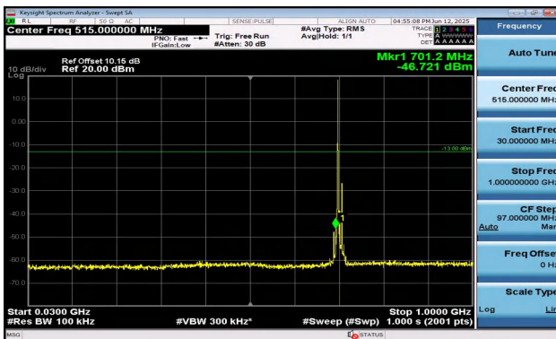
Band17-10MHz-16QAM-23790-1RB#0-30~1000-PASS
