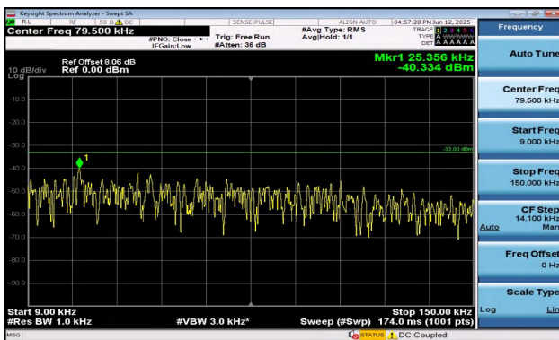
Band17-10MHz-QPSK-23800-1RB#0-0.009~0.15-PASS
