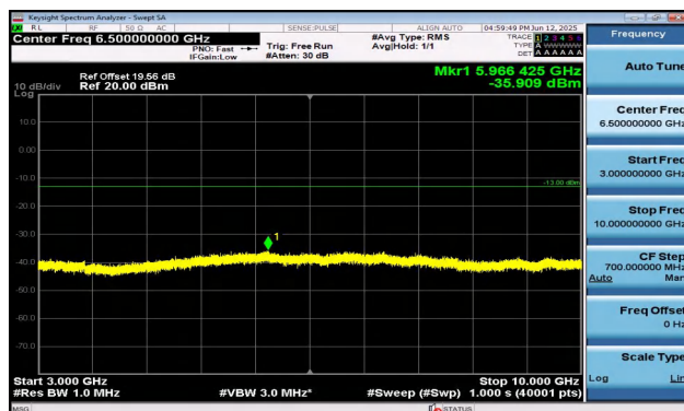
Band17-10MHz-QPSK-23800-1RB#49-3000~10000-PASS
