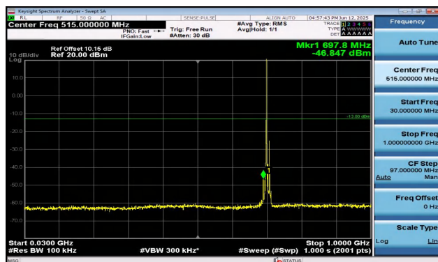
Band17-10MHz-QPSK-23800-1RB#0-30~1000-PASS
