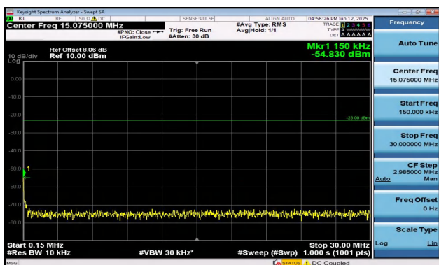
Band17-10MHz-16QAM-23800-1RB#0-0.15~30-PASS
