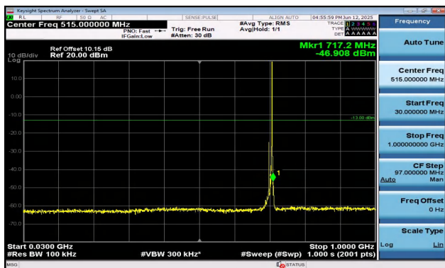
Band17-10MHz-QPSK-23790-1RB#49-30~1000-PASS
