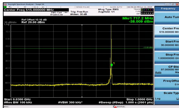
Band17-10MHz-QPSK-23800-1RB#49-30~1000-PASS
