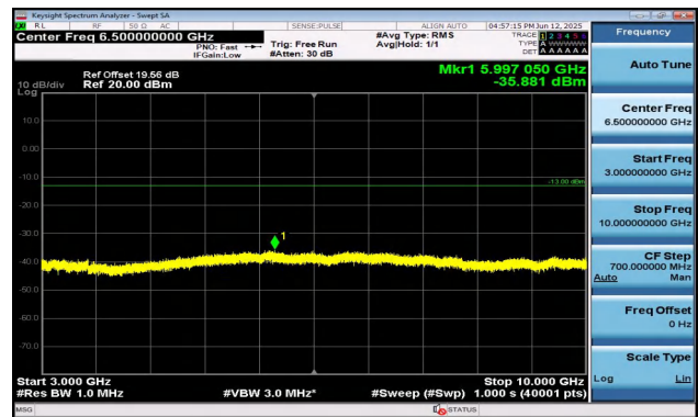
Band17-10MHz-16QAM-23790-1RB#49-3000~10000-PASS
