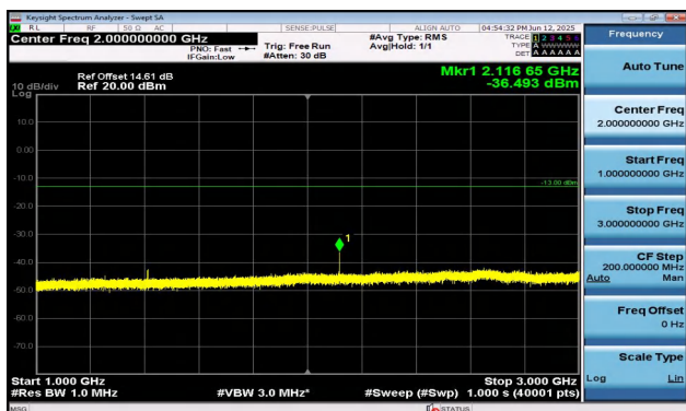
Band17-10MHz-QPSK-23790-1RB#0-1000~3000-PASS
