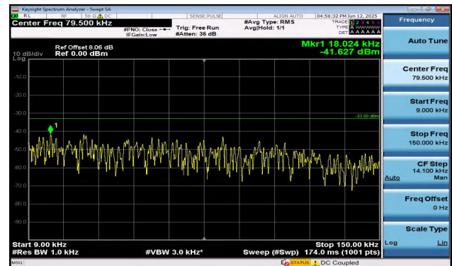
Band17-10MHz-16QAM-23790-1RB#49-0.009~0.15-PASS
