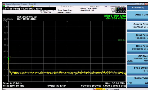
Band17-10MHz-QPSK-23790-1RB#49-0.15~30-PASS
