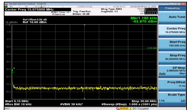
Band17-10MHz-16QAM-23790-1RB#0-0.15~30-PASS
