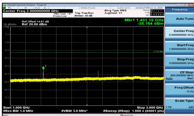
Band17-10MHz-QPSK-23800-1RB#49-1000~3000-PASS
