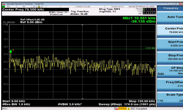
Band17-10MHz-16QAM-23790-1RB#0-0.009~0.15-PASS
