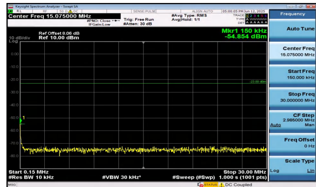
Band17-10MHz-16QAM-23800-1RB#49-0.15~30-PASS
