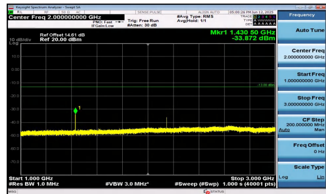
Band17-10MHz-16QAM-23800-1RB#49-1000~3000-PASS
