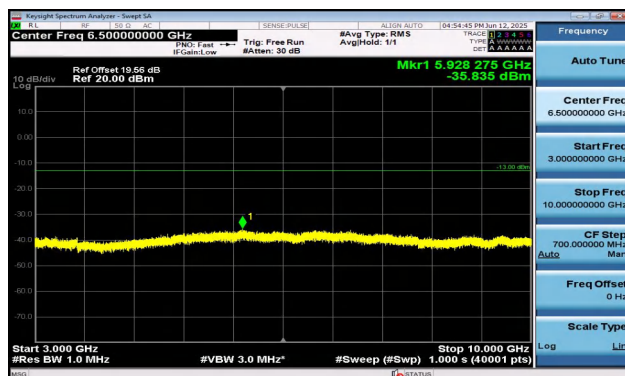
Band17-10MHz-QPSK-23790-1RB#0-3000~10000-PASS
