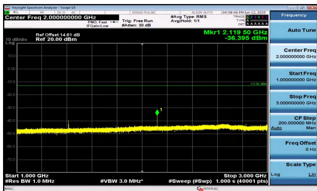
Band17-10MHz-16QAM-23800-1RB#0-1000~3000-PASS
