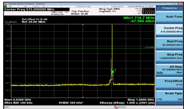
Band17-10MHz-16QAM-23790-1RB#49-30~1000-PASS
