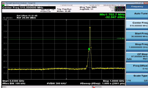
Band17-10MHz-QPSK-23800-50RB#0-30~1000-PASS
