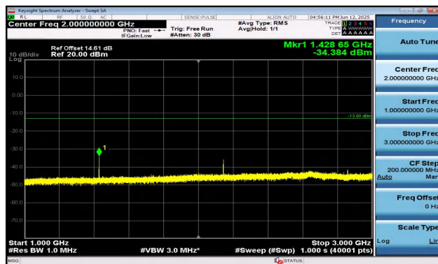
Band17-10MHz-QPSK-23790-1RB#49-1000~3000-PASS
