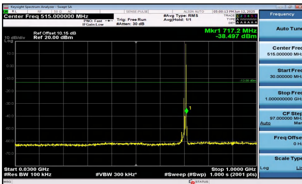
Band17-10MHz-16QAM-23800-1RB#49-30~1000-PASS
