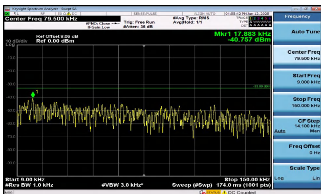
Band17-10MHz-QPSK-23790-1RB#49-0.009~0.15-PASS
