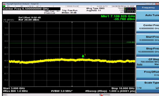
Band17-10MHz-16QAM-23800-1RB#0-3000~10000-PASS
