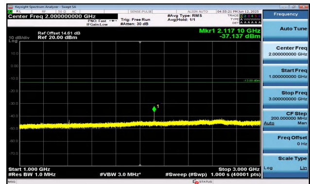
Band17-10MHz-16QAM-23790-1RB#0-1000~3000-PASS
