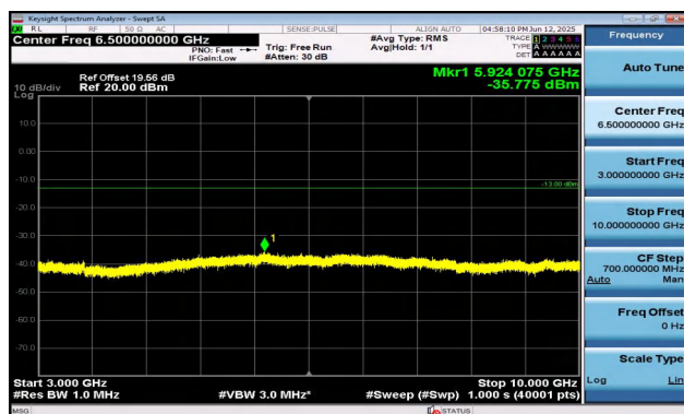
Band17-10MHz-QPSK-23800-1RB#0-3000~10000-PASS
