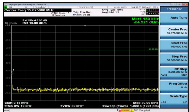
Band17-10MHz-QPSK-23800-1RB#0-0.15~30-PASS
