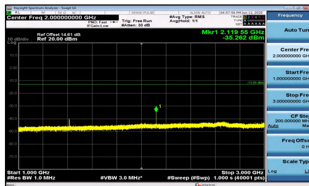
Band17-10MHz-QPSK-23800-1RB#0-1000~3000-PASS
