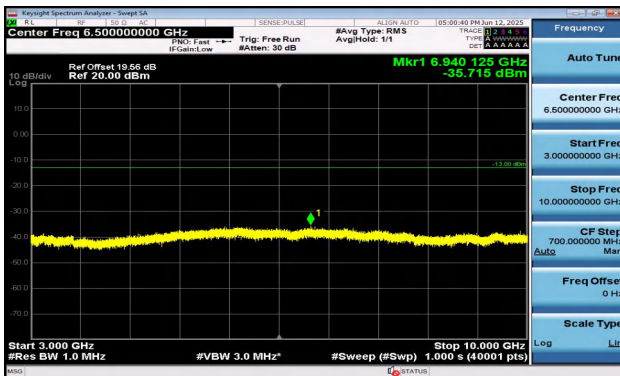
Band17-10MHz-16QAM-23800-1RB#49-3000~10000-PAS
