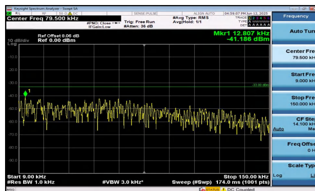
Band17-10MHz-QPSK-23800-1RB#49-0.009~0.15-PASS
