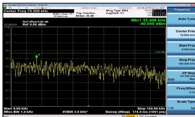
Band17-10MHz-16QAM-23800-1RB#0-0.009~0.15-PASS
