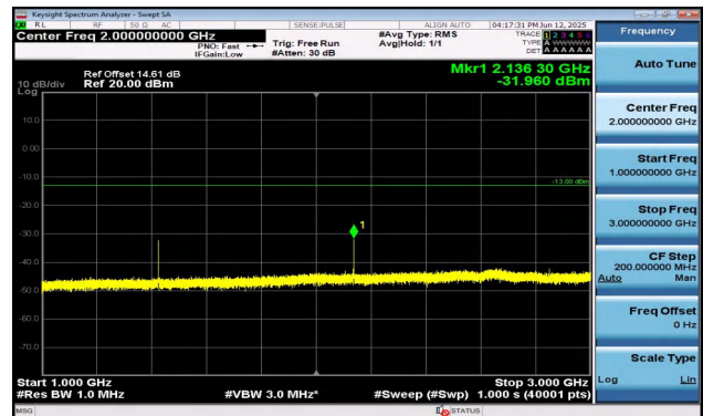
Band17-5MHz-16QAM-23790-1RB#24-1000~3000-PASS
