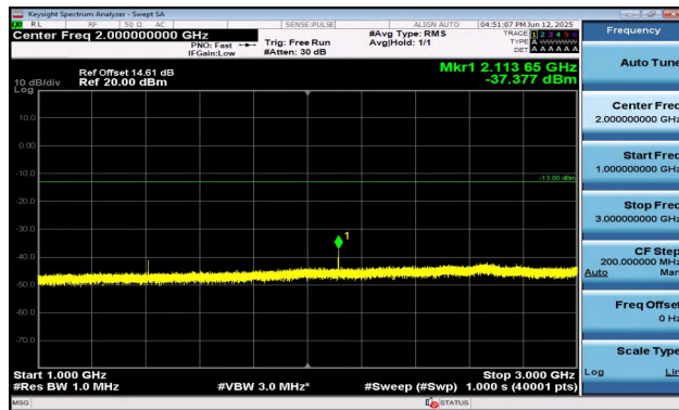
Band17-10MHz-QPSK-23780-1RB#0-1000~3000-PASS
