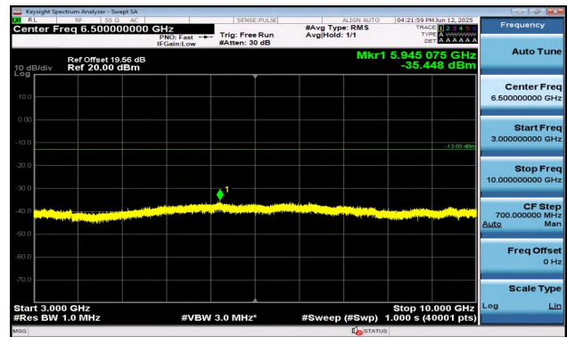
Band17-5MHz-QPSK-23825-1RB#24-3000~10000-PASS
