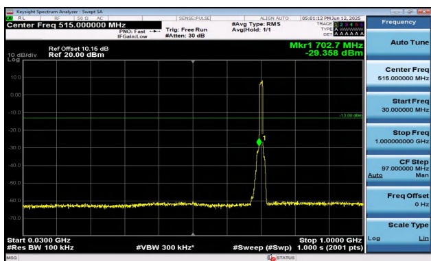
Band17-10MHz-QPSK-23780-50RB#0-0.30~1000-PASS
