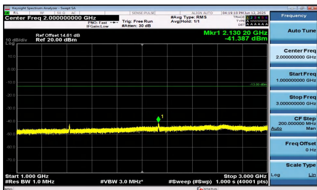
Band17-5MHz-16QAM-23790-25RB#0-1000~3000-PASS
