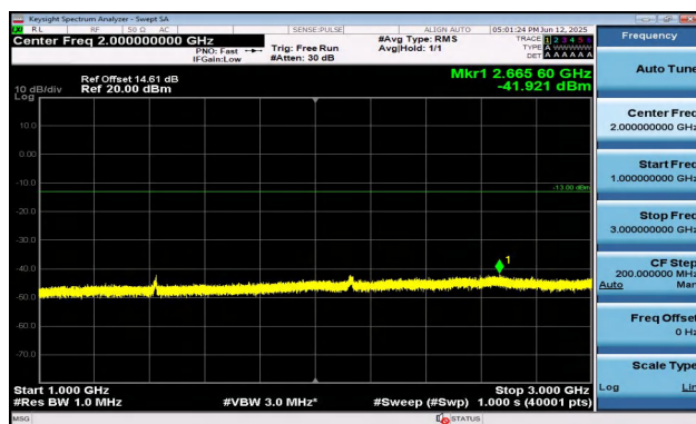
Band17-10MHz-QPSK-23780-50RB#0-1000~3000-PASS
