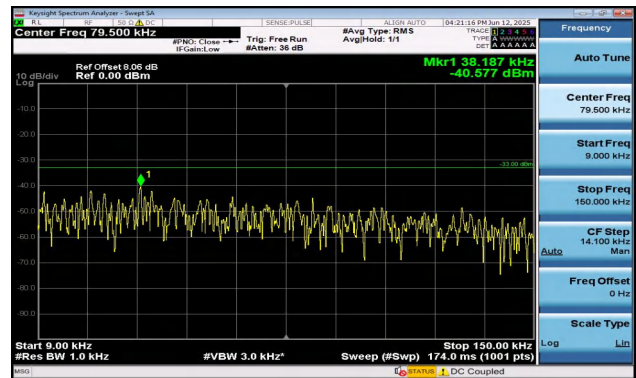
Band17-5MHz-QPSK-23825-1RB#24-0.009~0.15-PASS
