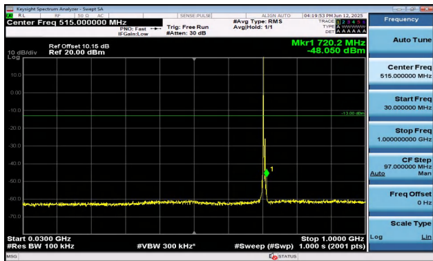
Band17-5MHz-QPSK-23825-1RB#0-30~1000-PASS
