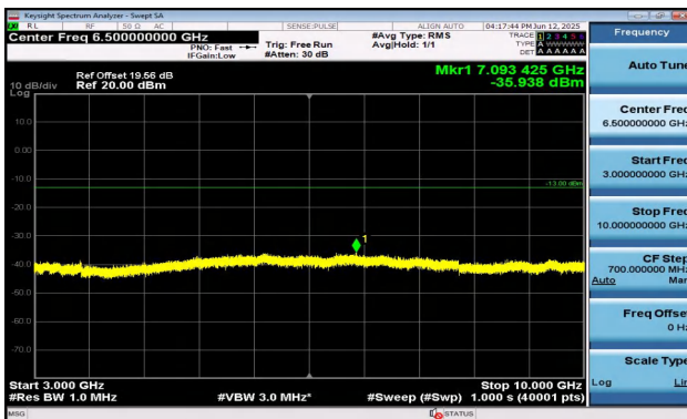
Band17-5MHz-16QAM-23790-1RB#24-3000~10000-PASS
