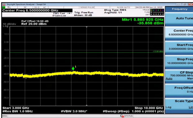
Band17-10MHz-16QAM-23780-1RB#49-3000~10000-PASS
