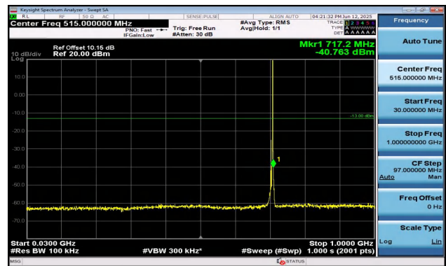
Band17-5MHz-QPSK-23825-1RB#24-30~1000-PASS
