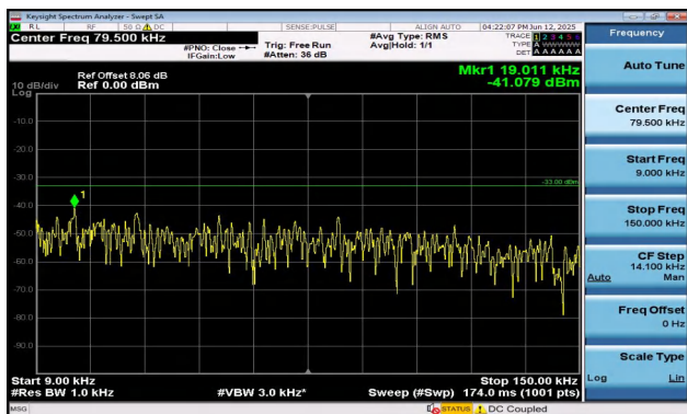
Band17-5MHz-16QAM-23825-1RB#24-0.009~0.15-PASS
