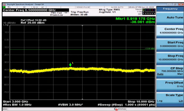
Band17-10MHz-QPSK-23780-50RB#0-3000~10000-PASS
