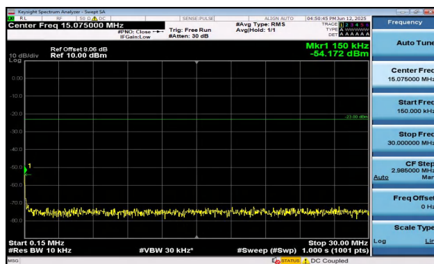
Band17-10MHz-QPSK-23780-1RB#0-0.15~30-PASS
