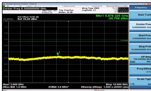
Band17-5MHz-16QAM-23790-25RB#0-3000~10000-PASS
