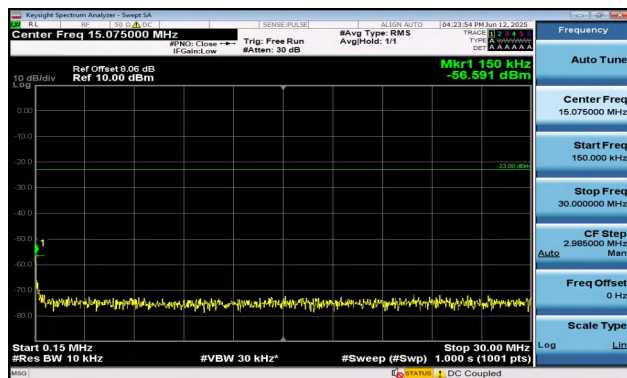
Band17-5MHz-16QAM-23825-25RB#0-0.15~30-PASS
