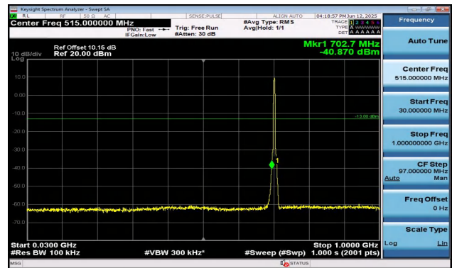
Band17-5MHz-16QAM-23790-25RB#0-30~1000-PASS
