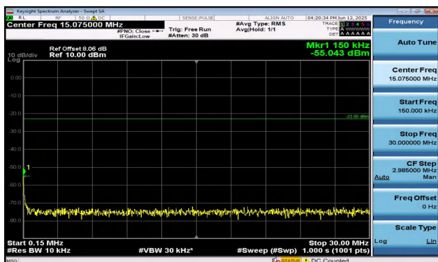
Band17-5MHz-16QAM-23825-1RB#0-0.15~30-PASS
