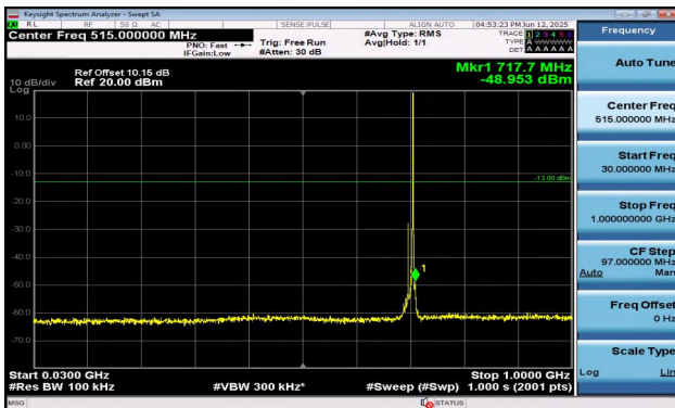
Band17-10MHz-16QAM-23780-1RB#49-30~1000-PASS
