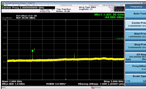
Band17-5MHz-QPSK-23825-1RB#24-1000~3000-PASS
