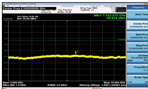
Band17-5MHz-16QAM-23825-25RB#0-3000~10000-PASS
