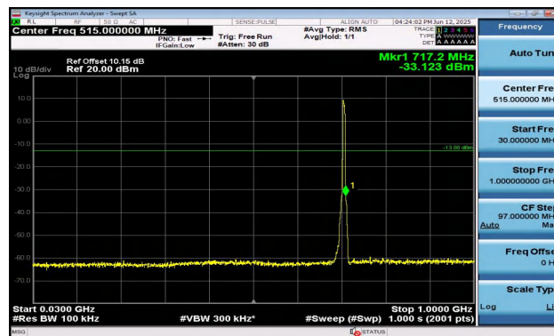
Band17-5MHz-16QAM-23825-25RB#0-30~1000-PASS
