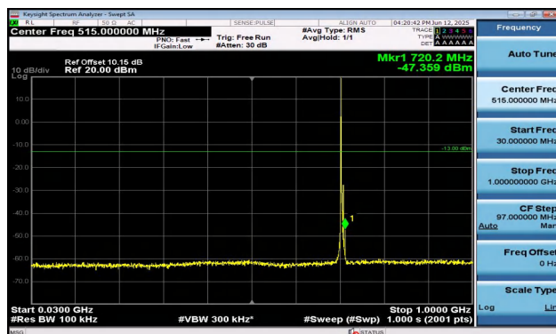
Band17-5MHz-16QAM-23825-1RB#0-30~1000-PASS
