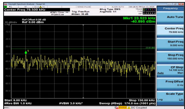
Band17-5MHz-16QAM-23790-25RB#0-0.009~0.15-PASS
