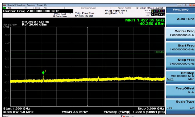
Band17-5MHz-16QAM-23825-25RB#0-1000~3000-PASS
