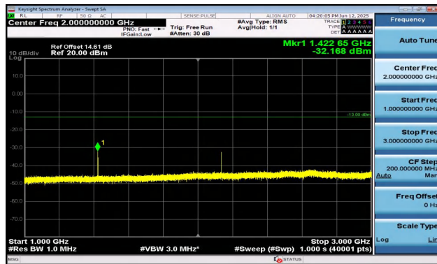
Band17-5MHz-QPSK-23825-1RB#0-1000~3000-PASS
