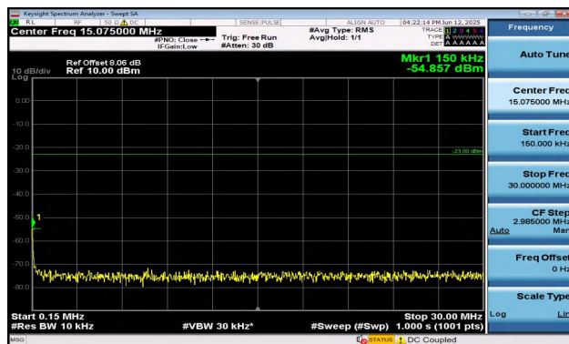
Band17-5MHz-16QAM-23825-1RB#24-0.15~30-PASS
