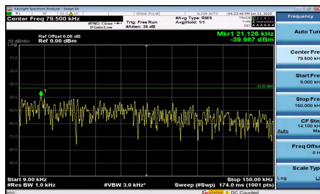
Band17-5MHz-16QAM-23825-25RB#0-0.009~0.15-PASS
