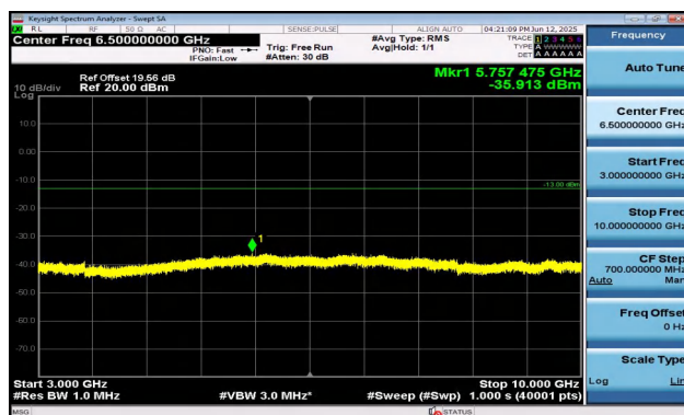
Band17-5MHz-16QAM-23825-1RB#0-3000~10000-PASS
