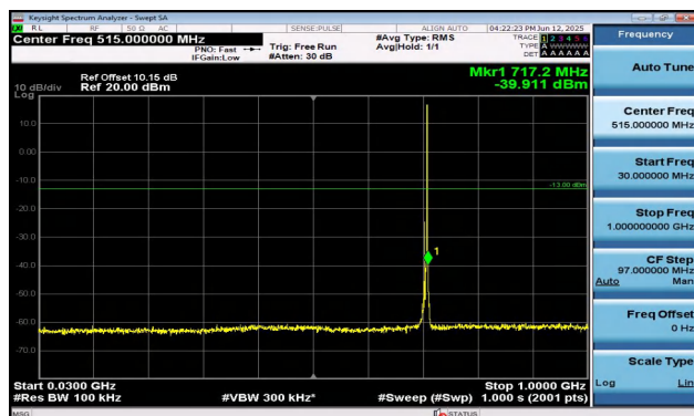
Band17-5MHz-16QAM-23825-1RB#24-30~1000-PASS
