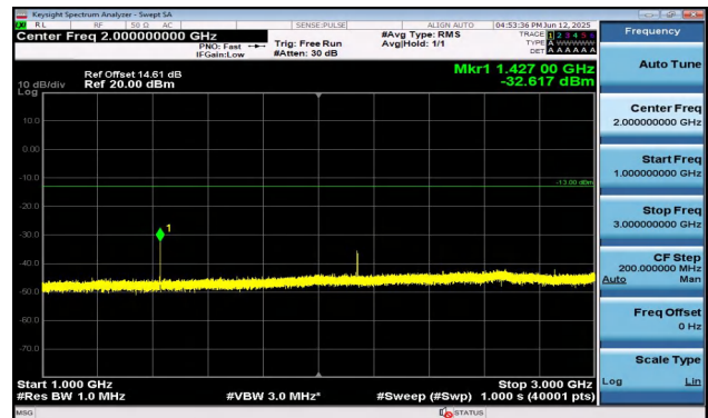
Band17-10MHz-16QAM-23780-1RB#49-1000~3000-PASS
