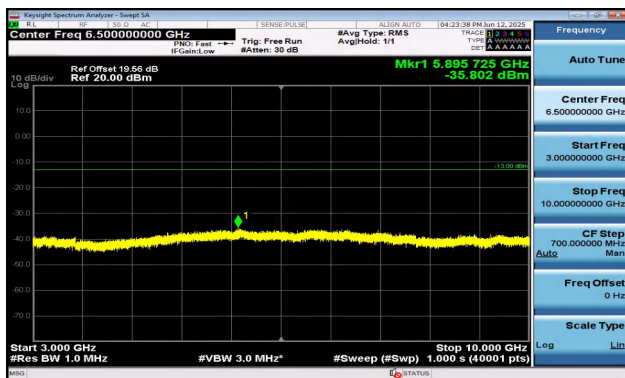
Band17-5MHz-QPSK-23825-25RB#0-3000~10000-PASS
