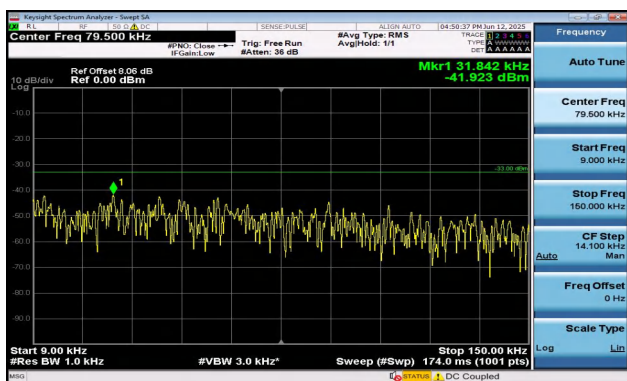
Band17-10MHz-QPSK-23780-1RB#0-0.009~0.15-PASS
