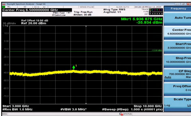
Band17-5MHz-QPSK-23825-1RB#0-3000~10000-PASS
