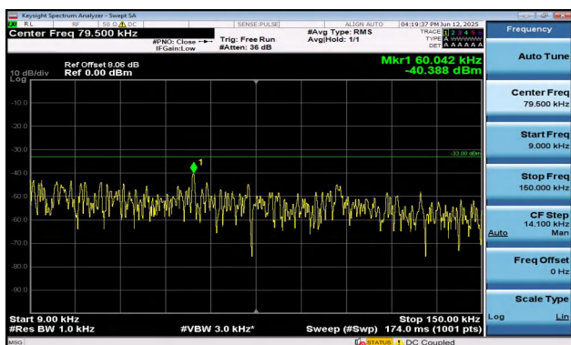
Band17-5MHz-QPSK-23825-1RB#0-0.009~0.15-PASS
