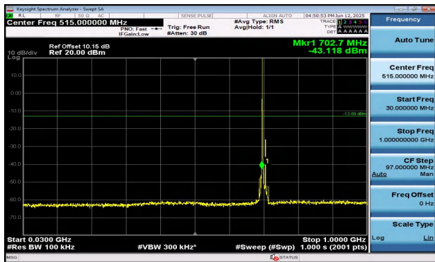
Band17-10MHz-QPSK-23780-1RB#0-30~1000-PASS
