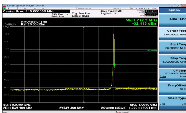
Band17-5MHz-QPSK-23825-25RB#0-30~1000-PASS
