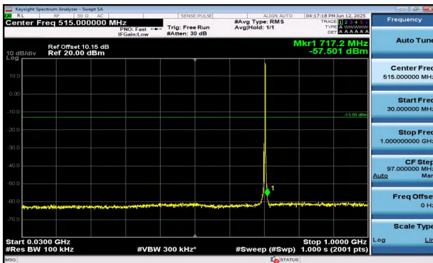
Band17-5MHz-16QAM-23790-1RB#24-30~1000-PASS
