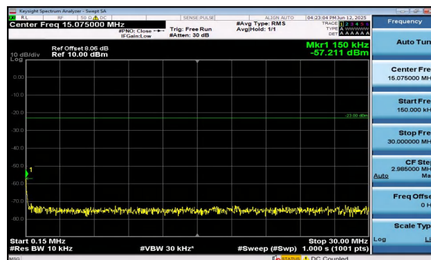
Band17-5MHz-QPSK-23825-25RB#0-0.15~30-PASS
