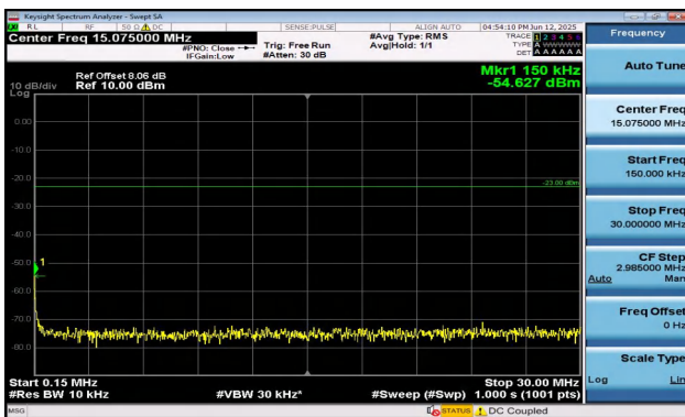
Band17-10MHz-QPSK-23790-1RB#0-0.15~30-PASS
