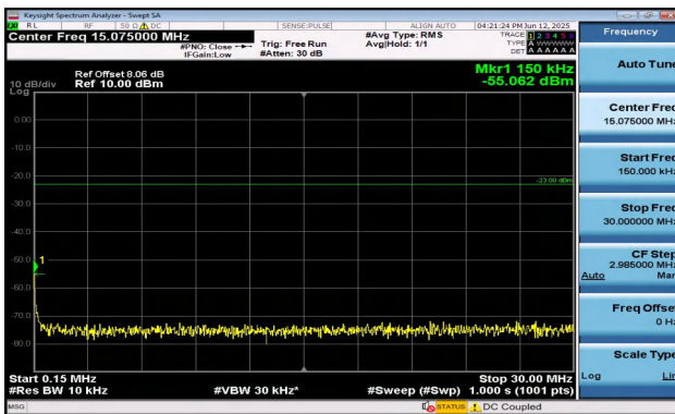
Band17-5MHz-QPSK-23825-1RB#24-0.15~30-PASS
