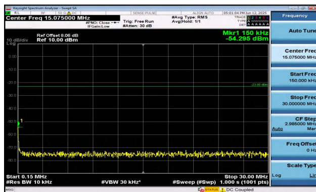
Band17-10MHz-QPSK-23780-50RB#0-0.15~30-PASS
