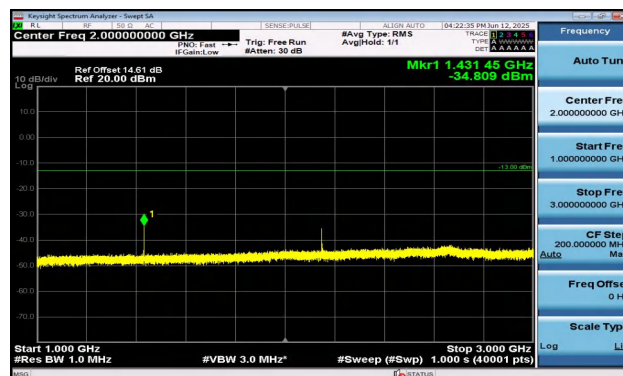
Band17-5MHz-16QAM-23825-1RB#24-1000~3000-PASS
