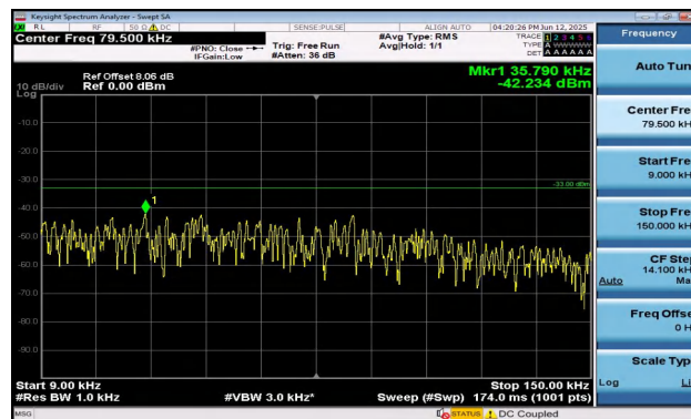
Band17-5MHz-16QAM-23825-1RB#0-0.009~0.15-PASS
