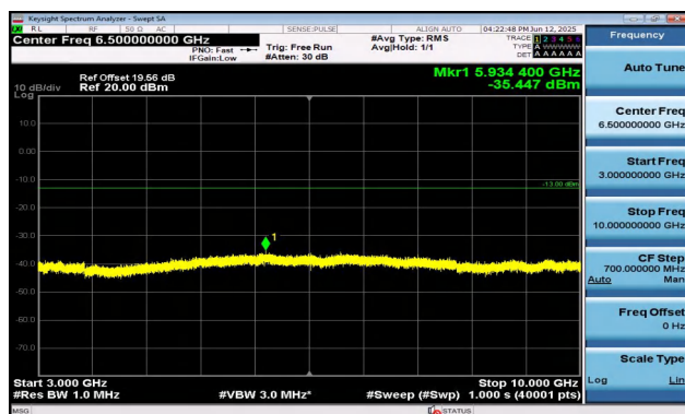
Band17-5MHz-16QAM-23825-1RB#24-3000~10000-PASS
