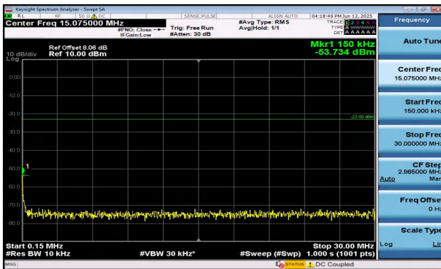
Band17-5MHz-16QAM-23790-25RB#0-0.15~30-PASS
