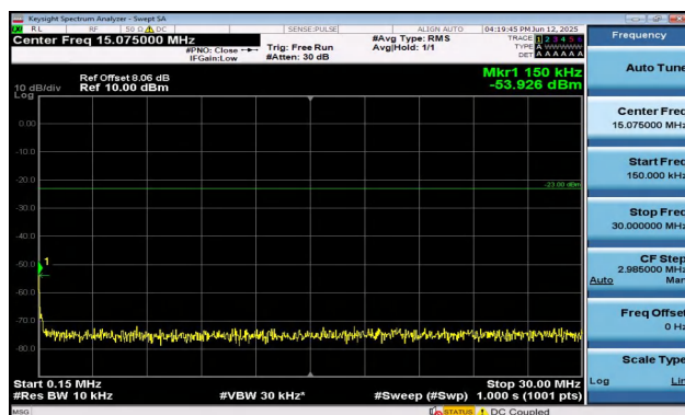
Band17-5MHz-QPSK-23825-1RB#0-0.15~30-PASS
