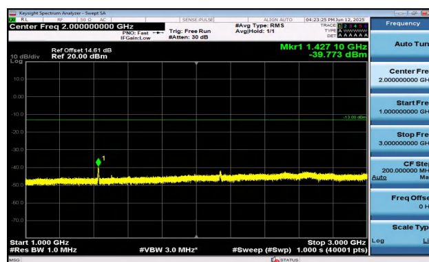
Band17-5MHz-QPSK-23825-25RB#0-1000~3000-PASS
