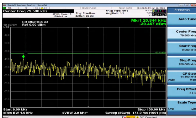
Band17-5MHz-QPSK-23825-25RB#0-0.009~0.15-PASS
