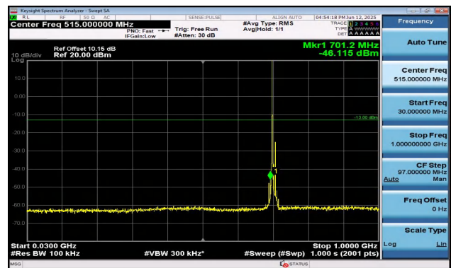
Band17-10MHz-QPSK-23790-1RB#0-30~1000-PASS
