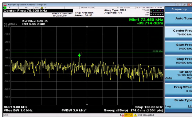
Band17-10MHz-16QAM-23780-1RB#0-0.009~0.15-PASS
