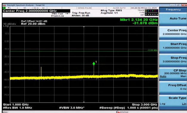
Band17-5MHz-16QAM-23825-1RB#0-1000~3000-PASS
