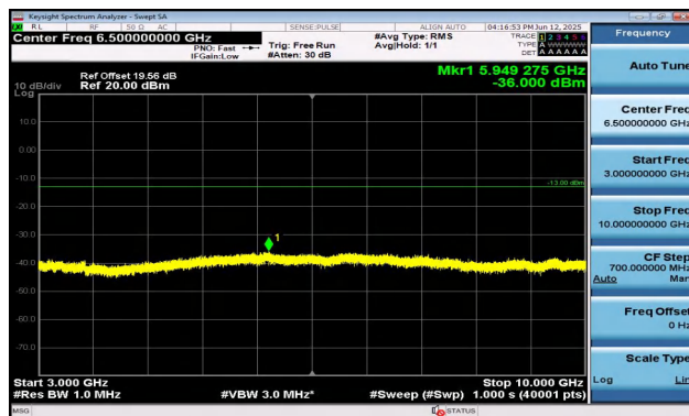
Band17-5MHz-QPSK-23790-1RB#24-3000~10000-PASS
