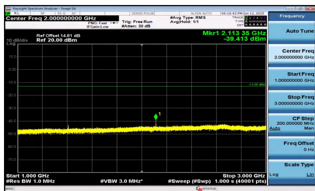
Band17-5MHz-16QAM-23755-1RB#0-1000~3000-PASS
