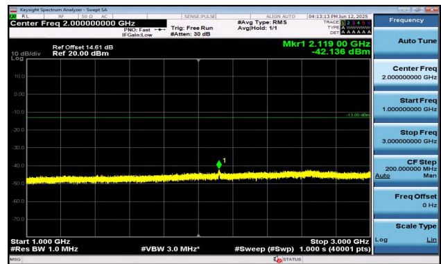
Band17-5MHz-QPSK-23755-25RB#0-1000~3000-PASS
