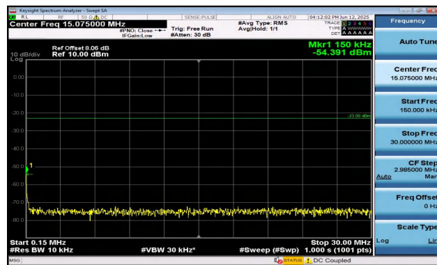
Band17-5MHz-16QAM-23755-1RB#24-0.15~30-PASS
