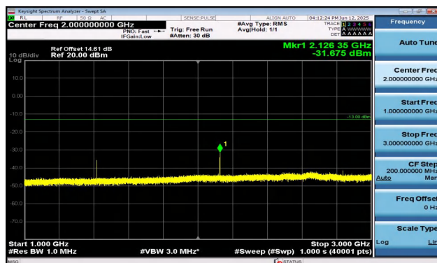
Band17-5MHz-16QAM-23755-1RB#24-1000~3000-PASS
