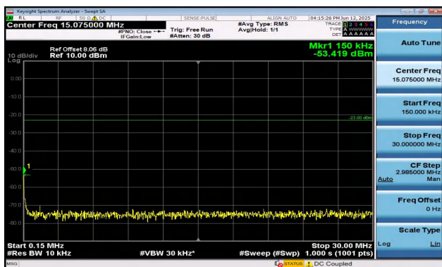
Band17-5MHz-16QAM-23790-1RB#0-0.15~30-PASS
