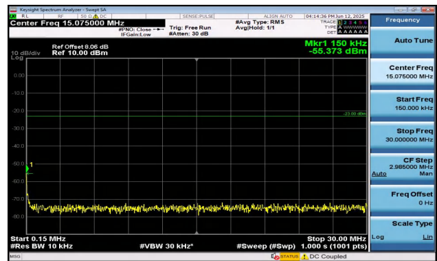
Band17-5MHz-QPSK-23790-1RB#0-0.15~30-PASS
