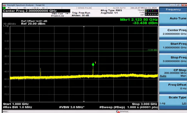
Band17-5MHz-16QAM-23790-1RB#0-1000~3000-PASS
