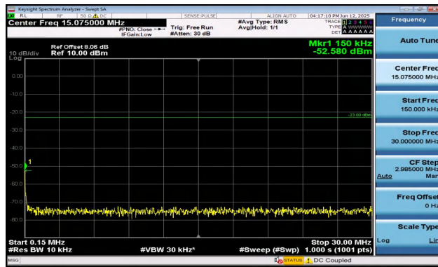
Band17-5MHz-16QAM-23790-1RB#24-0.15~30-PASS
