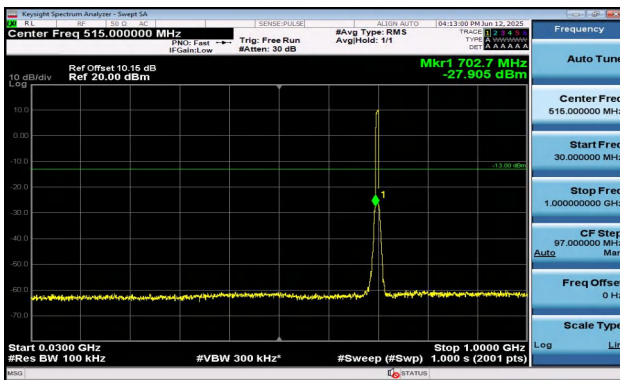
Band17-5MHz-QPSK-23755-25RB#0-30~1000-PASS
