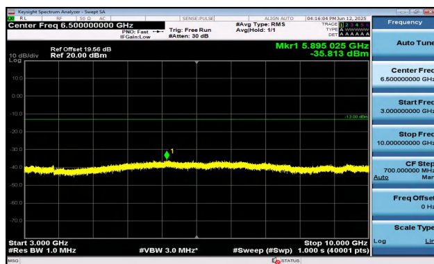
Band17-5MHz-16QAM-23790-1RB#0-3000~10000-PASS
