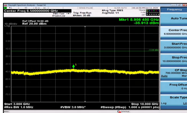
Band17-5MHz-16QAM-23755-1RB#0-3000~10000-PASS
