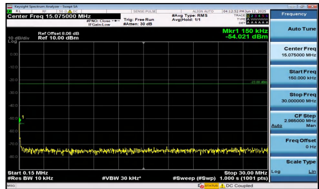
Band17-5MHz-QPSK-23755-25RB#0-0.15~30-PASS
