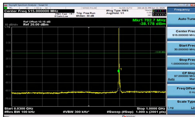
Band17-5MHz-16QAM-23755-1RB#0-30~1000-PASS
