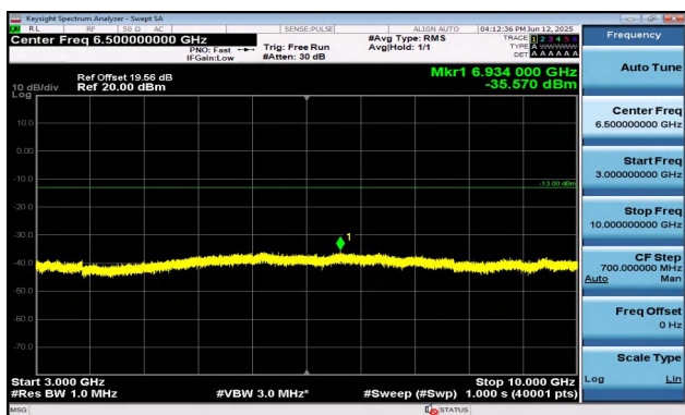
Band17-5MHz-16QAM-23755-1RB#24-3000~10000-PASS
