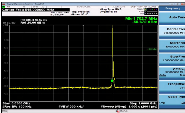
Band17-5MHz-QPSK-23790-1RB#0-30~1000-PASS
