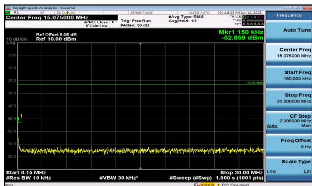
Band17-5MHz-16QAM-23755-1RB#0-0.15~30-PASS
