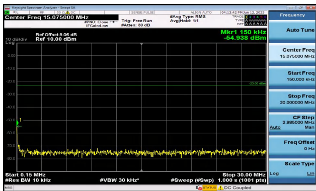
Band17-5MHz-16QAM-23755-25RB#0-0.15~30-PASS
