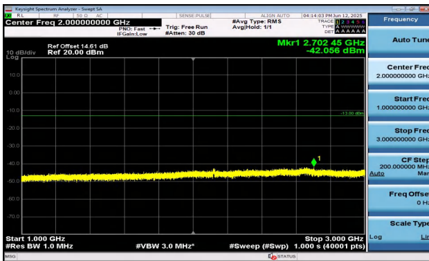
Band17-5MHz-16QAM-23755-25RB#0-1000~3000-PASS
