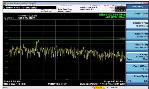
Band17-5MHz-16QAM-23755-1RB#0-0.009~0.15-PASS
