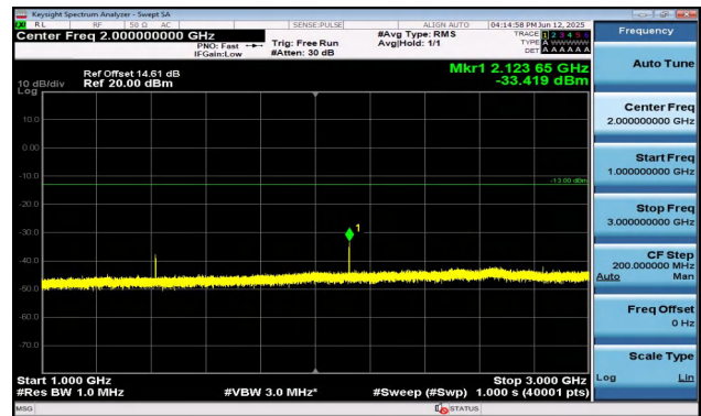
Band17-5MHz-QPSK-23790-1RB#0-1000~3000-PASS
