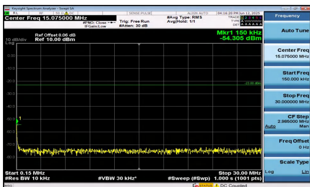
Band17-5MHz-QPSK-23790-1RB#24-0.15~30-PASS
