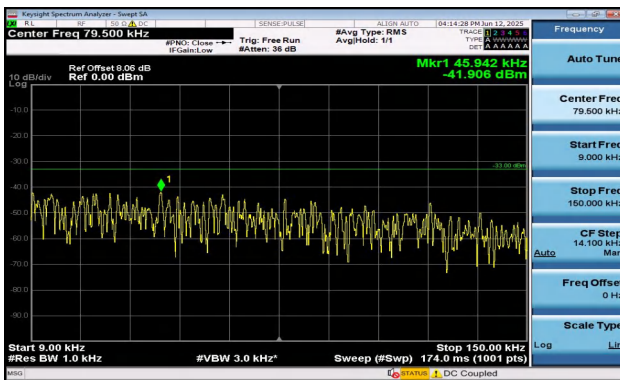
Band17-5MHz-QPSK-23790-1RB#0-0.009~0.15-PASS
