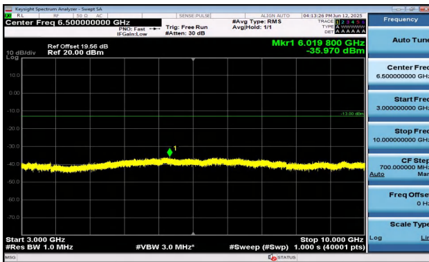
Band17-5MHz-QPSK-23755-25RB#0-3000~10000-PASS
