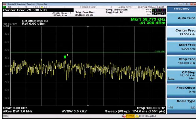
Band17-5MHz-16QAM-23790-1RB#24-0.009~0.15-PASS
