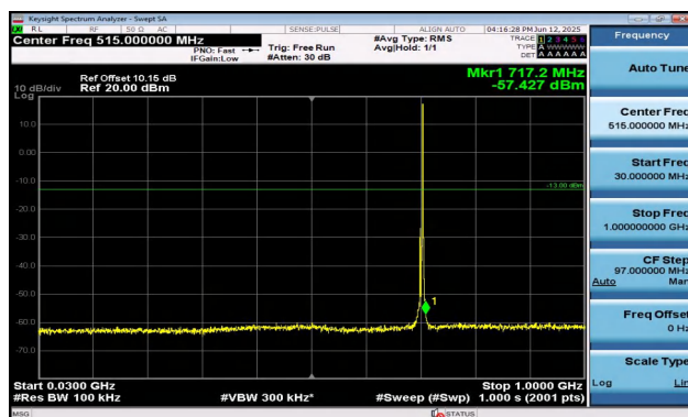
Band17-5MHz-QPSK-23790-1RB#24-30~1000-PASS
