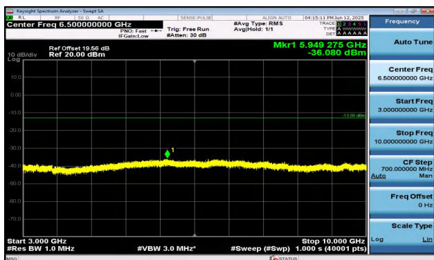
Band17-5MHz-QPSK-23790-1RB#0-3000~10000-PASS
