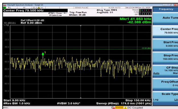
Band17-5MHz-16QAM-23755-25RB#0-0.009~0.15-PASS
