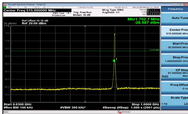
Band17-5MHz-16QAM-23755-25RB#0-30~1000-PASS
