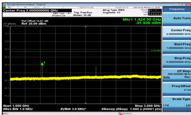
Band17-5MHz-QPSK-23790-1RB#24-1000~3000-PASS
