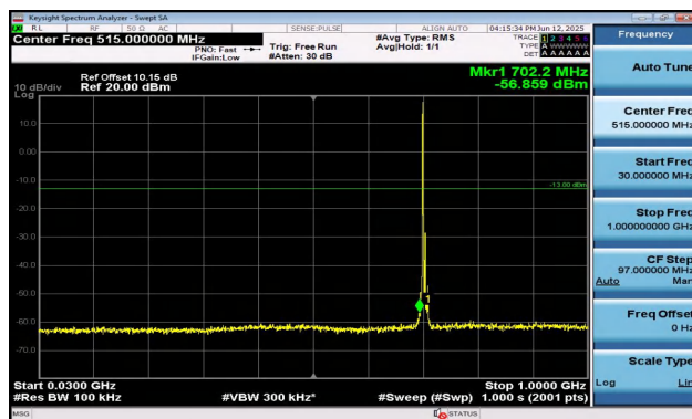
Band17-5MHz-16QAM-23790-1RB#0-30~1000-PASS
