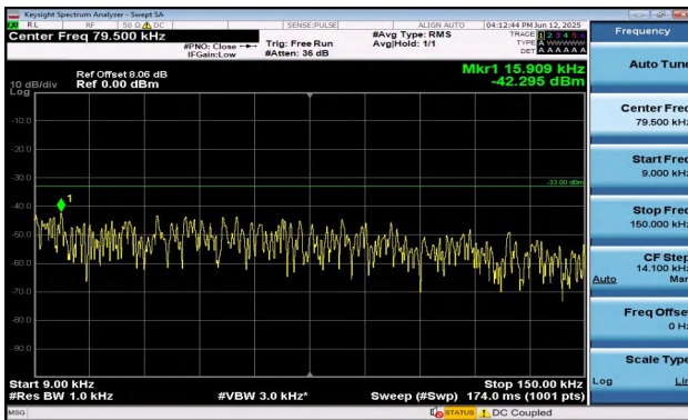
Band17-5MHz-QPSK-23755-25RB#0-0.009~0.15-PASS
