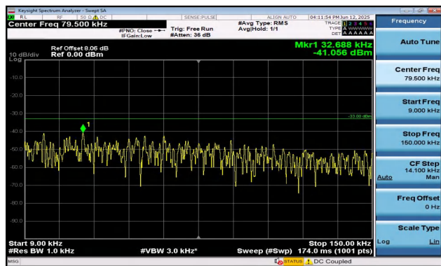
Band17-5MHz-16QAM-23755-1RB#24-0.009~0.15-PASS
