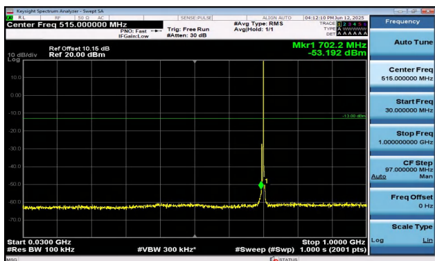
Band17-5MHz-16QAM-23755-1RB#24-30~1000-PASS
