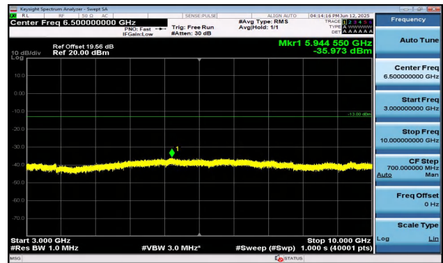
Band17-5MHz-16QAM-23755-25RB#0-3000~10000-PASS
