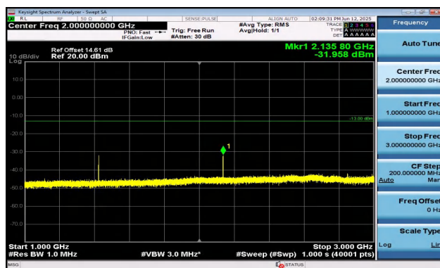
Band12-10MHz-QPSK-23095-1RB#49-1000~3000-PASS
