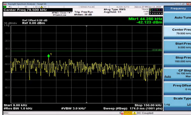
Band12-10MHz-16QAM-23130-1RB#0-0.009~0.15-PASS
