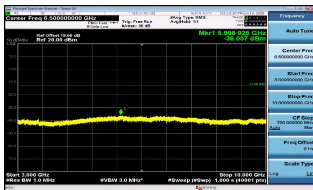
Band12-10MHz-16QAM-23130-1RB#0-3000~10000-PASS
