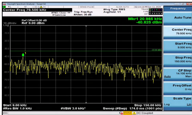
Band12-10MHz-QPSK-23060-50RB#0-0.009~0.15-PASS
