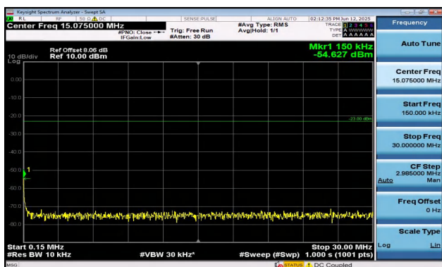
Band12-10MHz-QPSK-23130-1RB#49-0.15~30-PASS
