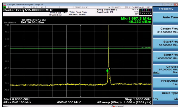
Band12-10MHz-16QAM-23130-1RB#0-30~1000-PASS
