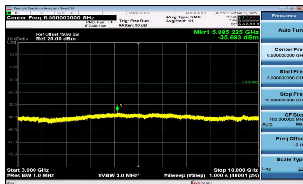
Band12-10MHz-QPSK-23095-50RB#0-3000~10000-PASS
