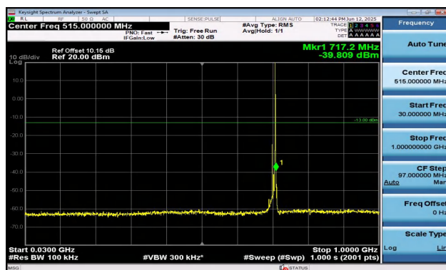
Band12-10MHz-QPSK-23130-1RB#49-30~1000-PASS
