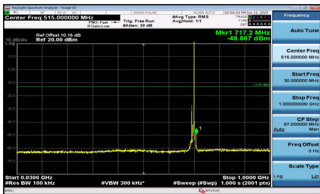
Band12-10MHz-16QAM-23060-1RB#49-30~1000-PASS
