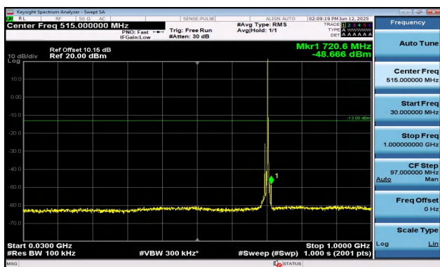
Band12-10MHz-QPSK-23095-1RB#49-30~1000-PASS
