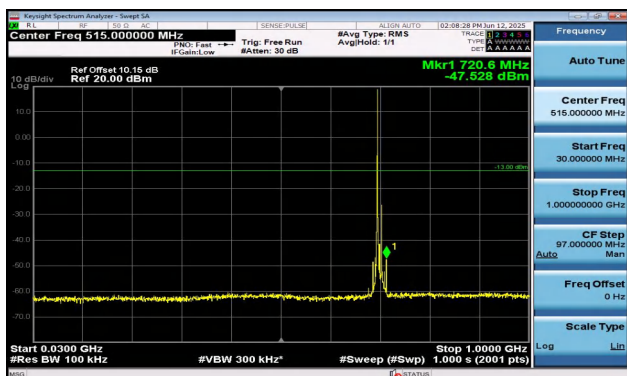
Band12-10MHz-16QAM-23095-1RB#0-30~1000-PASS
