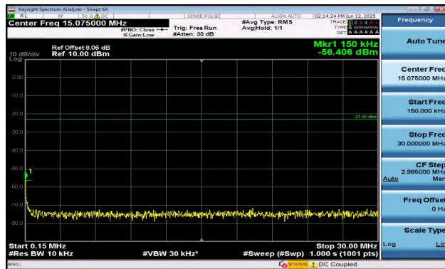
Band12-10MHz-QPSK-23060-50RB#0-0.15~30-PASS
