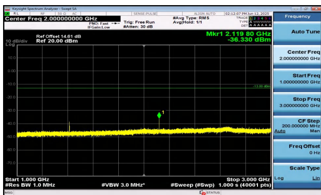
Band12-10MHz-16QAM-23130-1RB#0-1000~3000-PASS
