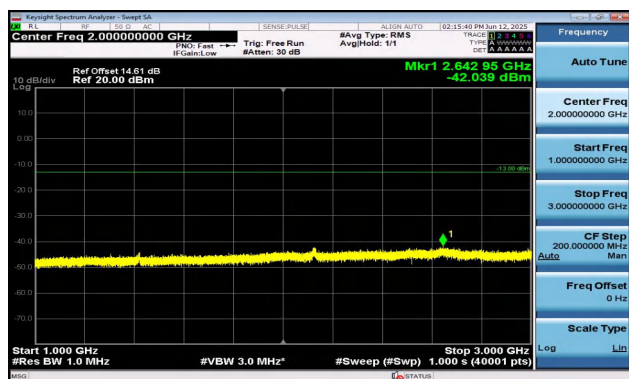
Band12-10MHz-QPSK-23095-50RB#0-1000~3000-PASS
