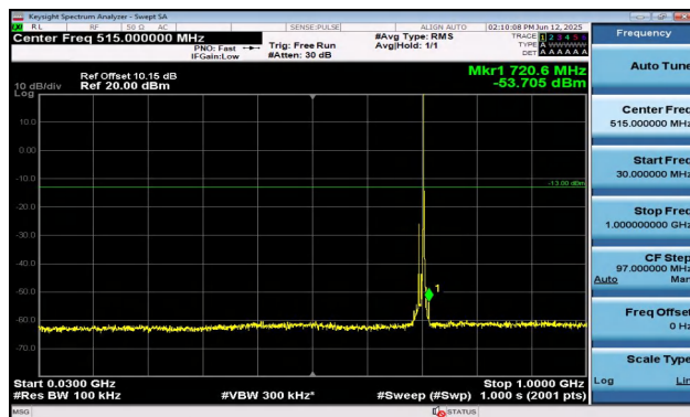
Band12-10MHz-16QAM-23095-1RB#49-30~1000-PASS
