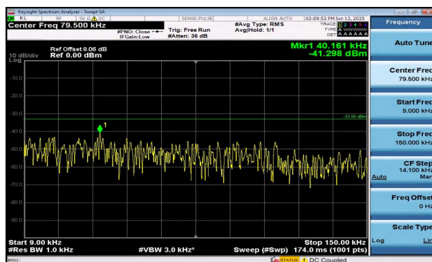
Band12-10MHz-16QAM-23095-1RB#49-0.009~0.15-PASS
