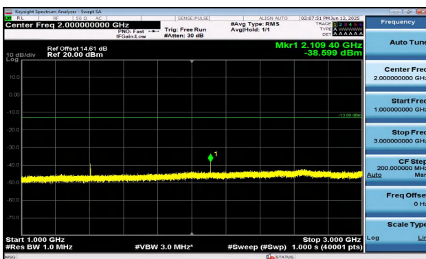
Band12-10MHz-QPSK-23095-1RB#0-1000~3000-PASS
