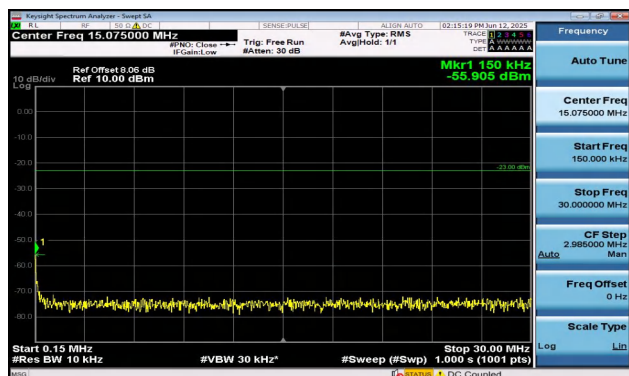
Band12-10MHz-QPSK-23095-50RB#0-0.15~30-PASS
