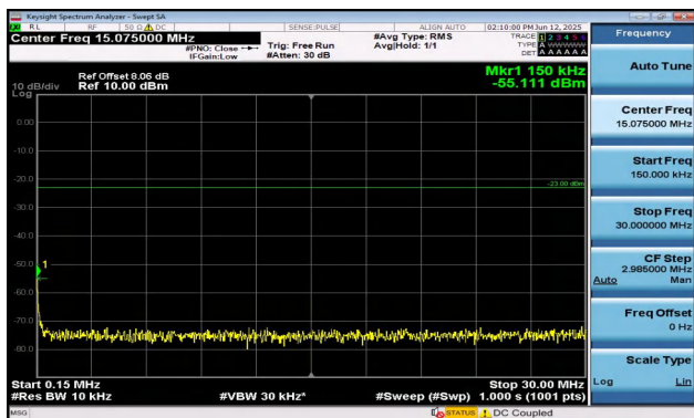
Band12-10MHz-16QAM-23095-1RB#49-0.15~30-PASS
