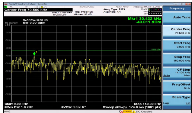
Band12-10MHz-QPSK-23095-1RB#0-0.009~0.15-PASS
