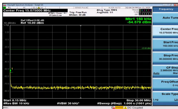
Band12-10MHz-16QAM-23060-1RB#49-0.15~30-PASS
