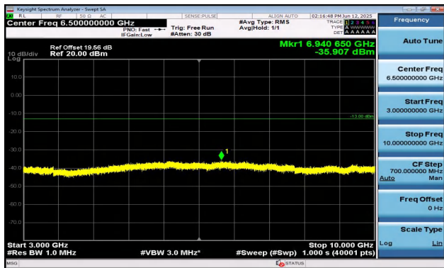
Band12-10MHz-QPSK-23130-50RB#0-3000~10000-PASS
