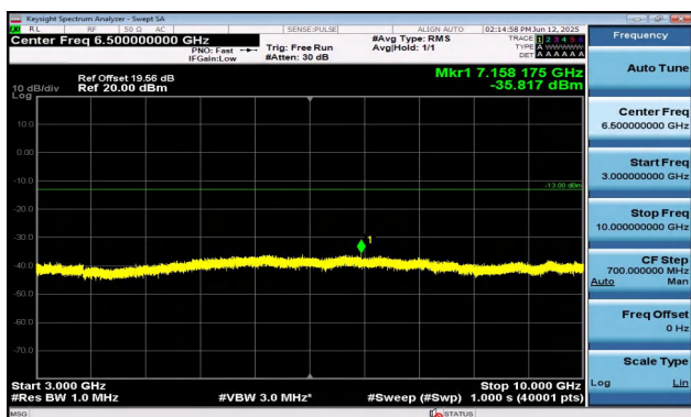
Band12-10MHz-QPSK-23060-50RB#0-3000~10000-PASS
