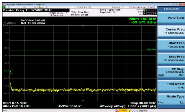
Band12-10MHz-16QAM-23060-1RB#0-0.15~30-PASS
