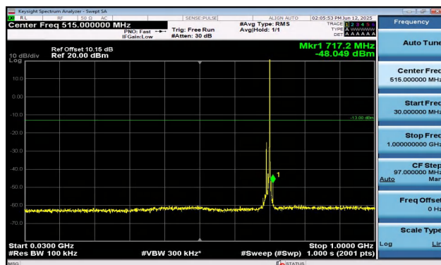
Band12-10MHz-QPSK-23060-1RB#49-30~1000-PASS
