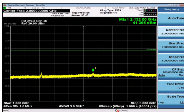
Band12-10MHz-QPSK-23130-50RB#0-1000~3000-PASS
