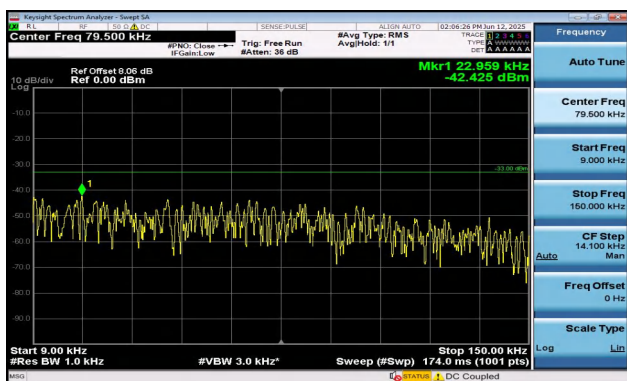
Band12-10MHz-16QAM-23060-1RB#49-0.009~0.15-PASS
