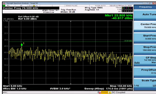
Band12-10MHz-QPSK-23095-50RB#0-0.009~0.15-PASS
