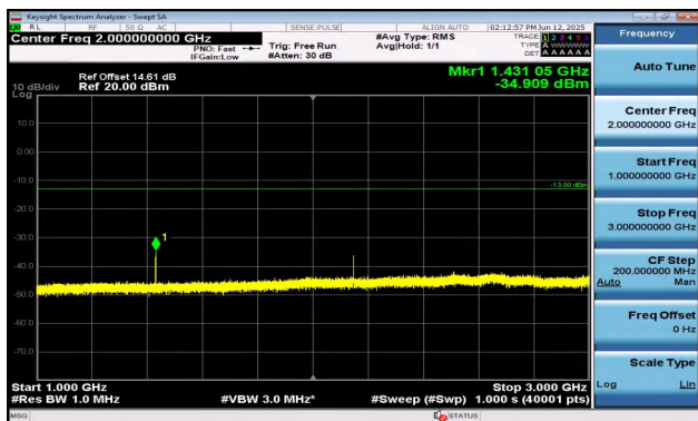
Band12-10MHz-QPSK-23130-1RB#49-1000~3000-PASS
