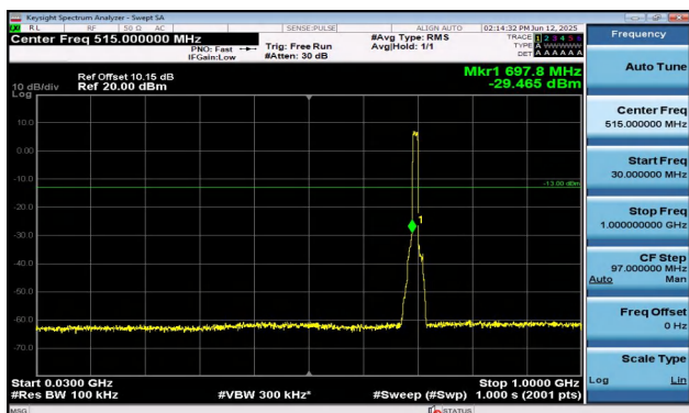
Band12-10MHz-QPSK-23060-50RB#0-30~1000-PASS
