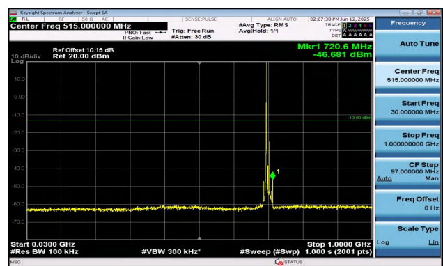
Band12-10MHz-QPSK-23095-1RB#0-30~1000-PASS
