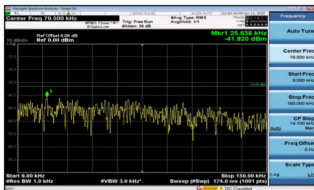
Band12-10MHz-16QAM-23060-1RB#0-0.009~0.15-PASS
