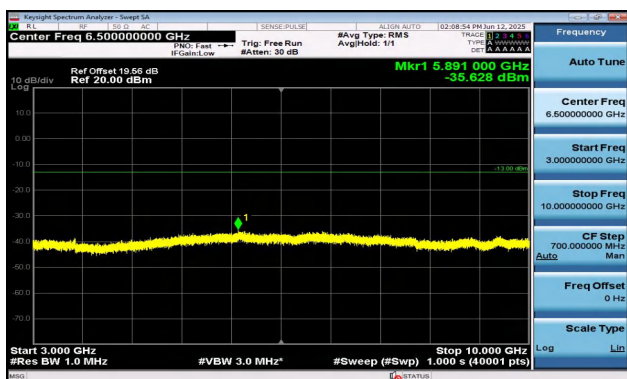
Band12-10MHz-16QAM-23095-1RB#0-3000~10000-PASS
