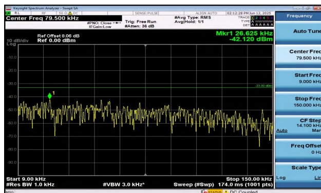
Band12-10MHz-QPSK-23130-1RB#49-0.009~0.15-PASS
