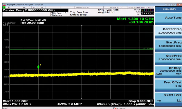
Band12-10MHz-16QAM-23060-1RB#0-1000~3000-PASS
