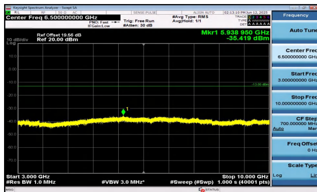
Band12-10MHz-QPSK-23130-1RB#49-3000~10000-PASS
