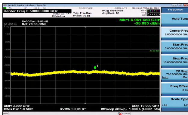
Band12-10MHz-QPSK-23060-1RB#49-3000~10000-PASS
