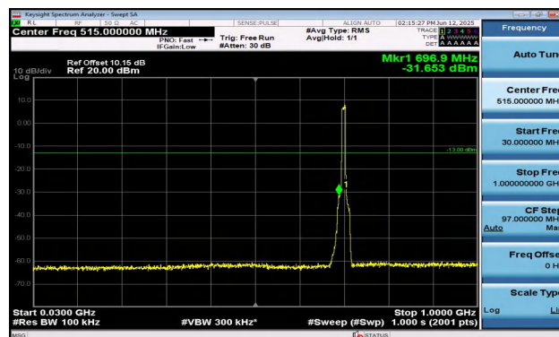
Band12-10MHz-QPSK-23095-50RB#0-30~1000-PASS
