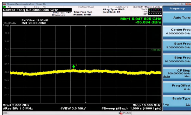
Band12-10MHz-QPSK-23095-1RB#49-3000~10000-PASS
