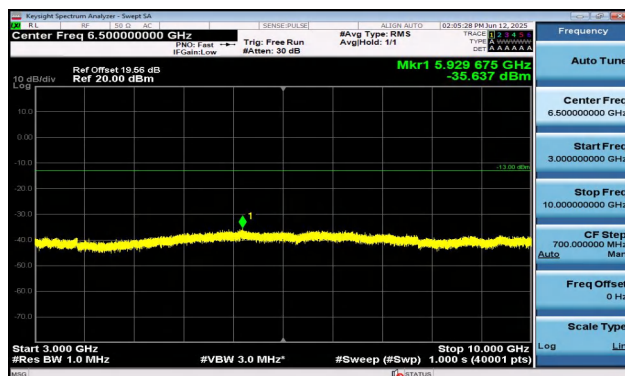
Band12-10MHz-16QAM-23060-1RB#0-3000~10000-PASS
