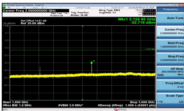
Band12-10MHz-QPSK-23060-1RB#49-1000~3000-PASS
