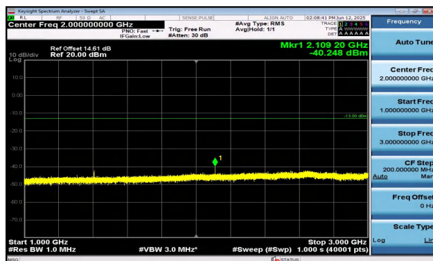
Band12-10MHz-16QAM-23095-1RB#0-1000~3000-PASS
