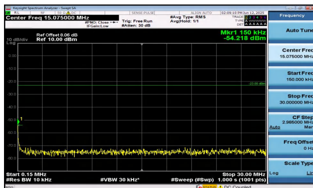
Band12-10MHz-QPSK-23095-1RB#49-0.15~30-PASS
