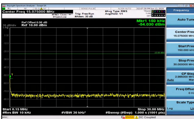
Band12-10MHz-QPSK-23095-1RB#0-0.15~30-PASS
