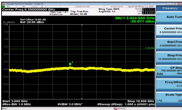
Band12-10MHz-16QAM-23060-1RB#49-3000~10000-PAS S
