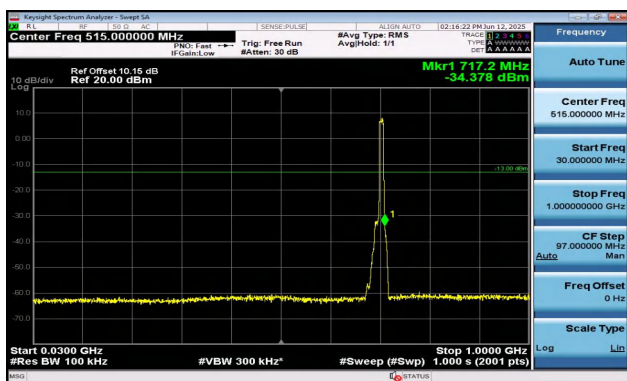
Band12-10MHz-QPSK-23130-50RB#0-30~1000-PASS
