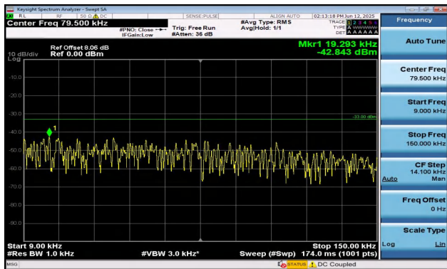
Band12-10MHz-16QAM-23130-1RB#49-0.009~0.15-PASS
