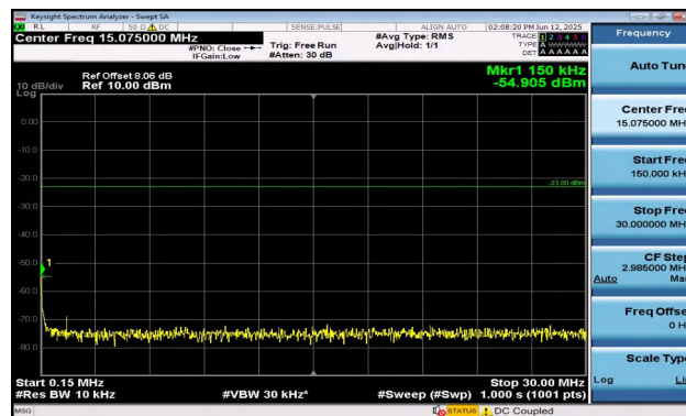
Band12-10MHz-16QAM-23095-1RB#0-0.15~30-PASS
