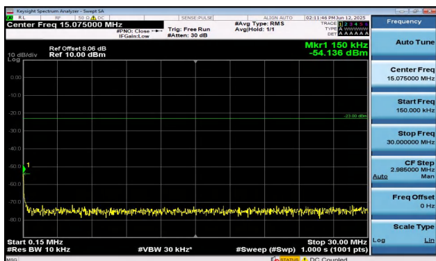
Band12-10MHz-16QAM-23130-1RB#0-0.15~30-PASS
