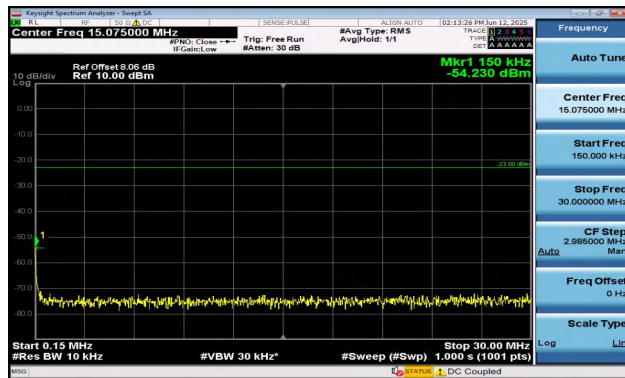
Band12-10MHz-16QAM-23130-1RB#49-0.15~30-PASS
