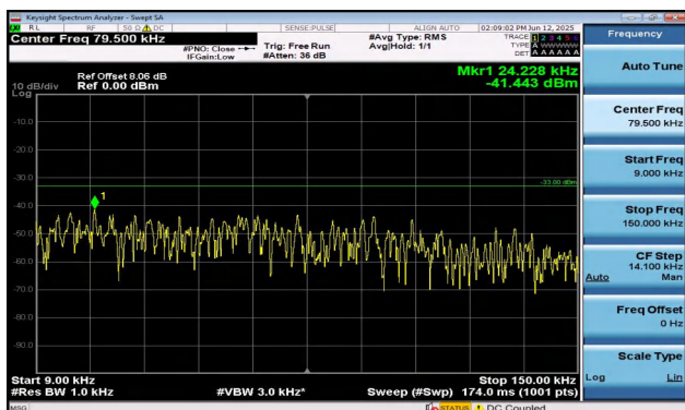
Band12-10MHz-QPSK-23095-1RB#49-0.009~0.15-PASS
