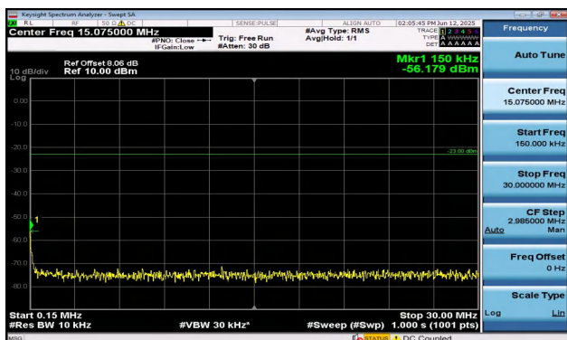
Band12-10MHz-QPSK-23060-1RB#49-0.15~30-PASS
