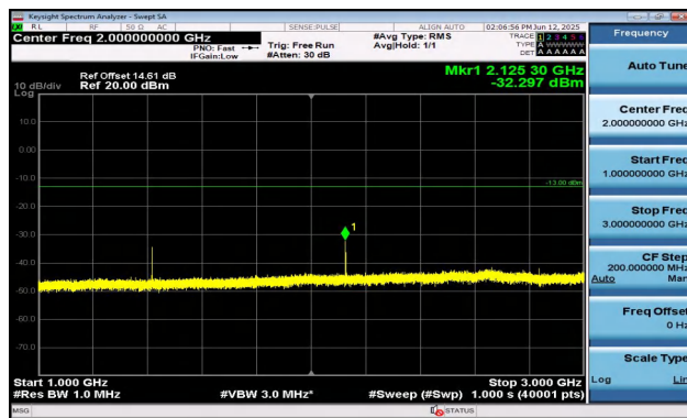
Band12-10MHz-16QAM-23060-1RB#49-1000~3000-PASS
