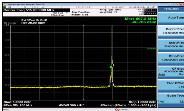
Band12-10MHz-16QAM-23060-1RB#0-30~1000-PASS
