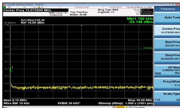
Band12-10MHz-QPSK-23130-50RB#0-0.15~30-PASS
