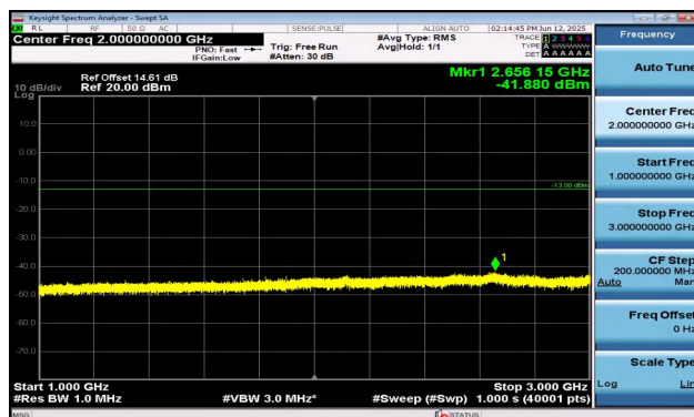
Band12-10MHz-QPSK-23060-50RB#0-1000~3000-PASS
