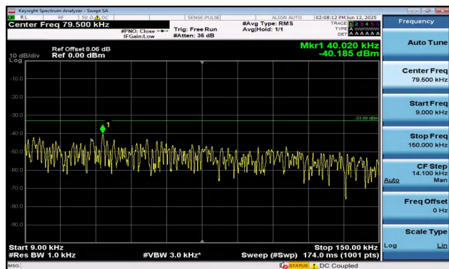
Band12-10MHz-16QAM-23095-1RB#0-0.009~0.15-PASS
