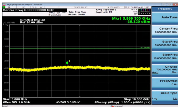
Band12-10MHz-QPSK-23130-1RB#0-3000~10000-PASS
