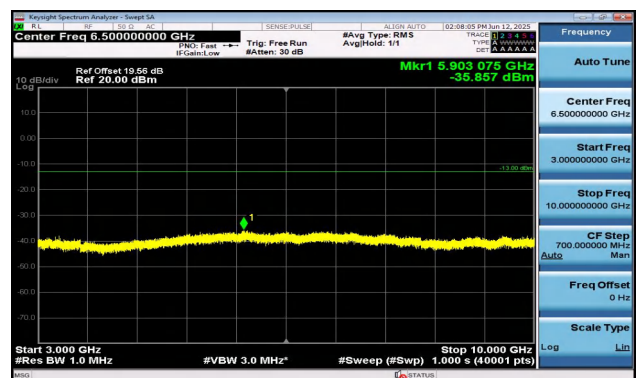
Band12-10MHz-QPSK-23095-1RB#0-3000~10000-PASS
