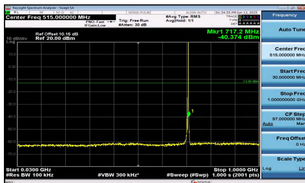
Band12-5MHz-QPSK-23155-1RB#24-30~1000-PASS
