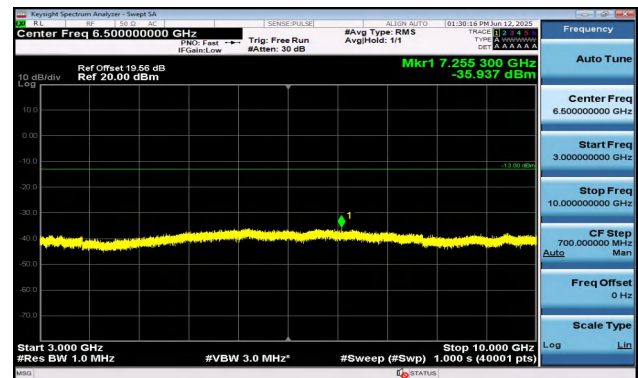
Band12-5MHz-QPSK-23095-1RB#24-3000~10000-PASS
