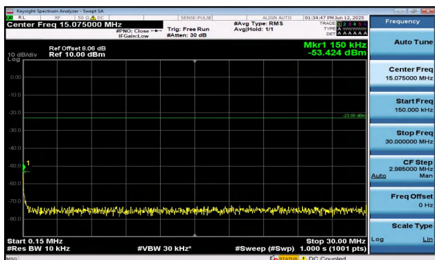
Band12-5MHz-QPSK-23155-1RB#24-0.15~30-PASS
