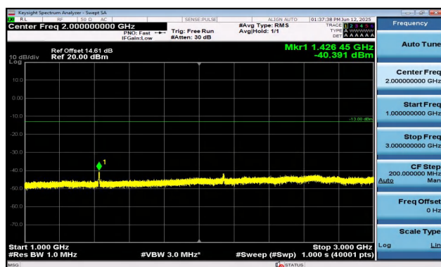
Band12-5MHz-16QAM-23155-25RB#0-1000~3000-PASS
