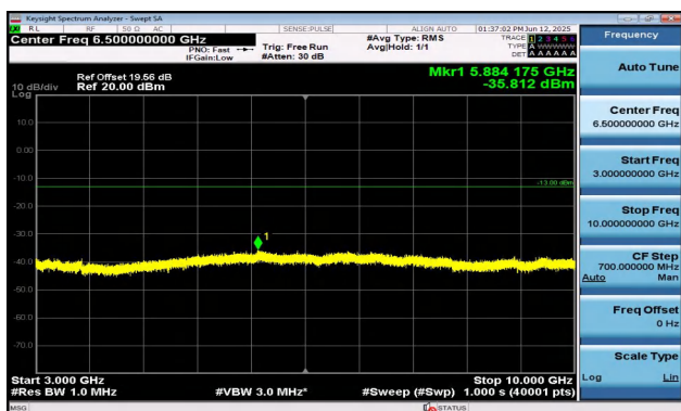
Band12-5MHz-QPSK-23155-25RB#0-3000~10000-PASS
