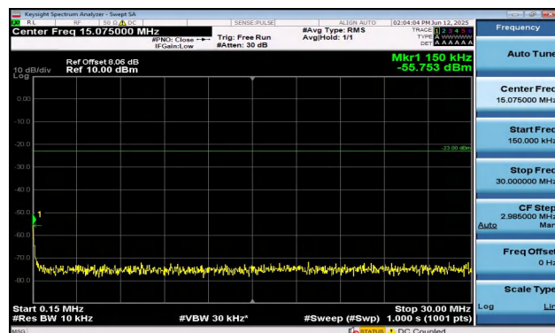
Band12-10MHz-QPSK-23060-1RB#0-0.15~30-PASS
