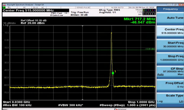
Band12-5MHz-QPSK-23095-25RB#0-30~1000-PASS
