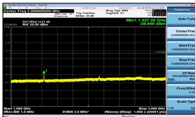
Band12-5MHz-QPSK-23155-25RB#0-1000~3000-PASS
