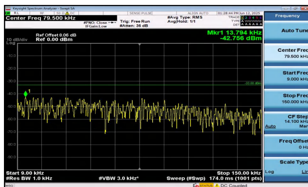
Band12-5MHz-16QAM-23095-1RB#0-0.009~0.15-PASS
