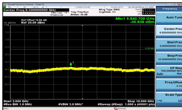
Band12-5MHz-16QAM-23095-25RB#0-3000~10000-PASS
