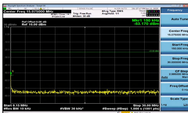
Band12-5MHz-16QAM-23155-25RB#0-0.15~30-PASS
