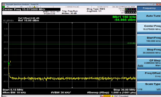
Band12-5MHz-16QAM-23095-25RB#0-0.15~30-PASS
