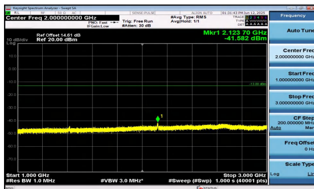
Band12-5MHz-QPSK-23095-25RB#0-1000~3000-PASS
