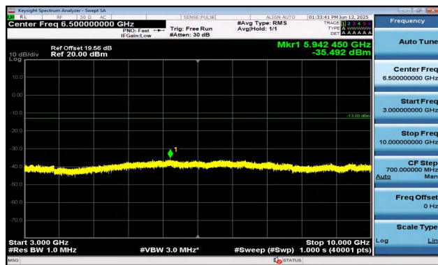
Band12-5MHz-QPSK-23155-1RB#0-3000~10000-PASS
