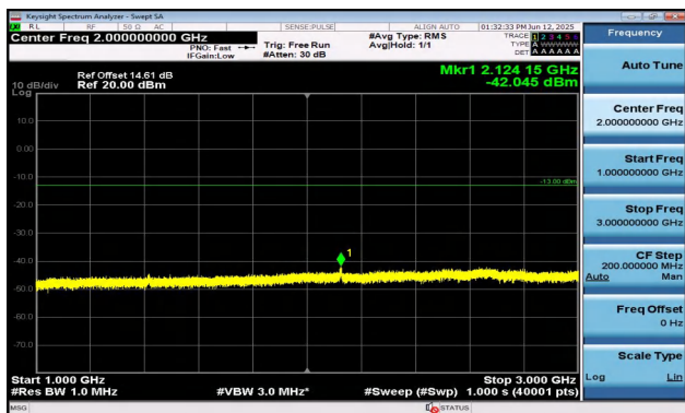
Band12-5MHz-16QAM-23095-25RB#0-1000~3000-PASS
