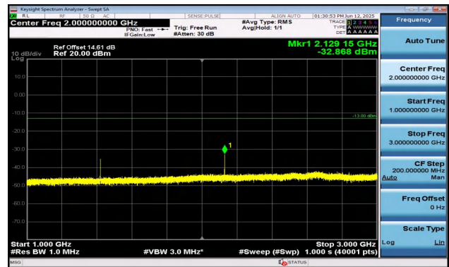
Band12-5MHz-16QAM-23095-1RB#24-1000~3000-PASS
