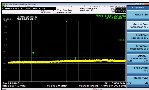
Band12-5MHz-QPSK-23155-1RB#24-1000~3000-PASS
