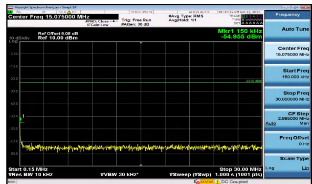
Band12-5MHz-QPSK-23095-25RB#0-0.15~30-PASS
