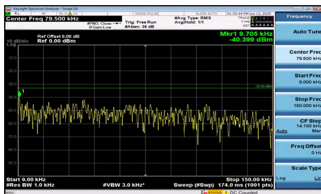
Band12-5MHz-16QAM-23155-1RB#0-0.009~0.15-PASS
