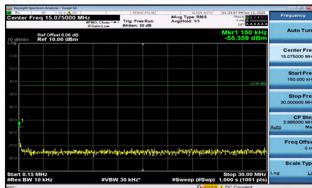
Band12-5MHz-QPSK-23155-1RB#0-0.15~30-PASS
