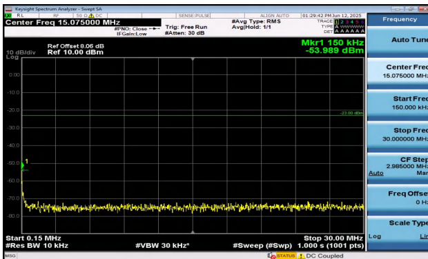
Band12-5MHz-QPSK-23095-1RB#24-0.15~30-PASS
