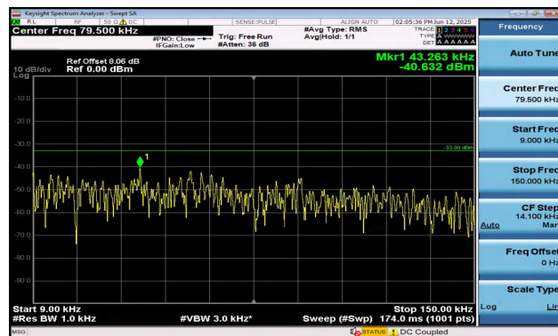
Band12-10MHz-QPSK-23060-1RB#49-0.009~0.15-PASS
