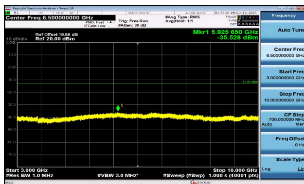
Band12-5MHz-QPSK-23155-1RB#24-3000~10000-PASS
