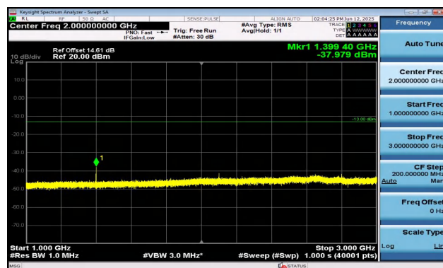
Band12-10MHz-QPSK-23060-1RB#0-1000~3000-PASS
