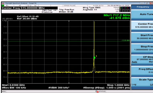
Band12-5MHz-16QAM-23155-1RB#24-30~1000-PASS
