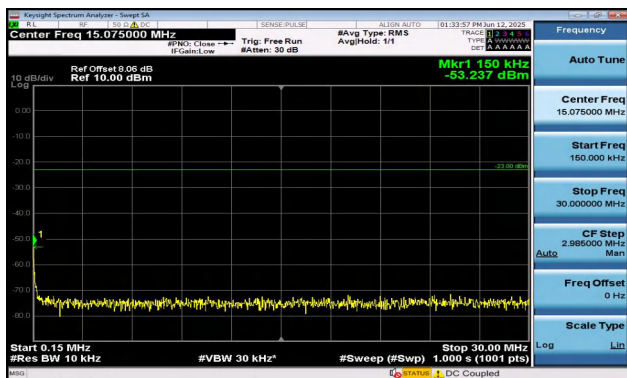
Band12-5MHz-16QAM-23155-1RB#0-0.15~30-PASS
