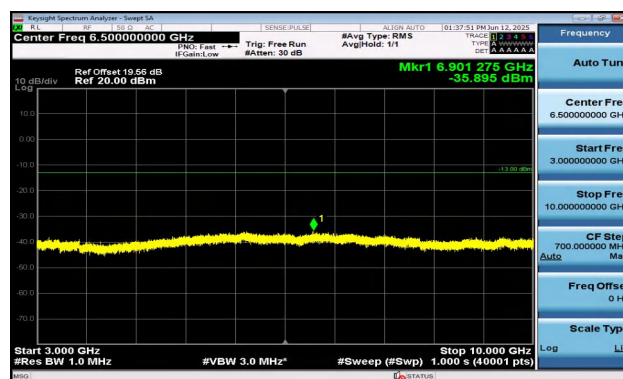
Band12-5MHz-16QAM-23155-25RB#0-3000~10000-PASS
