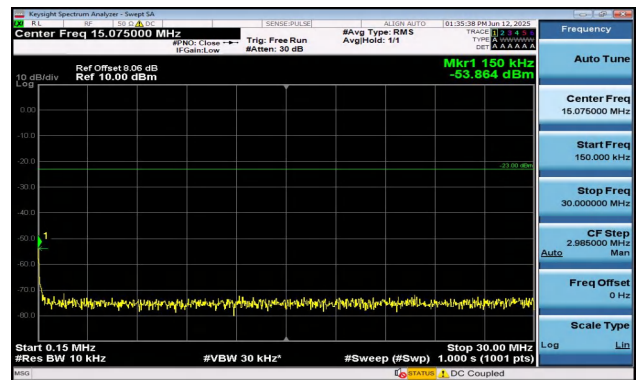
Band12-5MHz-16QAM-23155-1RB#24-0.15~30-PASS
