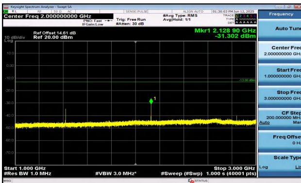
Band12-5MHz-QPSK-23095-1RB#24-1000~3000-PASS
