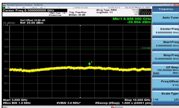
Band12-5MHz-QPSK-23095-25RB#0-3000~10000-PASS
