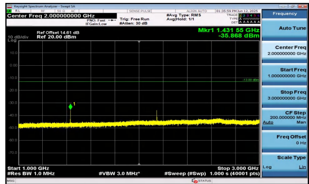
Band12-5MHz-16QAM-23155-1RB#24-1000~3000-PASS
