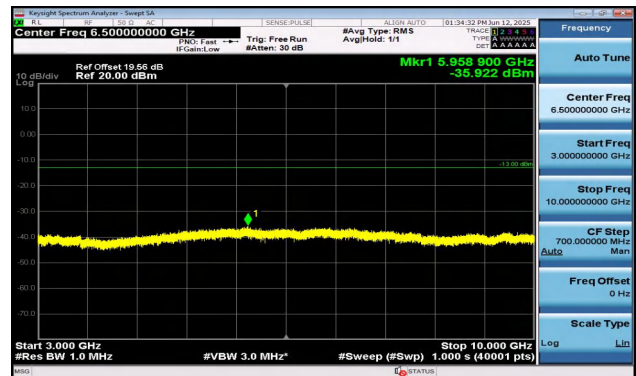
Band12-5MHz-16QAM-23155-1RB#0-3000~10000-PASS
