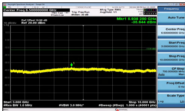
Band12-10MHz-QPSK-23060-1RB#0-3000~10000-PASS
