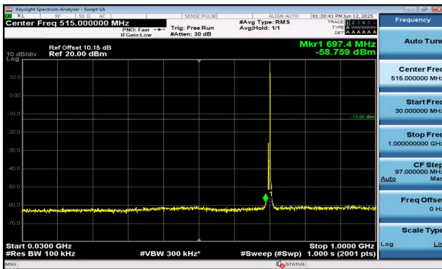
Band12-5MHz-16QAM-23095-1RB#24-30~1000-PASS
