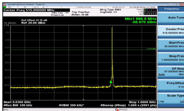
Band12-5MHz-16QAM-23095-1RB#0-30~1000-PASS
