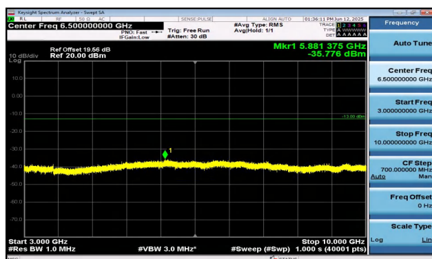
Band12-5MHz-16QAM-23155-1RB#24-3000~10000-PASS
