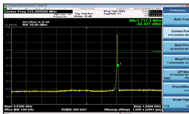
Band12-5MHz-16QAM-23155-25RB#0-30~1000-PASS
