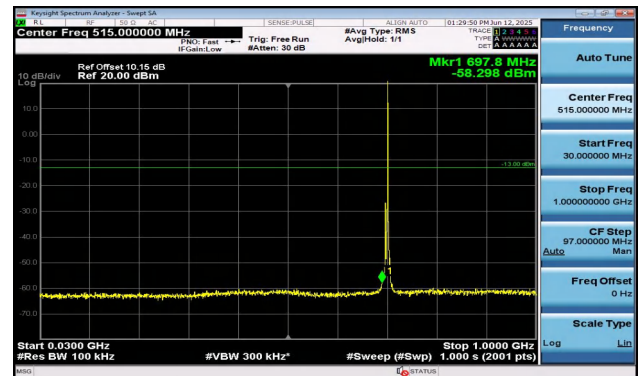
Band12-5MHz-QPSK-23095-1RB#24-30~1000-PASS
