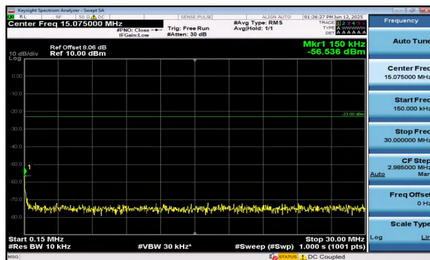
Band12-5MHz-QPSK-23155-25RB#0-0.15~30-PASS
