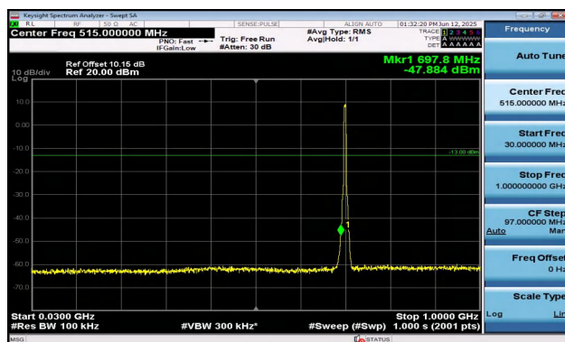
Band12-5MHz-16QAM-23095-25RB#0-30~1000-PASS
