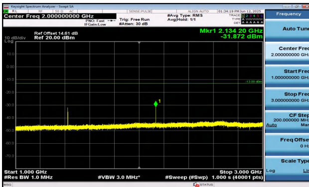
Band12-5MHz-16QAM-23155-1RB#0-1000~3000-PASS
