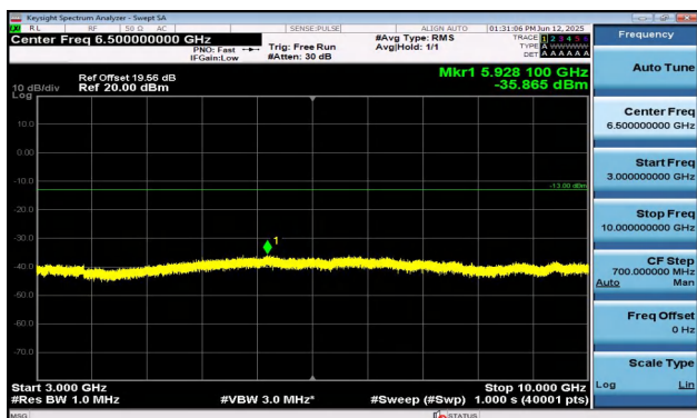
Band12-5MHz-16QAM-23095-1RB#24-3000~10000-PASS
