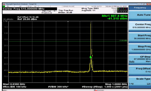
Band12-10MHz-QPSK-23060-1RB#0-30~1000-PASS
