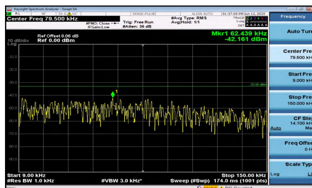
Band12-5MHz-16QAM-23155-25RB#0-0.009~0.15-PASS
