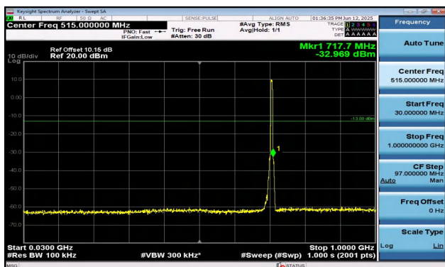
Band12-5MHz-QPSK-23155-25RB#0-30~1000-PASS
