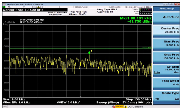
Band12-5MHz-QPSK-23155-25RB#0-0.009~0.15-PASS
