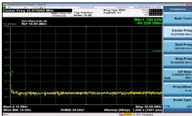
Band12-5MHz-16QAM-23095-1RB#0-0.15~30-PASS
