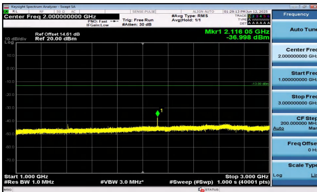
Band12-5MHz-16QAM-23095-1RB#0-1000~3000-PASS
