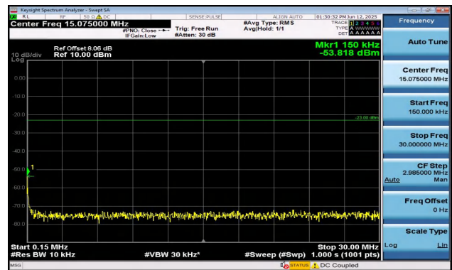
Band12-5MHz-16QAM-23095-1RB#24-0.15~30-PASS
