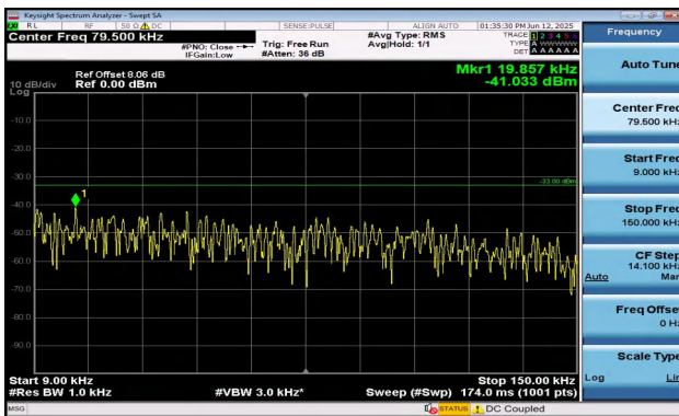
Band12-5MHz-16QAM-23155-1RB#24-0.009~0.15-PASS
