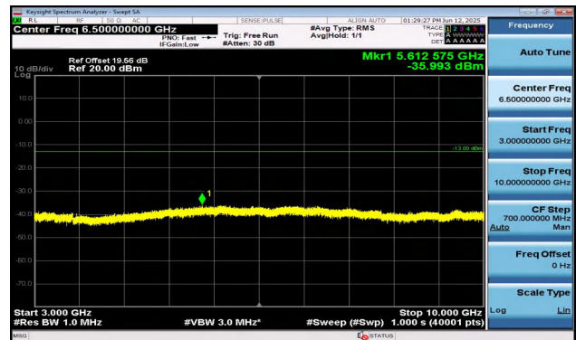
Band12-5MHz-16QAM-23095-1RB#0-3000~10000-PASS
