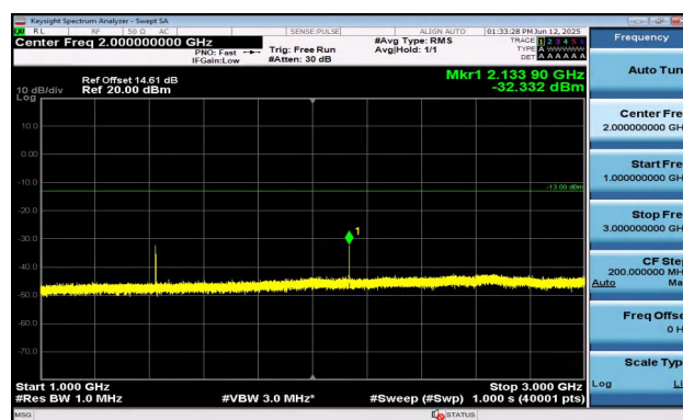
Band12-5MHz-QPSK-23155-1RB#0-1000~3000-PASS
