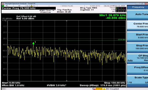
Band12-5MHz-QPSK-23095-25RB#0-0.009~0.15-PASS
