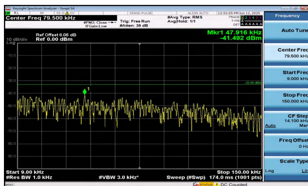
Band12-3MHz-16QAM-23165-1RB#0-0.009~0.15-PASS
