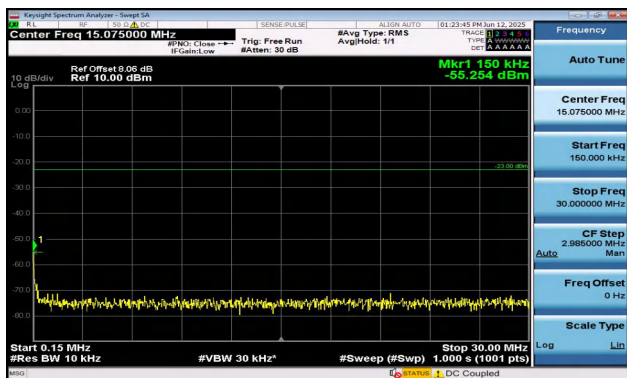
Band12-5MHz-16QAM-23035-1RB#0-0.15~30-PASS
