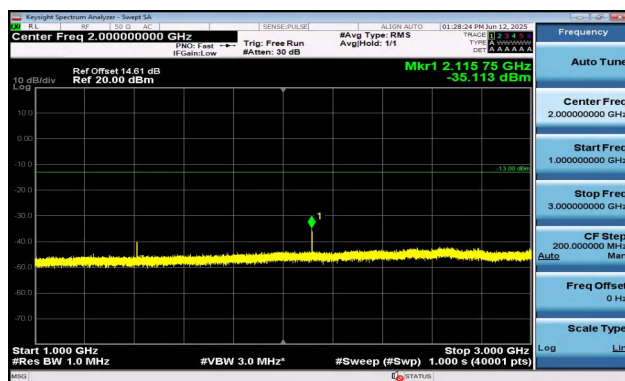
Band12-5MHz-QPSK-23095-1RB#0-1000~3000-PASS
