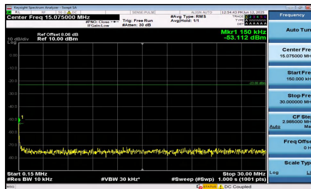
Band12-3MHz-QPSK-23165-15RB#0-0.15~30-PASS
