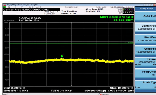
Band12-3MHz-QPSK-23165-1RB#14-3000~10000-PASS
