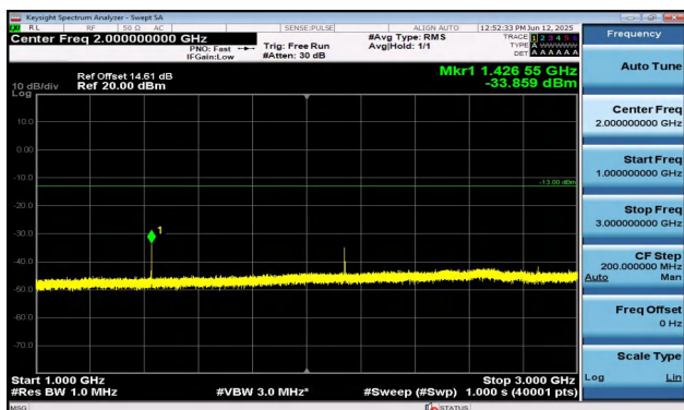
Band12-3MHz-16QAM-23165-1RB#0-1000~3000-PASS
