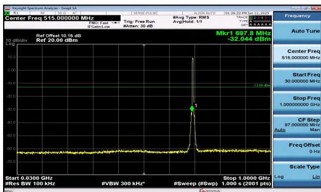
Band12-5MHz-QPSK-23035-25RB#0-30~1000-PASS
