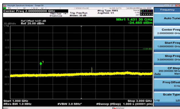
Band12-3MHz-QPSK-23165-1RB#14-1000~3000-PASS
