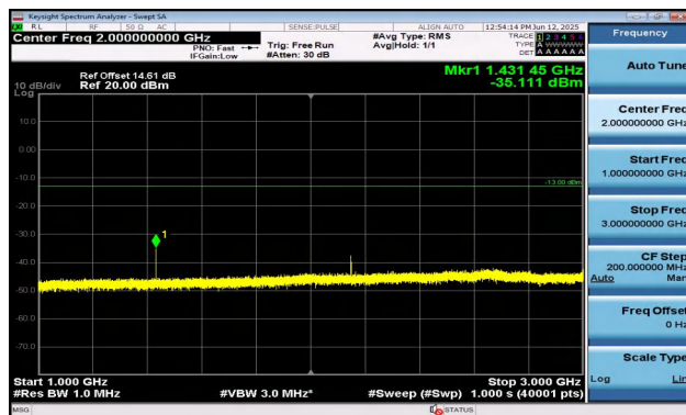
Band12-3MHz-16QAM-23165-1RB#14-1000~3000-PASS
