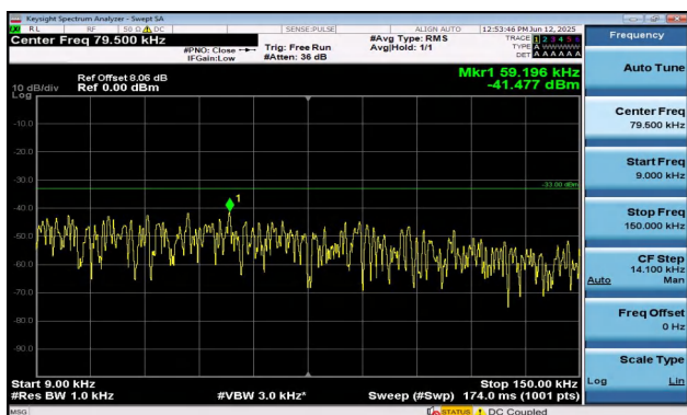
Band12-3MHz-16QAM-23165-1RB#14-0.009~0.15-PASS
