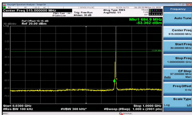
Band12-5MHz-16QAM-23035-1RB#24-30~1000-PASS
