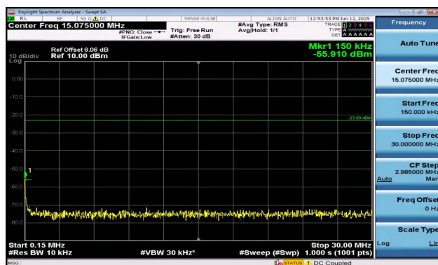
Band12-3MHz-16QAM-23165-1RB#14-0.15~30-PASS
