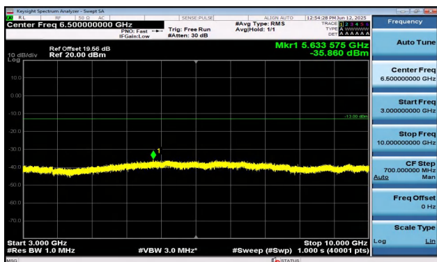
Band12-3MHz-16QAM-23165-1RB#14-3000~10000-PASS
