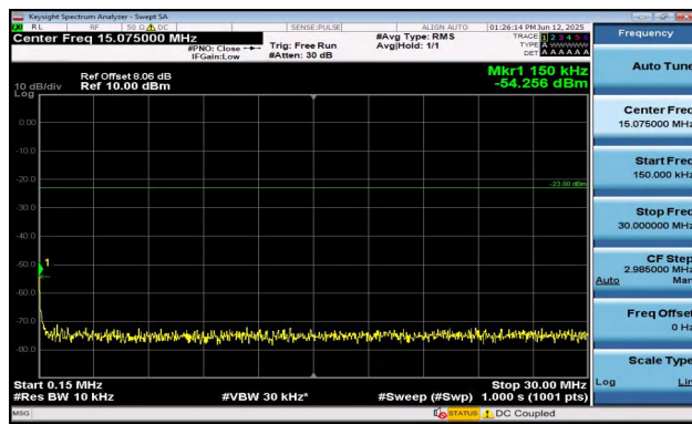
Band12-5MHz-QPSK-23035-25RB#0-0.15~30-PASS
