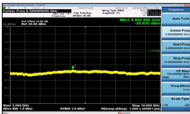
Band12-5MHz-QPSK-23035-25RB#0-3000~10000-PASS
