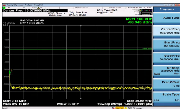
Band12-3MHz-16QAM-23165-15RB#0-0.15~30-PASS
