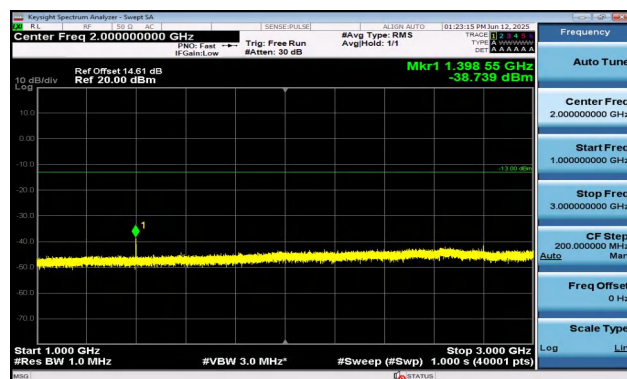
Band12-5MHz-QPSK-23035-1RB#0-1000~3000-PASS
