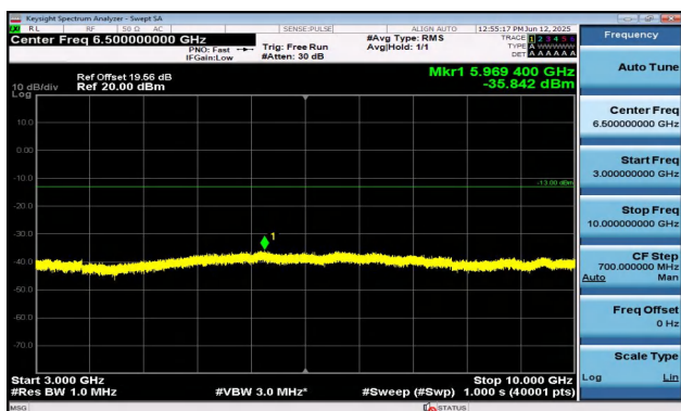
Band12-3MHz-QPSK-23165-15RB#0-3000~10000-PASS
