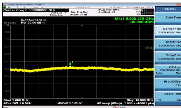
Band12-3MHz-16QAM-23165-1RB#0-3000~10000-PASS
