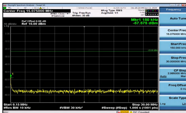
Band12-5MHz-16QAM-23035-1RB#24-0.15~30-PASS
