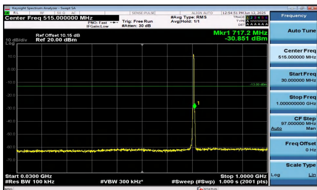
Band12-3MHz-QPSK-23165-15RB#0-30~1000-PASS
