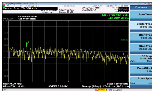
Band12-3MHz-QPSK-23165-15RB#0-0.009~0.15-PASS
