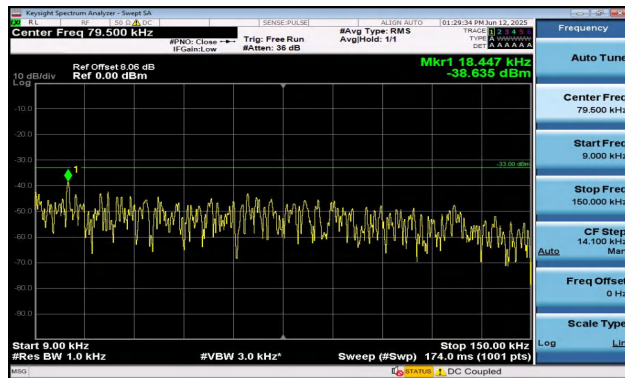
Band12-5MHz-QPSK-23095-1RB#24-0.009~0.15-PASS
