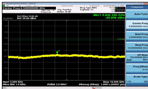
Band12-5MHz-QPSK-23035-1RB#0-3000~10000-PASS
