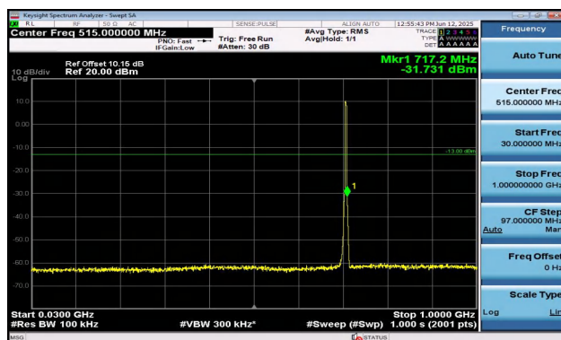
Band12-3MHz-16QAM-23165-15RB#0-30~1000-PASS
