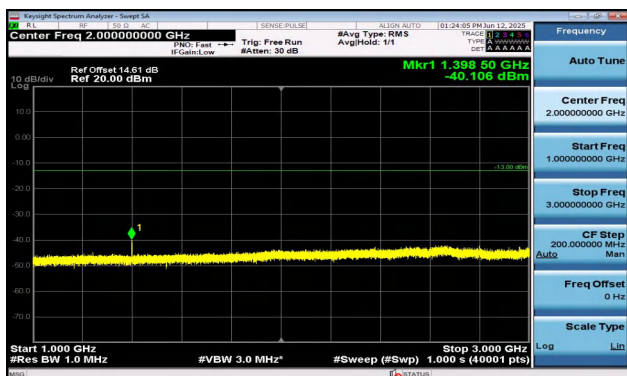
Band12-5MHz-16QAM-23035-1RB#0-1000~3000-PASS
