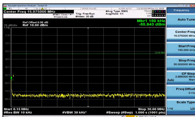
Band12-3MHz-QPSK-23165-1RB#14-0.15~30-PASS
