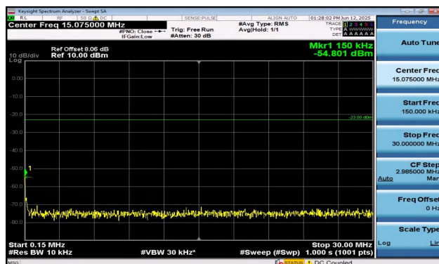
Band12-5MHz-QPSK-23095-1RB#0-0.15~30-PASS
