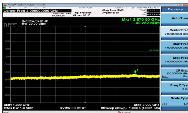
Band12-5MHz-QPSK-23035-25RB#0-1000~3000-PASS
