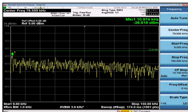
Band12-5MHz-QPSK-23035-1RB#0-0.009~0.15-PASS
