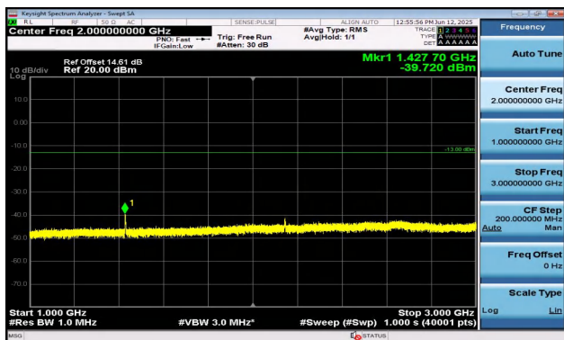
Band12-3MHz-16QAM-23165-15RB#0-1000~3000-PASS
