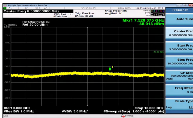
Band12-5MHz-QPSK-23035-1RB#24-3000~10000-PASS
