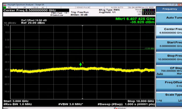
Band12-5MHz-16QAM-23035-1RB#0-3000~10000-PASS
