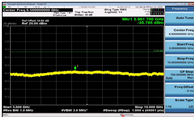
Band12-5MHz-QPSK-23095-1RB#0-3000~10000-PASS
