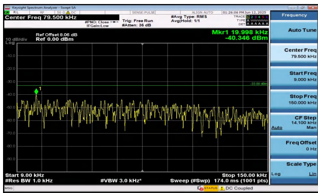
Band12-5MHz-QPSK-23035-25RB#0-0.009~0.15-PASS
