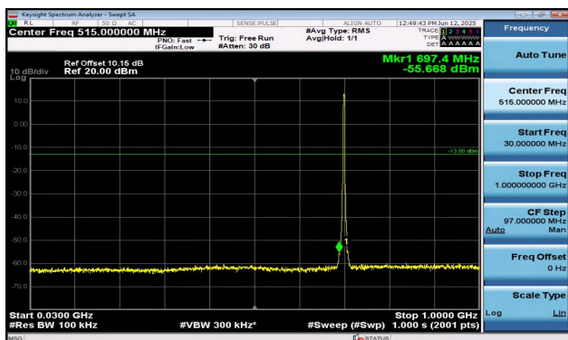
Band12-3MHz-QPSK-23095-15RB#0-30~1000-PASS
