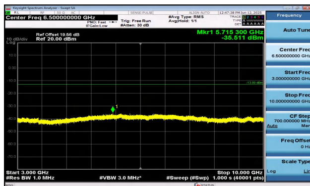
Band12-3MHz-16QAM-23095-1RB#0-3000~10000-PASS
