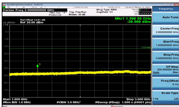
Band12-3MHz-16QAM-23025-1RB#0-1000~3000-PASS
