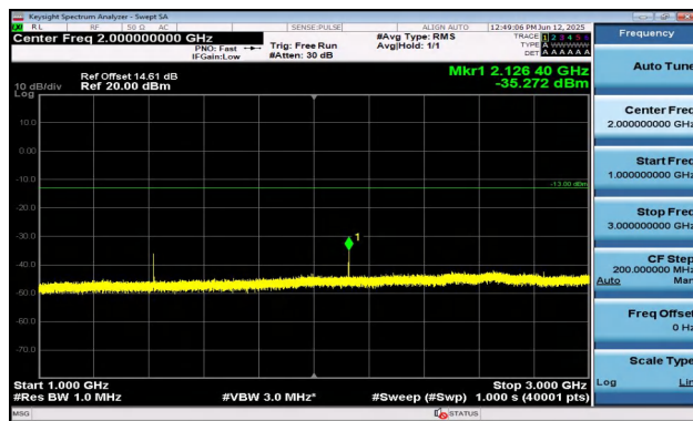
Band12-3MHz-16QAM-23095-1RB#14-1000~3000-PASS
