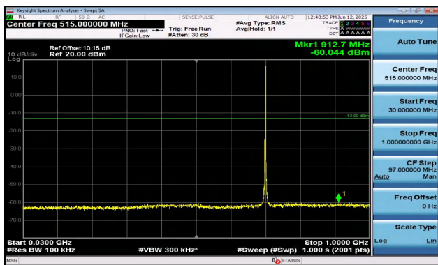
Band12-3MHz-16QAM-23095-1RB#14-30~1000-PASS
