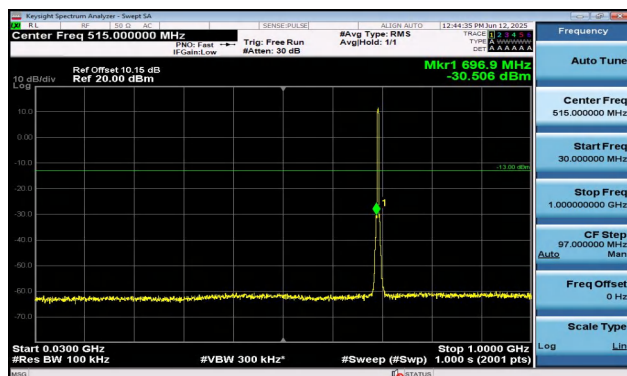
Band12-3MHz-QPSK-23025-15RB#0-30~1000-PASS
