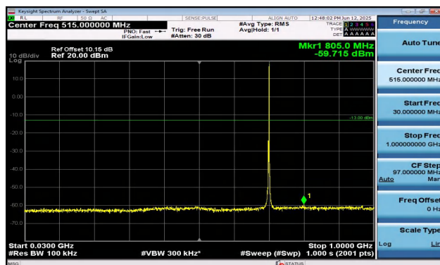
Band12-3MHz-QPSK-23095-1RB#14-30~1000-PASS
