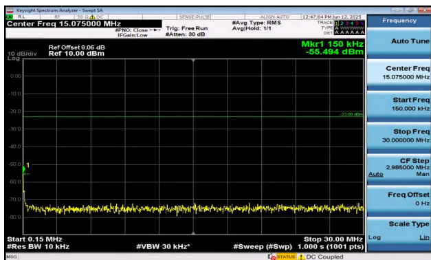
Band12-3MHz-16QAM-23095-1RB#0-0.15~30-PASS
