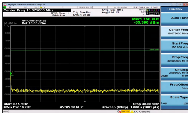
Band12-3MHz-16QAM-23025-1RB#0-0.15~30-PASS
