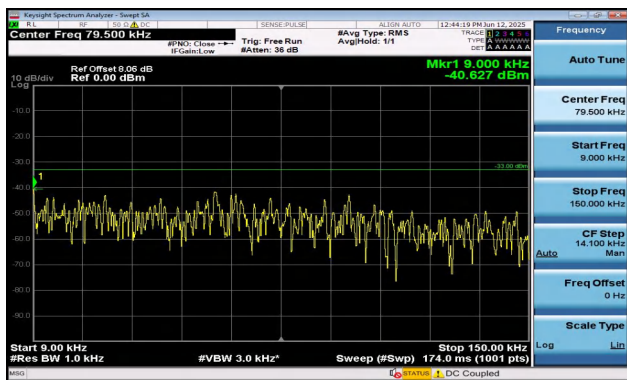
Band12-3MHz-QPSK-23025-15RB#0-0.009~0.15-PASS
