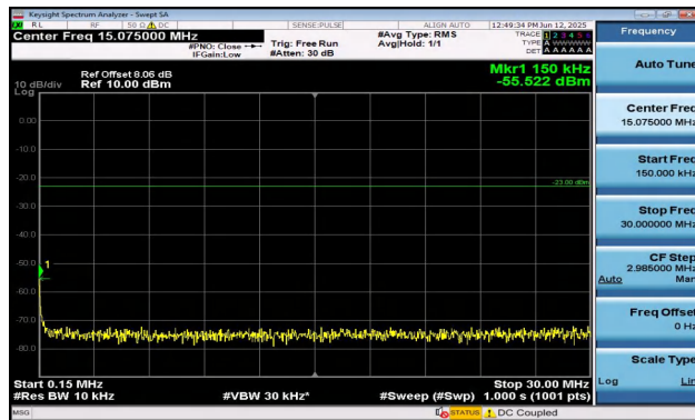
Band12-3MHz-QPSK-23095-15RB#0-0.15~30-PASS
