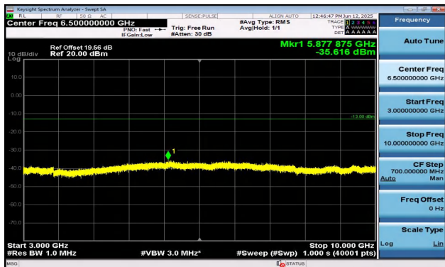
Band12-3MHz-QPSK-23095-1RB#0-3000~10000-PASS
