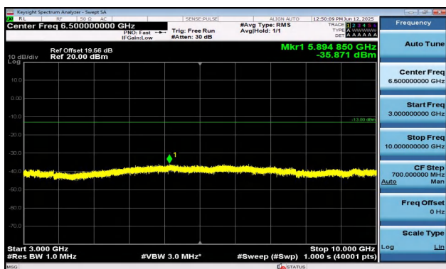
Band12-3MHz-QPSK-23095-15RB#0-3000~10000-PASS
