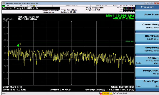
Band12-3MHz-QPSK-23095-15RB#0-0.009~0.15-PASS
