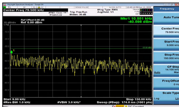
Band12-3MHz-16QAM-23025-15RB#0-0.009~0.15-PASS
