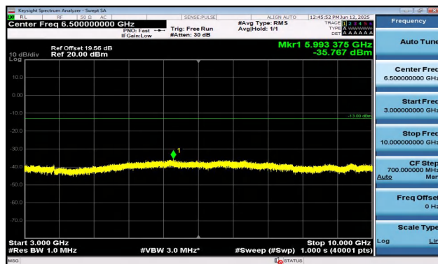
Band12-3MHz-16QAM-23025-15RB#0-3000~10000-PASS
