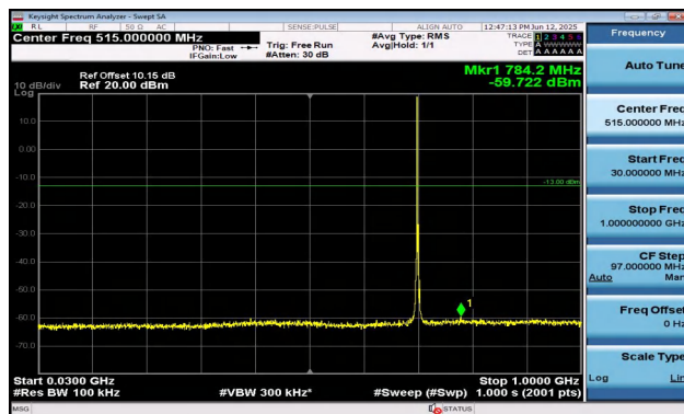
Band12-3MHz-16QAM-23095-1RB#0-30~1000-PASS
