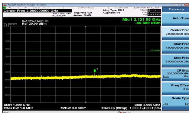
Band12-3MHz-QPSK-23095-15RB#0-1000~3000-PASS
