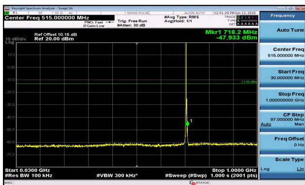
Band12-3MHz-QPSK-23165-1RB#0-30~1000-PASS
