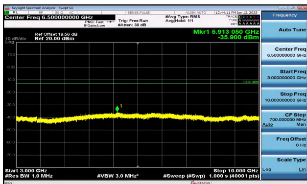
Band12-3MHz-16QAM-23025-1RB#14-3000~10000-PASS
