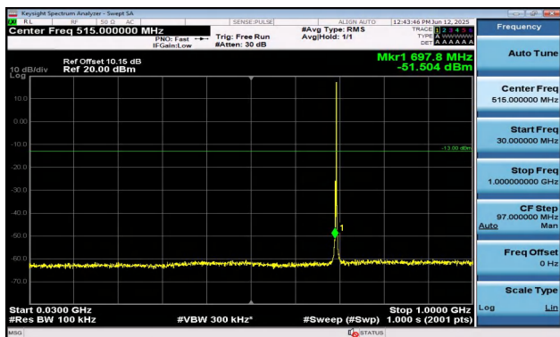
Band12-3MHz-16QAM-23025-1RB#14-30~1000-PASS
