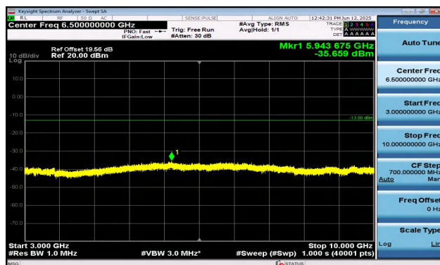
Band12-3MHz-16QAM-23025-1RB#0-3000~10000-PASS
