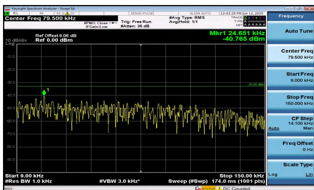
Band12-3MHz-16QAM-23025-1RB#14-0.009~0.15-PASS
