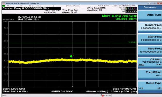
Band12-3MHz-QPSK-23165-1RB#0-3000~10000-PASS
