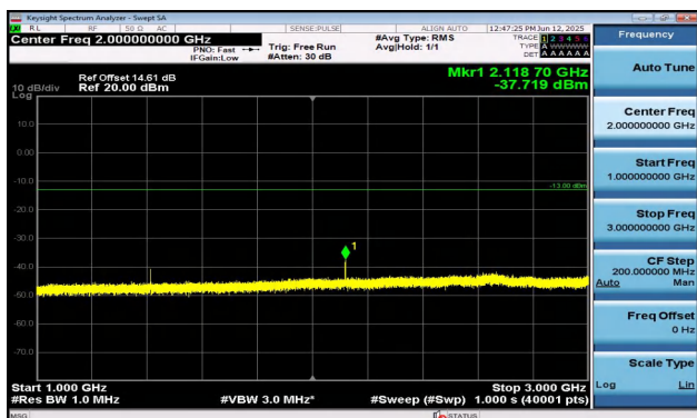
Band12-3MHz-16QAM-23095-1RB#0-1000~3000-PASS
