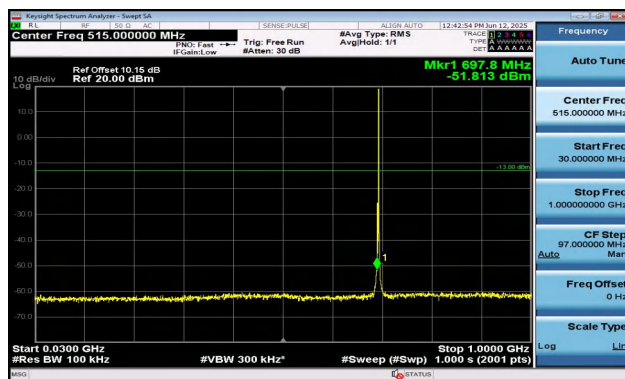
Band12-3MHz-QPSK-23025-1RB#14-30~1000-PASS
