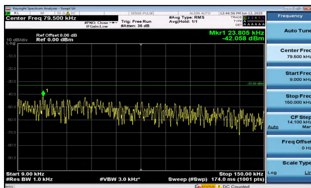
Band12-3MHz-16QAM-23095-1RB#0-0.009~0.15-PASS
