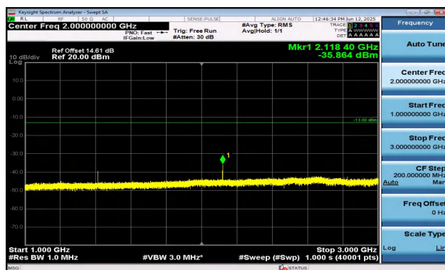
Band12-3MHz-QPSK-23095-1RB#0-1000~3000-PASS
