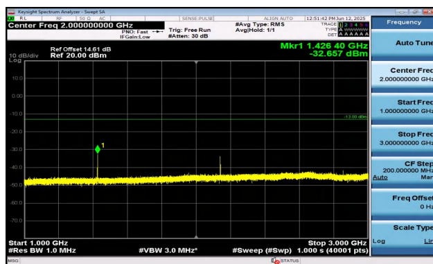
Band12-3MHz-QPSK-23165-1RB#0-1000~3000-PASS
