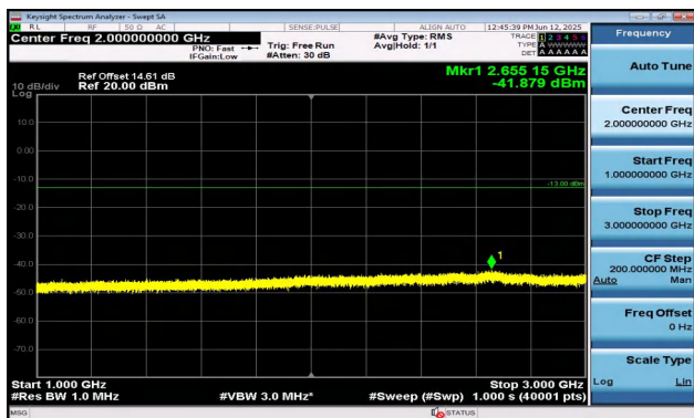
Band12-3MHz-16QAM-23025-15RB#0-1000~3000-PASS
