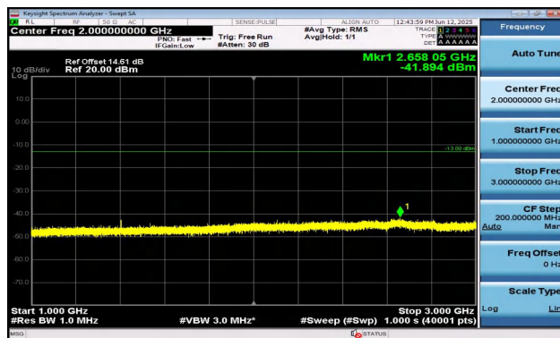
Band12-3MHz-16QAM-23025-1RB#14-1000~3000-PASS
