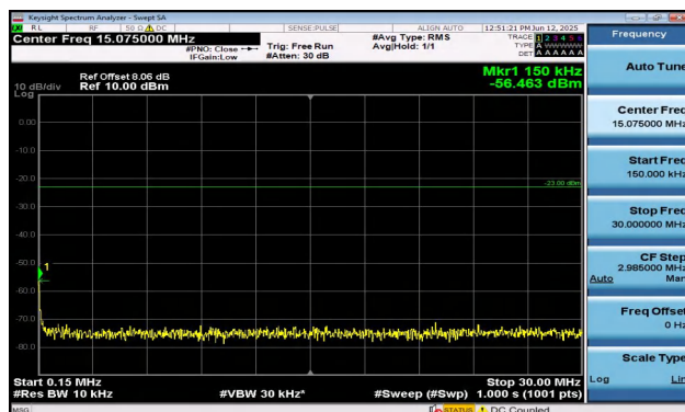
Band12-3MHz-QPSK-23165-1RB#0-0.15~30-PASS
