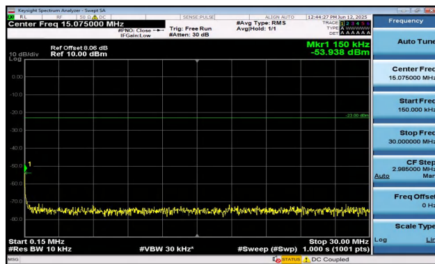
Band12-3MHz-QPSK-23025-15RB#0-0.15~30-PASS
