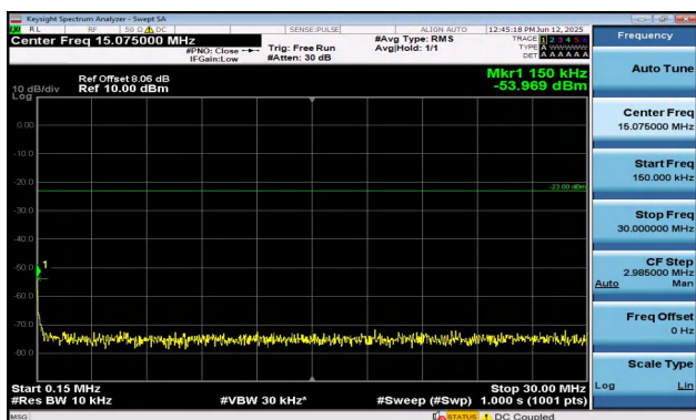
Band12-3MHz-16QAM-23025-15RB#0-0.15~30-PASS
