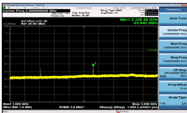
Band12-3MHz-QPSK-23095-1RB#14-1000~3000-PASS
