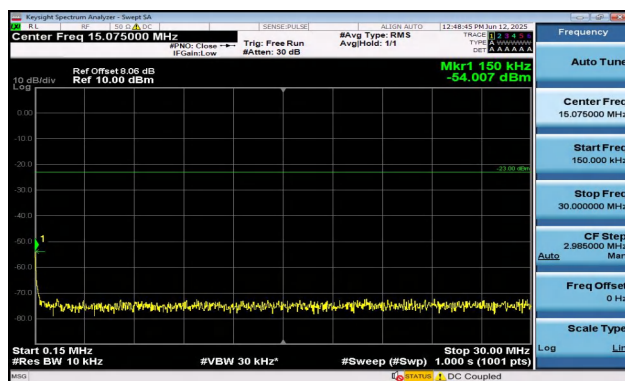
Band12-3MHz-16QAM-23095-1RB#14-0.15~30-PASS
