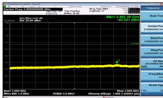
Band12-3MHz-QPSK-23025-15RB#0-1000~3000-PASS
