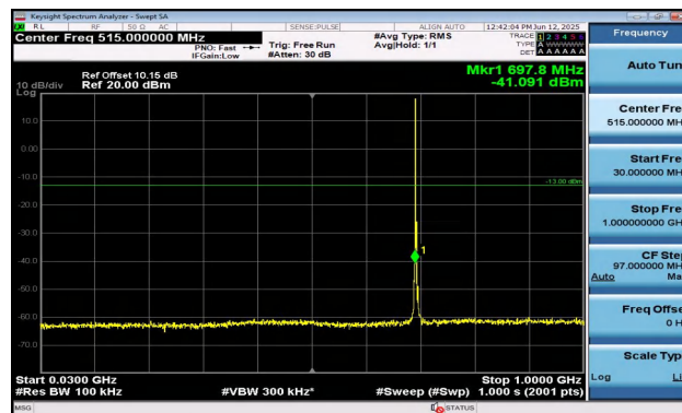
Band12-3MHz-16QAM-23025-1RB#0-30~1000-PASS
