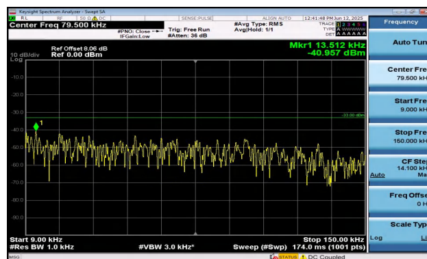
Band12-3MHz-16QAM-23025-1RB#0-0.009~0.15-PASS
