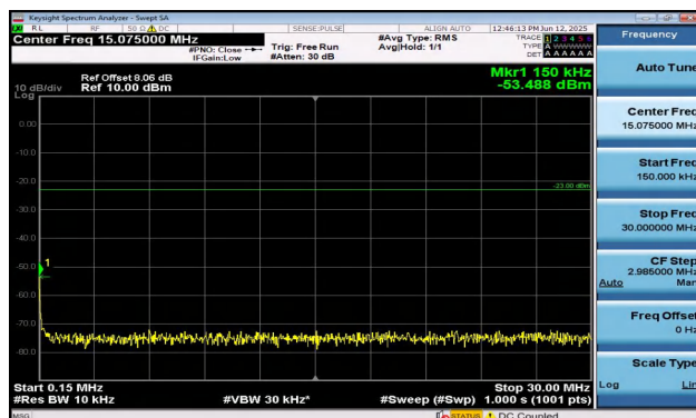
Band12-3MHz-QPSK-23095-1RB#0-0.15~30-PASS
