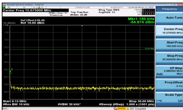
Band12-3MHz-QPSK-23025-1RB#14-0.15~30-PASS
