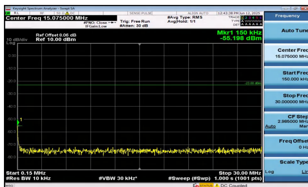
Band12-3MHz-16QAM-23025-1RB#14-0.15~30-PASS
