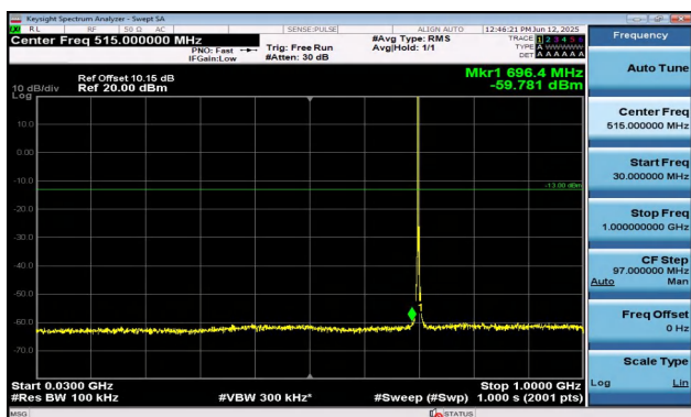
Band12-3MHz-QPSK-23095-1RB#0-30~1000-PASS
