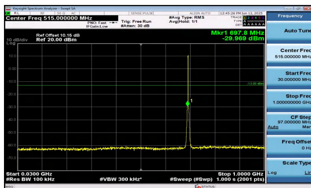
Band12-3MHz-16QAM-23025-15RB#0-30~1000-PASS
