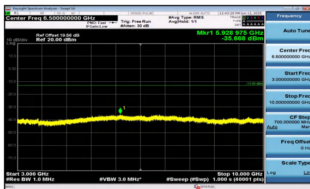
Band12-3MHz-QPSK-23025-1RB#14-3000~10000-PASS
