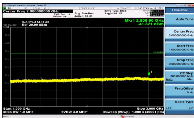
Band12-3MHz-QPSK-23025-1RB#14-1000~3000-PASS
