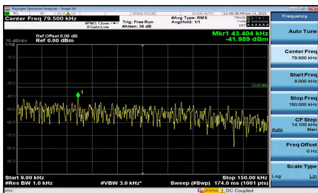
Band12-3MHz-16QAM-23095-1RB#14-0.009~0.15-PASS
