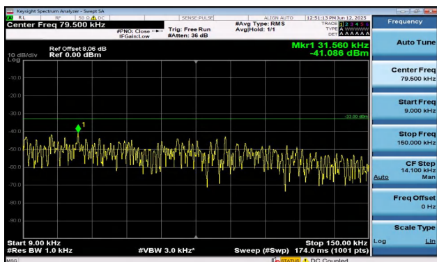
Band12-3MHz-QPSK-23165-1RB#0-0.009~0.15-PASS
