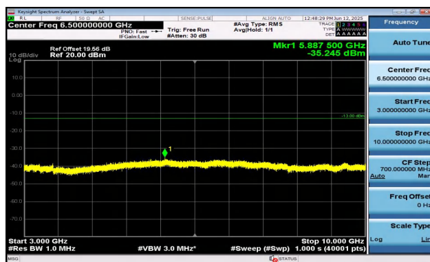
Band12-3MHz-QPSK-23095-1RB#14-3000~10000-PASS
