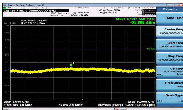
Band12-3MHz-QPSK-23025-15RB#0-3000~10000-PASS
