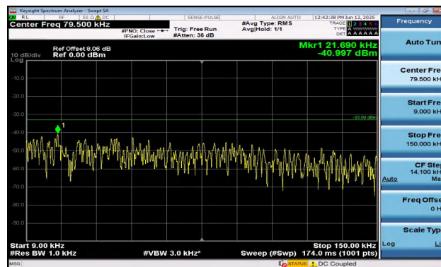
Band12-3MHz-QPSK-23025-1RB#14-0.009~0.15-PASS
