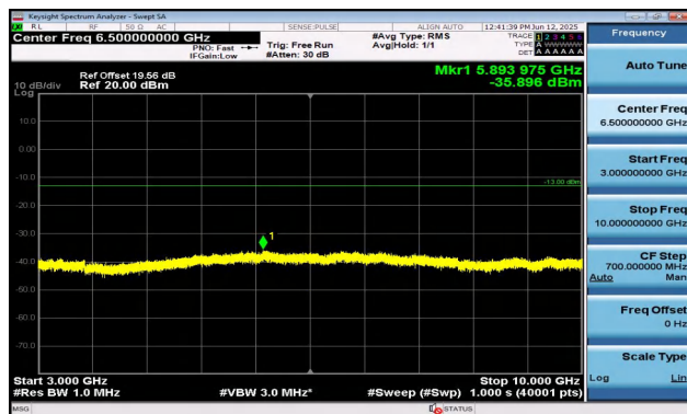
Band12-3MHz-QPSK-23025-1RB#0-3000~10000-PASS
