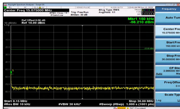
Band12-3MHz-QPSK-23025-1RB#0-0.15~30-PASS
