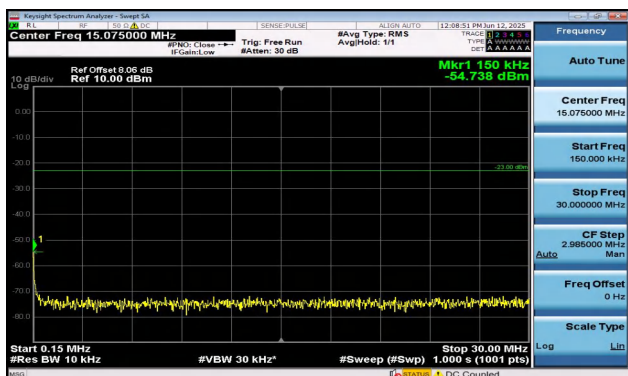
Band12-1.4MHz-QPSK-23173-1RB#5-0.15~30-PASS
