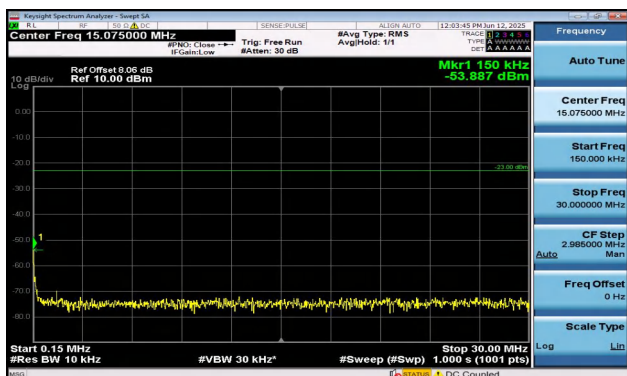
Band12-1.4MHz-QPSK-23095-1RB#5-0.15~30-PASS
