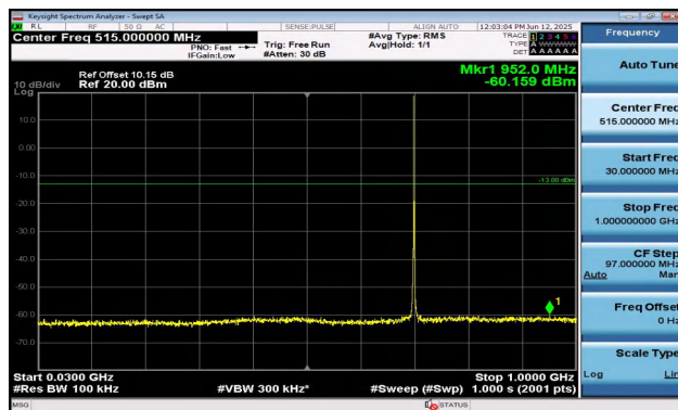
Band12-1.4MHz-16QAM-23095-1RB#0-30~1000-PASS
