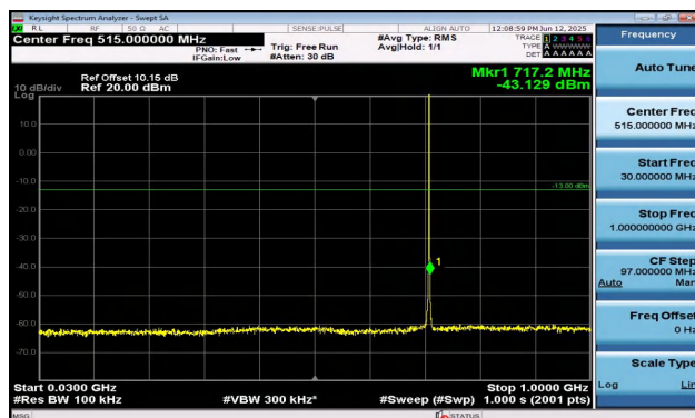
Band12-1.4MHz-QPSK-23173-1RB#5-30~1000-PASS
