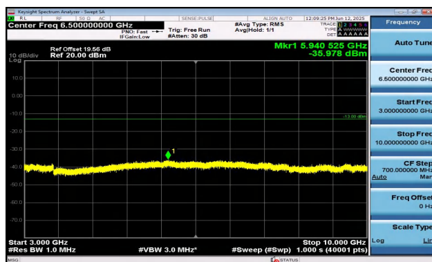
Band12-1.4MHz-QPSK-23173-1RB#5-3000~10000-PASS
