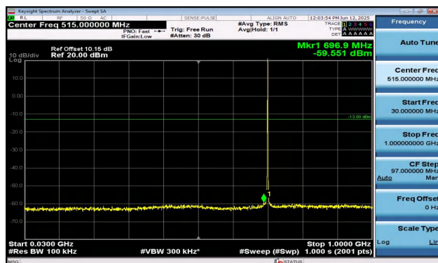
Band12-1.4MHz-QPSK-23095-1RB#5-30~1000-PASS
