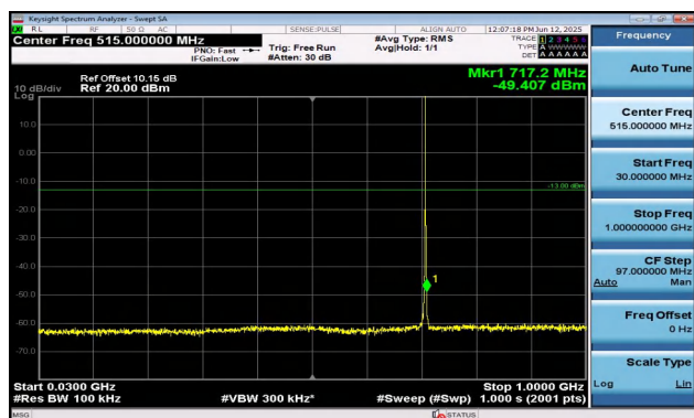
Band12-1.4MHz-QPSK-23173-1RB#0-30~1000-PASS
