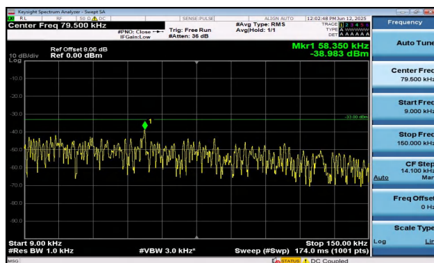
Band12-1.4MHz-16QAM-23095-1RB#0-0.009~0.15-PASS
