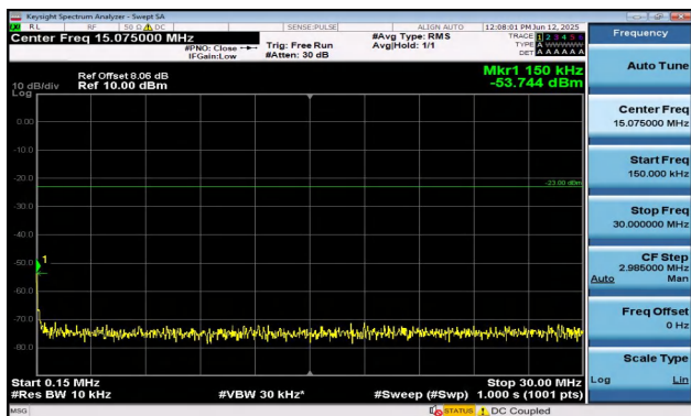
Band12-1.4MHz-16QAM-23173-1RB#0-0.15~30-PASS
