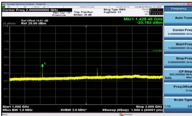
Band12-1.4MHz-16QAM-23173-1RB#0-1000~3000-PASS
