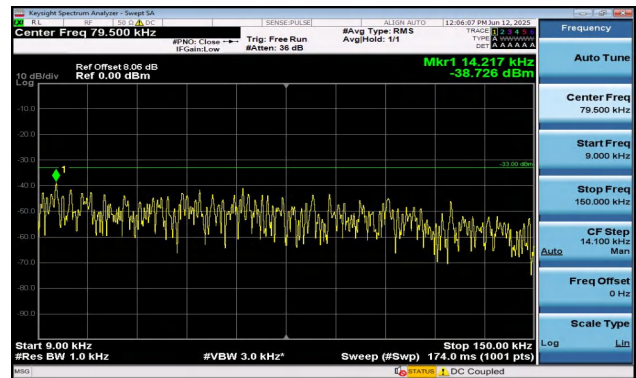
Band12-1.4MHz-16QAM-23095-6RB#0-0.009~0.15-PASS
