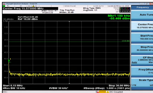
Band12-1.4MHz-QPSK-23095-6RB#0-0.15~30-PASS
