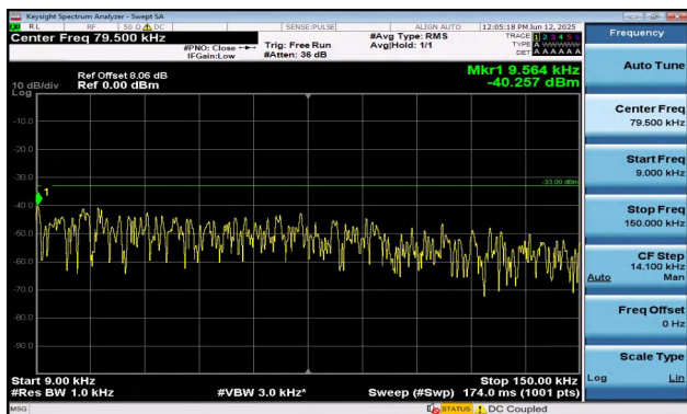
Band12-1.4MHz-QPSK-23095-6RB#0-0.009~0.15-PASS
