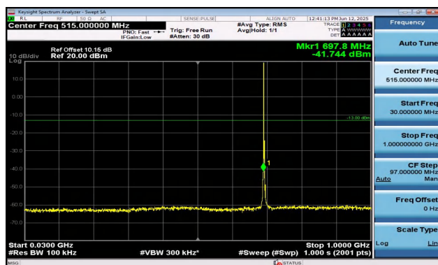
Band12-3MHz-QPSK-23025-1RB#0-30~1000-PASS
