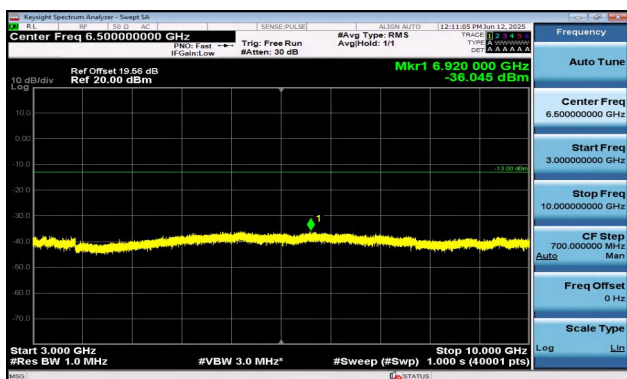
Band12-1.4MHz-QPSK-23173-6RB#0-3000~10000-PASS
