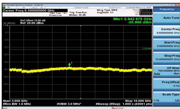
Band12-1.4MHz-QPSK-23095-6RB#0-3000~10000-PASS
