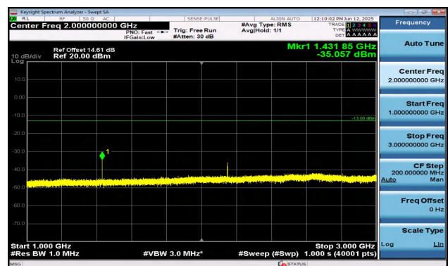
Band12-1.4MHz-16QAM-23173-1RB#5-1000~3000-PASS
