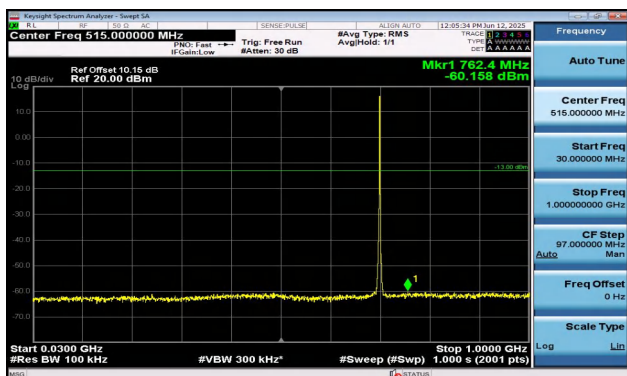
Band12-1.4MHz-QPSK-23095-6RB#0-30~1000-PASS
