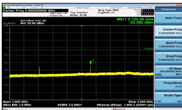
Band12-1.4MHz-QPSK-23095-1RB#5-1000~3000-PASS
