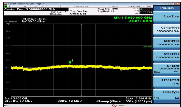
Band12-1.4MHz-16QAM-23173-1RB#0-3000~10000-PASS S
