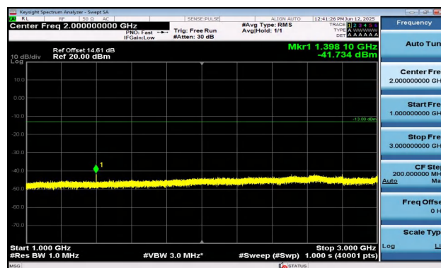
Band12-3MHz-QPSK-23025-1RB#0-1000~3000-PASS
