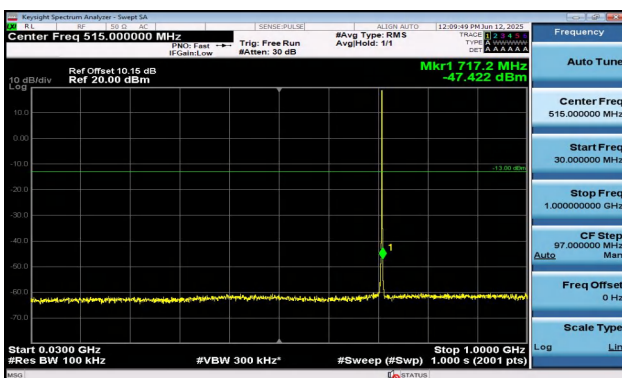
Band12-1.4MHz-16QAM-23173-1RB#5-30~1000-PASS
