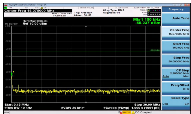
Band12-1.4MHz-16QAM-23173-1RB#5-0.15~30-PASS
