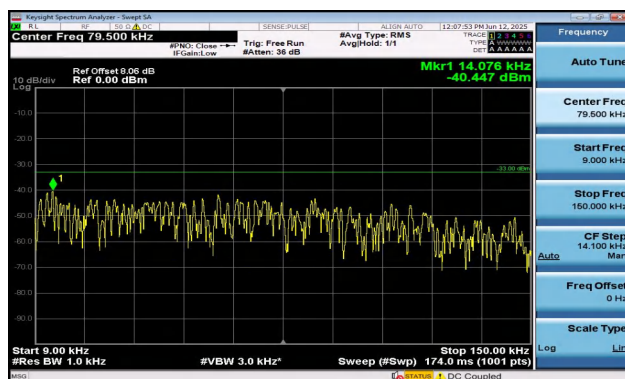
Band12-1.4MHz-16QAM-23173-1RB#0-0.009~0.15-PASS
