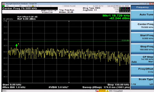
Band12-1.4MHz-QPSK-23173-6RB#0-0.009~0.15-PASS
