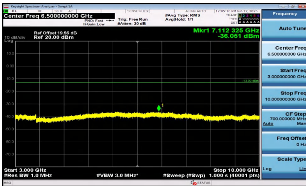
Band12-1.4MHz-16QAM-23095-1RB#5-3000~10000-PAS S
