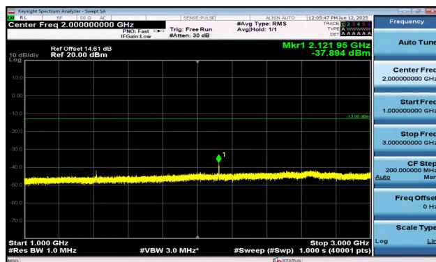
Band12-1.4MHz-QPSK-23095-6RB#0-1000~3000-PASS
