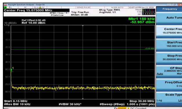
Band12-1.4MHz-QPSK-23173-1RB#0-0.15~30-PASS
