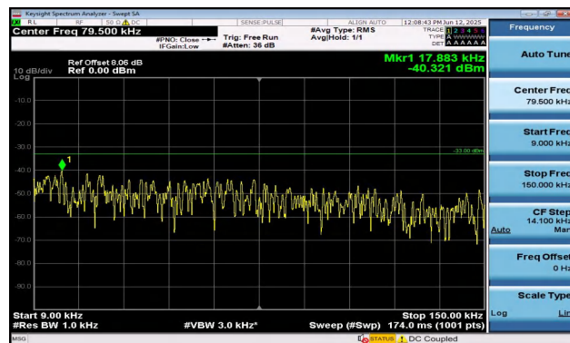
Band12-1.4MHz-QPSK-23173-1RB#5-0.009~0.15-PASS
