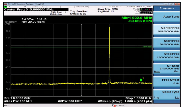
Band12-1.4MHz-16QAM-23095-6RB#0-30~1000-PASS
