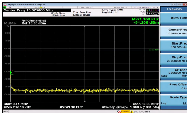
Band12-1.4MHz-QPSK-23173-6RB#0-0.15~30-PASS
