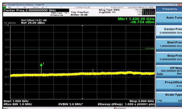
Band12-1.4MHz-QPSK-23173-6RB#0-1000~3000-PASS
