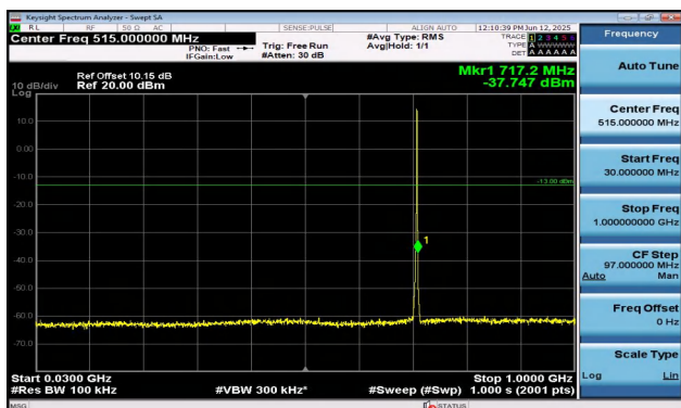
Band12-1.4MHz-QPSK-23173-6RB#0-30~1000-PASS
