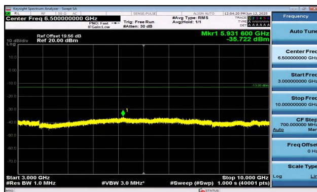
Band12-1.4MHz-QPSK-23095-1RB#5-3000~10000-PASS
