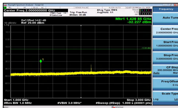
Band12-1.4MHz-QPSK-23173-1RB#0-1000~3000-PASS
