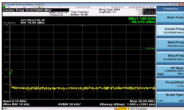
Band12-1.4MHz-16QAM-23095-1RB#0-0.15~30-PASS
