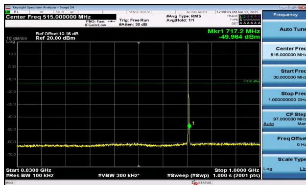
Band12-1.4MHz-16QAM-23173-1RB#0-30~1000-PASS
