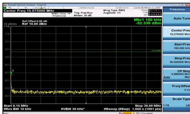
Band12-1.4MHz-QPSK-23095-1RB#0-0.15~30-PASS
