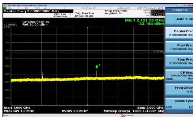
Band12-1.4MHz-QPSK-23095-1RB#0-1000~3000-PASS
