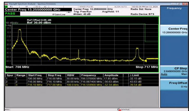
Band12-10MHz-QPSK-23130-1RB#0-PASS
