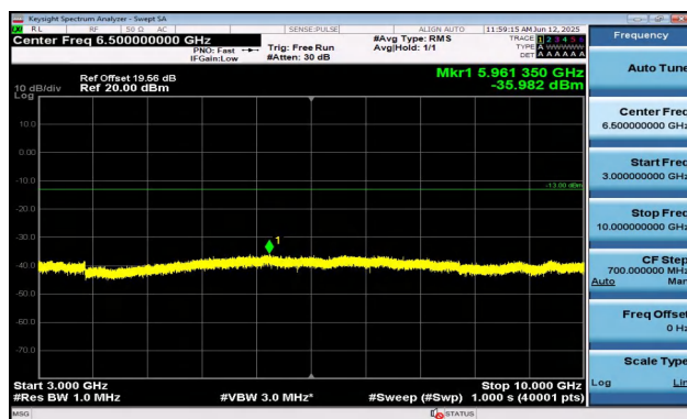
Band12-1.4MHz-QPSK-23017-1RB#5-3000~10000-PASS
