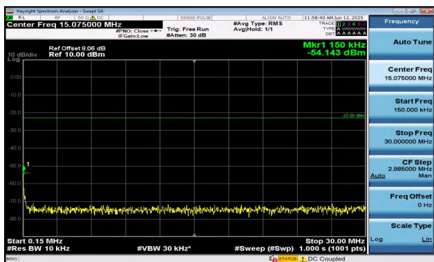
Band12-1.4MHz-QPSK-23017-1RB#5-0.15~30-PASS
