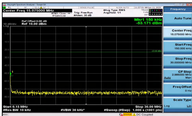
Band12-1.4MHz-16QAM-23017-1RB#0-0.15~30-PASS
