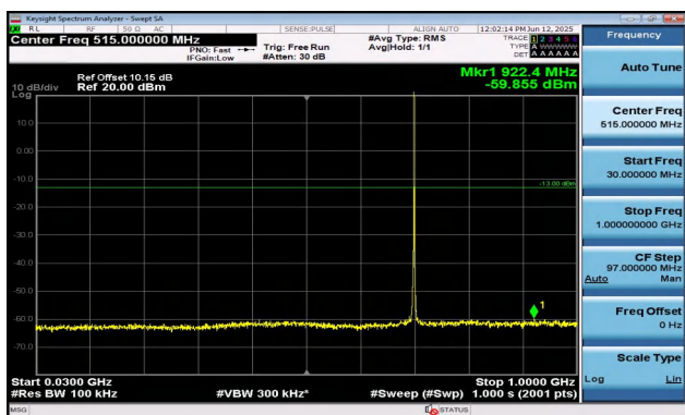
Band12-1.4MHz-QPSK-23095-1RB#0-30~1000-PASS
