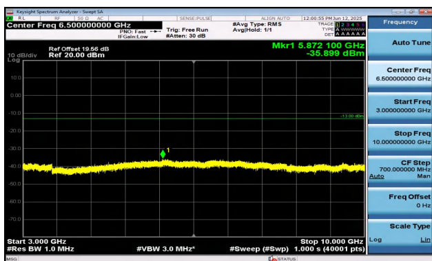
Band12-1.4MHz-QPSK-23017-6RB#0-3000~10000-PASS
