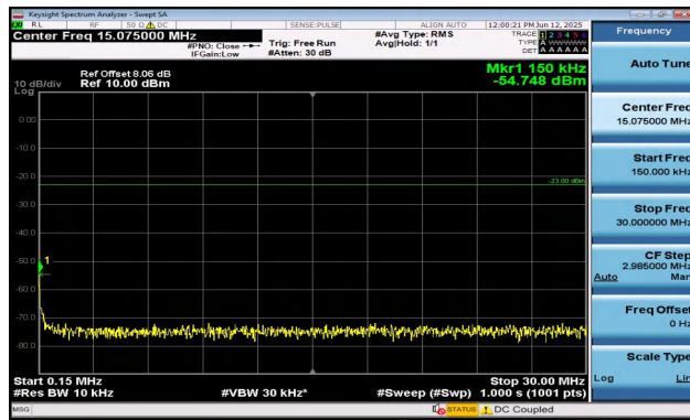
Band12-1.4MHz-QPSK-23017-6RB#0-0.15~30-PASS
