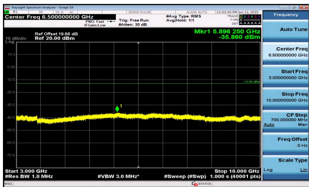
Band12-1.4MHz-QPSK-23095-1RB#0-3000~10000-PASS
