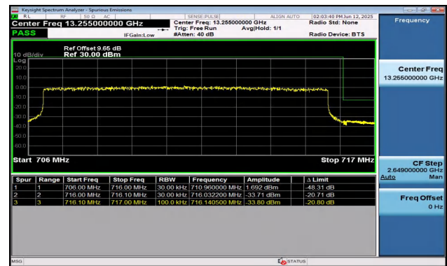
Band12-10MHz-QPSK-23130-50RB#0-PASS
