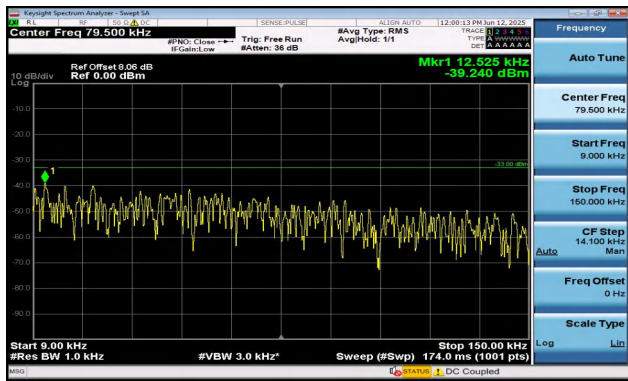
Band12-1.4MHz-QPSK-23017-6RB#0-0.009~0.15-PASS
