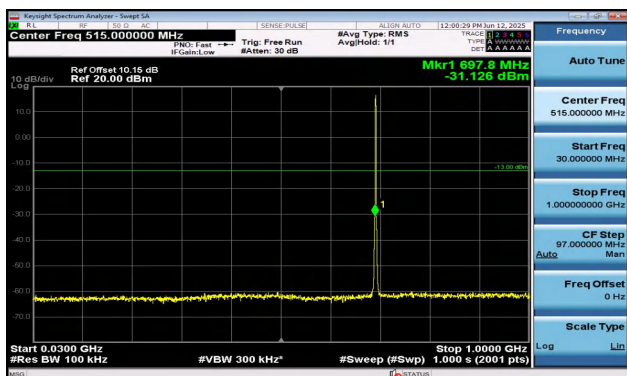
Band12-1.4MHz-QPSK-23017-6RB#0-30~1000-PASS
