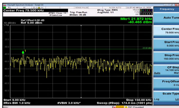
Band12-1.4MHz-16QAM-23017-1RB#0-0.009~0.15-PASS
