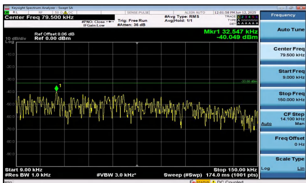
Band12-1.4MHz-QPSK-23095-1RB#0-0.009~0.15-PASS
