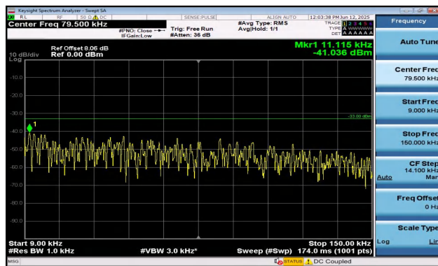
Band12-1.4MHz-QPSK-23095-1RB#5-0.009~0.15-PASS
