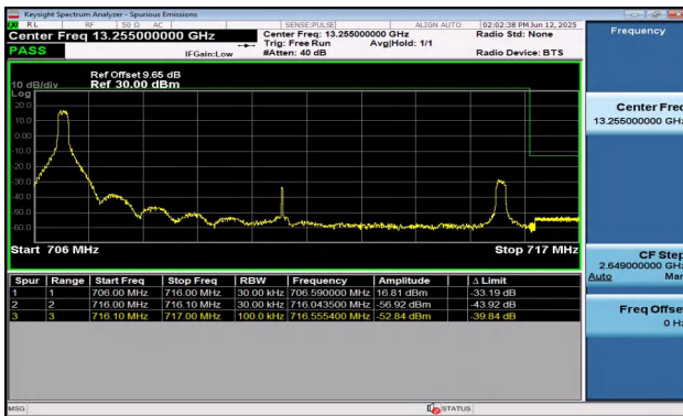
Band12-10MHz-16QAM-23130-1RB#0-PASS
