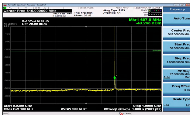
Band12-1.4MHz-QPSK-23017-1RB#5-30~1000-PASS
