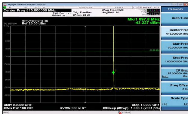
Band12-1.4MHz-16QAM-23017-1RB#0-30~1000-PASS
