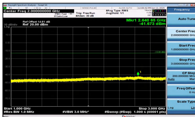
Band12-1.4MHz-QPSK-23017-6RB#0-1000~3000-PASS
