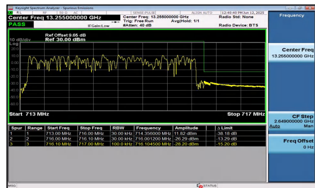
Band12-3MHz-16QAM-23165-15RB#0-PASS
