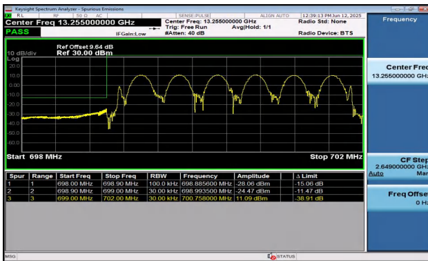
Band12-3MHz-QPSK-23025-15RB#0-PASS
