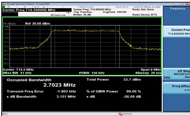
Band12-3MHz-QPSK-23165-15RB#0-PASS
