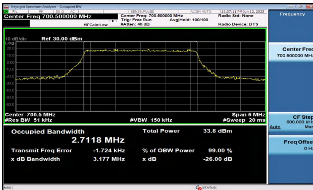
Band12-3MHz-QPSK-23025-15RB#0-PASS
