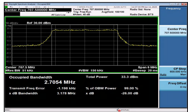
Band12-3MHz-16QAM-23095-15RB#0-PASS
