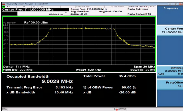
Band12-10MHz-QPSK-23130-50RB#0-PASS
