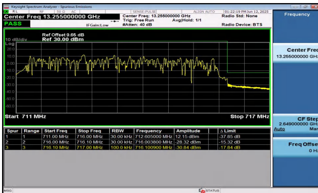
Band12-5MHz-QPSK-23155-25RB#0-PASS
