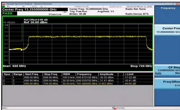
Band12-10MHz-QPSK-23060-50RB#0-PASS
