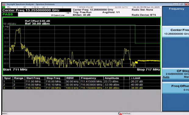
Band12-5MHz-QPSK-23155-1RB#0-PASS
