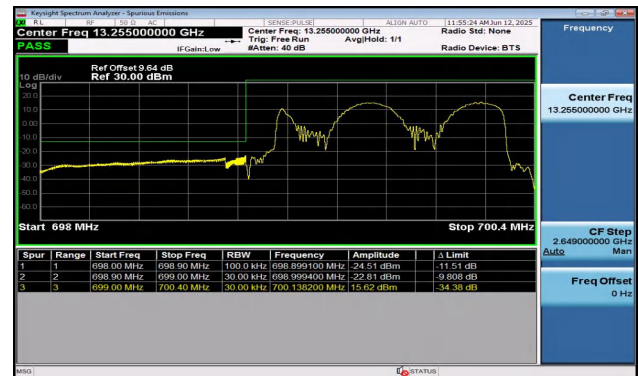
Band12-1.4MHz-16QAM-23017-6RB#0-PASS
