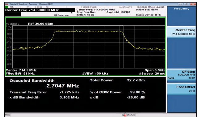
Band12-3MHz-16QAM-23165-15RB#0-PASS
