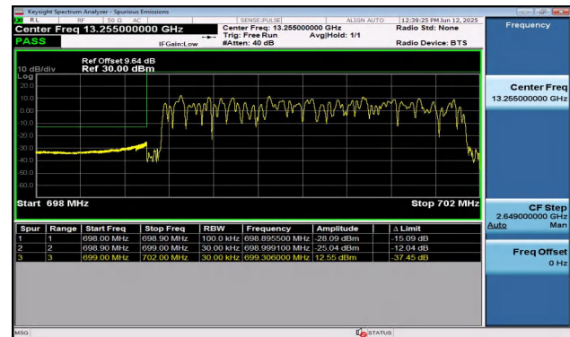
Band12-3MHz-16QAM-23025-15RB#0-PASS
