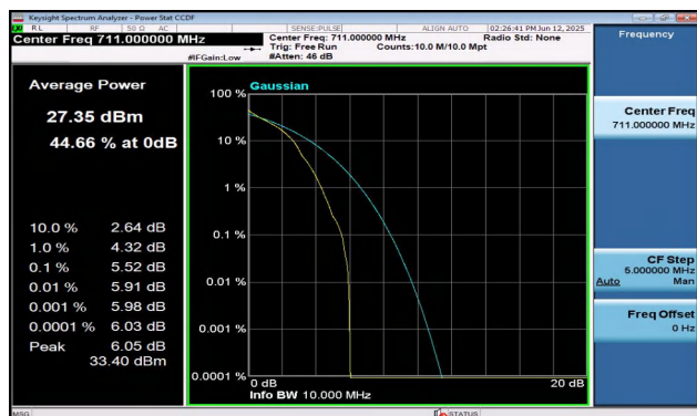
Band12-10MHz-QPSK-23130-1RB#0-PASS
