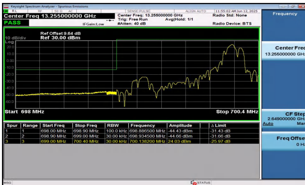
Band12-1.4MHz-16QAM-23017-1RB#5-PASS
