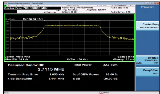
Band12-3MHz-16QAM-23025-15RB#0-PASS
