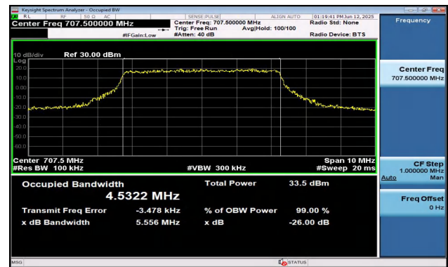
Band12-5MHz-16QAM-23095-25RB#0-PASS
