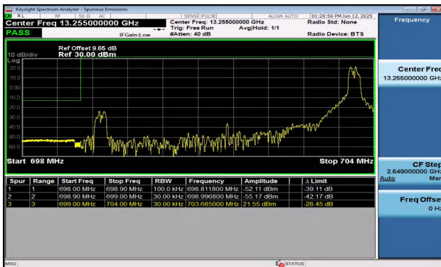
Band12-5MHz-16QAM-23035-1RB#24-PASS
