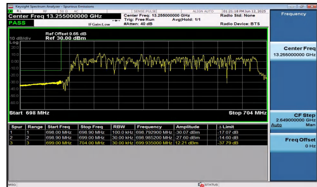
Band12-5MHz-16QAM-23035-25RB#0-PASS
