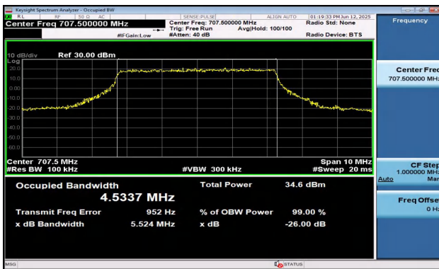
Band12-5MHz-QPSK-23095-25RB#0-PASS
