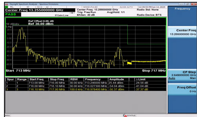
Band12-3MHz-16QAM-23165-1RB#0-PASS
