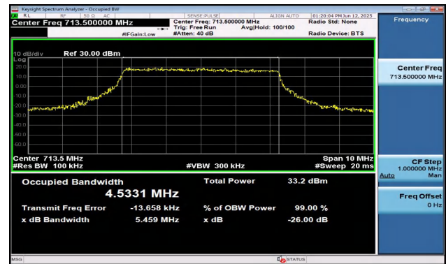
Band12-5MHz-16QAM-23155-25RB#0-PASS
