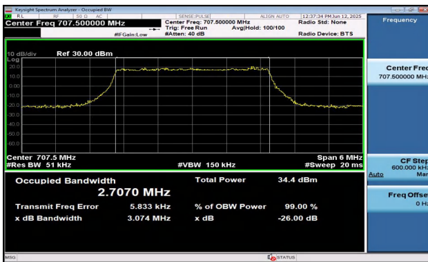
Band12-3MHz-QPSK-23095-15RB#0-PASS
