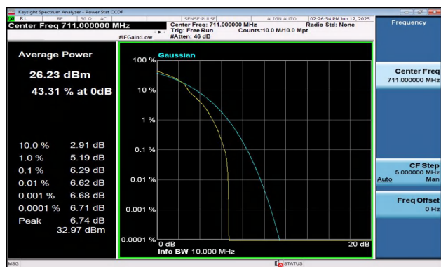
Band12-10MHz-16QAM-23130-1RB#0-PASS
