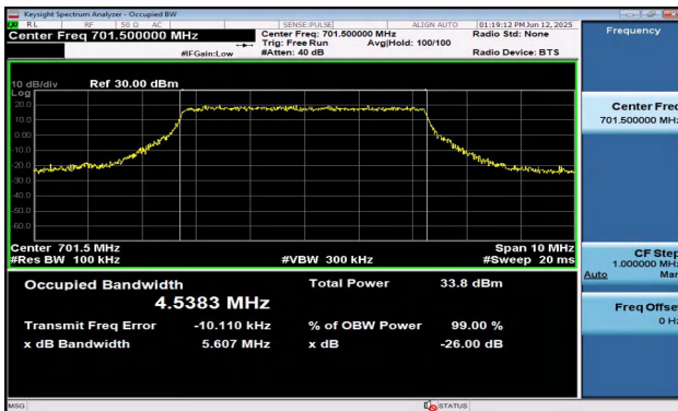
Band12-5MHz-QPSK-23035-25RB#0-PASS
