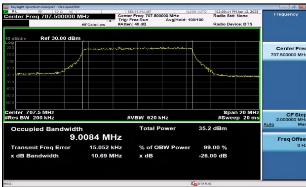
Band12-10MHz-QPSK-23095-50RB#0-PASS
