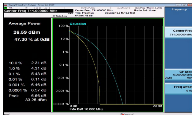
Band12-10MHz-QPSK-23130-50RB#0-PASS
