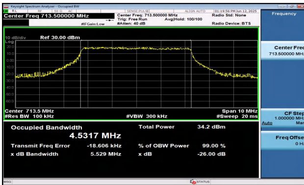
Band12-5MHz-QPSK-23155-25RB#0-PASS
