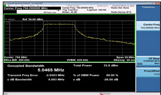
Band12-10MHz-16QAM-23060-27RB#0-PASS
