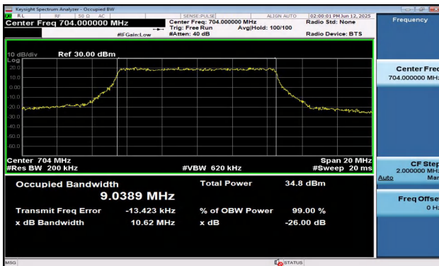
Band12-10MHz-QPSK-23060-50RB#0-PASS
