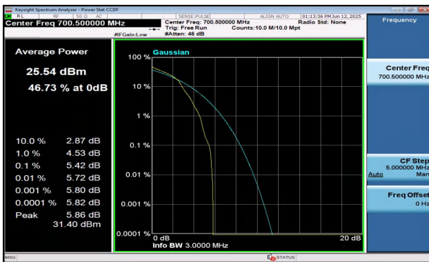
Band12-3MHz-16QAM-23025-1RB#0-PASS
