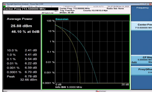
Band12-5MHz-QPSK-23155-25RB#0-PASS
