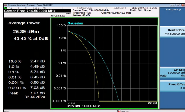
Band12-3MHz-16QAM-23165-15RB#0-PASS
