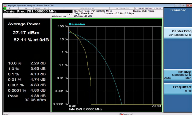
Band12-5MHz-QPSK-23035-1RB#0-PASS
