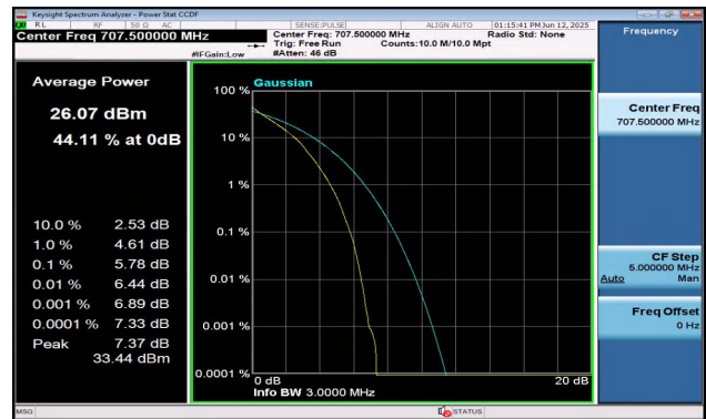
Band12-3MHz-QPSK-23095-15RB#0-PASS
