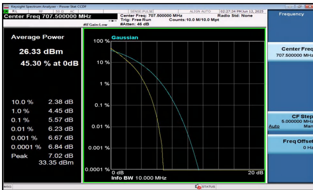
Band12-10MHz-QPSK-23095-50RB#0-PASS
