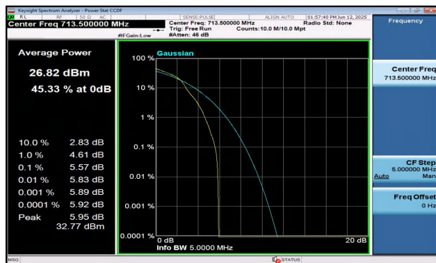
Band12-5MHz-16QAM-23155-1RB#0-PASS
