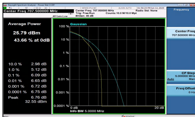
Band12-5MHz-16QAM-23095-1RB#0-PASS
