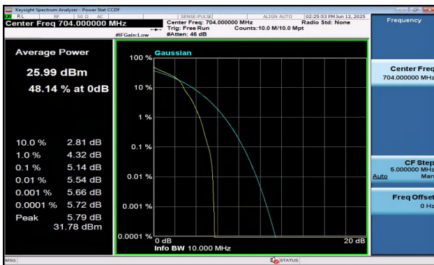
Band12-10MHz-16QAM-23060-1RB#0-PASS
