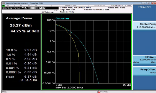
Band12-1.4MHz-16QAM-23173-1RB#0-PASS
