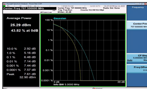
Band12-5MHz-16QAM-23095-25RB#0-PASS
