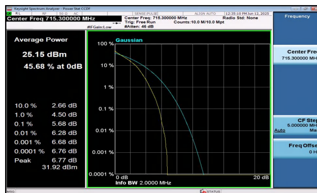
Band12-1.4MHz-QPSK-23173-6RB#0-PASS
