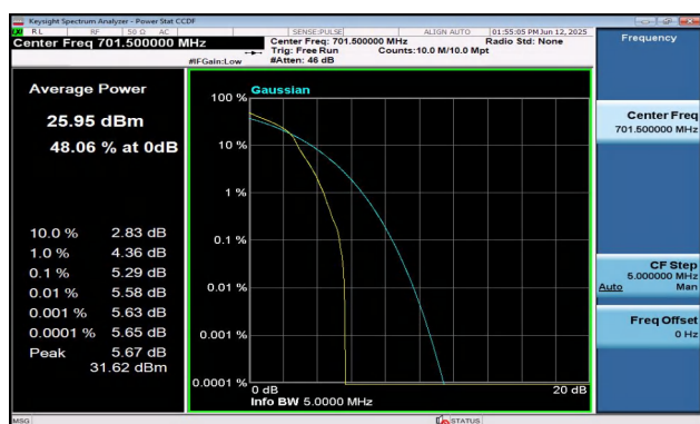
Band12-5MHz-16QAM-23035-1RB#0-PASS
