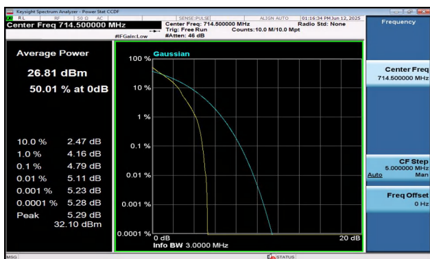
Band12-3MHz-16QAM-23165-1RB#0-PASS
