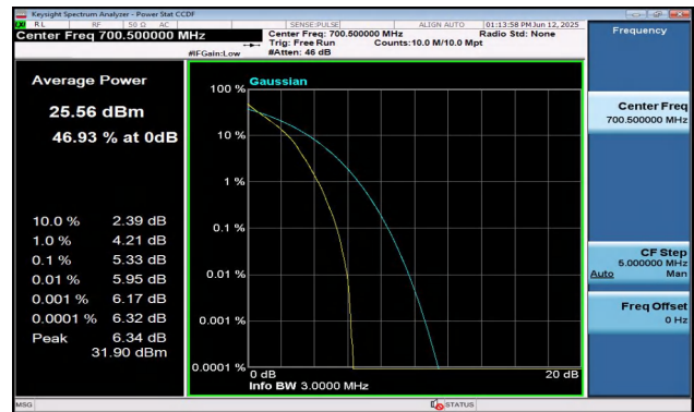
Band12-3MHz-QPSK-23025-15RB#0-PASS
