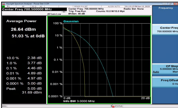
Band12-3MHz-QPSK-23025-1RB#0-PASS
