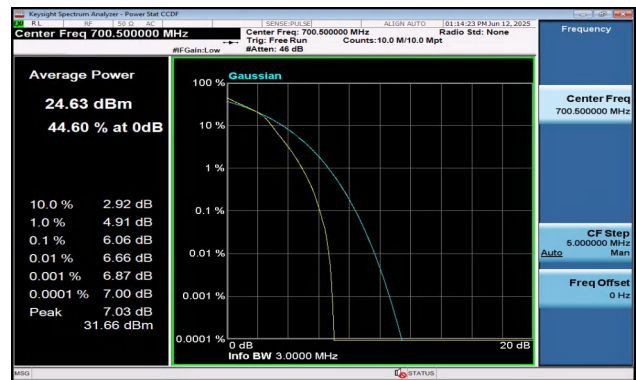
Band12-3MHz-16QAM-23025-15RB#0-PASS
