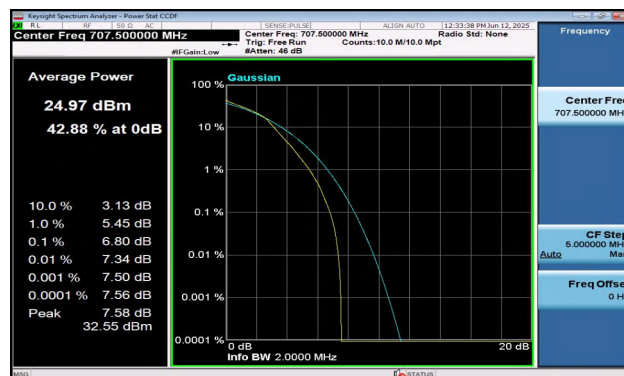
Band12-1.4MHz-16QAM-23095-6RB#0-PASS
