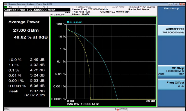
Band12-10MHz-QPSK-23095-1RB#0-PASS
