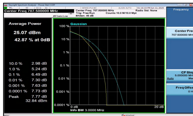
Band12-3MHz-16QAM-23095-15RB#0-PASS
