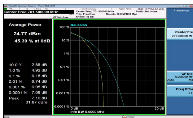
Band12-5MHz-16QAM-23035-25RB#0-PASS
