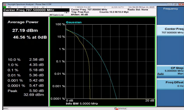
Band12-5MHz-QPSK-23095-1RB#0-PASS
