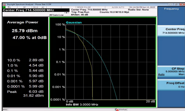
Band12-3MHz-QPSK-23165-1RB#0-PASS
