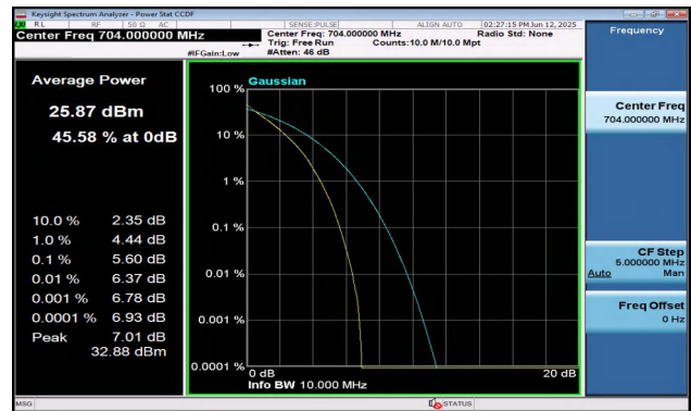
Band12-10MHz-QPSK-23060-50RB#0-PASS
