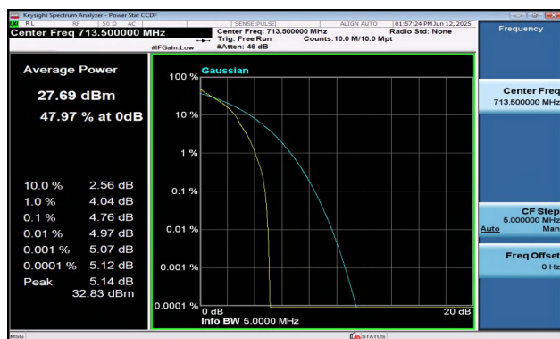
Band12-5MHz-QPSK-23155-1RB#0-PASS
