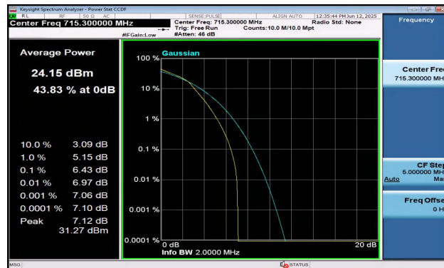
Band12-1.4MHz-16QAM-23173-6RB#0-PASS
