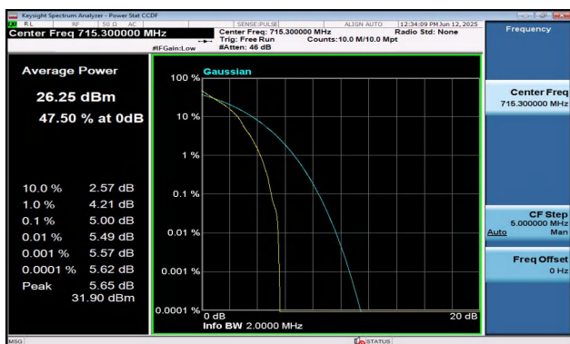
Band12-1.4MHz-QPSK-23173-1RB#0-PASS
