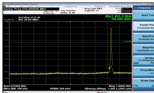
Band5-5MHz-16QAM-20525-25RB#0-30~1000-PASS
