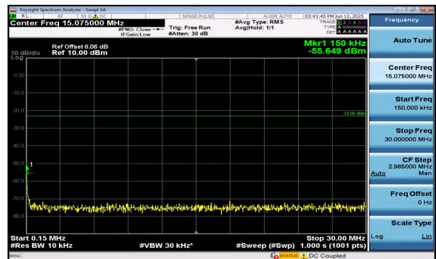
Band5-10MHz-16QAM-20450-1RB#49-0.15~30-PASS
