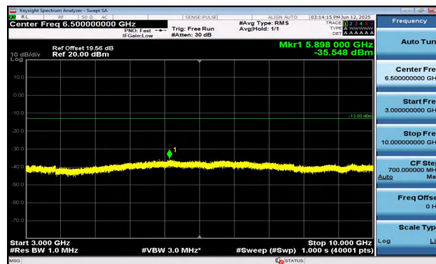
Band5-5MHz-16QAM-20525-25RB#0-3000~10000-PASS
