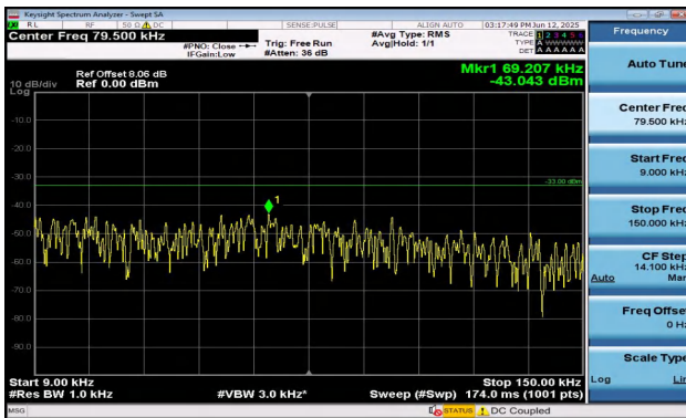
Band5-5MHz-QPSK-20625-25RB#0-0.009~0.15-PASS
