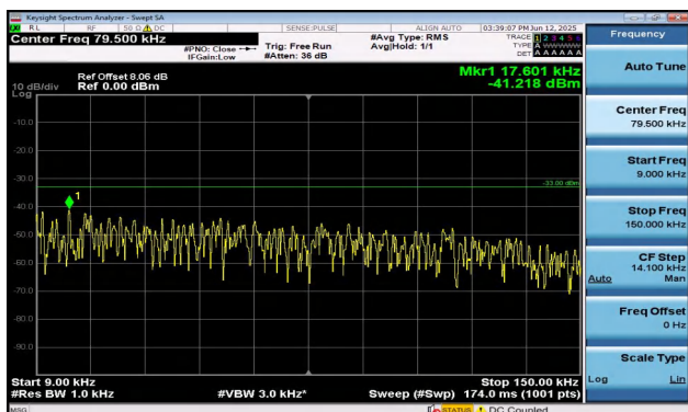
Band5-10MHz-QPSK-20450-1RB#0-0.009~0.15-PASS
