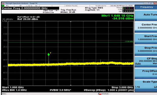
Band5-10MHz-16QAM-20450-1RB#0-1000~3000-PASS
