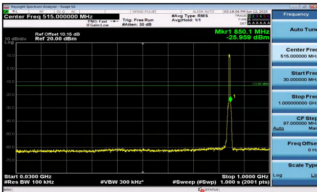
Band5-5MHz-QPSK-20625-25RB#0-30~1000-PASS
