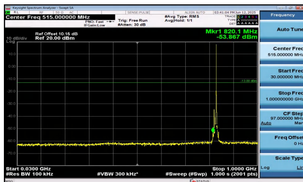
Band5-10MHz-QPSK-20450-1RB#49-30~1000-PASS
