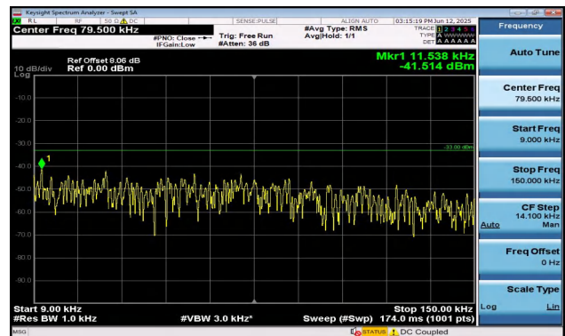
Band5-5MHz-16QAM-20625-1RB#0-0.009~0.15-PASS
