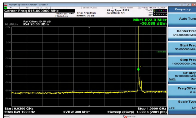
Band5-10MHz-16QAM-20450-1RB#0-30~1000-PASS
