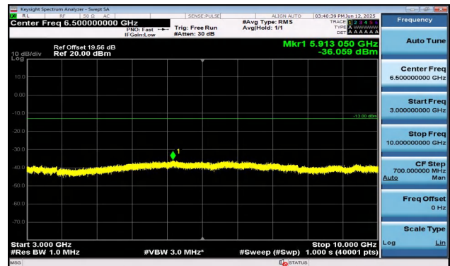
Band5-10MHz-16QAM-20450-1RB#0-3000~10000-PASS
