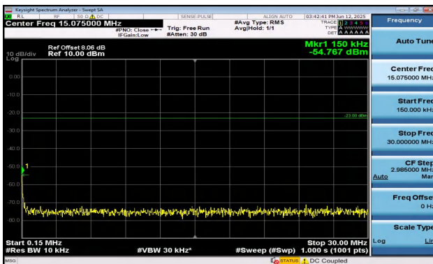
Band5-10MHz-QPSK-20525-1RB#0-0.15~30-PASS
