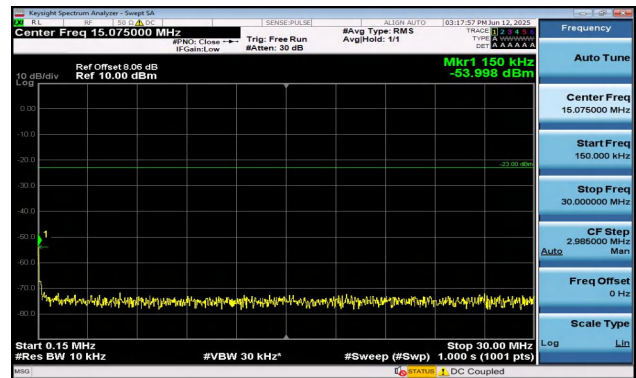
Band5-5MHz-QPSK-20625-25RB#0-0.15~30-PASS
