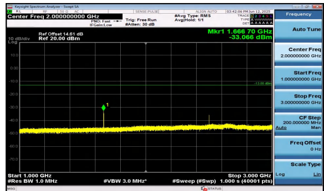
Band5-10MHz-16QAM-20450-1RB#49-1000~3000-PASS
