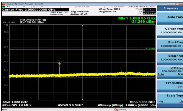
Band5-5MHz-16QAM-20625-1RB#0-1000~3000-PASS
