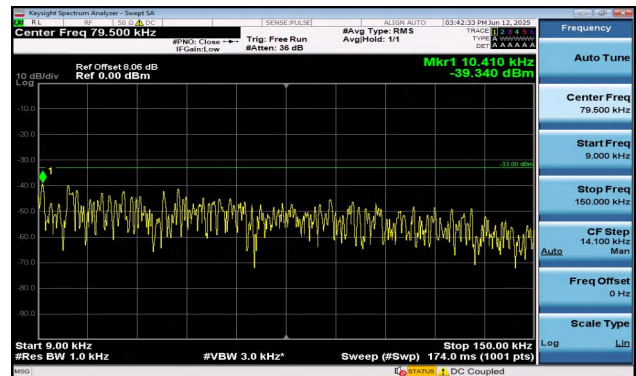
Band5-10MHz-QPSK-20525-1RB#0-0.009~0.15-PASS
