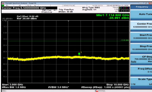
Band5-10MHz-16QAM-20450-1RB#49-3000~10000-PASS
