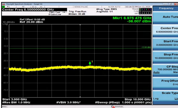
Band5-5MHz-QPSK-20625-25RB#0-3000~10000-PASS
