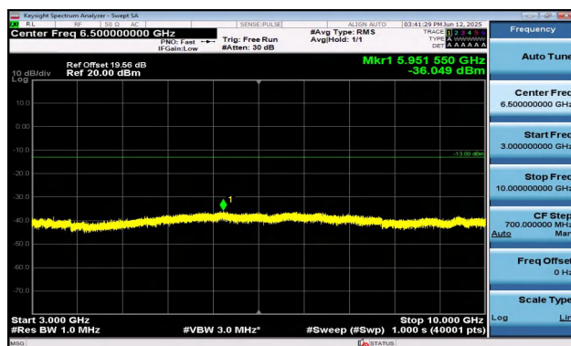
Band5-10MHz-QPSK-20450-1RB#49-3000~10000-PASS
