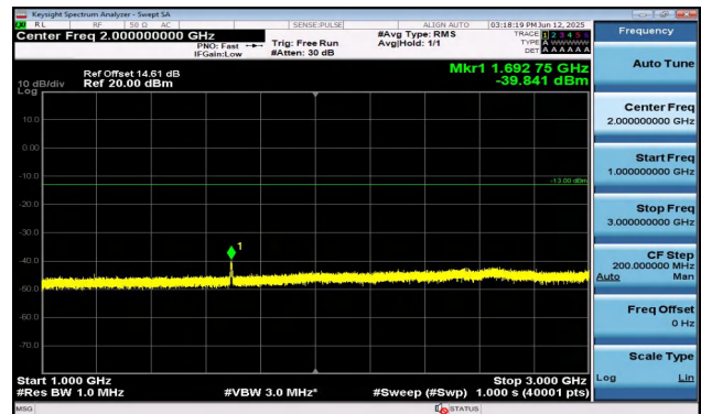
Band5-5MHz-QPSK-20625-25RB#0-1000~3000-PASS
