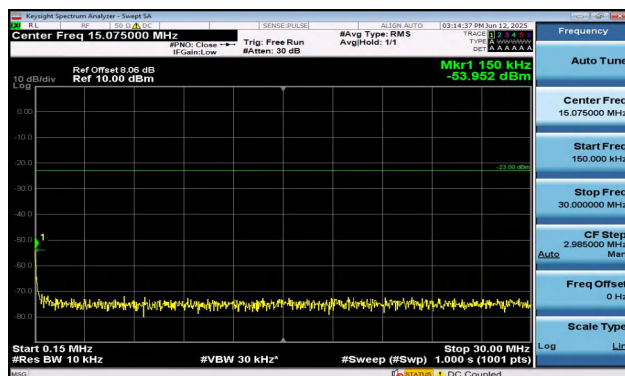
Band5-5MHz-QPSK-20625-1RB#0-0.15~30-PASS
