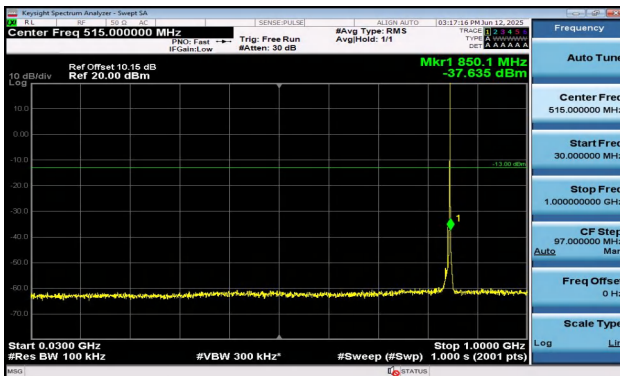
Band5-5MHz-16QAM-20625-1RB#24-30~1000-PASS
