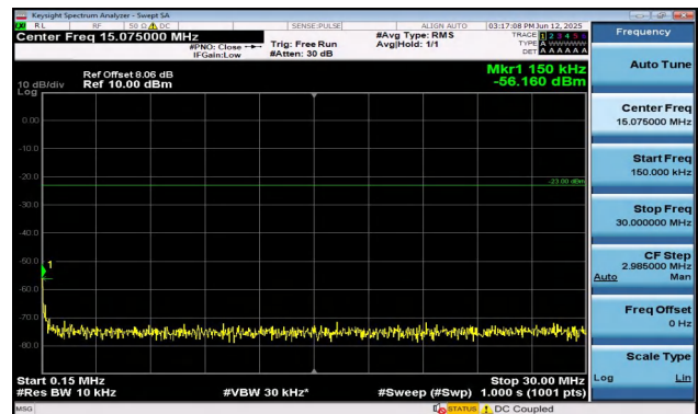
Band5-5MHz-16QAM-20625-1RB#24-0.15~30-PASS
