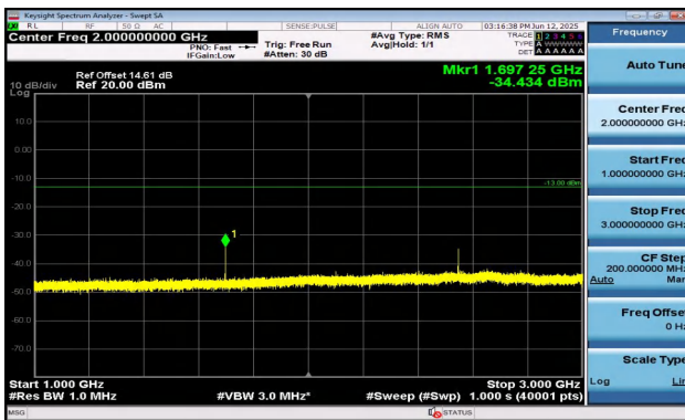
Band5-5MHz-QPSK-20625-1RB#24-1000~3000-PASS
