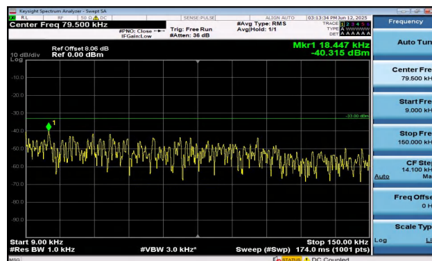
Band5-5MHz-16QAM-20525-25RB#0-0.009~0.15-PASS
