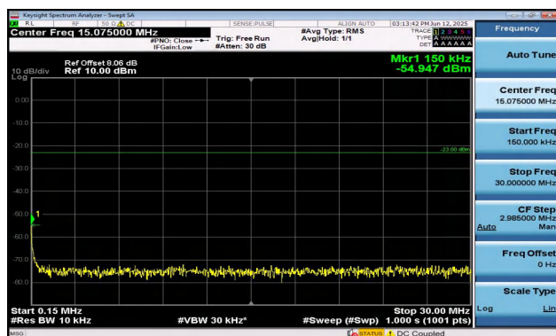
Band5-5MHz-16QAM-20525-25RB#0-0.15~30-PASS
