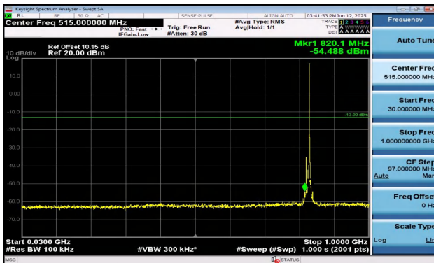
Band5-10MHz-16QAM-20450-1RB#49-30~1000-PASS
