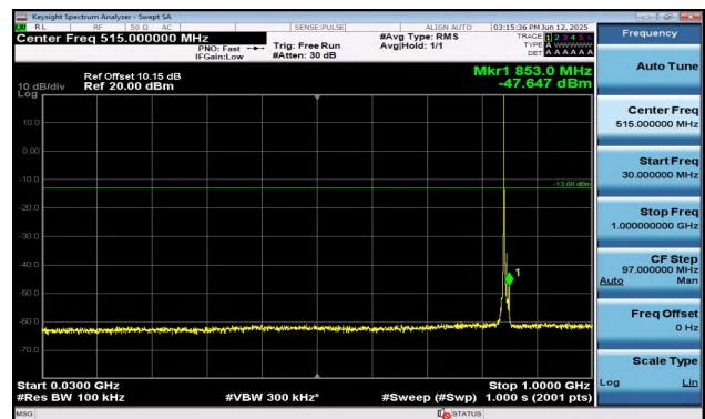
Band5-5MHz-16QAM-20625-1RB#0-30~1000-PASS
