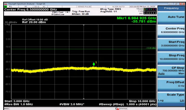
Band5-5MHz-16QAM-20625-1RB#0-3000~10000-PASS
