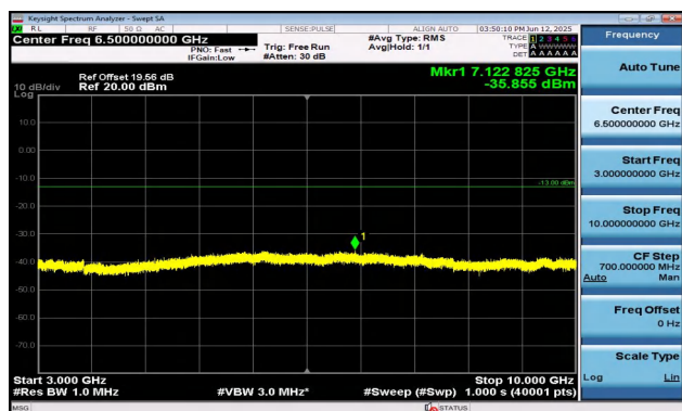
Band5-10MHz-QPSK-20450-50RB#0-3000~10000-PASS
