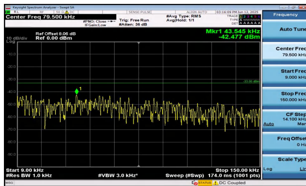
Band5-5MHz-QPSK-20625-1RB#24-0.009~0.15-PASS
