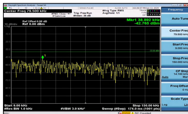
Band5-10MHz-16QAM-20450-1RB#0-0.009~0.15-PASS
