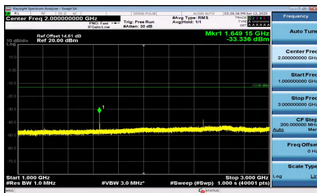
Band5-10MHz-QPSK-20450-1RB#0-1000~3000-PASS
