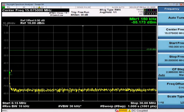
Band5-5MHz-16QAM-20625-1RB#0-0.15~30-PASS
