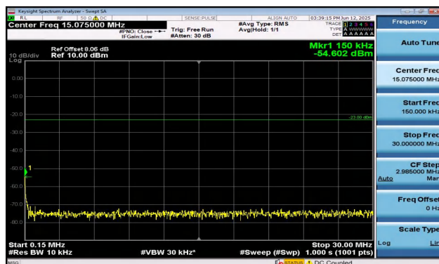
Band5-10MHz-QPSK-20450-1RB#0-0.15~30-PASS
