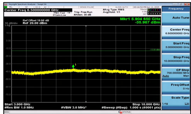
Band5-5MHz-QPSK-20625-1RB#24-3000~10000-PASS
