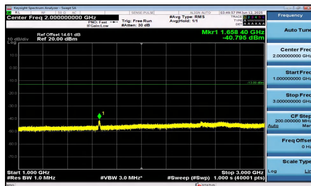
Band5-10MHz-QPSK-20450-50RB#0-1000~3000-PASS
