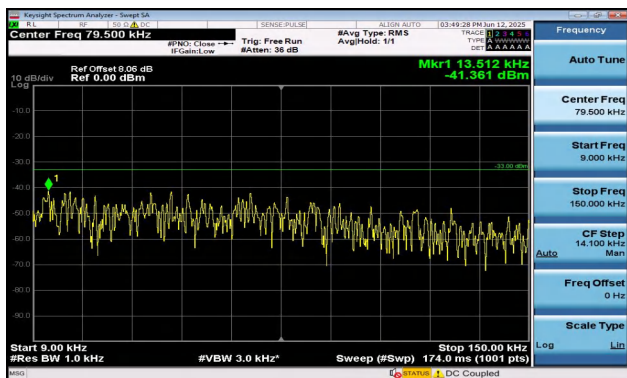
Band5-10MHz-QPSK-20450-50RB#0-0.009~0.15-PASS
