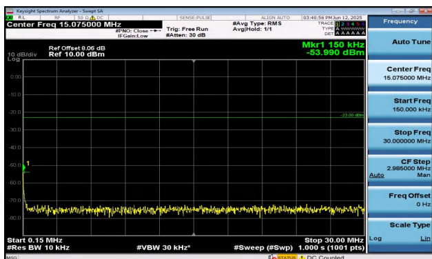
Band5-10MHz-QPSK-20450-1RB#49-0.15~30-PASS
