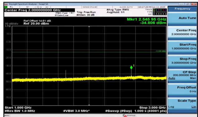
Band5-5MHz-16QAM-20625-1RB#24-1000~3000-PASS
