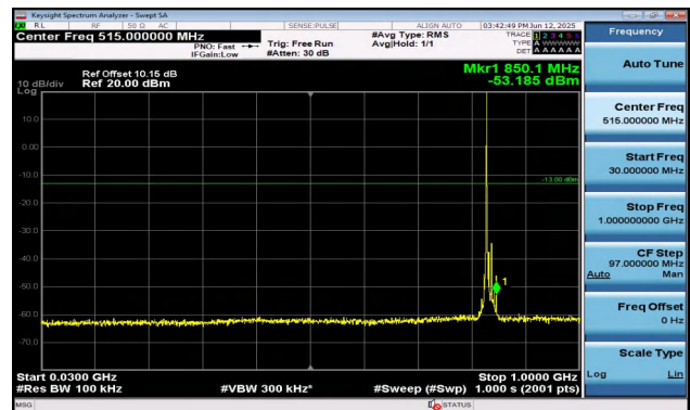
Band5-10MHz-QPSK-20525-1RB#0-30~1000-PASS
