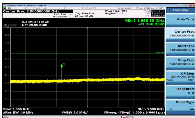
Band5-10MHz-QPSK-20450-1RB#49-1000~3000-PASS
