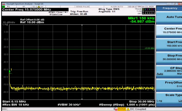
Band5-5MHz-QPSK-20625-1RB#24-0.15~30-PASS
