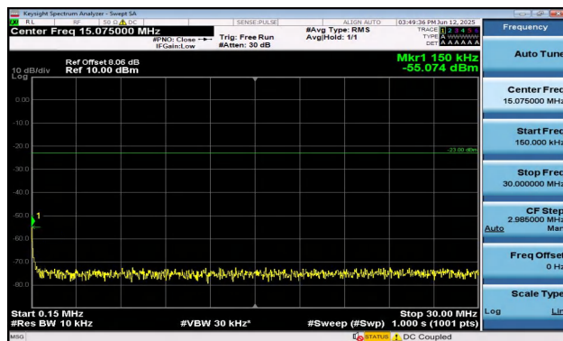
Band5-10MHz-QPSK-20450-50RB#0-0.15~30-PASS
