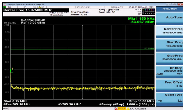
Band5-10MHz-16QAM-20450-1RB#0-0.15~30-PASS
