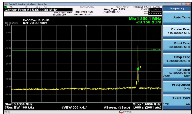
Band5-5MHz-QPSK-20625-1RB#24-30~1000-PASS
