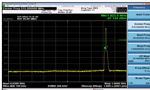
Band5-10MHz-QPSK-20450-50RB#0-30~1000-PASS
