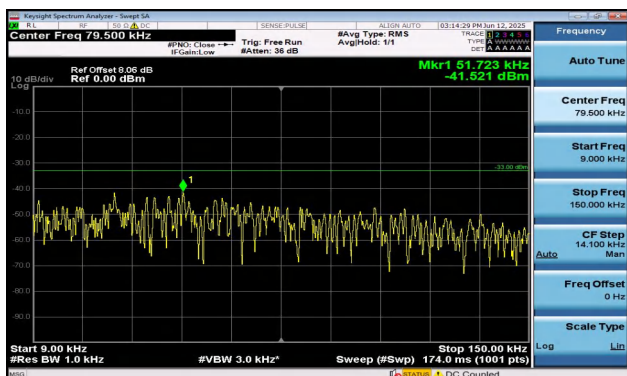
Band5-5MHz-QPSK-20625-1RB#0-0.009~0.15-PASS
