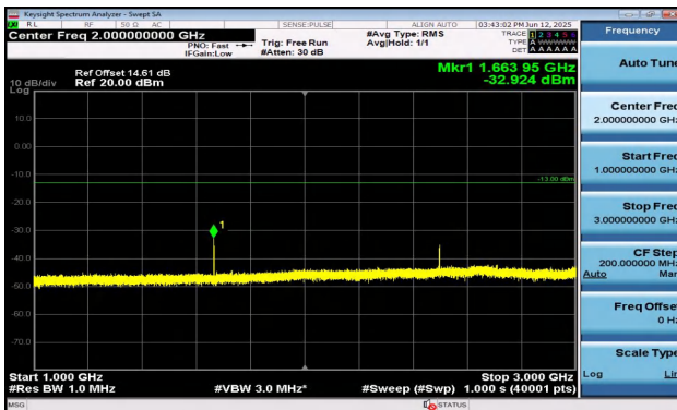
Band5-10MHz-QPSK-20525-1RB#0-1000~3000-PASS
