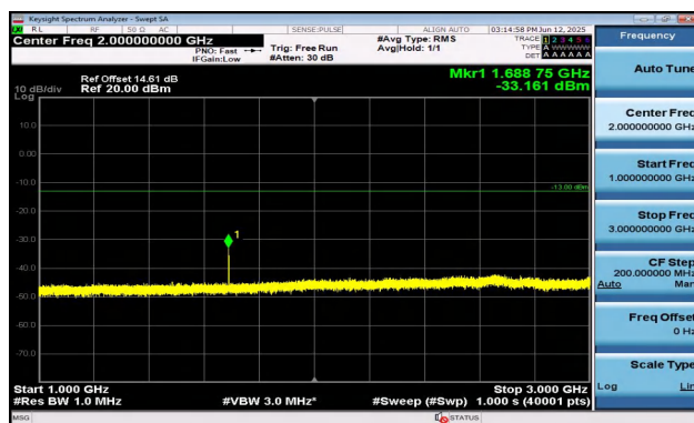
Band5-5MHz-QPSK-20625-1RB#0-1000~3000-PASS
