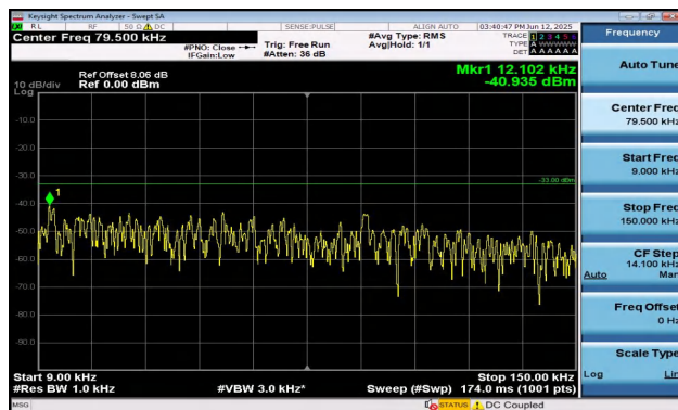
Band5-10MHz-QPSK-20450-1RB#49-0.009~0.15-PASS
