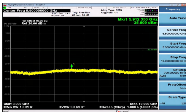
Band5-5MHz-16QAM-20525-1RB#24-3000~10000-PASS
