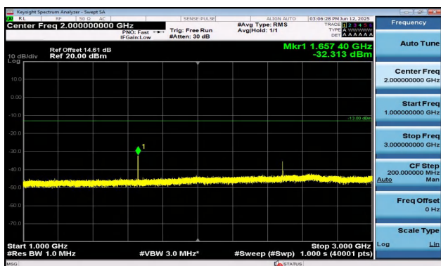
Band5-5MHz-QPSK-20425-1RB#24-1000~3000-PASS
