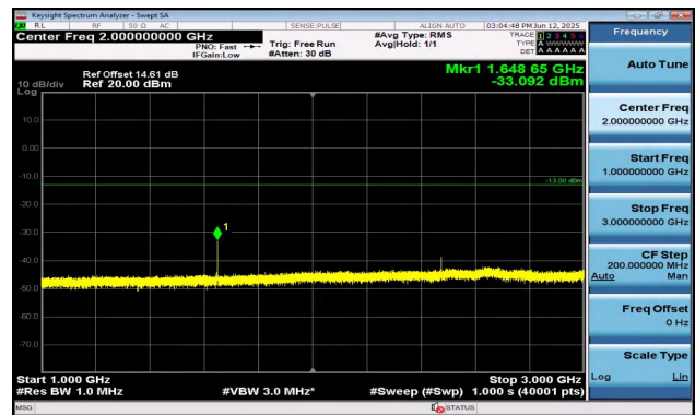
Band5-5MHz-QPSK-20425-1RB#0-1000~3000-PASS
