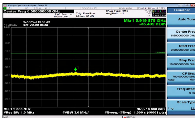
Band5-5MHz-QPSK-20425-1RB#24-3000~10000-PASS
