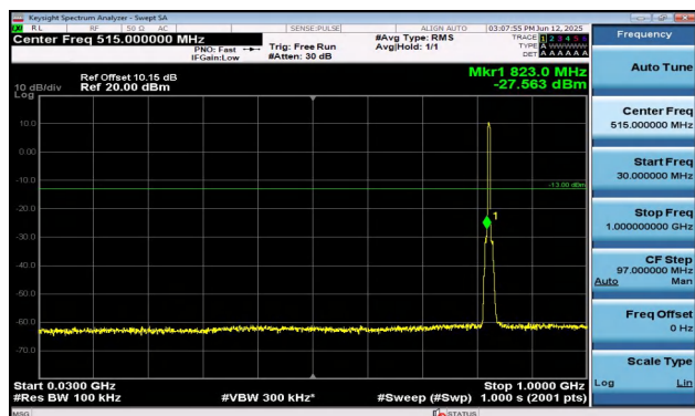
Band5-5MHz-QPSK-20425-25RB#0-30~1000-PASS
