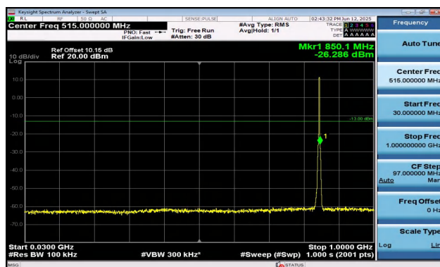
Band5-3MHz-16QAM-20635-15RB#0-30~1000-PASS
