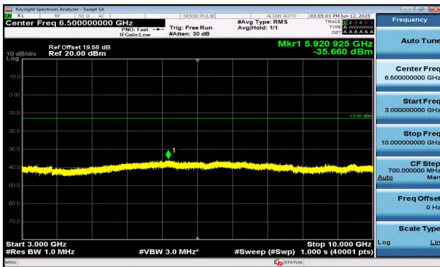
Band5-5MHz-QPSK-20425-1RB#0-3000~10000-PASS
