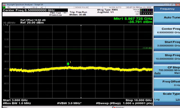
Band5-5MHz-16QAM-20425-1RB#24-3000~10000-PASS
