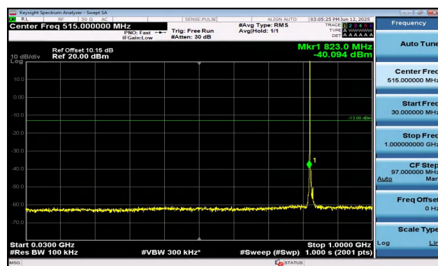
Band5-5MHz-16QAM-20425-1RB#0-30~1000-PASS
