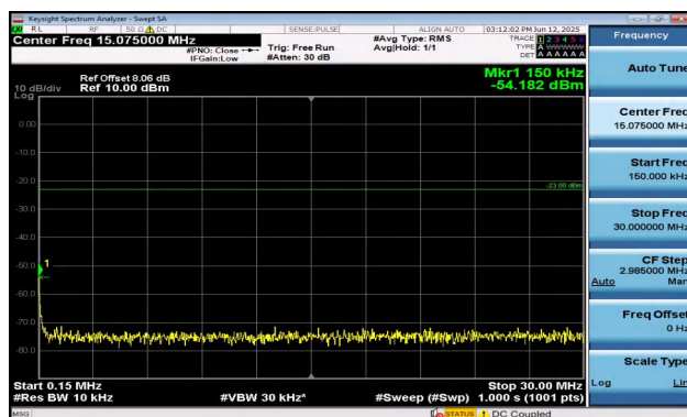
Band5-5MHz-16QAM-20525-1RB#24-0.15~30-PASS
