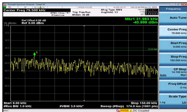
Band5-5MHz-QPSK-20525-25RB#0-0.009~0.15-PASS
