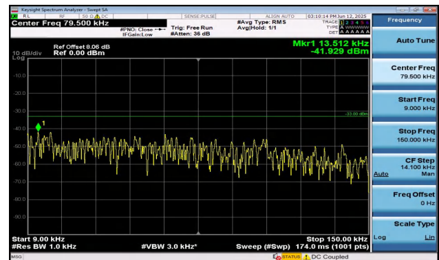
Band5-5MHz-16QAM-20525-1RB#0-0.009~0.15-PASS
