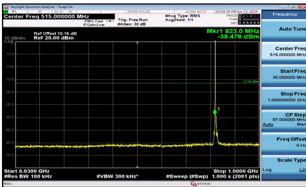
Band5-5MHz-QPSK-20425-1RB#0-30~1000-PASS
