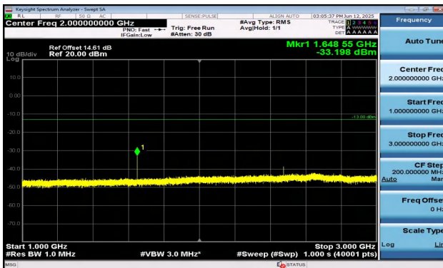
Band5-5MHz-16QAM-20425-1RB#0-1000~3000-PASS
