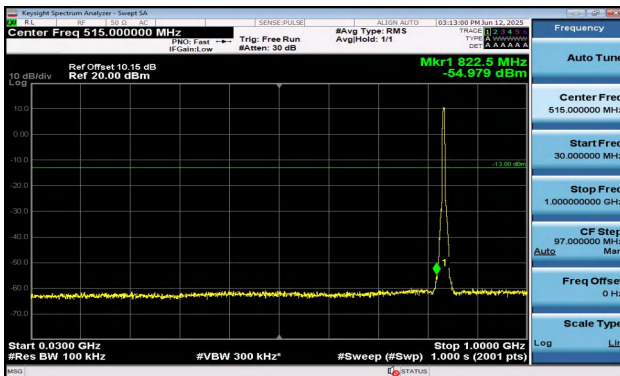
Band5-5MHz-QPSK-20525-25RB#0-30~1000-PASS
