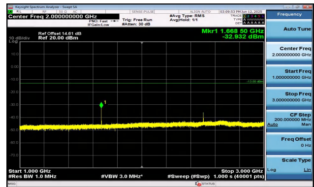
Band5-5MHz-QPSK-20525-1RB#0-1000~3000-PASS
