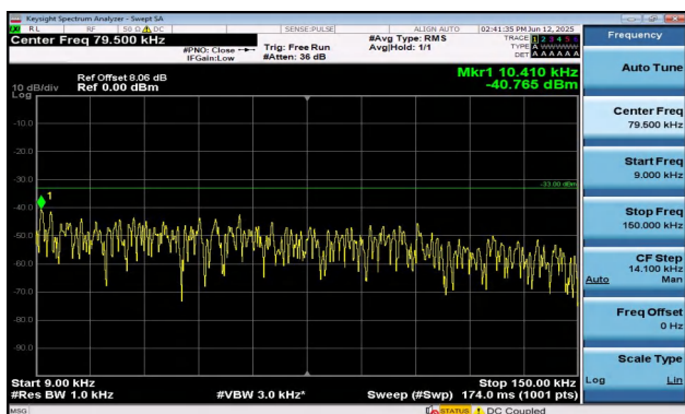
Band5-3MHz-16QAM-20635-1RB#14-0.009~0.15-PASS
