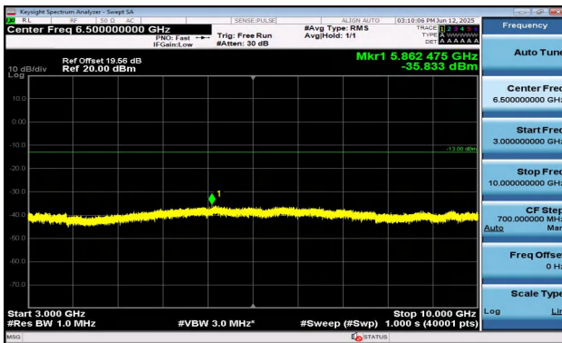
Band5-5MHz-QPSK-20525-1RB#0-3000~10000-PASS
