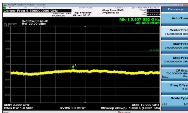
Band5-5MHz-16QAM-20525-1RB#0-3000~10000-PASS
