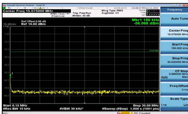
Band5-5MHz-16QAM-20425-25RB#0-0.15~30-PASS
