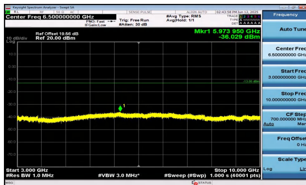
Band5-3MHz-16QAM-20635-15RB#0-3000~10000-PASS
