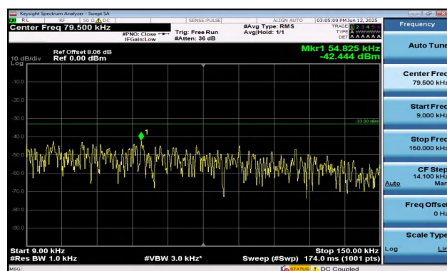
Band5-5MHz-16QAM-20425-1RB#0-0.009~0.15-PASS
