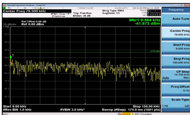
Band5-5MHz-16QAM-20525-1RB#24-0.009~0.15-PASS
