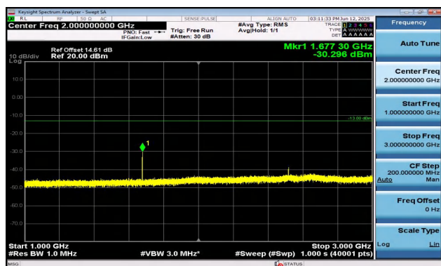
Band5-5MHz-QPSK-20525-1RB#24-1000~3000-PASS
