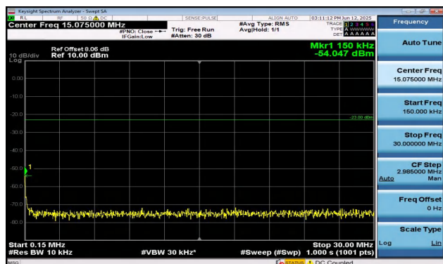
Band5-5MHz-QPSK-20525-1RB#24-0.15~30-PASS
