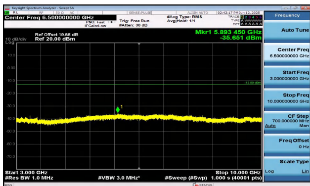
Band5-3MHz-16QAM-20635-1RB#14-3000~10000-PASS
