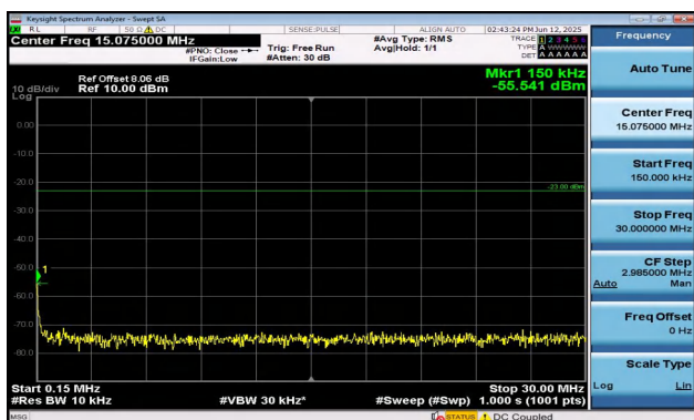
Band5-3MHz-16QAM-20635-15RB#0-0.15~30-PASS
