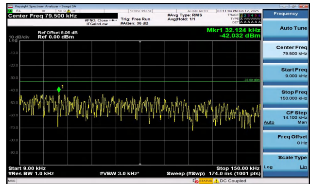
Band5-5MHz-QPSK-20525-1RB#24-0.009~0.15-PASS
