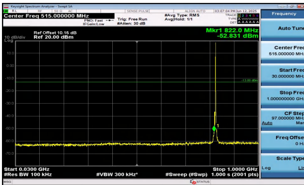
Band5-5MHz-16QAM-20425-1RB#24-30~1000-PASS
