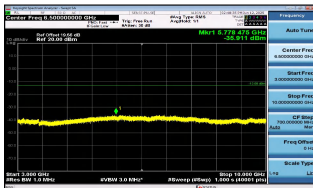
Band5-3MHz-16QAM-20635-1RB#0-3000~10000-PASS
