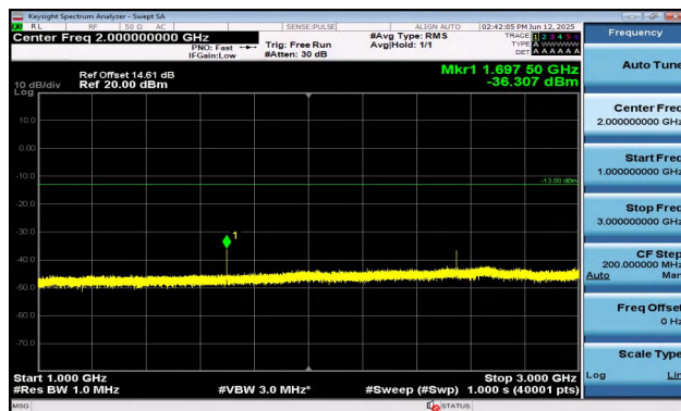
Band5-3MHz-16QAM-20635-1RB#14-1000~3000-PASS
