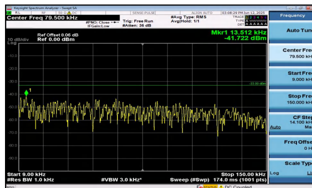
Band5-5MHz-16QAM-20425-25RB#0-0.009~0.15-PASS
