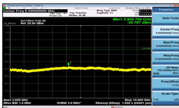
Band5-5MHz-QPSK-20425-25RB#0-3000~10000-PASS
