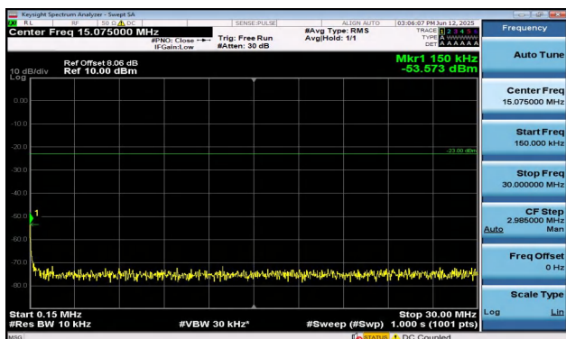
Band5-5MHz-QPSK-20425-1RB#24-0.15~30-PASS
