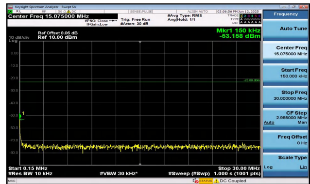
Band5-5MHz-16QAM-20425-1RB#24-0.15~30-PASS
