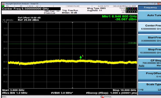
Band5-5MHz-QPSK-20525-25RB#0-3000~10000-PASS
