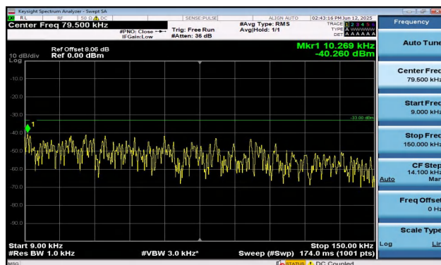
Band5-3MHz-16QAM-20635-15RB#0-0.009~0.15-PASS
