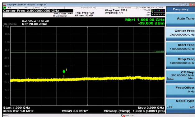
Band5-3MHz-16QAM-20635-15RB#0-1000~3000-PASS
