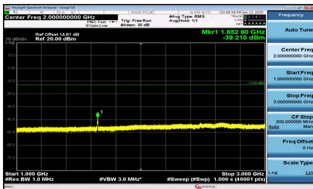
Band5-5MHz-16QAM-20425-25RB#0-1000~3000-PASS
