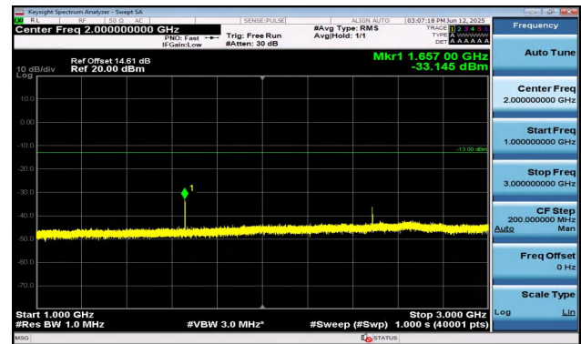
Band5-5MHz-16QAM-20425-1RB#24-1000~3000-PASS
