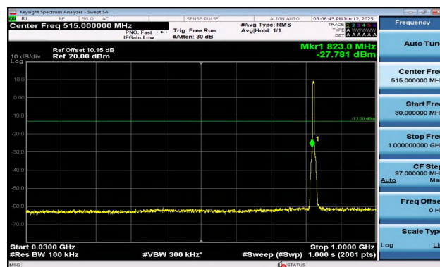
Band5-5MHz-16QAM-20425-25RB#0-30~1000-PASS
