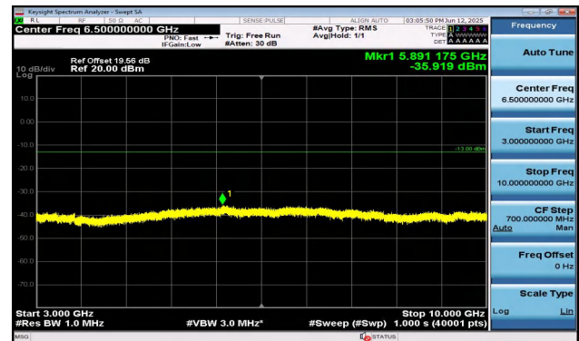
Band5-5MHz-16QAM-20425-1RB#0-3000~10000-PASS
