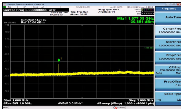
Band5-5MHz-16QAM-20525-1RB#24-1000~3000-PASS
