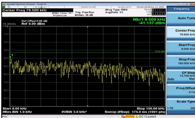
Band5-5MHz-QPSK-20425-1RB#0-0.009~0.15-PASS
