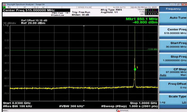
Band5-3MHz-16QAM-20635-1RB#14-30~1000-PASS
