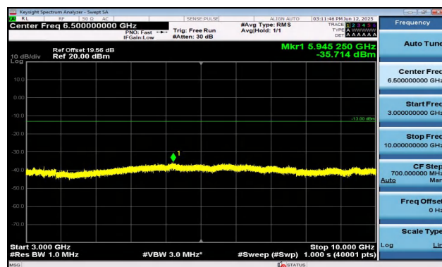
Band5-5MHz-QPSK-20525-1RB#24-3000~10000-PASS
