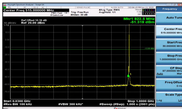
Band5-5MHz-QPSK-20425-1RB#24-30~1000-PASS
