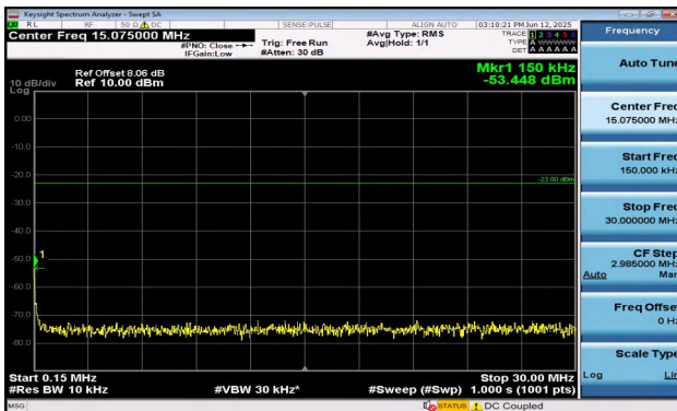
Band5-5MHz-16QAM-20525-1RB#0-0.15~30-PASS
