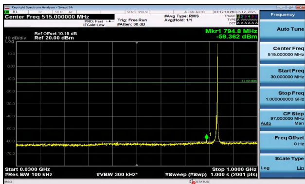
Band5-5MHz-16QAM-20525-1RB#24-30~1000-PASS
