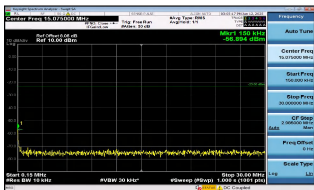
Band5-5MHz-16QAM-20425-1RB#0-0.15~30-PASS
