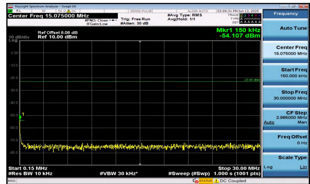
Band5-5MHz-QPSK-20525-1RB#0-0.15~30-PASS
