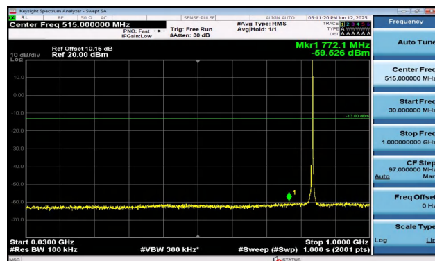
Band5-5MHz-QPSK-20525-1RB#24-30~1000-PASS
