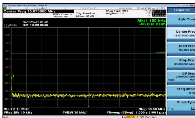
Band5-3MHz-16QAM-20635-1RB#14-0.15~30-PASS
