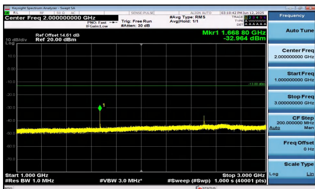
Band5-5MHz-16QAM-20525-1RB#0-1000~3000-PASS
