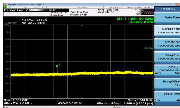
Band5-5MHz-QPSK-20425-25RB#0-1000~3000-PASS
