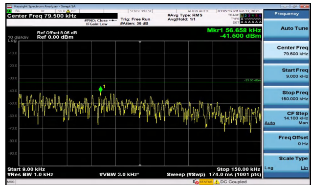
Band5-5MHz-QPSK-20425-1RB#24-0.009~0.15-PASS
