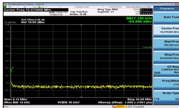
Band5-5MHz-QPSK-20525-25RB#0-0.15~30-PASS
