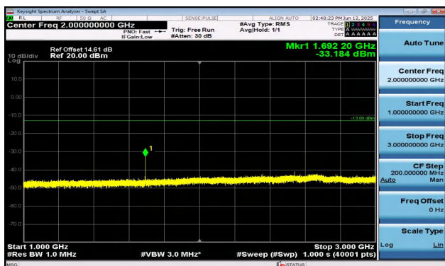
Band5-3MHz-16QAM-20635-1RB#0-1000~3000-PASS
