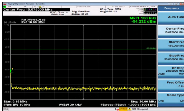
Band5-5MHz-QPSK-20425-25RB#0-0.15~30-PASS
