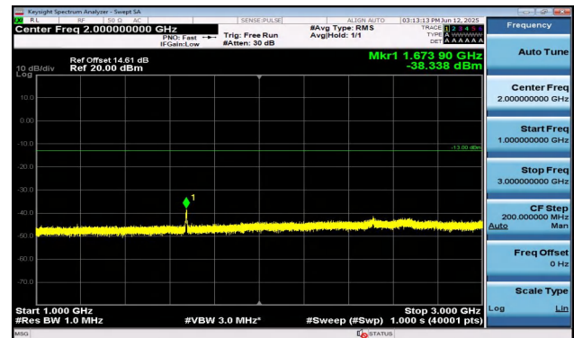
Band5-5MHz-QPSK-20525-25RB#0-1000~3000-PASS
