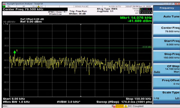
Band5-5MHz-QPSK-20425-25RB#0-0.009~0.15-PASS
