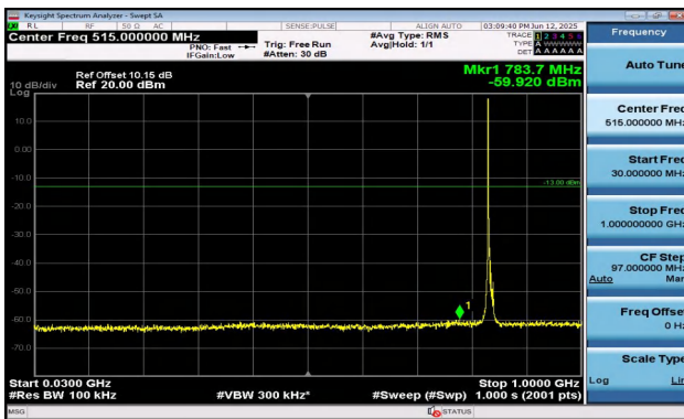
Band5-5MHz-QPSK-20525-1RB#0-30~1000-PASS
