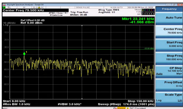
Band5-3MHz-QPSK-20525-1RB#0-0.009~0.15-PASS
