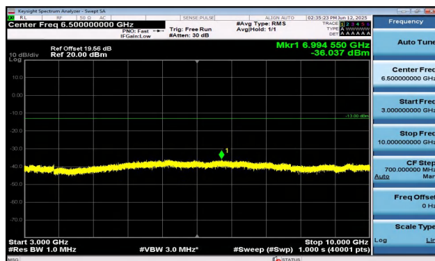
Band5-3MHz-16QAM-20525-1RB#0-3000~10000-PASS
