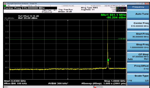
Band5-3MHz-16QAM-20635-1RB#0-30~1000-PASS
