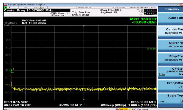
Band5-3MHz-QPSK-20635-1RB#0-0.15~30-PASS
