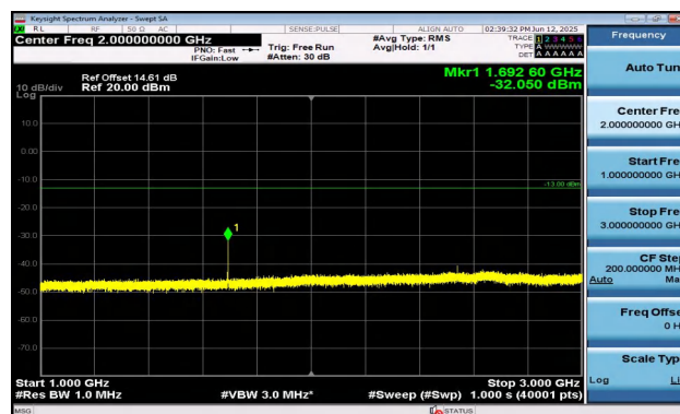
Band5-3MHz-QPSK-20635-1RB#0-1000~3000-PASS
