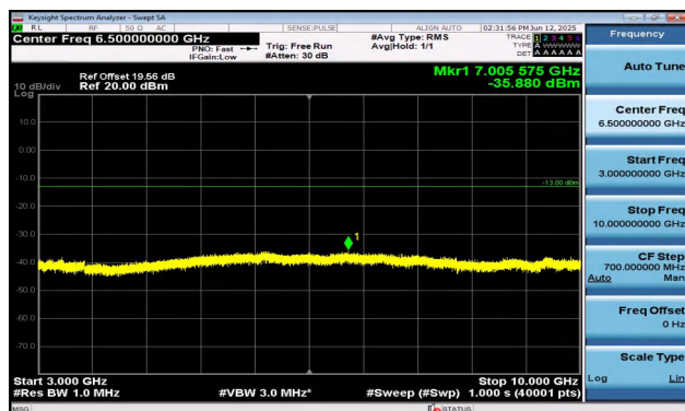
Band5-3MHz-16QAM-20415-1RB#14-3000~10000-PASS
