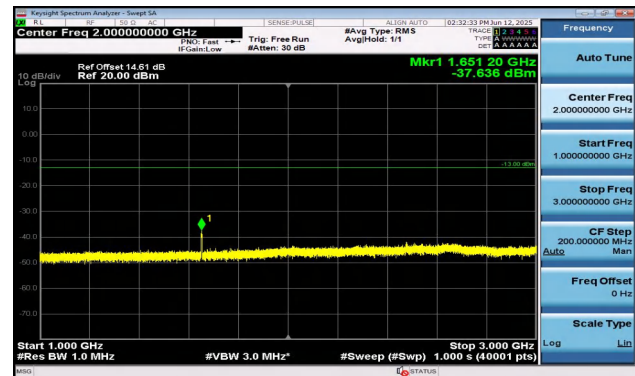
Band5-3MHz-QPSK-20415-15RB#0-1000~3000-PASS
