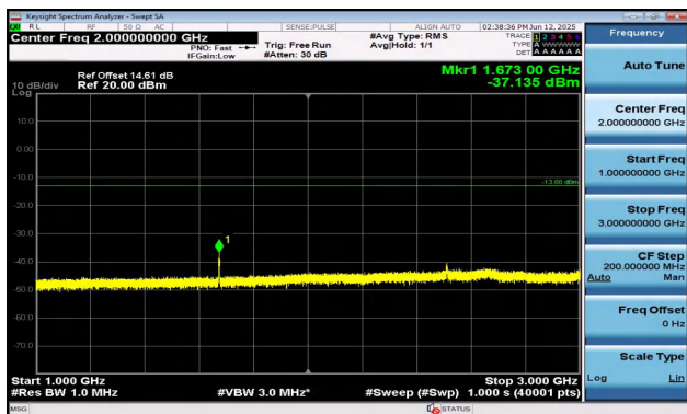
Band5-3MHz-16QAM-20525-15RB#0-1000~3000-PASS
