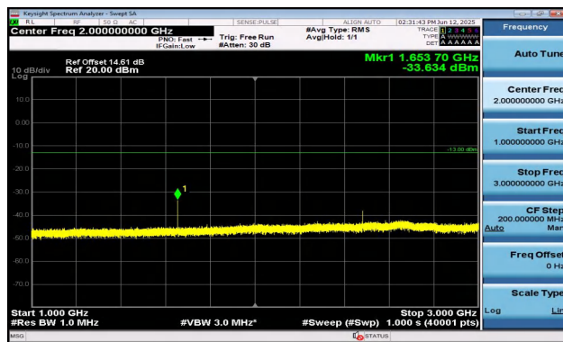
Band5-3MHz-16QAM-20415-1RB#14-1000~3000-PASS
