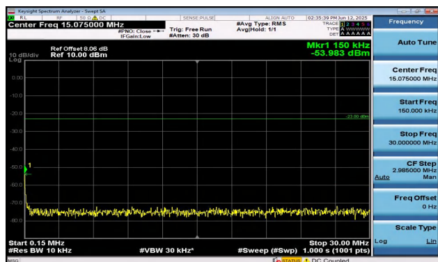
Band5-3MHz-QPSK-20525-1RB#14-0.15~30-PASS
