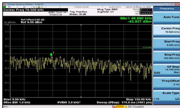
Band5-3MHz-QPSK-20525-15RB#0-0.009~0.15-PASS
