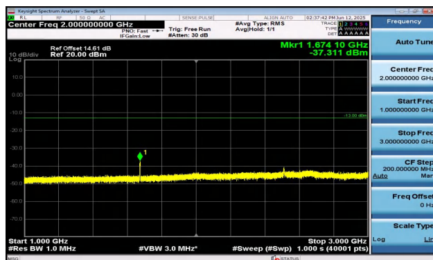
Band5-3MHz-QPSK-20525-15RB#0-1000~3000-PASS
