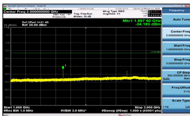
Band5-3MHz-QPSK-20635-1RB#14-1000~3000-PASS
