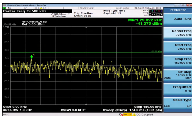
Band5-3MHz-16QAM-20525-1RB#14-0.009~0.15-PASS
