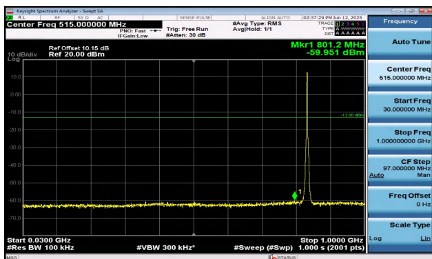
Band5-3MHz-QPSK-20525-15RB#0-30~1000-PASS
