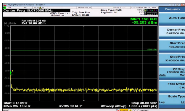
Band5-3MHz-QPSK-20525-1RB#0-0.15~30-PASS
