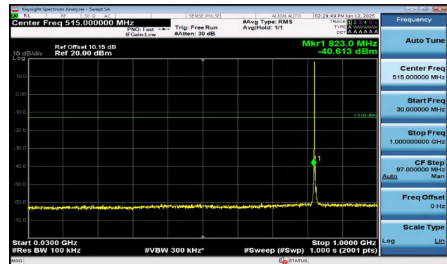
Band5-3MHz-16QAM-20415-1RB#0-30~1000-PASS
