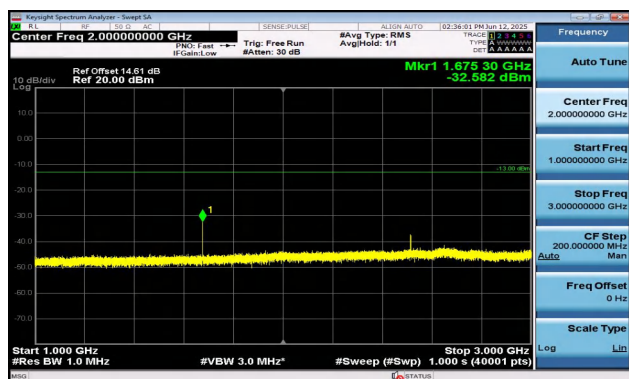
Band5-3MHz-QPSK-20525-1RB#14-1000~3000-PASS
