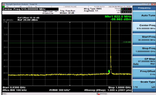
Band5-3MHz-QPSK-20525-1RB#0-30~1000-PASS
