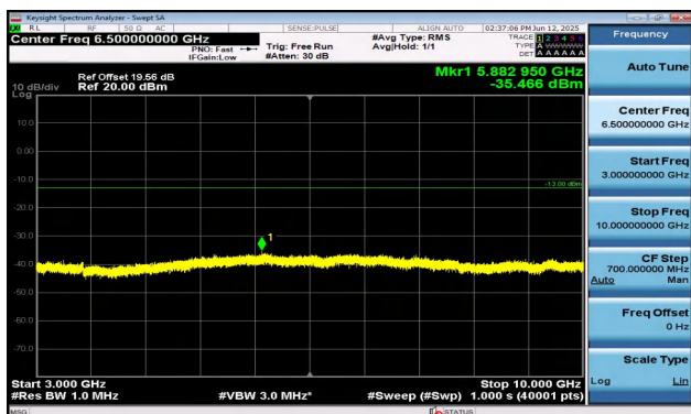
Band5-3MHz-16QAM-20525-1RB#14-3000~10000-PASS
