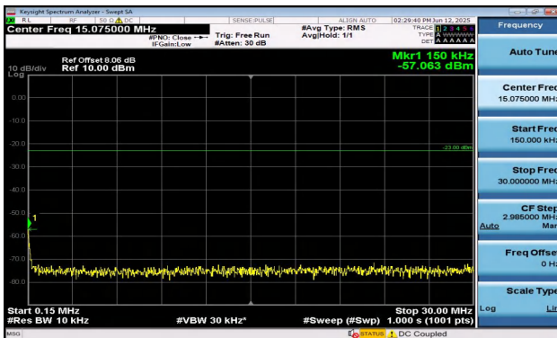
Band5-3MHz-16QAM-20415-1RB#0-0.15~30-PASS
