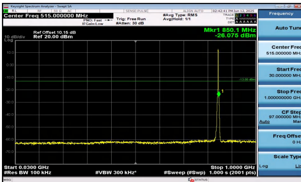
Band5-3MHz-QPSK-20635-15RB#0-30~1000-PASS
