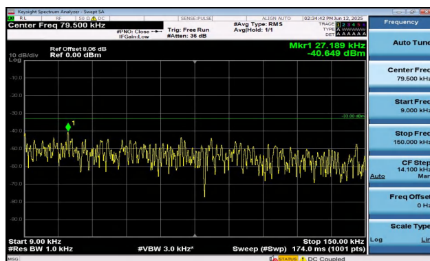
Band5-3MHz-16QAM-20525-1RB#0-0.009~0.15-PASS
