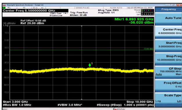
Band5-3MHz-QPSK-20525-15RB#0-3000~10000-PASS
