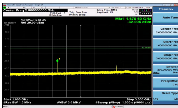
Band5-3MHz-QPSK-20525-1RB#0-1000~3000-PASS
