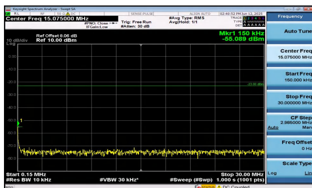
Band5-3MHz-QPSK-20635-1RB#14-0.15~30-PASS
