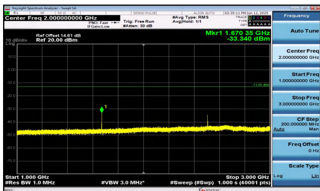
Band5-3MHz-16QAM-20525-1RB#0-1000~3000-PASS
