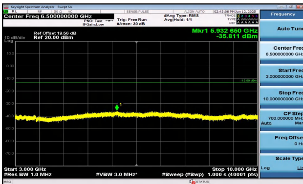
Band5-3MHz-QPSK-20635-15RB#0-3000~10000-PASS
