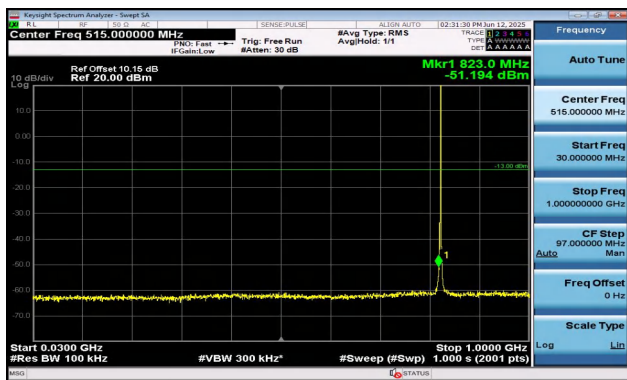
Band5-3MHz-16QAM-20415-1RB#14-30~1000-PASS
