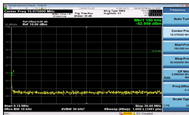
Band5-3MHz-QPSK-20635-15RB#0-0.15~30-PASS
