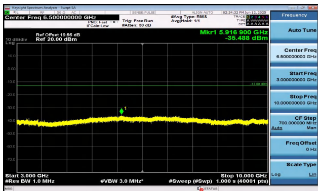
Band5-3MHz-QPSK-20525-1RB#0-3000~10000-PASS
