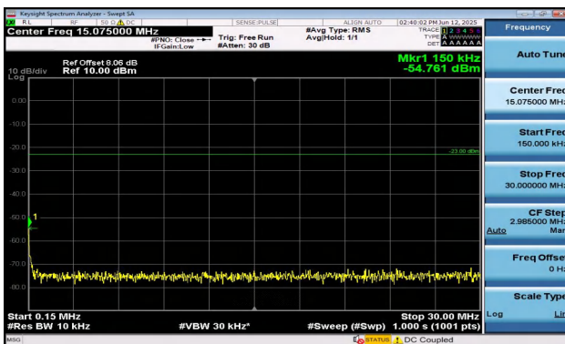
Band5-3MHz-16QAM-20635-1RB#0-0.15~30-PASS
