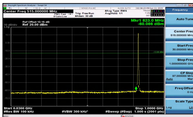
Band5-3MHz-16QAM-20525-15RB#0-30~1000-PASS
