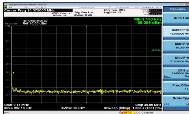
Band5-3MHz-QPSK-20525-15RB#0-0.15~30-PASS
