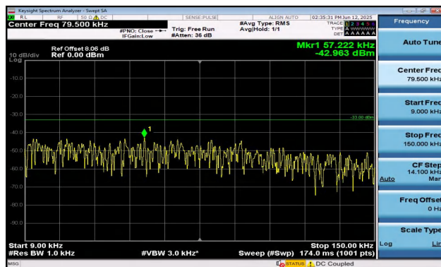
Band5-3MHz-QPSK-20525-1RB#14-0.009~0.15-PASS
