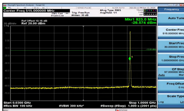
Band5-3MHz-16QAM-20415-15RB#0-30~1000-PASS
