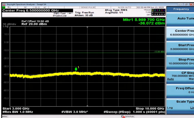
Band5-3MHz-QPSK-20415-15RB#0-3000~10000-PASS
