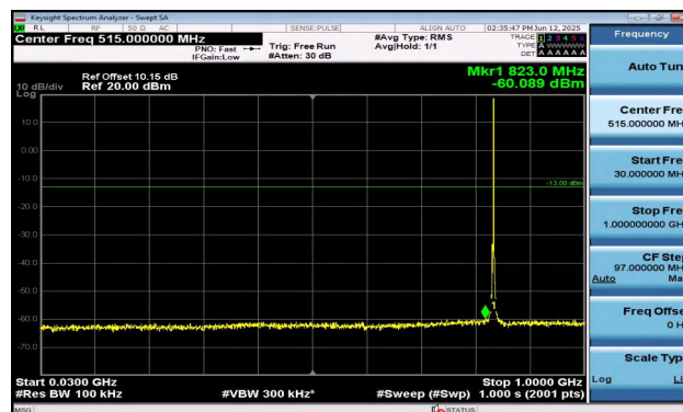
Band5-3MHz-QPSK-20525-1RB#14-30~1000-PASS
