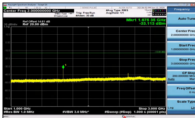
Band5-3MHz-16QAM-20525-1RB#14-1000~3000-PASS
