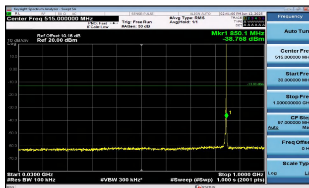
Band5-3MHz-QPSK-20635-1RB#14-30~1000-PASS
