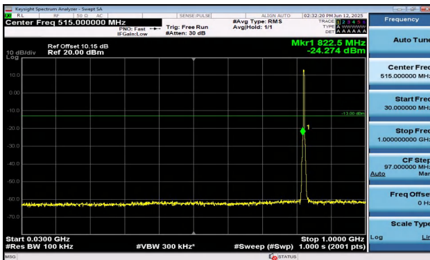
Band5-3MHz-QPSK-20415-15RB#0-30~1000-PASS
