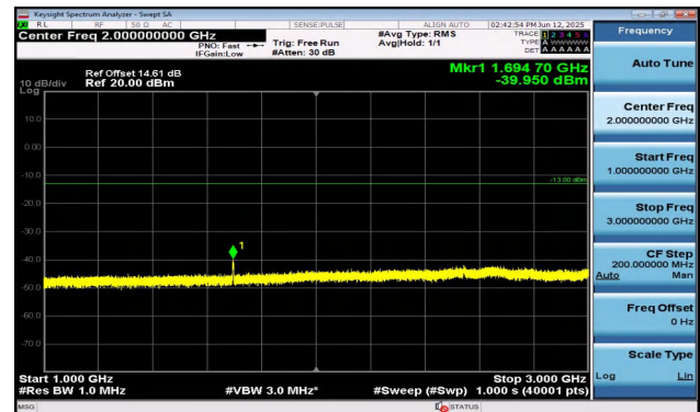
Band5-3MHz-QPSK-20635-15RB#0-1000~3000-PASS
