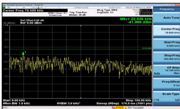
Band5-3MHz-16QAM-20415-1RB#14-0.009~0.15-PASS
