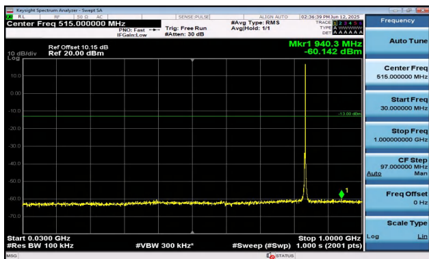
Band5-3MHz-16QAM-20525-1RB#14-30~1000-PASS
