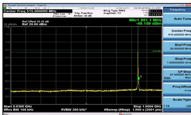
Band5-3MHz-QPSK-20635-1RB#0-30~1000-PASS
