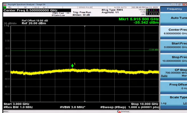
Band5-3MHz-16QAM-20525-15RB#0-3000~10000-PASS
