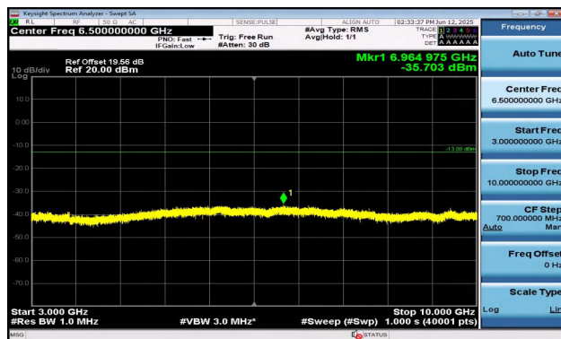
Band5-3MHz-16QAM-20415-15RB#0-3000~10000-PASS
