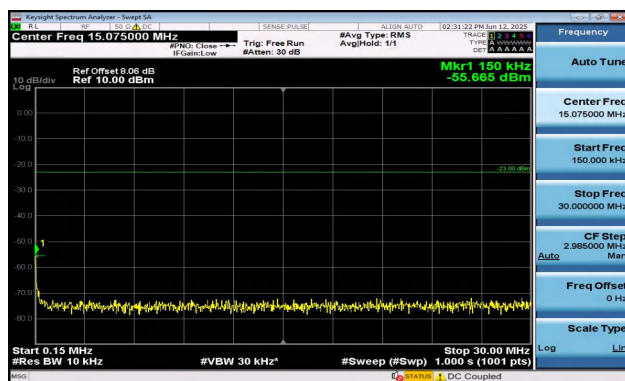
Band5-3MHz-16QAM-20415-1RB#14-0.15~30-PASS
