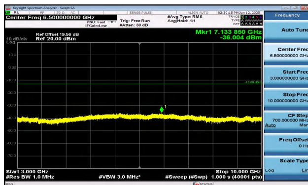
Band5-3MHz-16QAM-20415-1RB#0-3000~10000-PASS
