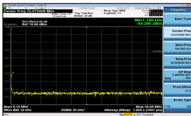
Band5-3MHz-16QAM-20525-1RB#14-0.15~30-PASS
