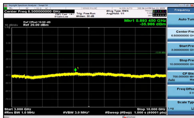
Band5-3MHz-QPSK-20525-1RB#14-3000~10000-PASS
