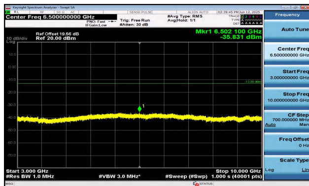
Band5-3MHz-QPSK-20635-1RB#0-3000~10000-PASS
