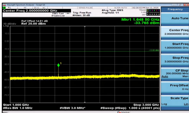
Band5-3MHz-16QAM-20415-1RB#0-1000~3000-PASS
