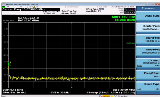
Band5-3MHz-16QAM-20525-15RB#0-0.15~30-PASS
