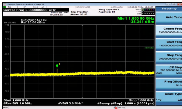
Band5-3MHz-16QAM-20415-15RB#0-1000~3000-PASS
