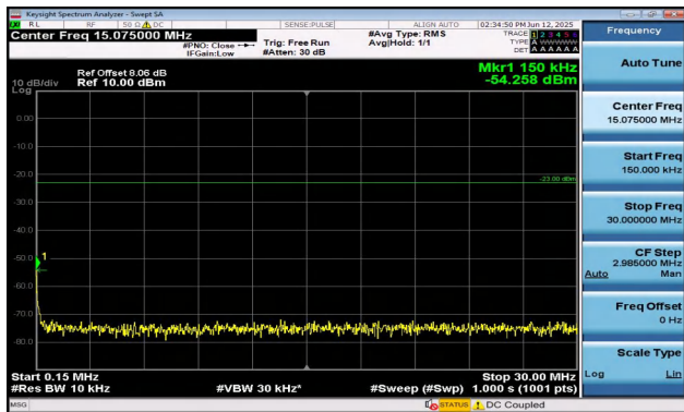
Band5-3MHz-16QAM-20525-1RB#0-0.15~30-PASS
