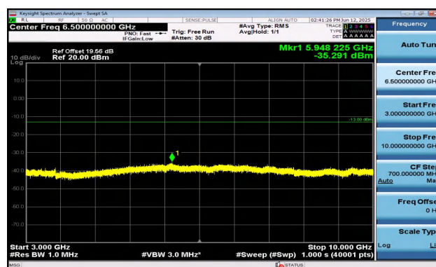
Band5-3MHz-QPSK-20635-1RB#14-3000~10000-PASS
