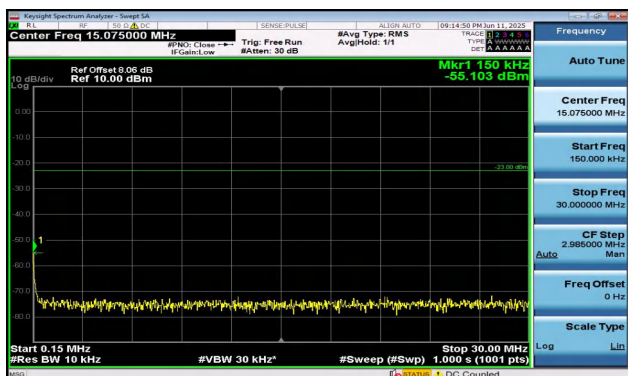
Band5-1.4MHz-QPSK-20643-1RB#5-0.15~30-PASS
