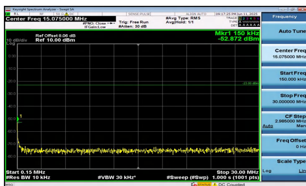
Band5-1.4MHz-16QAM-20643-6RB#0-0.15~30-PASS
