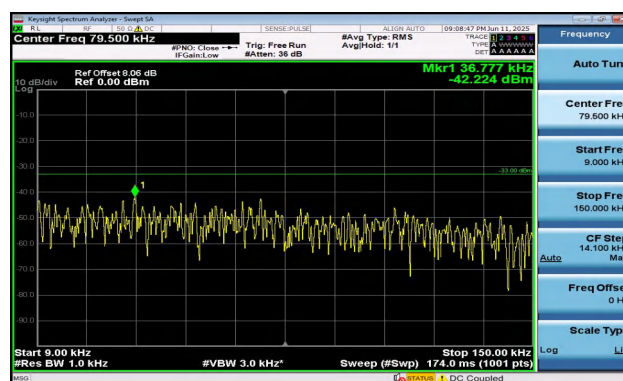
Band5-1.4MHz-16QAM-20525-1RB#0-0.009~0.15-PASS
