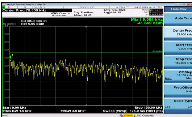
Band5-1.4MHz-16QAM-20525-1RB#5-0.009~0.15-PASS
