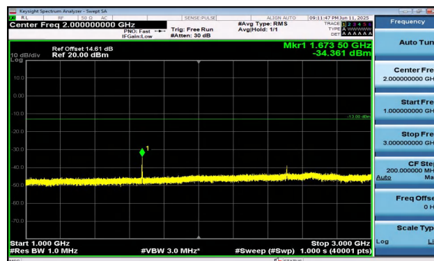
Band5-1.4MHz-QPSK-20525-6RB#0-1000~3000-PASS
