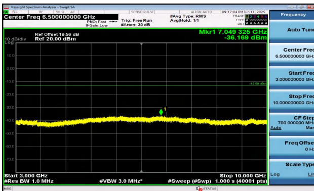
Band5-1.4MHz-QPSK-20643-6RB#0-3000~10000-PASS
