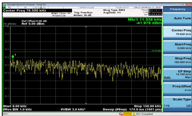
Band5-1.4MHz-QPSK-20525-6RB#0-0.009~0.15-PASS
