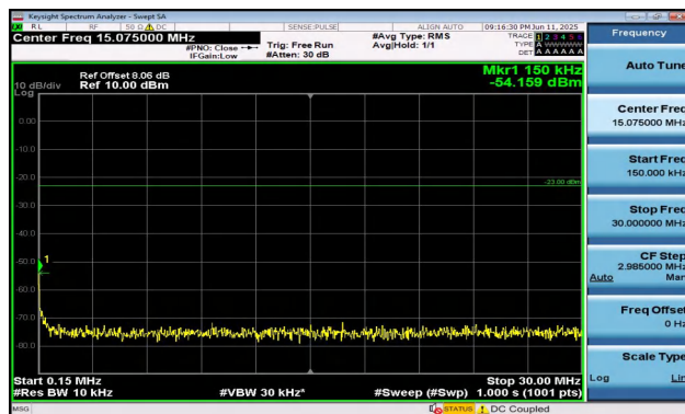
Band5-1.4MHz-QPSK-20643-6RB#0-0.15~30-PASS
