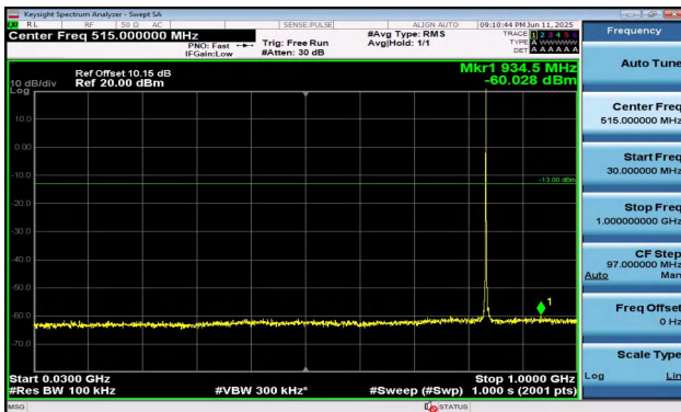
Band5-1.4MHz-16QAM-20525-1RB#5-30~1000-PASS
