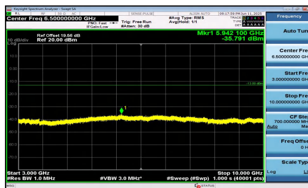
Band5-1.4MHz-16QAM-20643-6RB#0-3000~10000-PASS
