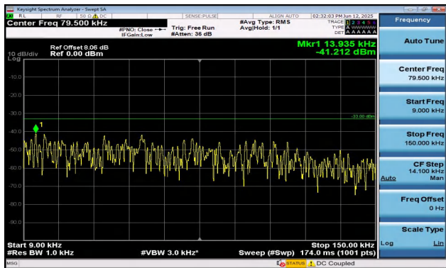
Band5-3MHz-QPSK-20415-15RB#0-0.009~0.15-PASS
