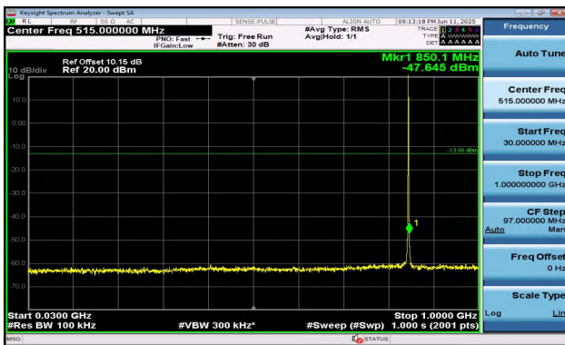
Band5-1.4MHz-QPSK-20643-1RB#0-30~1000-PASS
