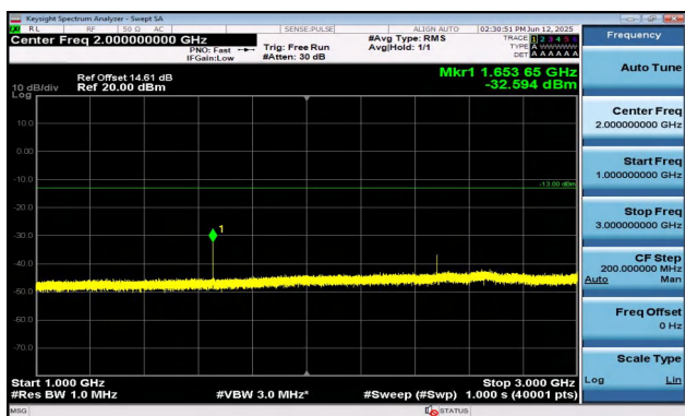
Band5-3MHz-QPSK-20415-1RB#14-1000~3000-PASS
