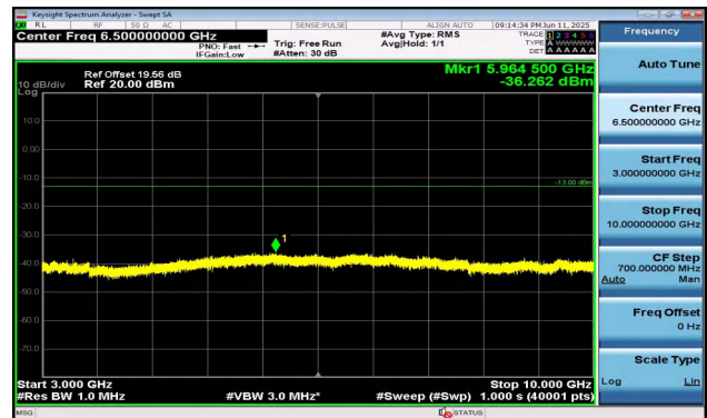
Band5-1.4MHz-16QAM-20643-1RB#0-3000~10000-PASS
