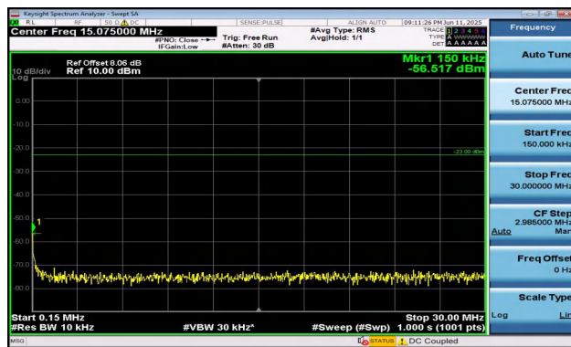
Band5-1.4MHz-QPSK-20525-6RB#0-0.15~30-PASS
