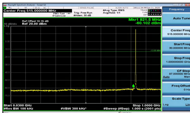
Band5-1.4MHz-QPSK-20525-6RB#0-30~1000-PASS
