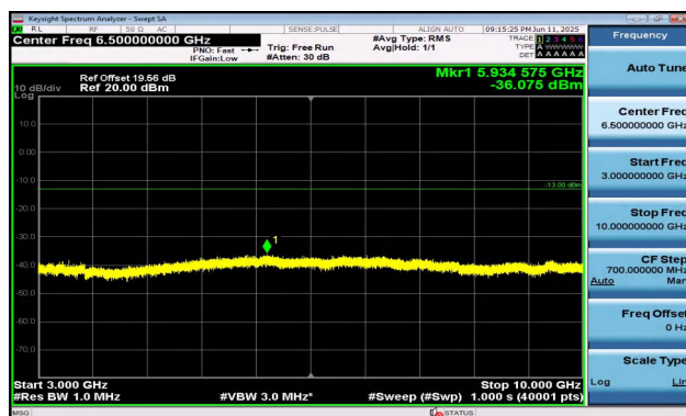
Band5-1.4MHz-QPSK-20643-1RB#5-3000~10000-PASS
