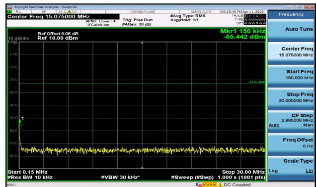
Band5-1.4MHz-16QAM-20643-1RB#5-0.15~30-PASS
