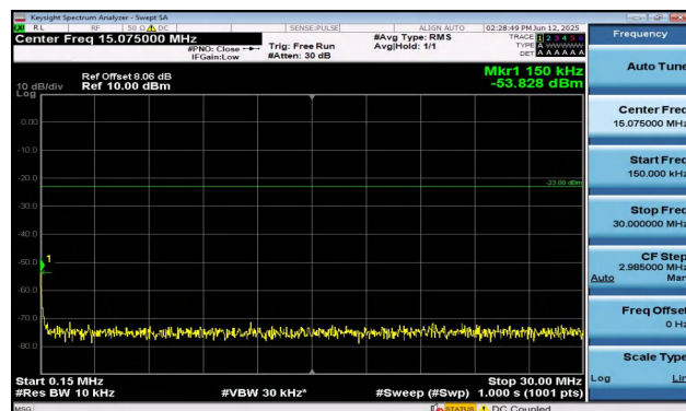
Band5-3MHz-QPSK-20415-1RB#0-0.15~30-PASS
