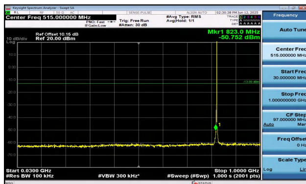
Band5-3MHz-QPSK-20415-1RB#14-30~1000-PASS
