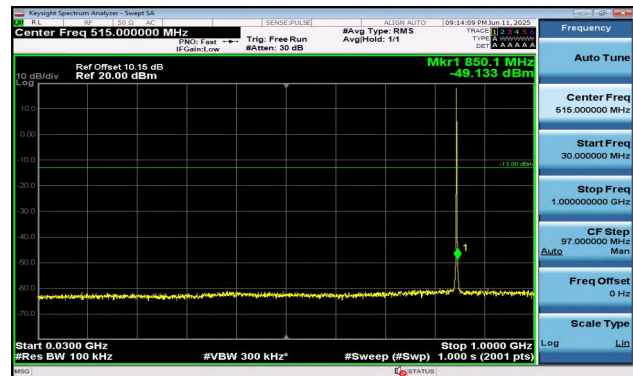
Band5-1.4MHz-16QAM-20643-1RB#0-30~1000-PASS
