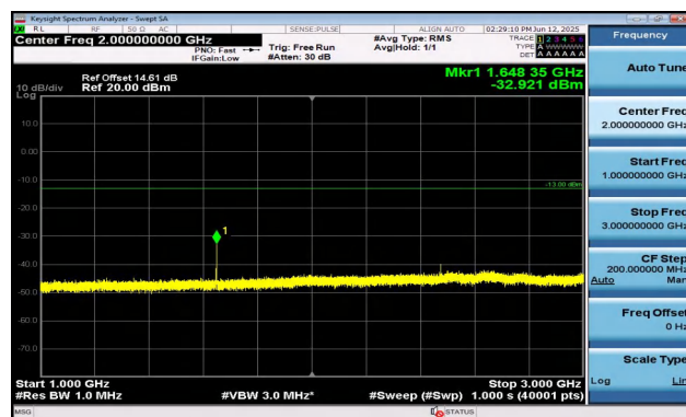
Band5-3MHz-QPSK-20415-1RB#0-1000~3000-PASS
