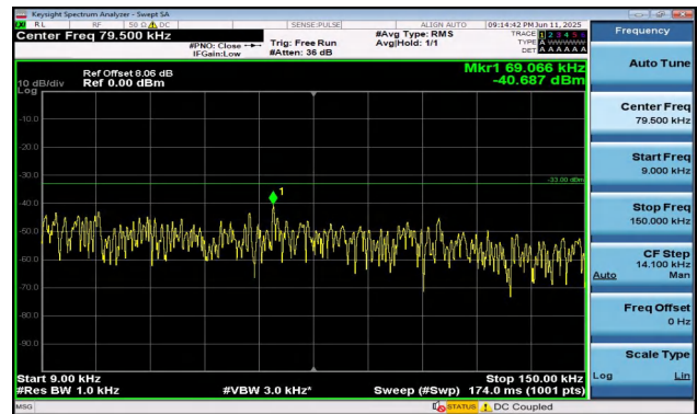
Band5-1.4MHz-QPSK-20643-1RB#5-0.009~0.15-PASS
