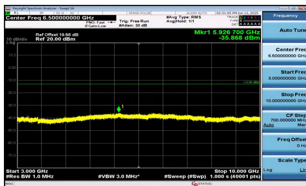
Band5-3MHz-QPSK-20415-1RB#14-3000~10000-PASS
