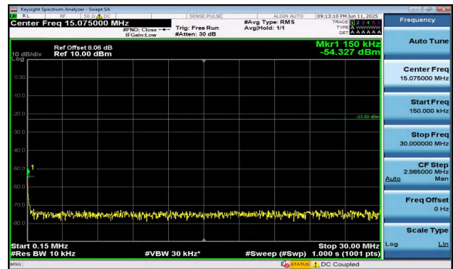
Band5-1.4MHz-QPSK-20643-1RB#0-0.15~30-PASS
