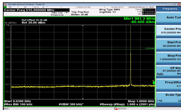
Band5-1.4MHz-16QAM-20525-1RB#0-30~1000-PASS
