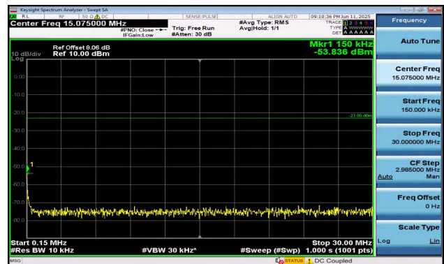
Band5-1.4MHz-16QAM-20525-1RB#5-0.15~30-PASS
