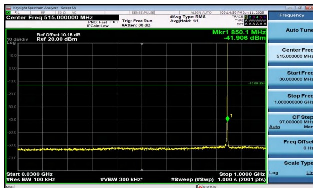
Band5-1.4MHz-QPSK-20643-1RB#5-30~1000-PASS
