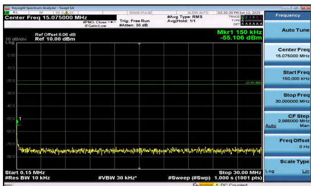
Band5-3MHz-QPSK-20415-1RB#14-0.15~30-PASS
