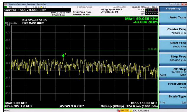
Band5-1.4MHz-16QAM-20643-1RB#0-0.009~0.15-PASS
