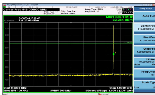
Band5-1.4MHz-16QAM-20643-6RB#0-30~1000-PASS
