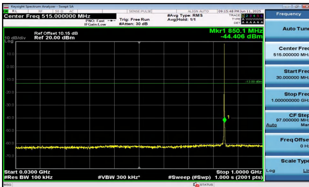
Band5-1.4MHz-16QAM-20643-1RB#5-30~1000-PASS
