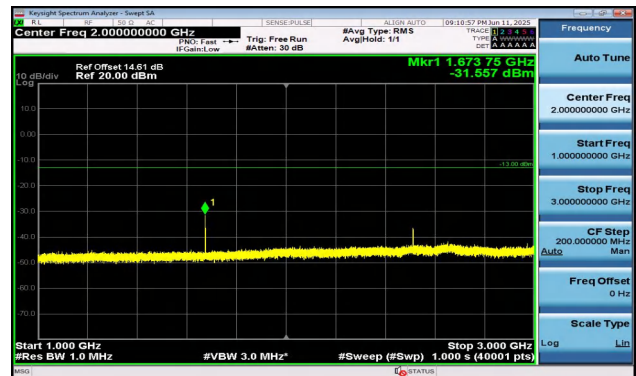
Band5-1.4MHz-16QAM-20525-1RB#5-1000~3000-PASS
