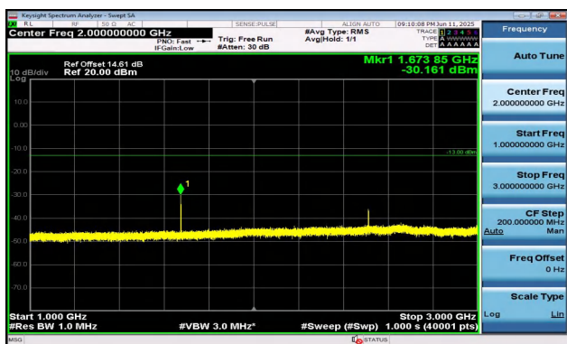
Band5-1.4MHz-QPSK-20525-1RB#5-1000~3000-PASS
