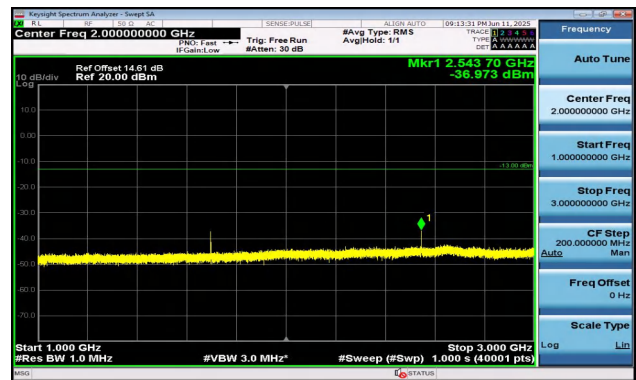
Band5-1.4MHz-QPSK-20643-1RB#0-1000~3000-PASS
