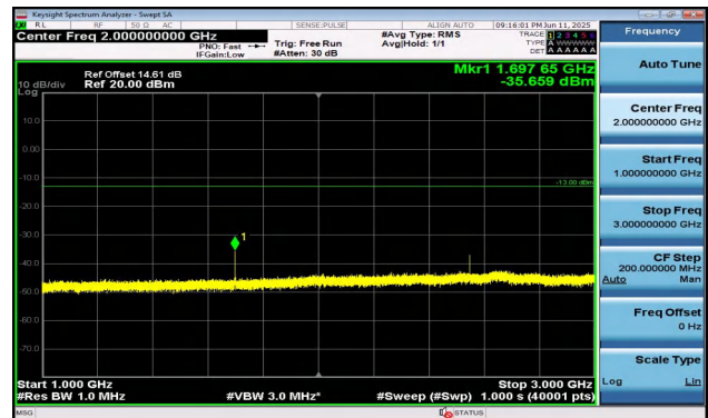
Band5-1.4MHz-16QAM-20643-1RB#5-1000~3000-PASS
