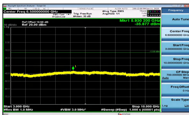
Band5-1.4MHz-QPSK-20525-6RB#0-3000~10000-PASS
