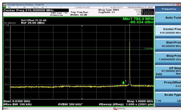
Band5-1.4MHz-QPSK-20525-1RB#5-30~1000-PASS
