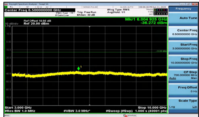
Band5-1.4MHz-16QAM-20525-1RB#0-3000~10000-PASS
