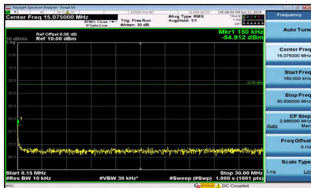
Band5-1.4MHz-16QAM-20525-1RB#0-0.15~30-PASS
