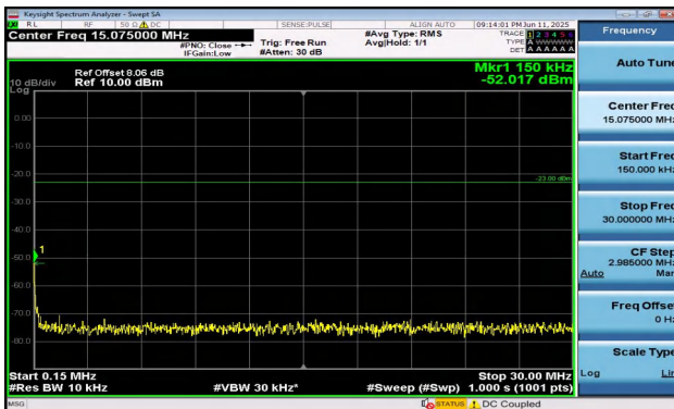
Band5-1.4MHz-16QAM-20643-1RB#0-0.15~30-PASS
