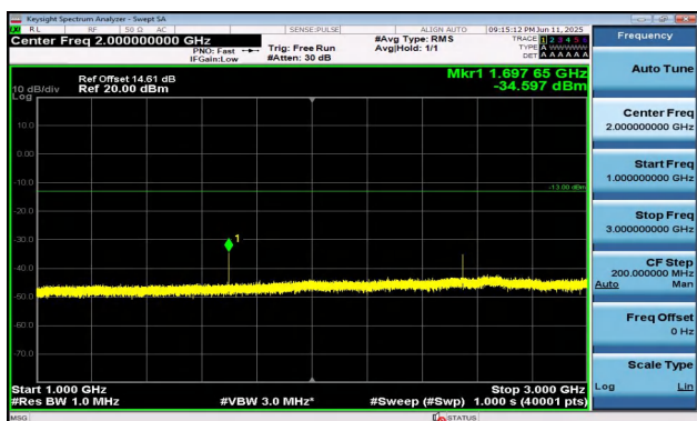
Band5-1.4MHz-QPSK-20643-1RB#5-1000~3000-PASS
