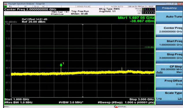
Band5-1.4MHz-QPSK-20643-6RB#0-1000~3000-PASS
