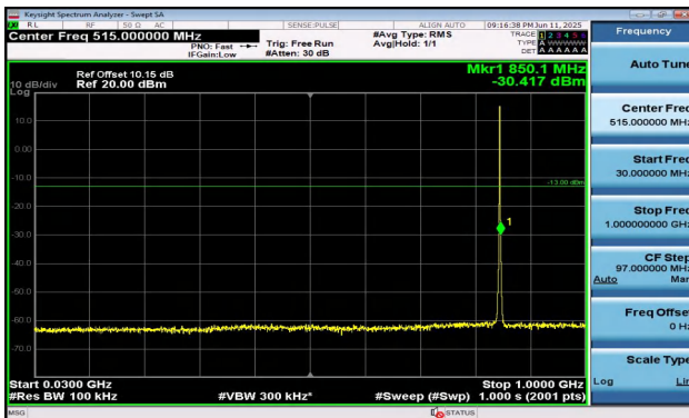
Band5-1.4MHz-QPSK-20643-6RB#0-30~1000-PASS
