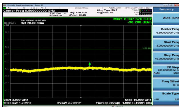
Band5-1.4MHz-16QAM-20643-1RB#5-3000~10000-PASS
