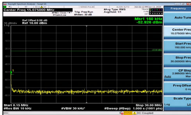
Band5-3MHz-QPSK-20415-15RB#0-0.15~30-PASS
