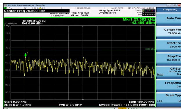
Band5-1.4MHz-16QAM-20643-6RB#0-0.009~0.15-PASS
