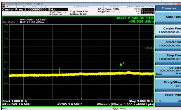
Band5-1.4MHz-16QAM-20643-1RB#0-1000~3000-PASS
