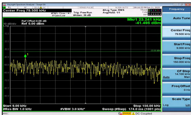
Band5-1.4MHz-QPSK-20643-6RB#0-0.009~0.15-PASS
