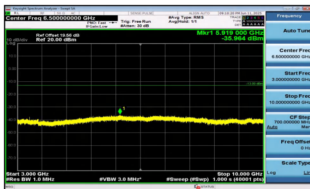
Band5-1.4MHz-QPSK-20525-1RB#5-3000~10000-PASS
