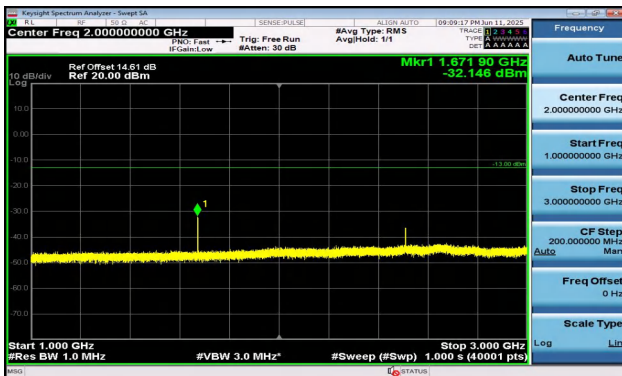
Band5-1.4MHz-16QAM-20525-1RB#0-1000~3000-PASS
