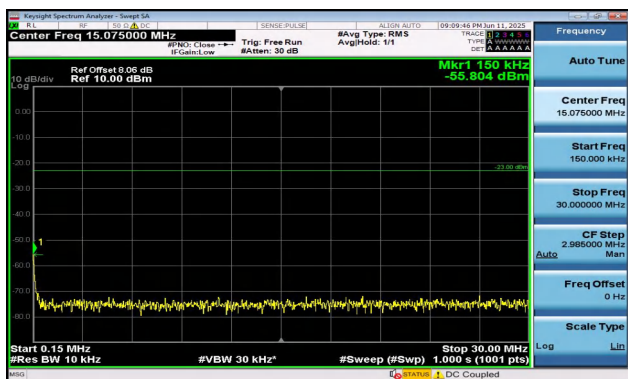
Band5-1.4MHz-QPSK-20525-1RB#5-0.15~30-PASS
