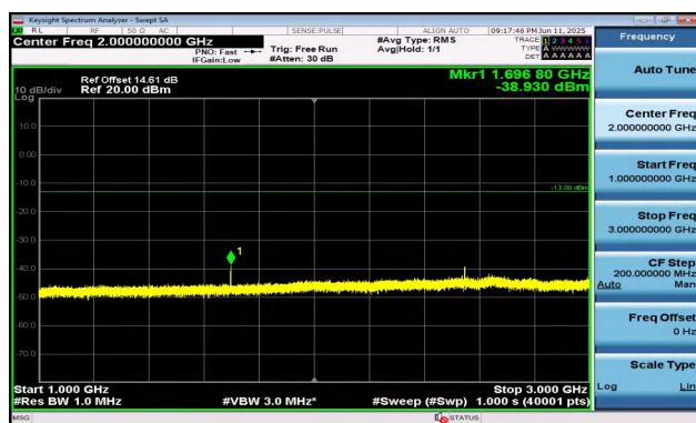
Band5-1.4MHz-16QAM-20643-6RB#0-1000~3000-PASS
