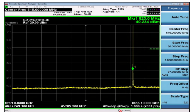
Band5-1.4MHz-16QAM-20407-1RB#0-30~1000-PASS
