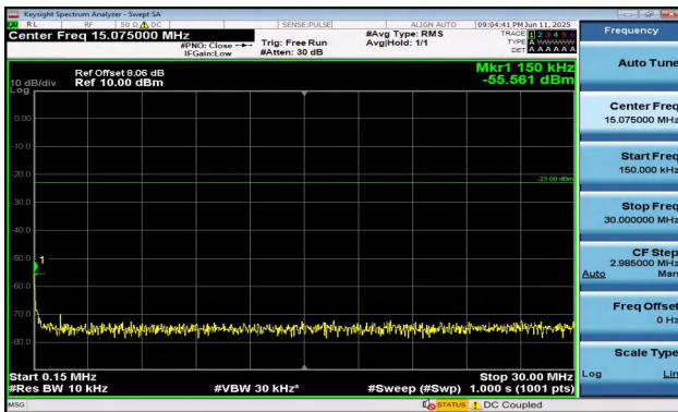
Band5-1.4MHz-QPSK-20407-1RB#5-0.15~30-PASS
