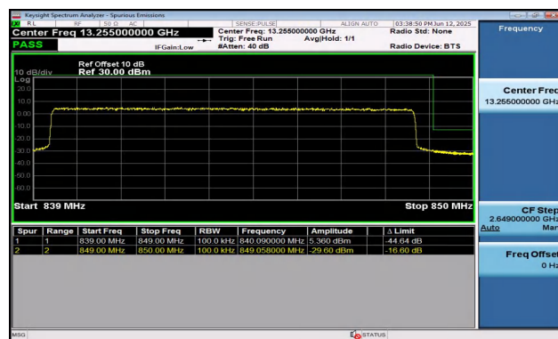
Band5-10MHz-QPSK-20600-50RB#0-PASS
