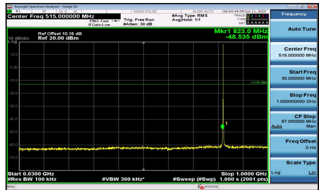
Band5-1.4MHz-QPSK-20407-1RB#5-30~1000-PASS
