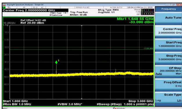
Band5-1.4MHz-16QAM-20407-1RB#0-1000~3000-PASS
