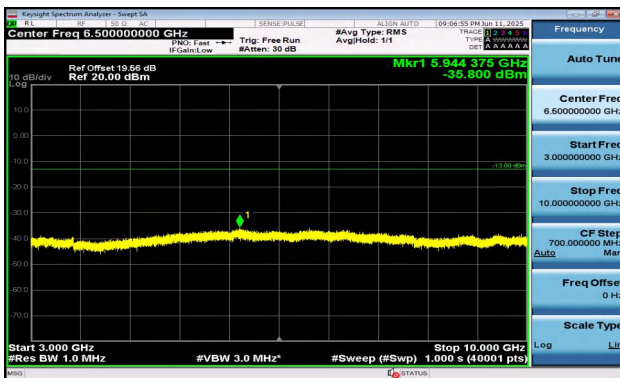
Band5-1.4MHz-QPSK-20407-6RB#0-3000~10000-PASS
