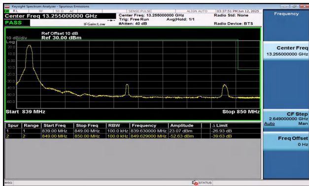
Band5-10MHz-16QAM-20600-1RB#0-PASS
