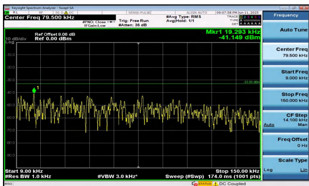
Band5-1.4MHz-QPSK-20525-1RB#0-0.009~0.15-PASS
