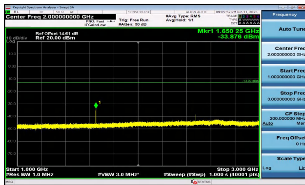
Band5-1.4MHz-16QAM-20407-1RB#5-1000~3000-PASS
