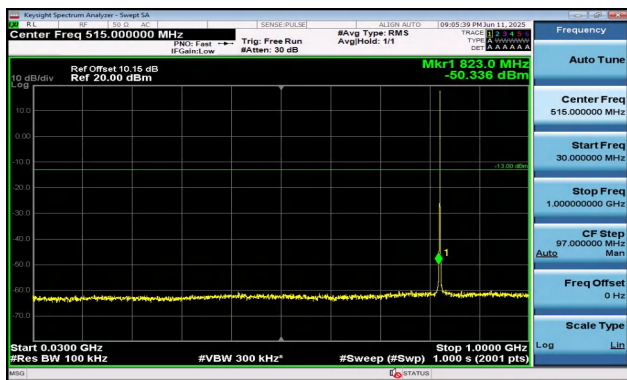
Band5-1.4MHz-16QAM-20407-1RB#5-30~1000-PASS
