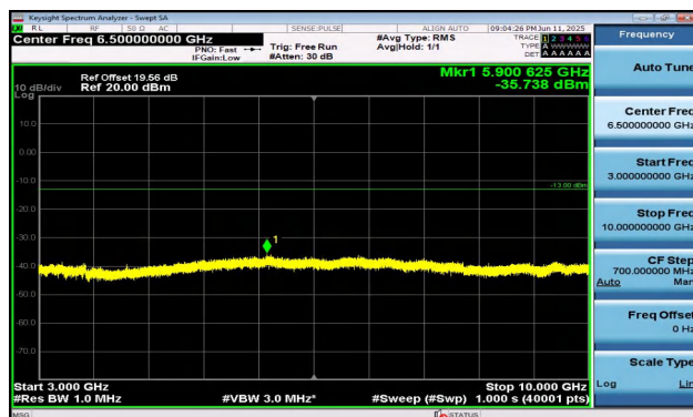
Band5-1.4MHz-16QAM-20407-1RB#0-3000~10000-PASS
