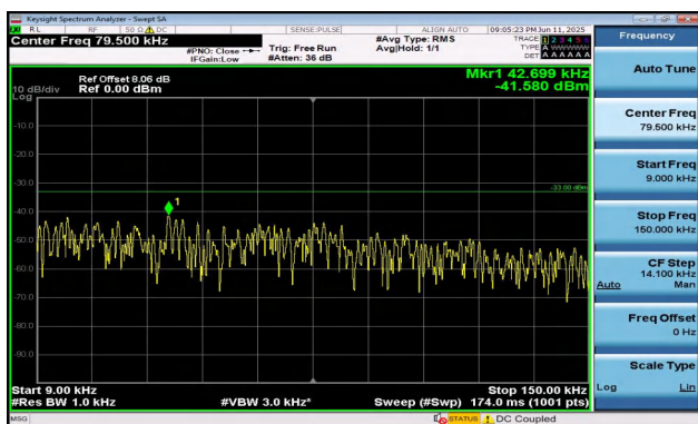
Band5-1.4MHz-16QAM-20407-1RB#5-0.009~0.15-PASS
