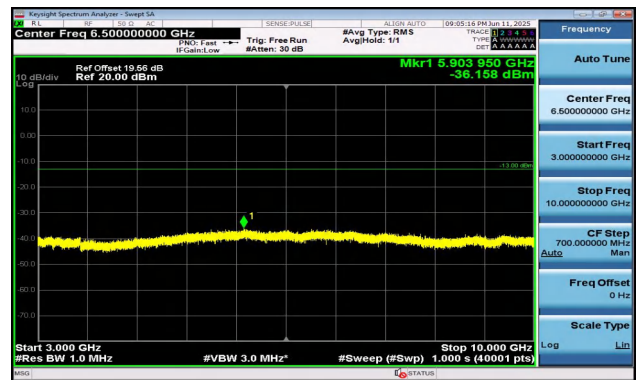
Band5-1.4MHz-QPSK-20407-1RB#5-3000~10000-PASS
