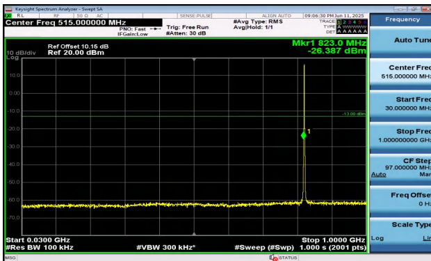
Band5-1.4MHz-QPSK-20407-6RB#0-30~1000-PASS
