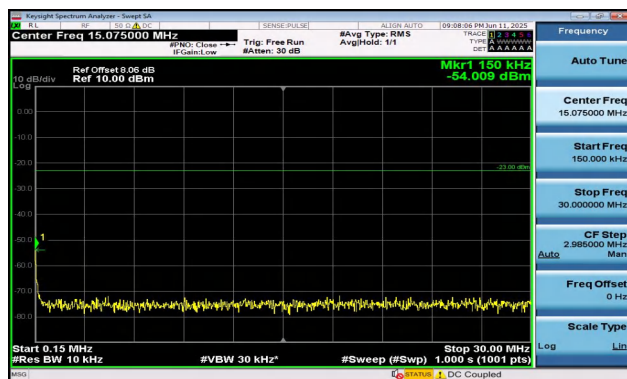
Band5-1.4MHz-QPSK-20525-1RB#0-0.15~30-PASS
