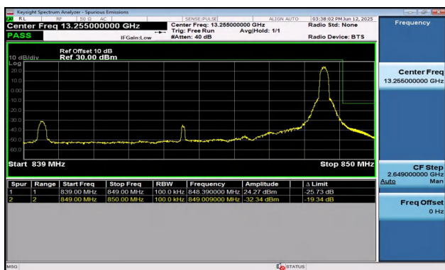
Band5-10MHz-QPSK-20600-1RB#49-PASS
