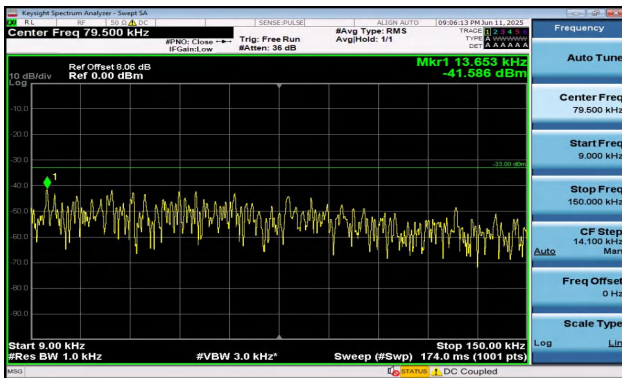
Band5-1.4MHz-QPSK-20407-6RB#0-0.009~0.15-PASS
