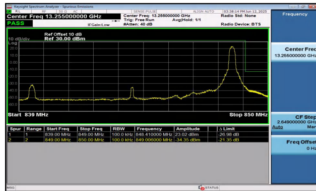
Band5-10MHz-16QAM-20600-1RB#49-PASS
