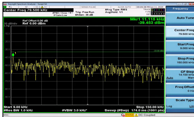
Band5-1.4MHz-QPSK-20525-1RB#5-0.009~0.15-PASS
