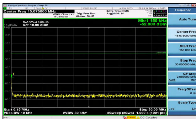
Band5-1.4MHz-16QAM-20407-1RB#5-0.15~30-PASS
