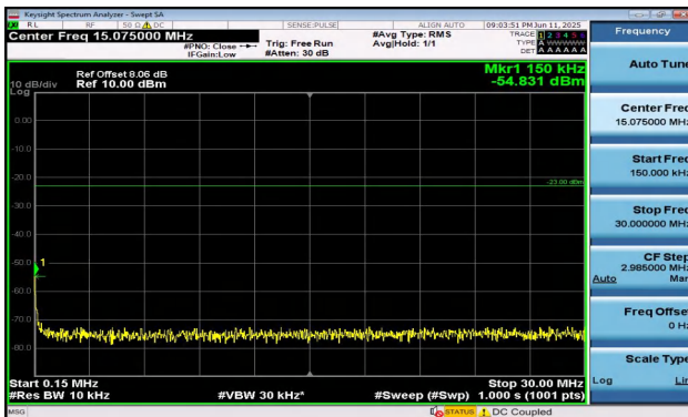
Band5-1.4MHz-16QAM-20407-1RB#0-0.15~30-PASS
