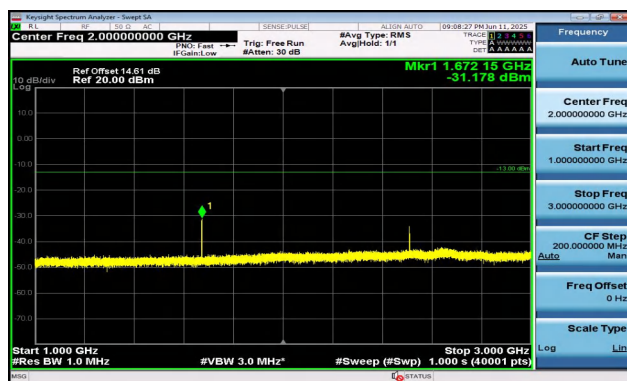
Band5-1.4MHz-QPSK-20525-1RB#0-1000~3000-PASS
