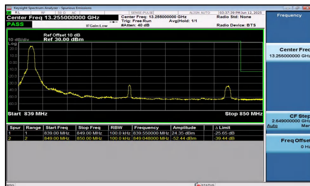
Band5-10MHz-QPSK-20600-1RB#0-PASS
