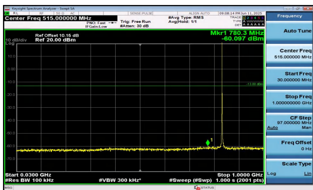
Band5-1.4MHz-QPSK-20525-1RB#0-30~1000-PASS
