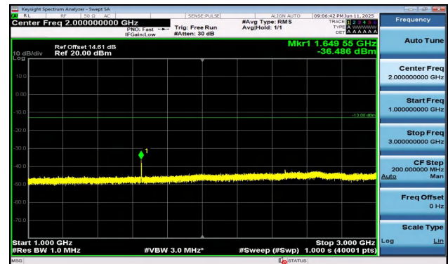
Band5-1.4MHz-QPSK-20407-6RB#0-1000~3000-PASS
