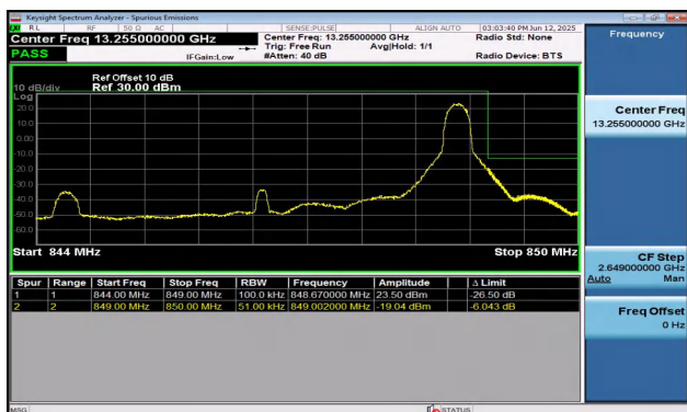
Band5-5MHz-16QAM-20625-1RB#24-PASS
