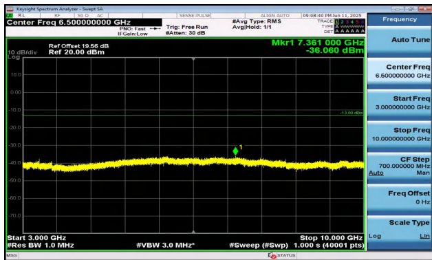
Band5-1.4MHz-QPSK-20525-1RB#0-3000~10000-PASS
