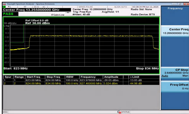
Band5-10MHz-QPSK-20450-50RB#0-PASS
