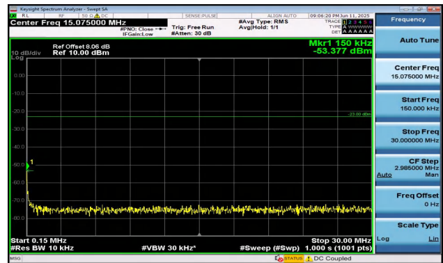
Band5-1.4MHz-QPSK-20407-6RB#0-0.15~30-PASS
