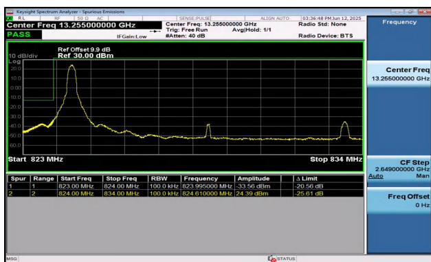
Band5-10MHz-QPSK-20450-1RB#0-PASS
