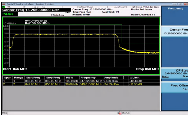
Band5-3MHz-QPSK-20635-15RB#0-PASS
