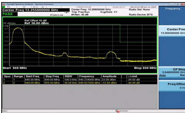
Band5-3MHz-QPSK-20635-1RB#0-PASS
