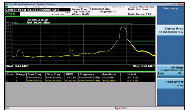
Band5-5MHz-QPSK-20625-1RB#24-PASS
