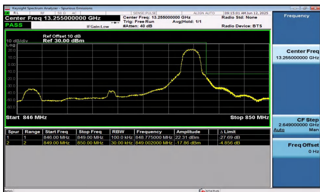
Band5-3MHz-16QAM-20635-1RB#14-PASS
