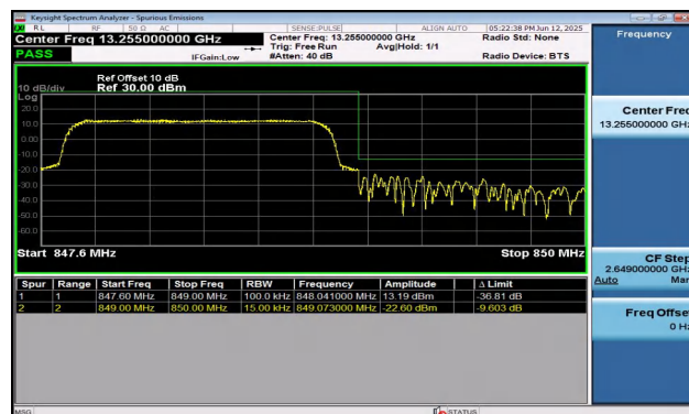
Band5-1.4MHz-16QAM-20643-6RB#0-PASS
