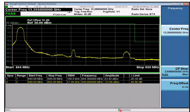
Band5-5MHz-16QAM-20625-1RB#0-PASS
