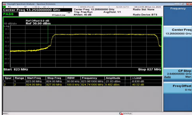
Band5-3MHz-QPSK-20415-15RB#0-PASS
