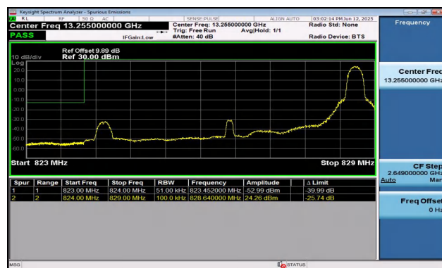
Band5-5MHz-QPSK-20425-1RB#24-PASS
