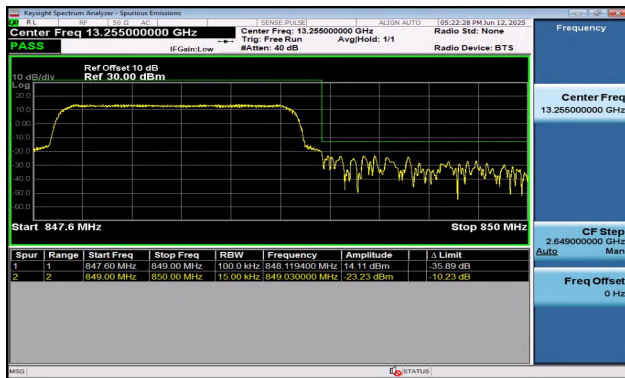
Band5-1.4MHz-QPSK-20643-6RB#0-PASS
