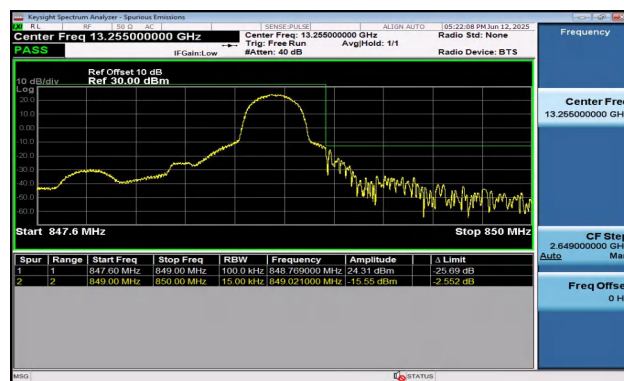
Band5-1.4MHz-QPSK-20643-1RB#5-PASS
