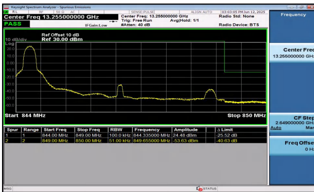
Band5-5MHz-QPSK-20625-1RB#0-PASS
