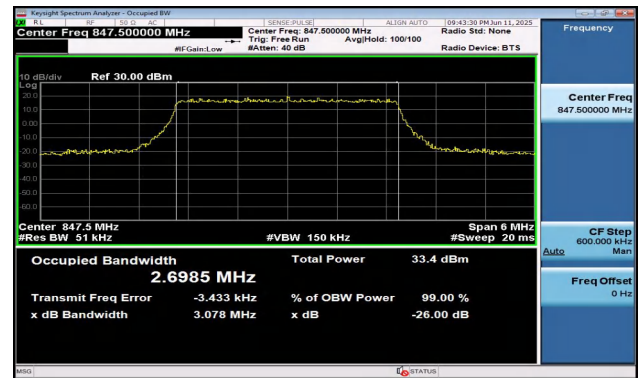
Band5-3MHz-16QAM-20635-15RB#0-PASS
