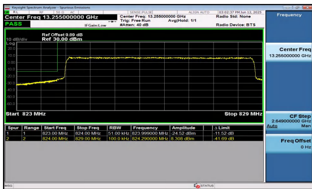
Band5-5MHz-QPSK-20425-25RB#0-PASS
