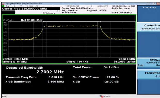
Band5-3MHz-QPSK-20525-15RB#0-PASS
