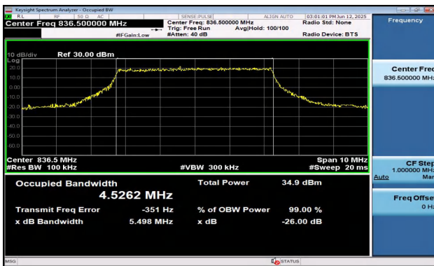
Band5-5MHz-QPSK-20525-25RB#0-PASS
