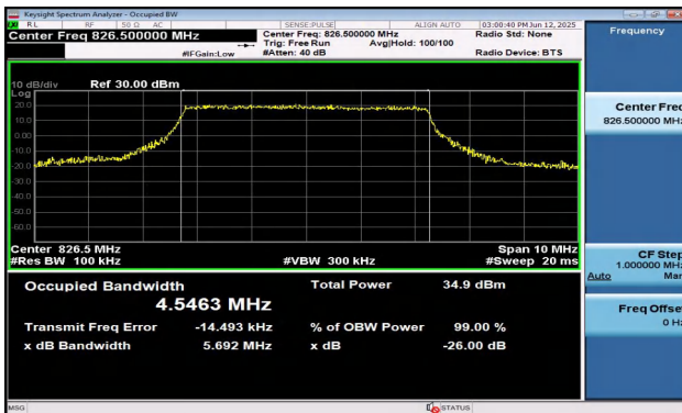
Band5-5MHz-QPSK-20425-25RB#0-PASS
