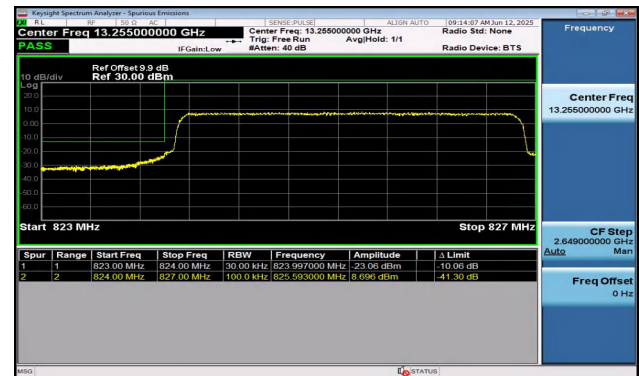
Band5-3MHz-16QAM-20415-15RB#0-PASS
