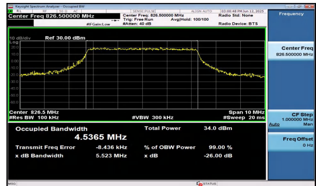
Band5-5MHz-16QAM-20425-25RB#0-PASS
