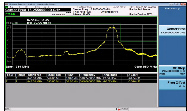
Band5-3MHz-QPSK-20635-1RB#14-PASS
