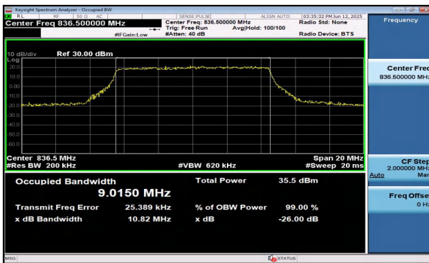
Band5-10MHz-QPSK-20525-50RB#0-PASS
