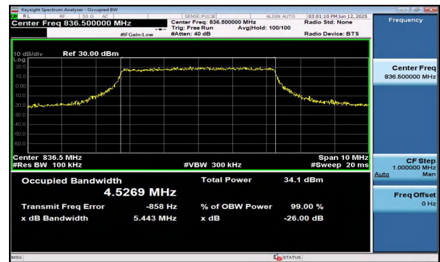
Band5-5MHz-16QAM-20525-25RB#0-PASS
