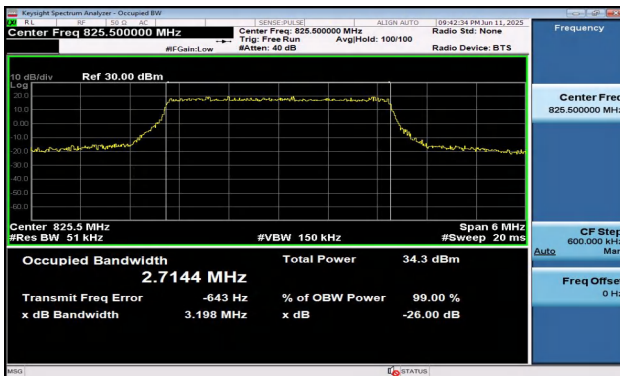
Band5-3MHz-QPSK-20415-15RB#0-PASS
