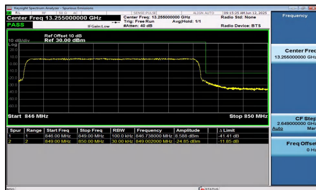
Band5-3MHz-16QAM-20635-15RB#0-PASS
