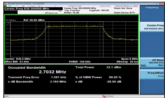
Band5-3MHz-16QAM-20525-15RB#0-PASS
