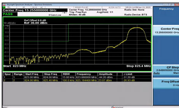
Band5-1.4MHz-16QAM-20407-1RB#5-PASS
