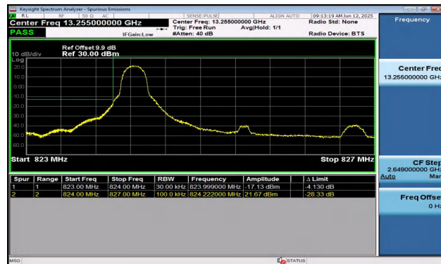
Band5-3MHz-16QAM-20415-1RB#0-PASS
