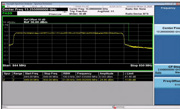
Band5-5MHz-QPSK-20625-25RB#0-PASS
