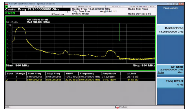
Band5-3MHz-16QAM-20635-1RB#0-PASS
