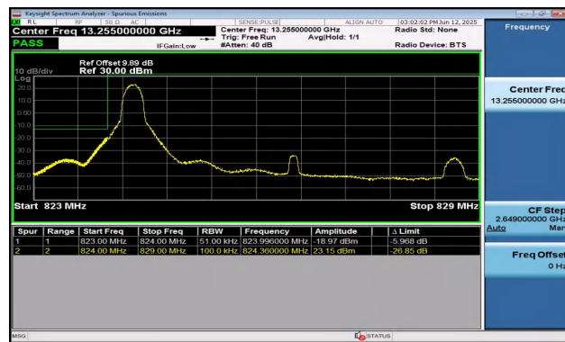
Band5-5MHz-16QAM-20425-1RB#0-PASS
