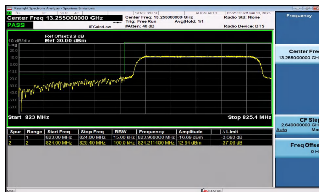
Band5-1.4MHz-16QAM-20407-6RB#0-PASS
