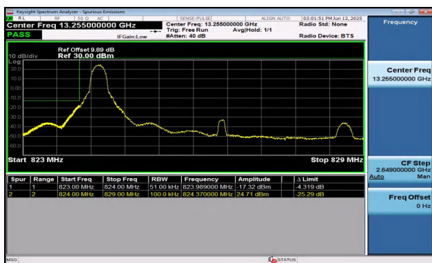
Band5-5MHz-QPSK-20425-1RB#0-PASS
