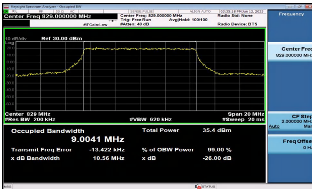
Band5-10MHz-QPSK-20450-50RB#0-PASS
