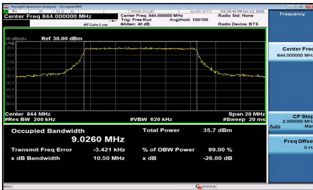
Band5-10MHz-QPSK-20600-50RB#0-PASS
