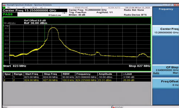
Band5-3MHz-QPSK-20415-1RB#0-PASS
