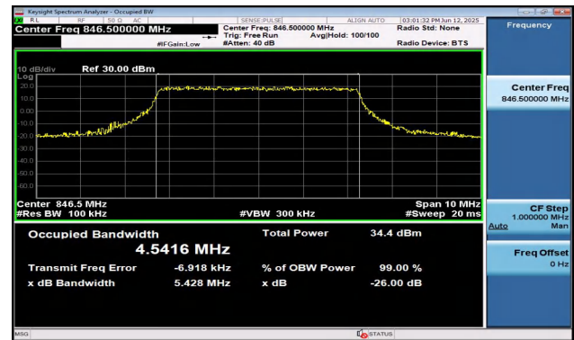
Band5-5MHz-16QAM-20625-25RB#0-PASS
