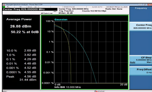
Band5-10MHz-16QAM-20450-1RB#0-PASS
