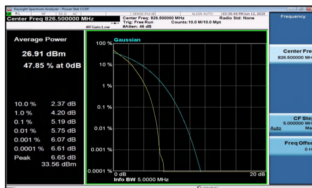
Band5-5MHz-QPSK-20425-25RB#0-PASS
