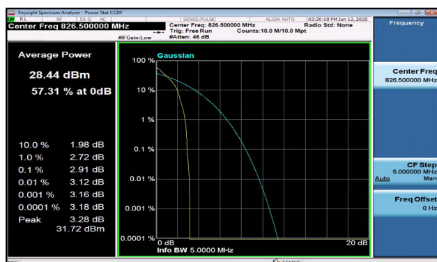
Band5-5MHz-QPSK-20425-1RB#0-PASS
