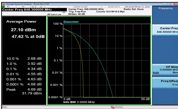
Band5-1.4MHz-QPSK-20643-1RB#0-PASS
