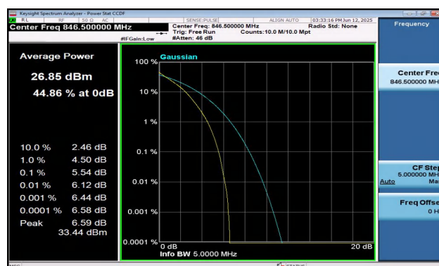
Band5-5MHz-16QAM-20625-25RB#0-PASS
