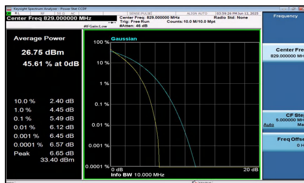
Band5-10MHz-QPSK-20450-50RB#0-PASS
