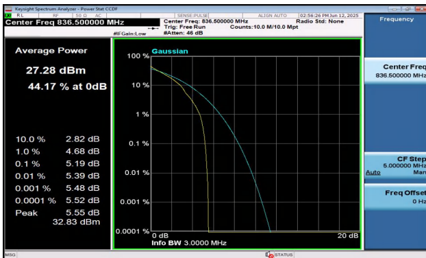
Band5-3MHz-QPSK-20525-1RB#0-PASS
