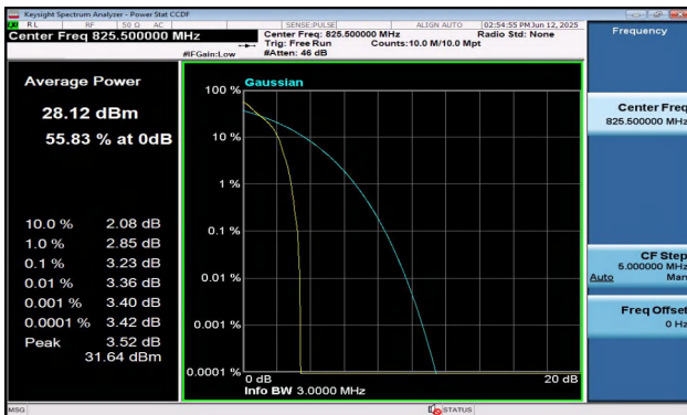
Band5-3MHz-QPSK-20415-1RB#0-PASS
