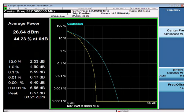
Band5-3MHz-QPSK-20635-15RB#0-PASS
