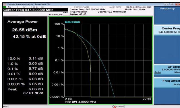
Band5-3MHz-16QAM-20635-1RB#0-PASS
