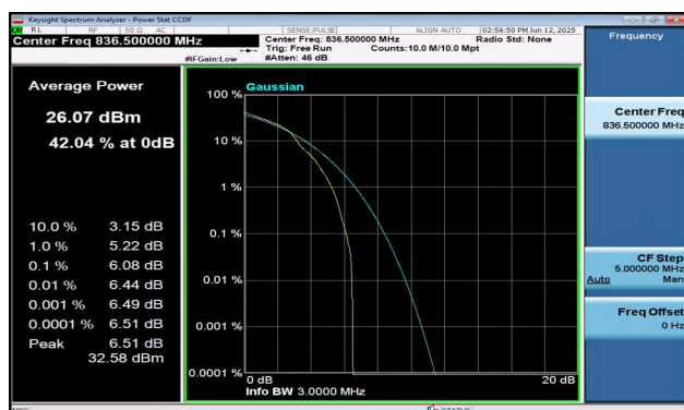
Band5-3MHz-16QAM-20525-1RB#0-PASS
