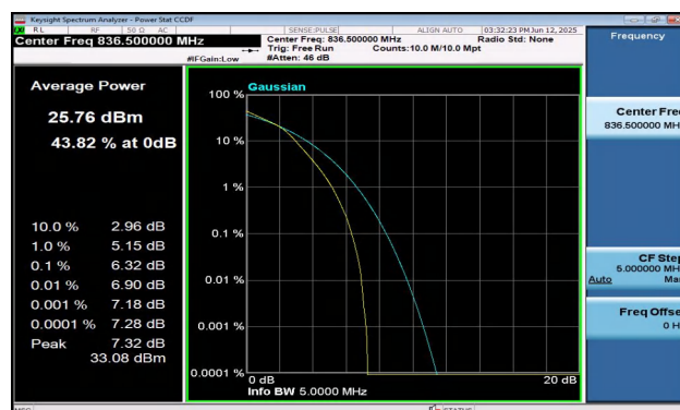
Band5-5MHz-16QAM-20525-25RB#0-PASS
