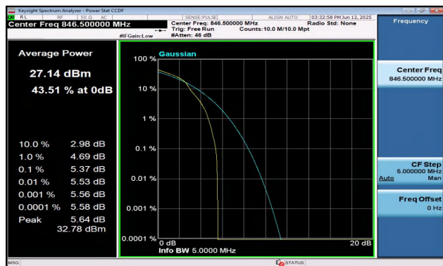
Band5-5MHz-QPSK-20625-1RB#0-PASS
