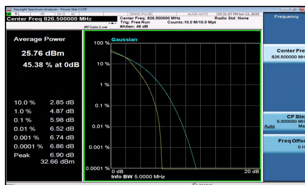
Band5-5MHz-16QAM-20425-25RB#0-PASS
