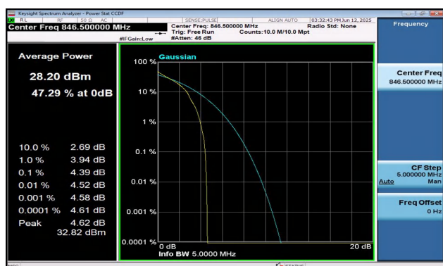
Band5-5MHz-16QAM-20625-1RB#0-PASS
