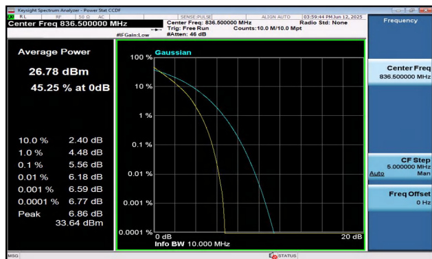
Band5-10MHz-QPSK-20525-50RB#0-PASS
