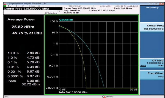
Band5-3MHz-16QAM-20415-15RB#0-PASS
