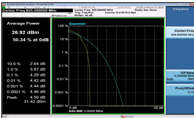
Band5-3MHz-16QAM-20415-1RB#0-PASS
