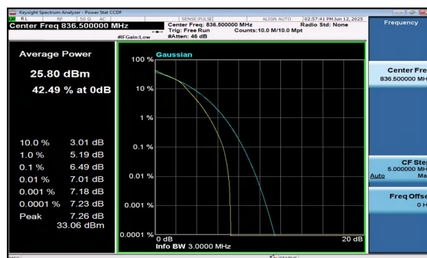
Band5-3MHz-16QAM-20525-15RB#0-PASS
