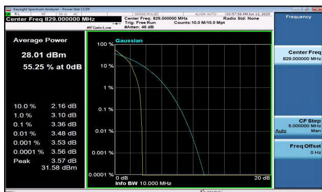
Band5-10MHz-QPSK-20450-1RB#0-PASS
