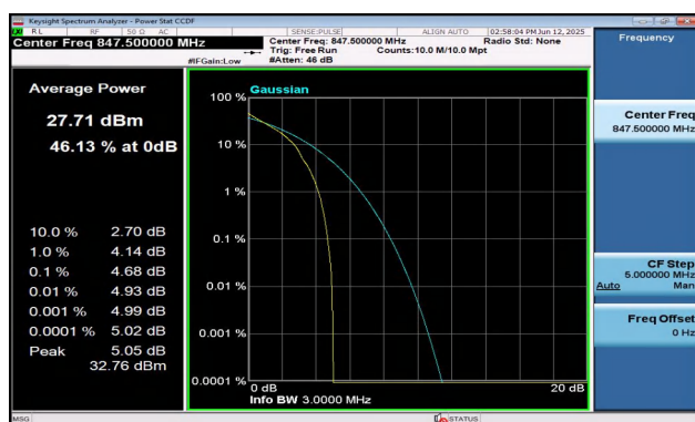
Band5-3MHz-QPSK-20635-1RB#0-PASS
