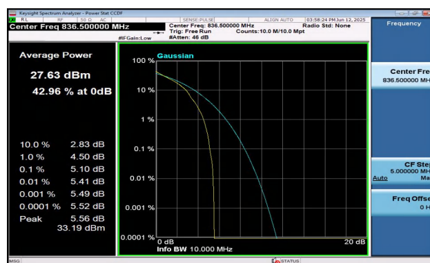
Band5-10MHz-QPSK-20525-1RB#0-PASS
