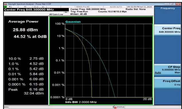
Band5-1.4MHz-QPSK-20643-6RB#0-PASS
