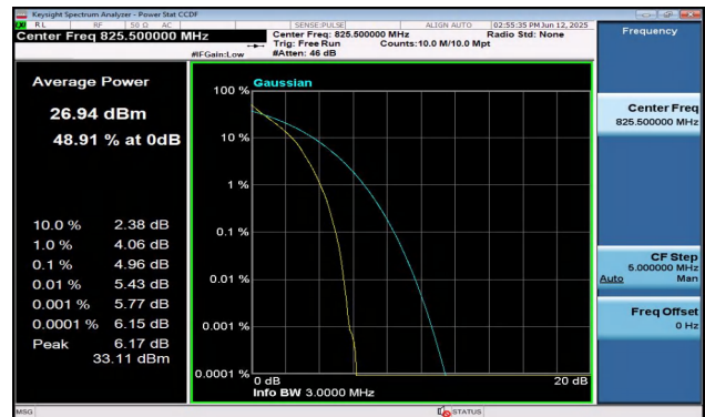
Band5-3MHz-QPSK-20415-15RB#0-PASS
