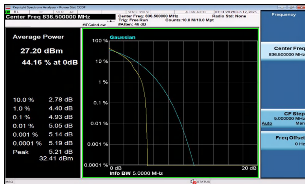
Band5-5MHz-QPSK-20525-1RB#0-PASS
