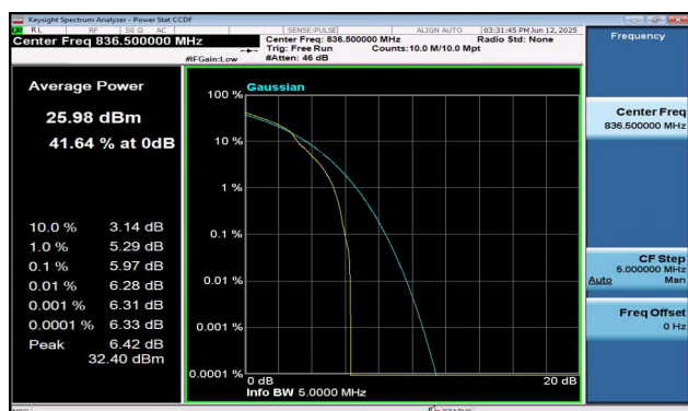
Band5-5MHz-16QAM-20525-1RB#0-PASS
