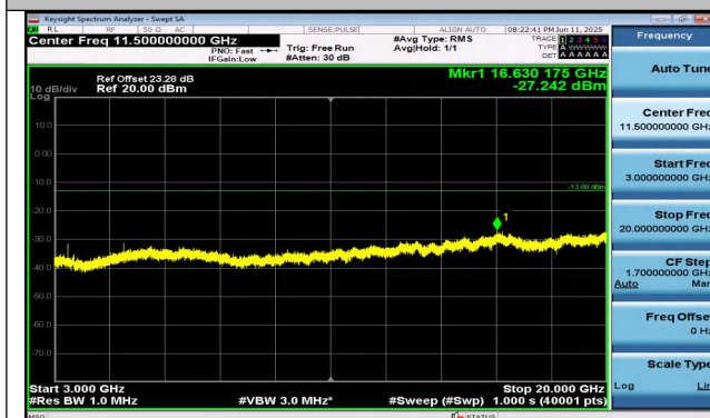
Band4-20MHz-QPSK-20050-1RB#0-3000~20000-PASS
