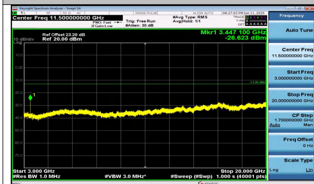
Band4-20MHz-16QAM-20175-1RB#0-3000~20000-PASS
