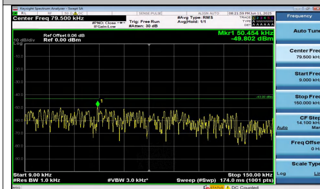
Band4-20MHz-QPSK-20050-1RB#0-0.009~0.15-PASS
