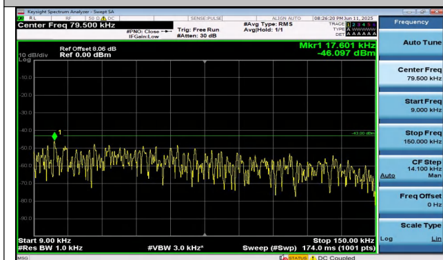
Band4-20MHz-16QAM-20175-1RB#0-0.009~0.15-PASS
