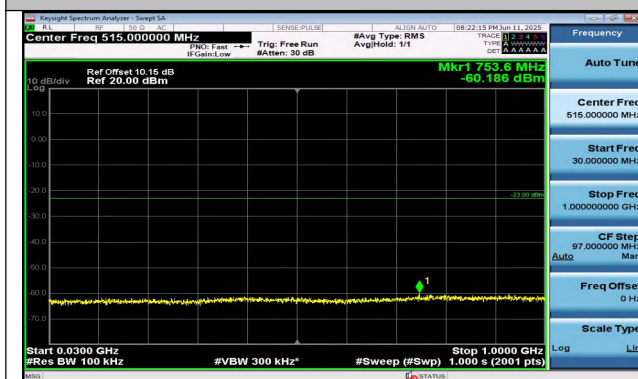
Band4-20MHz-QPSK-20050-1RB#0-30~1000-PASS
