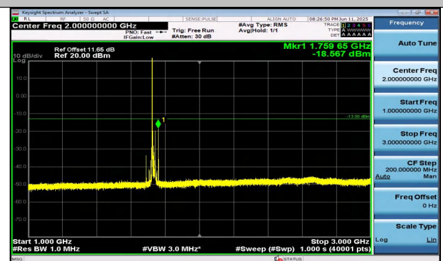
Band4-20MHz-16QAM-20175-1RB#0-1000~3000-PASS
