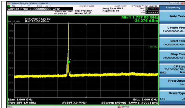
Band4-15MHz-16QAM-20325-1RB#74-1000~3000-PASS
