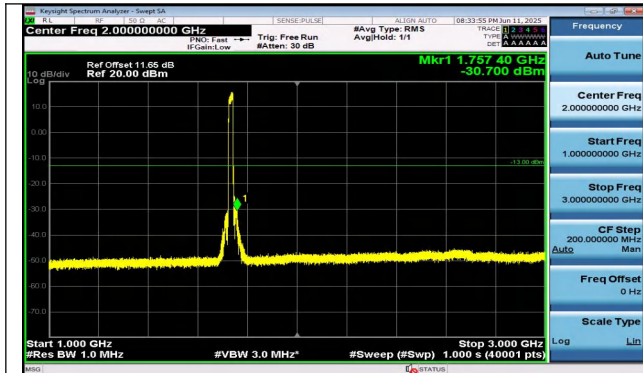
Band4-20MHz-QPSK-20175-100RB#0-1000~3000-PASS
