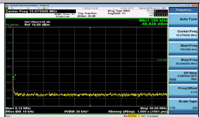
Band4-20MHz-16QAM-20175-1RB#0-0.15~30-PASS
