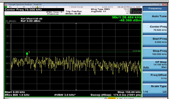
Band4-20MHz-16QAM-20175-1RB#99-0.009~0.15-PASS
