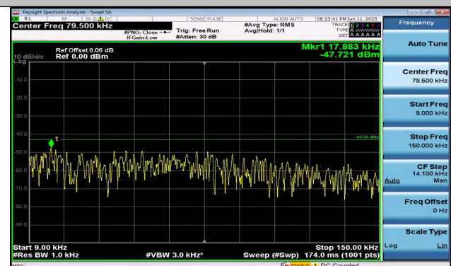
Band4-20MHz-QPSK-20050-1RB#99-0.009~0.15-PASS
