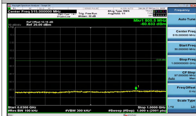
Band4-20MHz-16QAM-20175-1RB#0-0.30~1000-PASS
