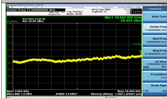
Band4-10MHz-16QAM-20350-1RB#49-3000~20000-PASS
