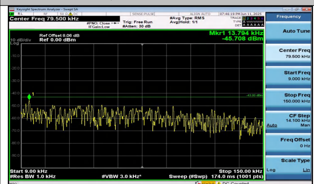
Band4-15MHz-QPSK-20025-1RB#0-0.009~0.15-PASS
