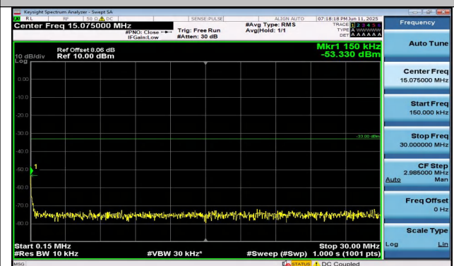
Band4-10MHz-16QAM-20350-1RB#49-0.15~30-PASS
