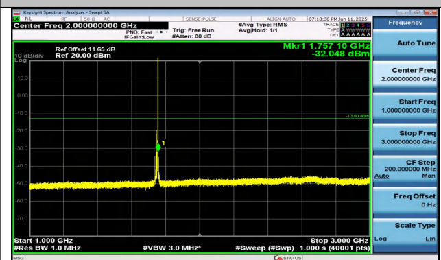
Band4-10MHz-16QAM-20350-1RB#49-1000~3000-PASS
