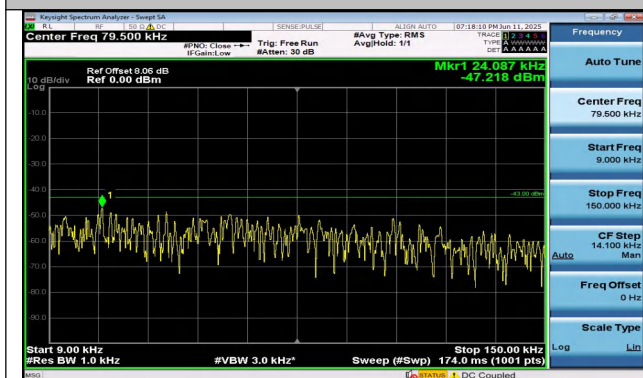
Band4-10MHz-16QAM-20350-1RB#49-0.009~0.15-PASS
