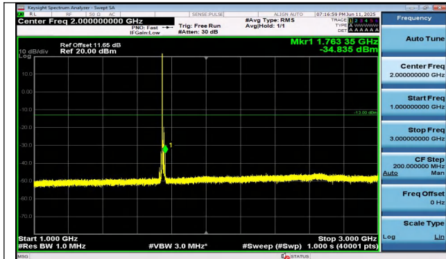
Band4-10MHz-16QAM-20350-1RB#0-1000~3000-PASS
