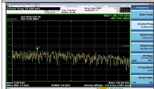
Band4-5MHz-QPSK-20175-25RB#0-0.009~0.15-PASS
