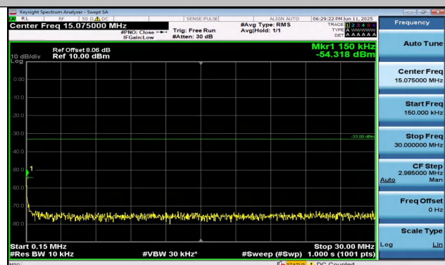
Band4-5MHz-QPSK-20175-25RB#0-0.15~30-PASS
