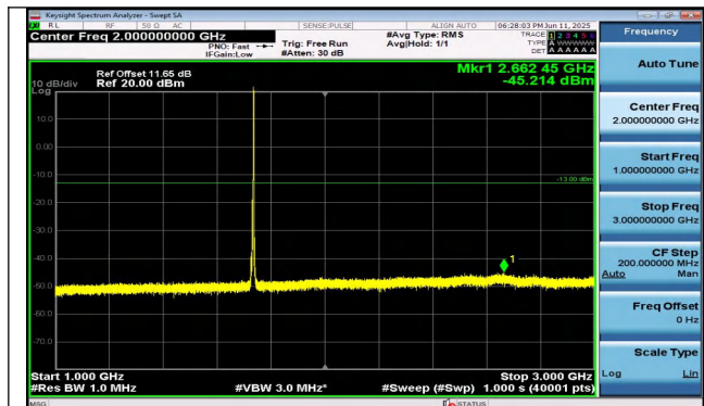
Band4-5MHz-QPSK-20175-1RB#24-1000~3000-PASS
