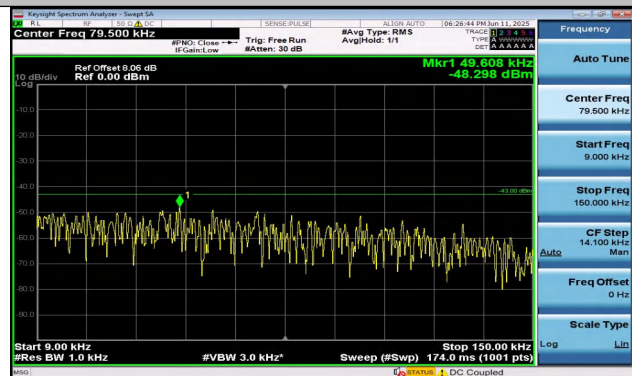
Band4-5MHz-16QAM-20175-1RB#0-0.009~0.15-PASS
