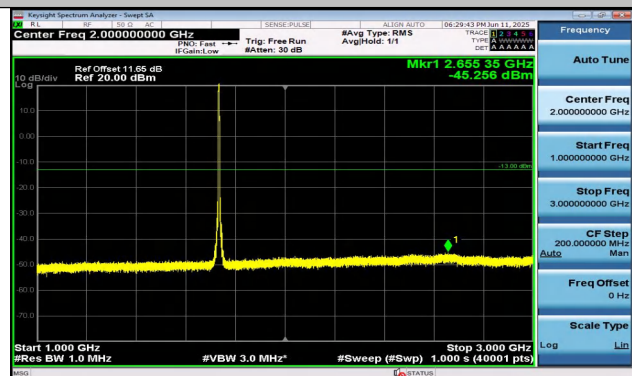
Band4-5MHz-QPSK-20175-25RB#0-1000~3000-PASS
