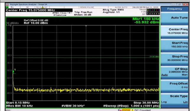
Band4-5MHz-QPSK-19975-1RB#0-0.15~30-PASS
