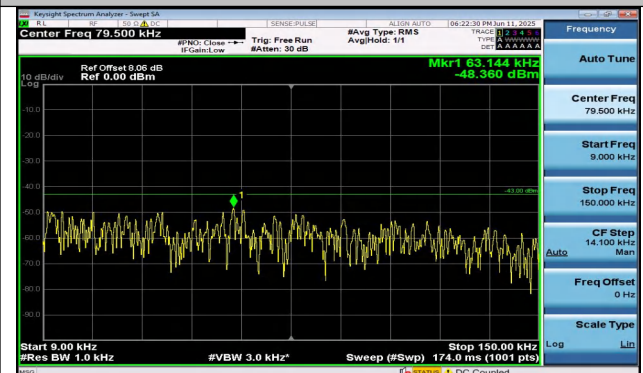
Band4-5MHz-QPSK-19975-1RB#24-0.009~0.15-PASS
