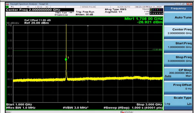
Band4-5MHz-QPSK-19975-1RB#0-1000~3000-PASS
