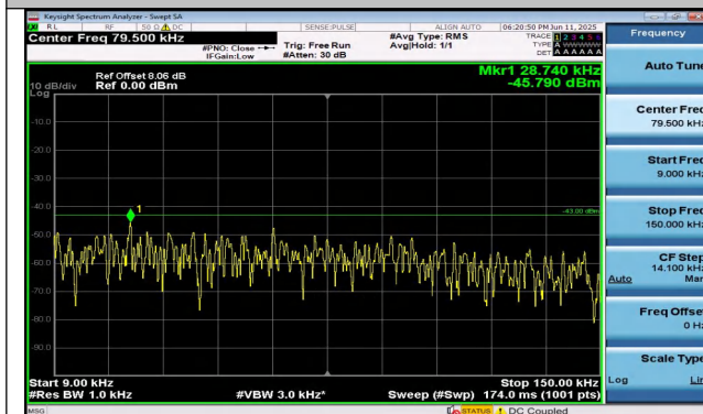
Band4-5MHz-QPSK-19975-1RB#0-0.009~0.15-PASS
