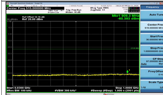
Band4-5MHz-QPSK-19975-1RB#0-30~1000-PASS
