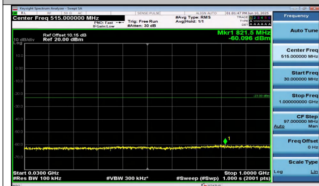
Band4-1.4MHz-QPSK-20393-6RB#0-30~1000-PASS
