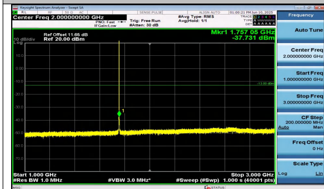
Band4-1.4MHz-QPSK-20393-1RB#5-1000~3000-PASS
