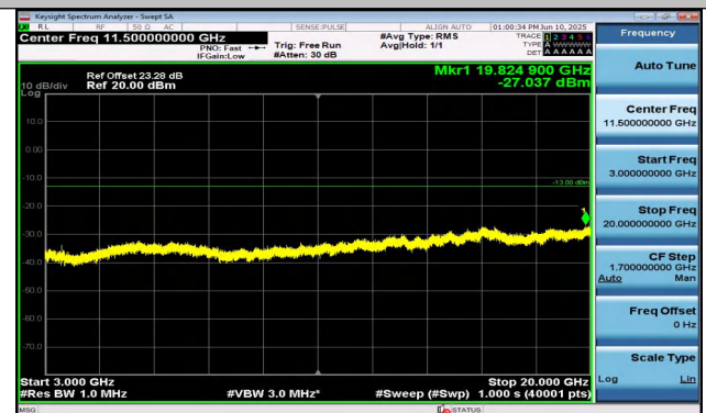
Band4-1.4MHz-QPSK-20393-1RB#5-3000~20000-PASS
