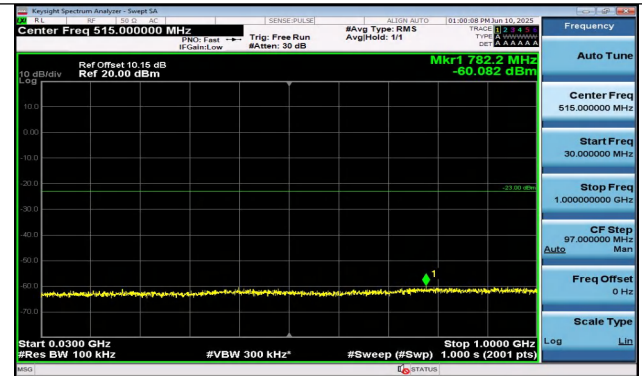
Band4-1.4MHz-QPSK-20393-1RB#5-30~1000-PASS
