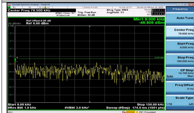
Band4-1.4MHz-QPSK-20393-6RB#0-0.009~0.15-PASS
