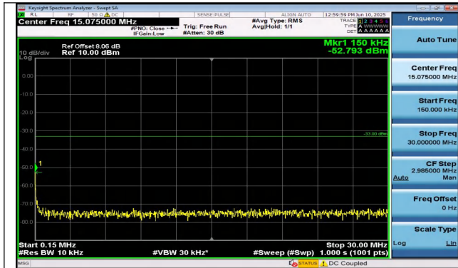
Band4-1.4MHz-QPSK-20393-1RB#5-0.15~30-PASS
