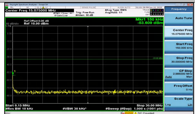
Band4-1.4MHz-QPSK-20393-6RB#0-0.15~30-PASS
