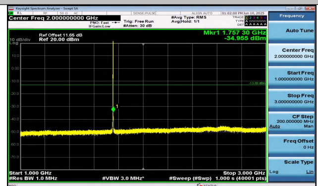
Band4-1.4MHz-QPSK-20393-6RB#0-1000~3000-PASS
