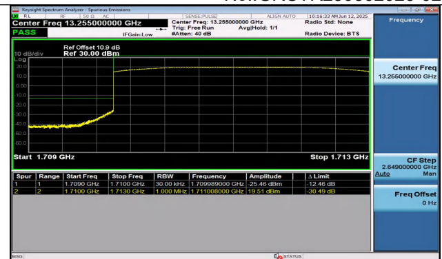
Band4-3MHz-16QAM-19965-15RB#0-PASS
