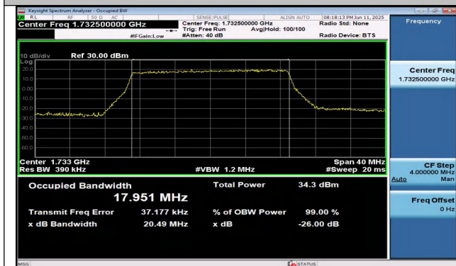
Band4-20MHz-QPSK-20175-100RB#0-PASS
