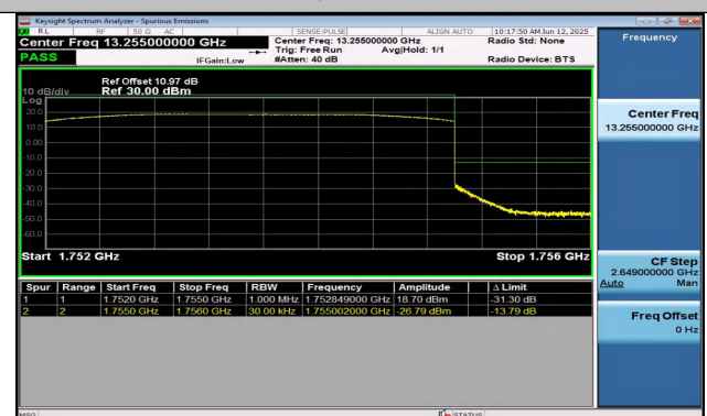
Band4-3MHz-16QAM-20385-15RB#0-PASS
