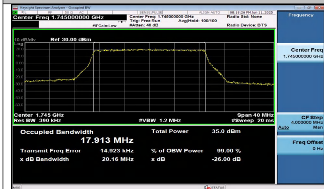
Band4-20MHz-QPSK-20300-100RB#0-PASS
