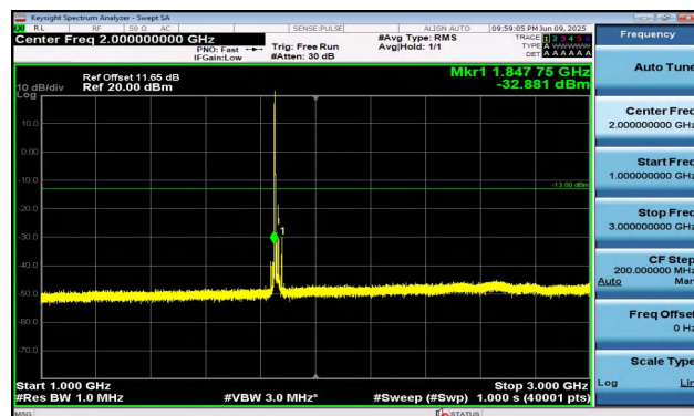
Band2-15MHz-16QAM-18675-1RB#0-1000~3000-PASS
