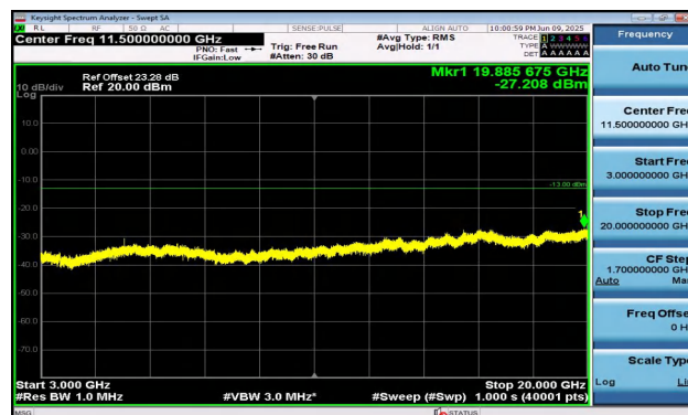
Band2-15MHz-16QAM-18675-1RB#74-3000~20000-PASS
