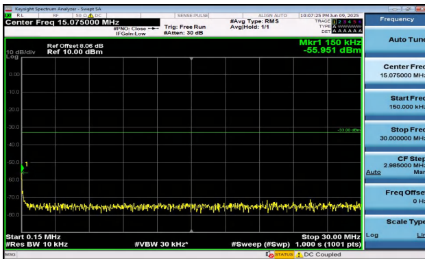
Band2-15MHz-16QAM-19125-1RB#74-0.15~30-PASS
