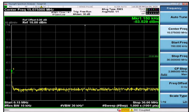
Band2-20MHz-QPSK-18700-1RB#0-0.15~30-PASS
