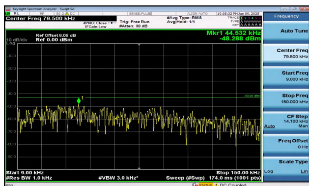
Band2-15MHz-16QAM-19125-1RB#0-0.009~0.15-PASS
