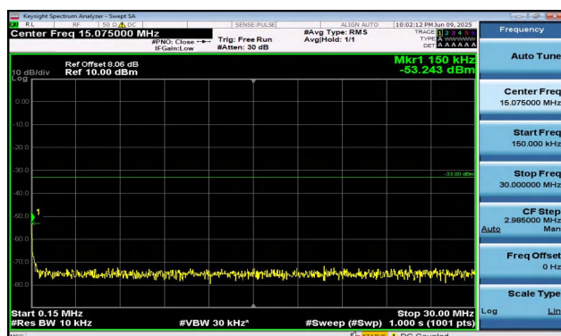
Band2-15MHz-16QAM-18900-1RB#0-0.15~30-PASS
