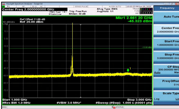
Band2-15MHz-QPSK-18900-1RB#74-1000~3000-PASS
