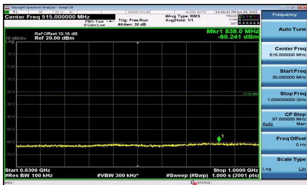
Band2-15MHz-QPSK-19125-1RB#74-30~1000-PASS
