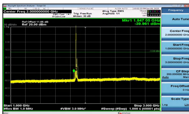
Band2-15MHz-16QAM-18900-1RB#0-1000~3000-PASS
