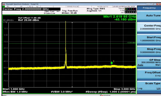
Band2-15MHz-QPSK-19125-1RB#0-1000~3000-PASS
