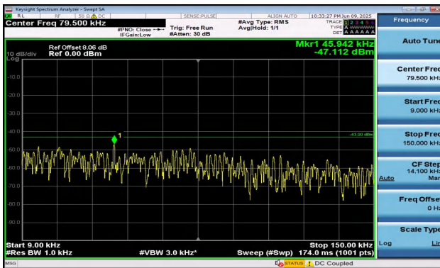
Band2-20MHz-QPSK-18700-1RB#0-0.009~0.15-PASS
