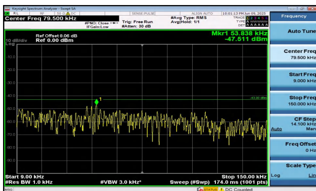
Band2-15MHz-QPSK-18900-1RB#0-0.009~0.15-PASS
