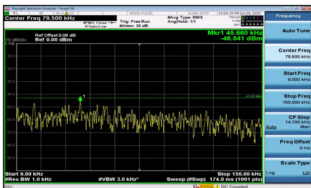
Band2-15MHz-QPSK-19125-1RB#74-0.009~0.15-PASS
