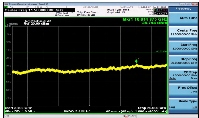
Band2-15MHz-QPSK-18900-1RB#74-3000~20000-PASS
