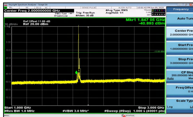
Band2-15MHz-QPSK-18900-1RB#0-1000~3000-PASS
