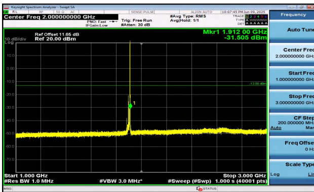
Band2-15MHz-16QAM-19125-1RB#74-1000~3000-PASS
