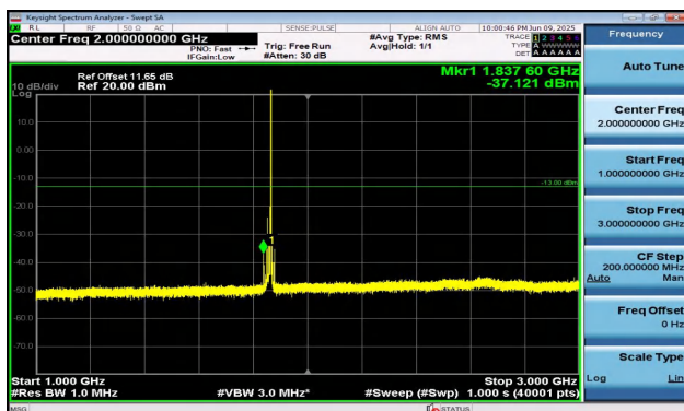
Band2-15MHz-16QAM-18675-1RB#74-1000~3000-PASS
