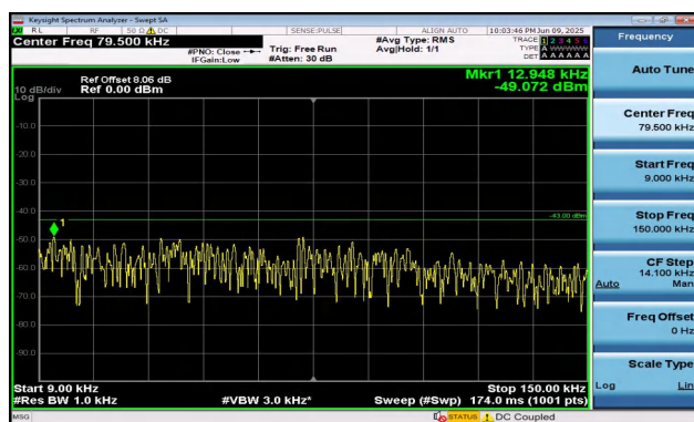
Band2-15MHz-16QAM-18900-1RB#74-0.009~0.15-PASS
