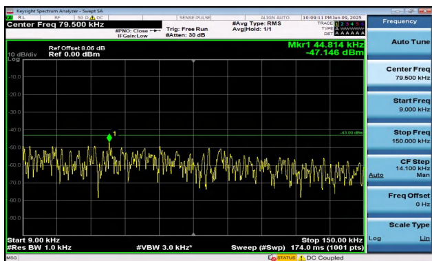
Band2-15MHz-QPSK-18900-75RB#0-0.009~0.15-PASS
