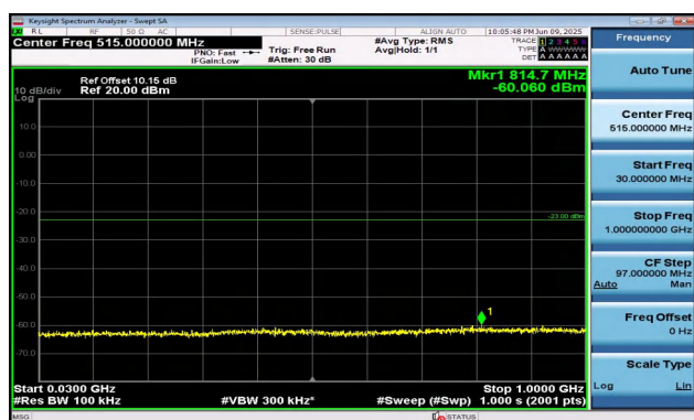
Band2-15MHz-16QAM-19125-1RB#0-30~1000-PASS
