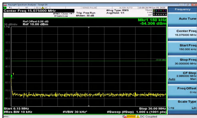
Band2-15MHz-16QAM-18675-1RB#74-0.15~30-PASS
