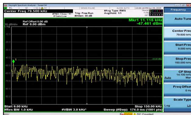
Band2-15MHz-16QAM-18675-1RB#74-0.009~0.15-PASS
