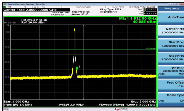
Band2-15MHz-QPSK-18900-75RB#0-1000~3000-PASS
