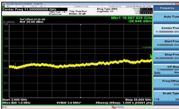
Band2-15MHz-QPSK-18900-1RB#0-3000~20000-PASS
