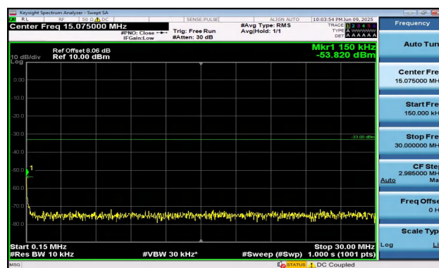
Band2-15MHz-16QAM-18900-1RB#74-0.15~30-PASS
