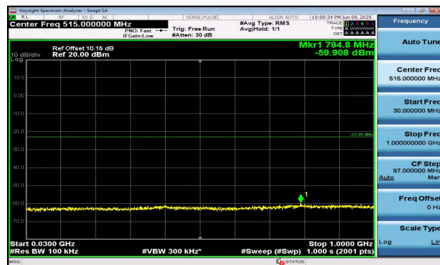
Band2-15MHz-16QAM-18675-1RB#74-30~1000-PASS
