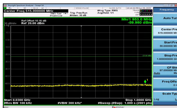
Band2-15MHz-QPSK-19125-75RB#0-30~1000-PASS
