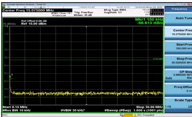
Band2-15MHz-QPSK-18900-1RB#74-0.15~30-PASS
