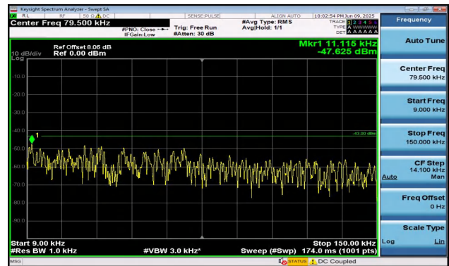
Band2-15MHz-QPSK-18900-1RB#74-0.009~0.15-PASS
