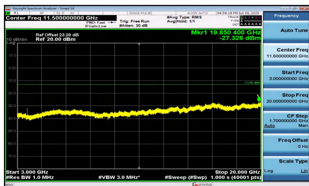
Band2-15MHz-16QAM-18675-1RB#0-3000~20000-PASS
