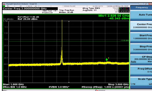
Band2-15MHz-16QAM-18900-1RB#74-1000~3000-PASS
