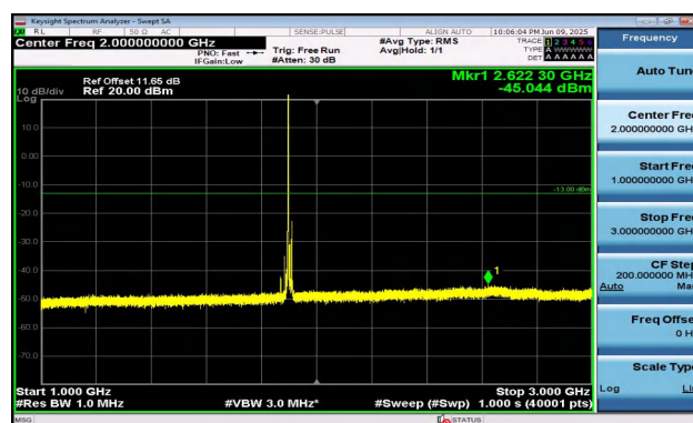
Band2-15MHz-16QAM-19125-1RB#0-1000~3000-PASS
