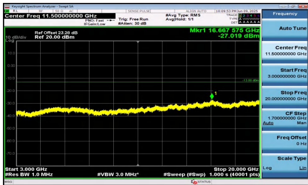
Band2-15MHz-QPSK-18900-75RB#0-3000~20000-PASS
