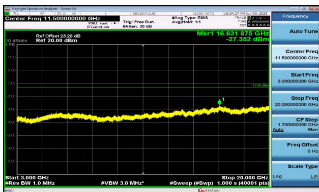
Band2-15MHz-16QAM-18900-1RB#74-3000~20000-PASS
