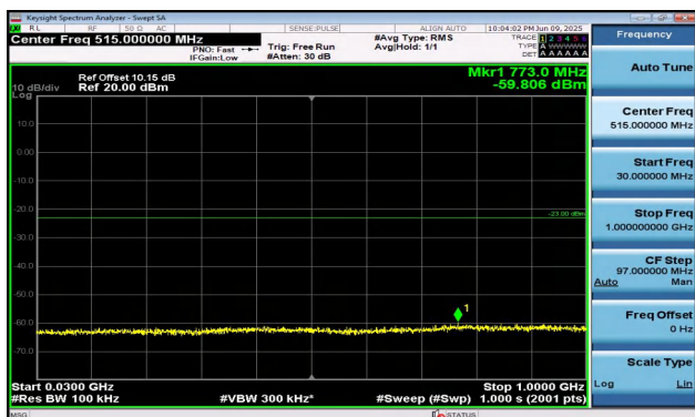
Band2-15MHz-16QAM-18900-1RB#74-30~1000-PASS
