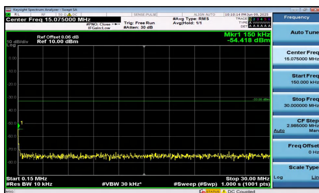
Band2-15MHz-QPSK-19125-75RB#0-0.15~30-PASS
