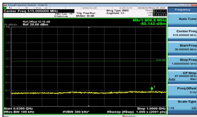
Band2-15MHz-16QAM-18675-1RB#0-30~1000-PASS
