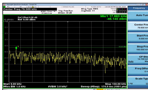
Band2-20MHz-QPSK-18700-1RB#99-0.009~0.15-PASS
