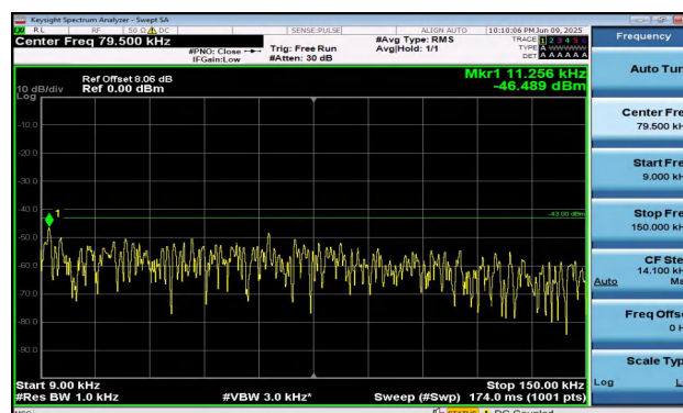
Band2-15MHz-QPSK-19125-75RB#0-0.009~0.15-PASS
