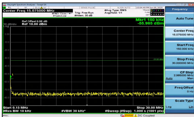
Band2-15MHz-QPSK-19125-1RB#0-0.15~30-PASS
