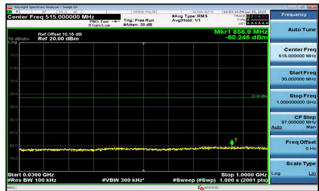
Band2-15MHz-QPSK-18900-1RB#74-30~1000-PASS
