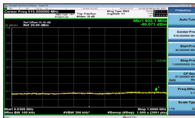
Band2-20MHz-QPSK-18700-1RB#99-30~1000-PASS
