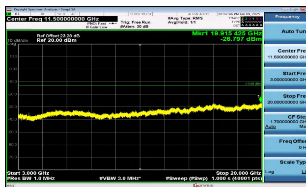
Band2-15MHz-16QAM-18900-1RB#0-3000~20000-PASS
