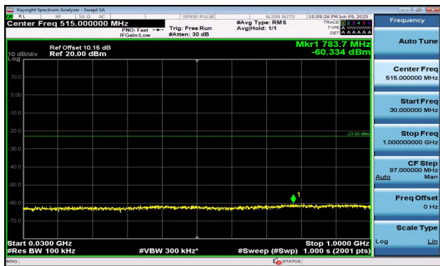
Band2-15MHz-QPSK-18900-75RB#0-30~1000-PASS
