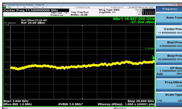
Band2-15MHz-QPSK-19125-1RB#0-3000~20000-PASS
