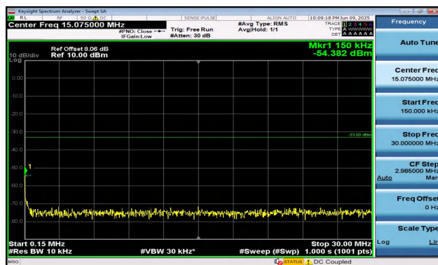
Band2-15MHz-QPSK-18900-75RB#0-0.15~30-PASS
