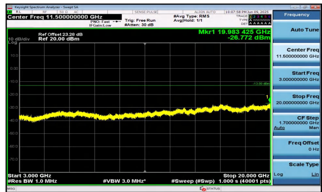
Band2-15MHz-16QAM-19125-1RB#74-3000~20000-PASS
