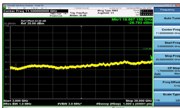
Band2-20MHz-QPSK-18700-1RB#0-3000~20000-PASS
