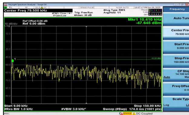
Band2-15MHz-16QAM-19125-1RB#74-0.009~0.15-PASS
