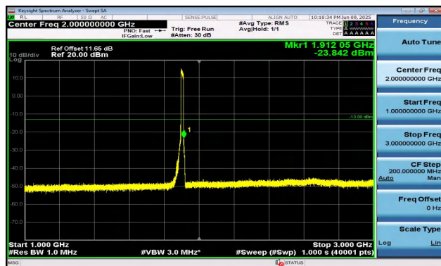
Band2-15MHz-QPSK-19125-75RB#0-1000~3000-PASS
