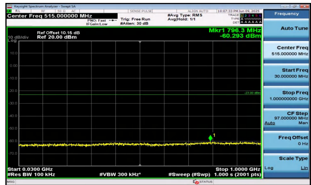
Band2-15MHz-16QAM-19125-1RB#74-30~1000-PASS
