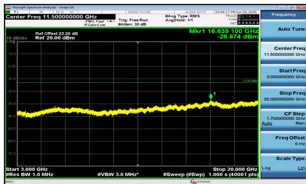
Band2-15MHz-16QAM-19125-1RB#0-3000~20000-PASS
