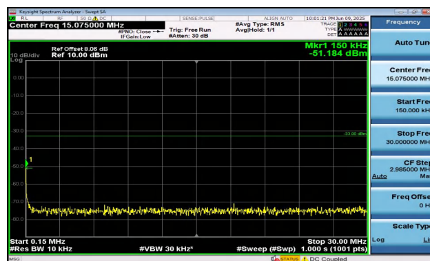
Band2-15MHz-QPSK-18900-1RB#0-0.15~30-PASS
