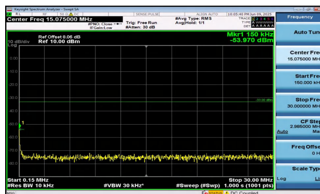
Band2-15MHz-16QAM-19125-1RB#0-0.15~30-PASS
