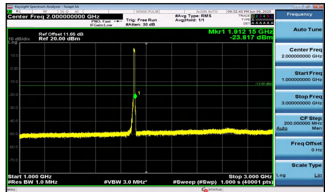
Band2-10MHz-QPSK-19150-50RB#0-1000~3000-PASS
