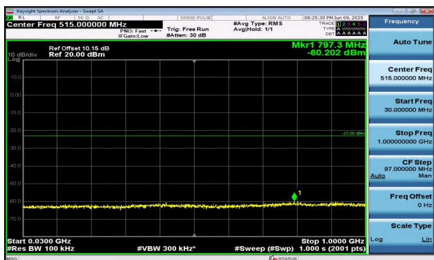
Band2-10MHz-QPSK-18900-1RB#49-30~1000-PASS
