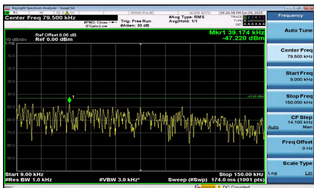
Band2-10MHz-QPSK-19150-1RB#0-0.009~0.15-PASS
