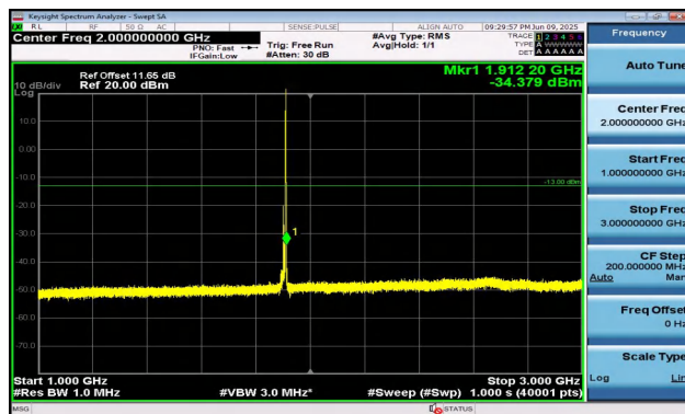
Band2-10MHz-16QAM-19150-1RB#49-1000~3000-PASS
