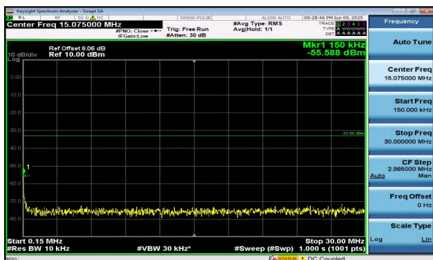
Band2-10MHz-QPSK-19150-1RB#49-0.15~30-PASS
