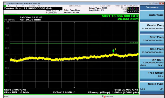
Band2-15MHz-QPSK-18675-1RB#0-3000~20000-PASS
