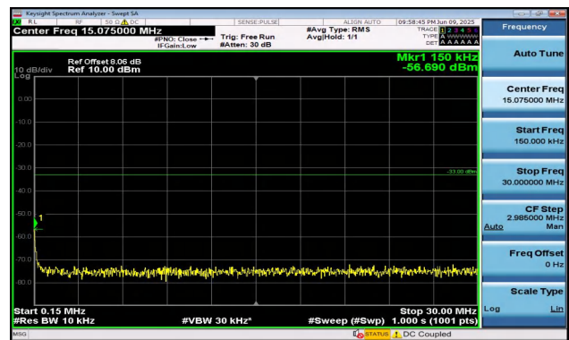
Band2-15MHz-16QAM-18675-1RB#0-0.15~30-PASS
