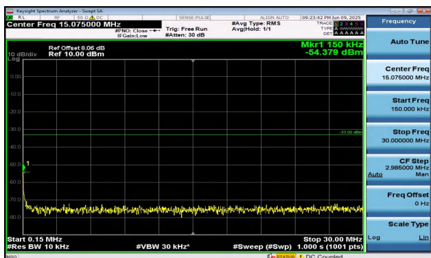
Band2-10MHz-QPSK-18900-1RB#0-0.15~30-PASS
