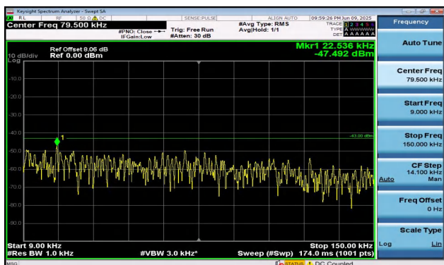
Band2-15MHz-QPSK-18675-1RB#74-0.009~0.15-PASS
