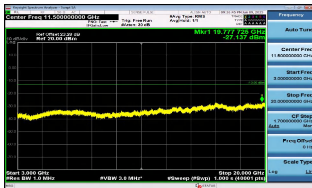
Band2-10MHz-16QAM-18900-1RB#49-3000~20000-PASS
