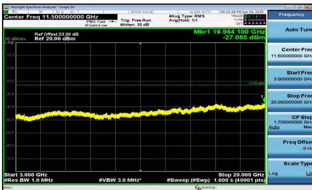
Band2-10MHz-QPSK-19150-50RB#0-3000~20000-PASS
