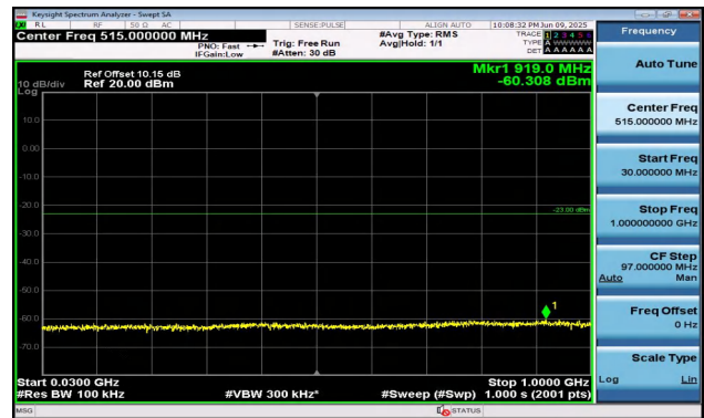
Band2-15MHz-QPSK-18675-75RB#0-30~1000-PASS
