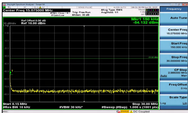
Band2-10MHz-QPSK-18900-50RB#0-0.15~30-PASS
