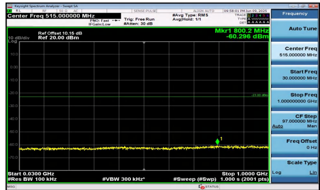
Band2-15MHz-QPSK-18675-1RB#0-30~1000-PASS
