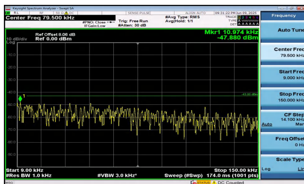
Band2-10MHz-QPSK-18900-50RB#0-0.009~0.15-PASS
