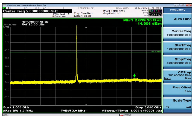
Band2-10MHz-QPSK-18900-1RB#0-1000~3000-PASS
