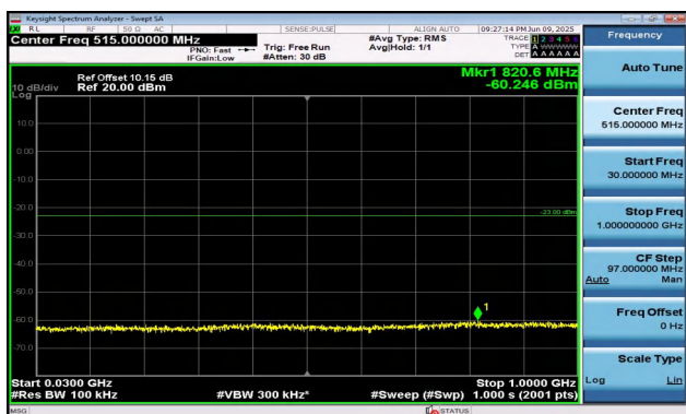
Band2-10MHz-QPSK-19150-1RB#0-30~1000-PASS
