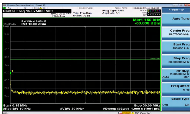
Band2-10MHz-16QAM-18900-1RB#49-0.15~30-PASS
