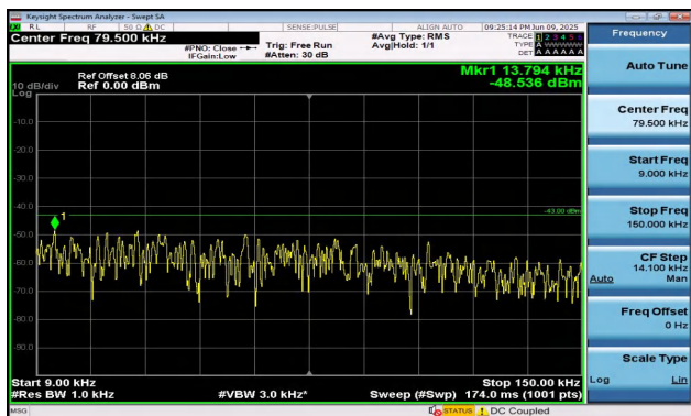
Band2-10MHz-QPSK-18900-1RB#49-0.009~0.15-PASS
