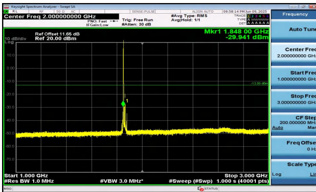
Band2-15MHz-QPSK-18675-1RB#0-1000~3000-PASS
