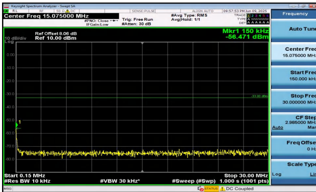
Band2-15MHz-QPSK-18675-1RB#0-0.15~30-PASS
