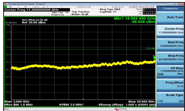
Band2-15MHz-QPSK-18675-75RB#0-3000~20000-PASS
