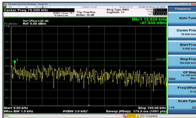
Band2-15MHz-QPSK-18675-75RB#0-0.009~0.15-PASS
