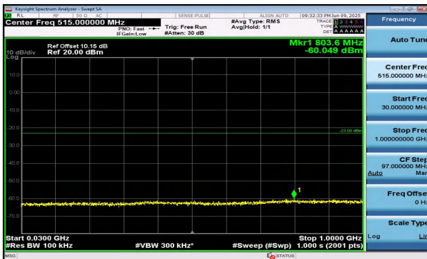
Band2-10MHz-QPSK-19150-50RB#0-30~1000-PASS
