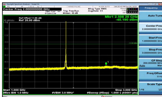
Band2-10MHz-QPSK-18900-1RB#49-1000~3000-PASS
