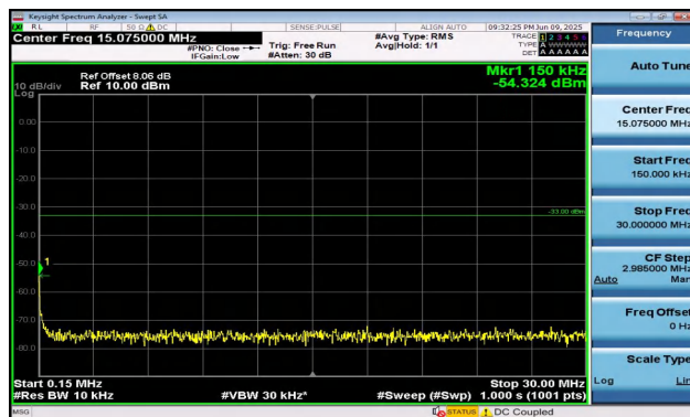
Band2-10MHz-QPSK-19150-50RB#0-0.15~30-PASS
