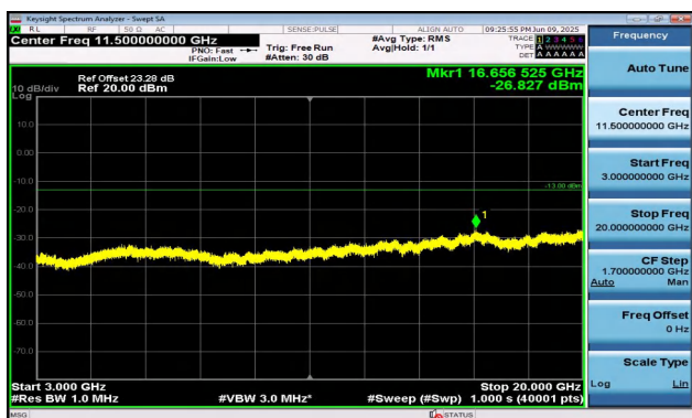
Band2-10MHz-QPSK-18900-1RB#49-3000~20000-PASS
