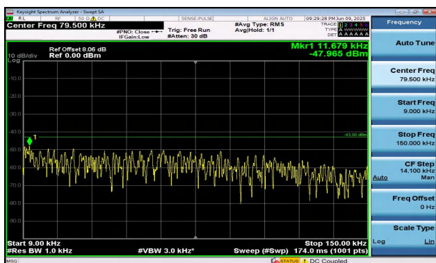
Band2-10MHz-16QAM-19150-1RB#49-0.009~0.15-PASS
