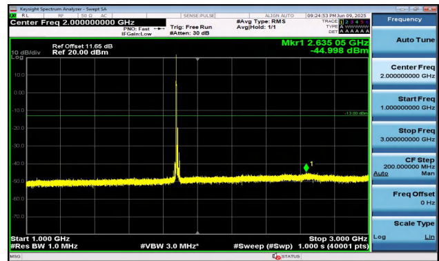
Band2-10MHz-16QAM-18900-1RB#0-1000~3000-PASS
