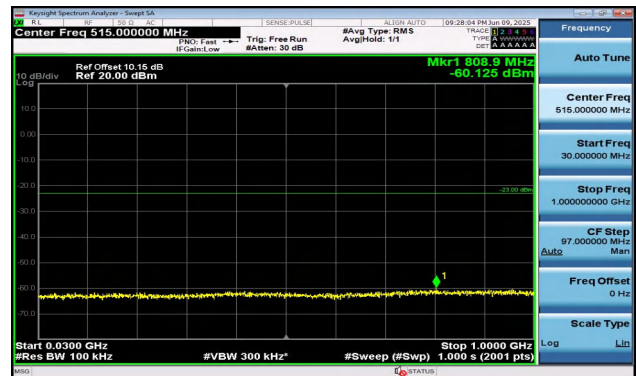
Band2-10MHz-16QAM-19150-1RB#0-30~1000-PASS
