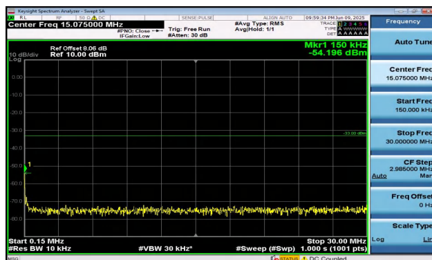
Band2-15MHz-QPSK-18675-1RB#74-0.15~30-PASS
