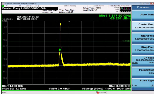
Band2-15MHz-QPSK-18675-75RB#0-1000~3000-PASS
