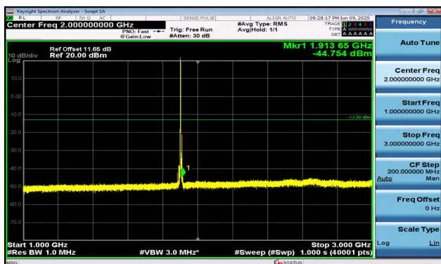
Band2-10MHz-16QAM-19150-1RB#0-1000~3000-PASS
