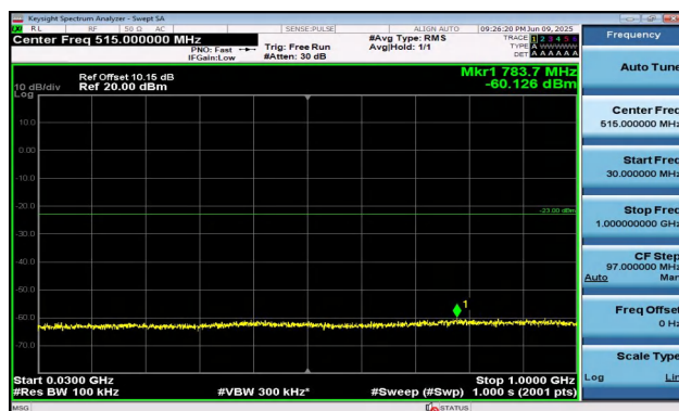
Band2-10MHz-16QAM-18900-1RB#49-30~1000-PASS
