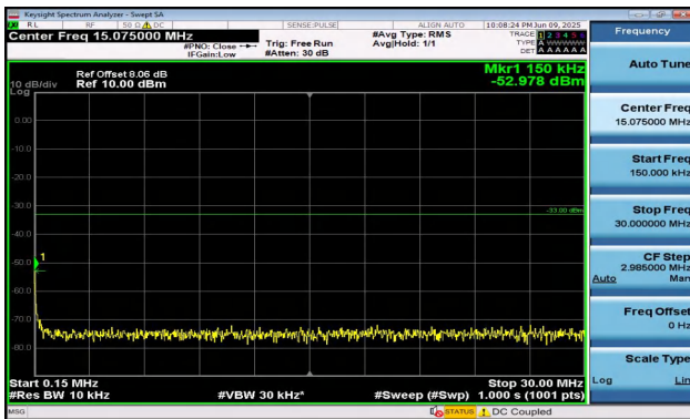
Band2-15MHz-QPSK-18675-75RB#0-0.15~30-PASS
