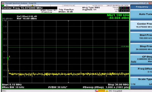
Band2-10MHz-16QAM-19150-1RB#0-0.15~30-PASS
