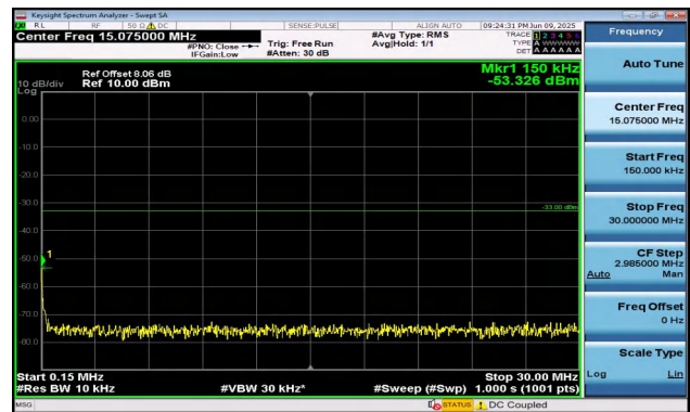
Band2-10MHz-16QAM-18900-1RB#0-0.15~30-PASS
