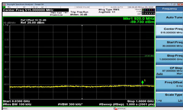
Band2-10MHz-16QAM-19150-1RB#49-30~1000-PASS
