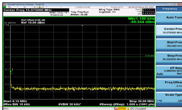
Band2-10MHz-QPSK-18900-1RB#49-0.15~30-PASS
