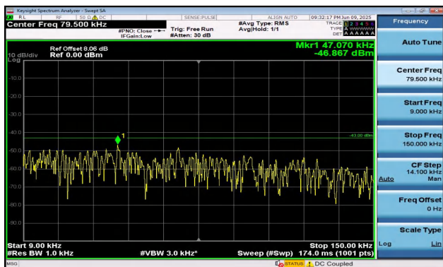
Band2-10MHz-QPSK-19150-50RB#0-0.009~0.15-PASS
