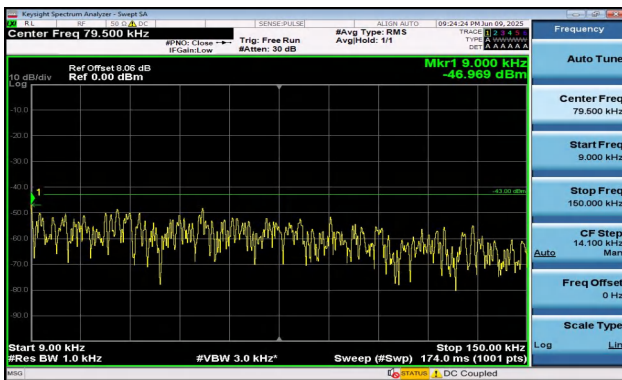
Band2-10MHz-16QAM-18900-1RB#0-0.009~0.15-PASS
