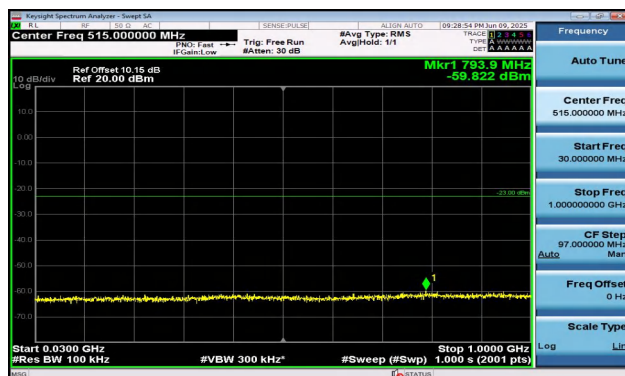
Band2-10MHz-QPSK-19150-1RB#49-30~1000-PASS
