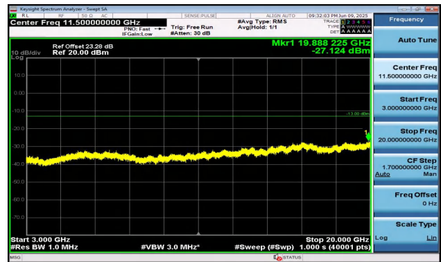
Band2-10MHz-QPSK-18900-50RB#0-3000~20000-PASS
