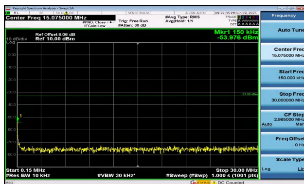
Band2-10MHz-16QAM-19150-1RB#49-0.15~30-PASS
