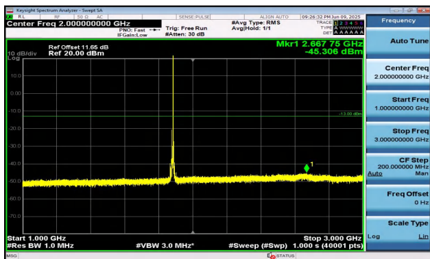
Band2-10MHz-16QAM-18900-1RB#49-1000~3000-PASS
