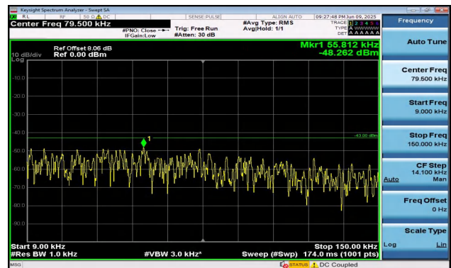
Band2-10MHz-16QAM-19150-1RB#0-0.009~0.15-PASS
