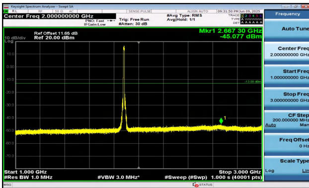
Band2-10MHz-QPSK-18900-50RB#0-1000~3000-PASS
