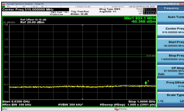
Band2-10MHz-16QAM-18900-1RB#0-30~1000-PASS
