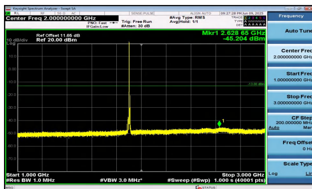
Band2-10MHz-QPSK-19150-1RB#0-1000~3000-PASS
