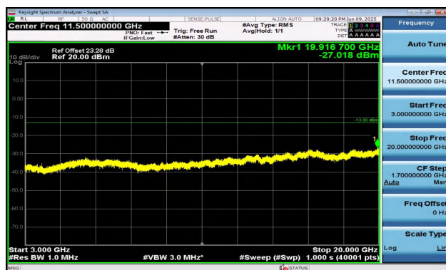
Band2-10MHz-QPSK-19150-1RB#49-3000~20000-PASS
