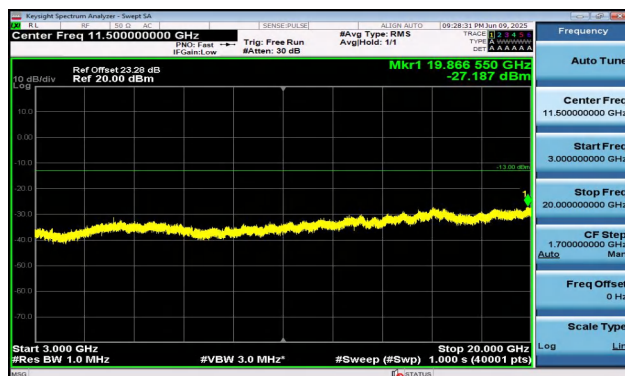
Band2-10MHz-16QAM-19150-1RB#0-3000~20000-PASS
