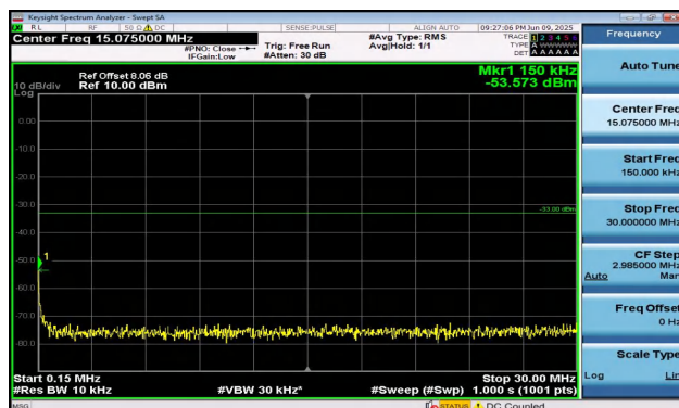
Band2-10MHz-QPSK-19150-1RB#0-0.15~30-PASS
