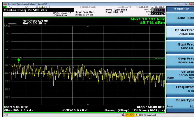
Band2-10MHz-QPSK-19150-1RB#49-0.009~0.15-PASS
