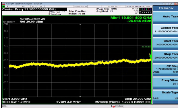
Band2-10MHz-16QAM-19150-1RB#49-3000~20000-PASS
