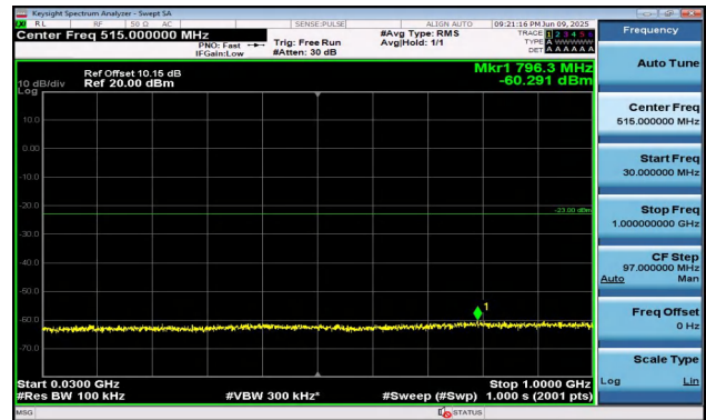
Band2-10MHz-16QAM-18650-1RB#0-30~1000-PASS
