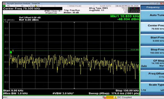
Band2-5MHz-16QAM-19175-25RB#0-0.009~0.15-PASS
