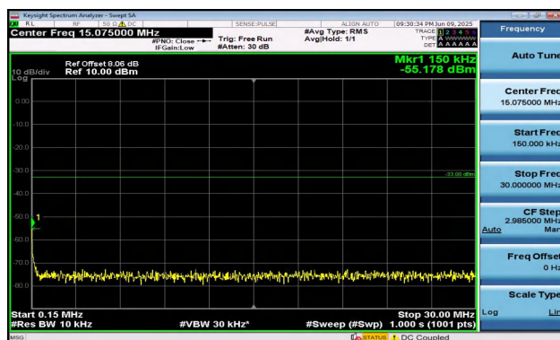
Band2-10MHz-QPSK-18650-50RB#0-0.15~30-PASS
