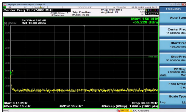
Band2-10MHz-QPSK-18650-1RB#0-0.15~30-PASS
