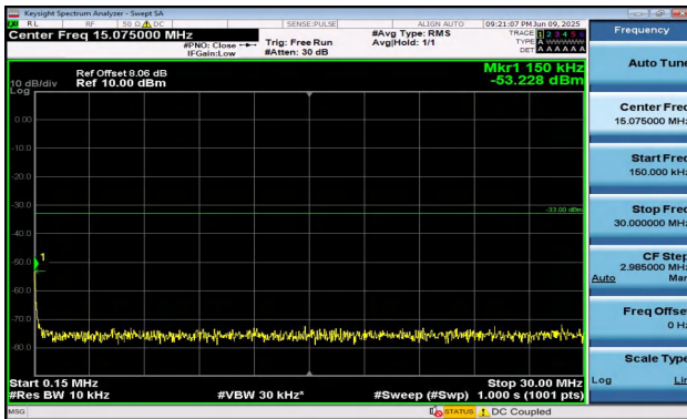
Band2-10MHz-16QAM-18650-1RB#0-0.15~30-PASS
