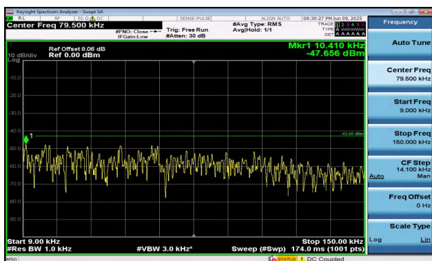
Band2-10MHz-QPSK-18650-50RB#0-0.009~0.15-PASS
