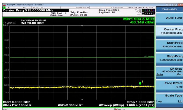
Band2-10MHz-QPSK-18650-1RB#0-30~1000-PASS
