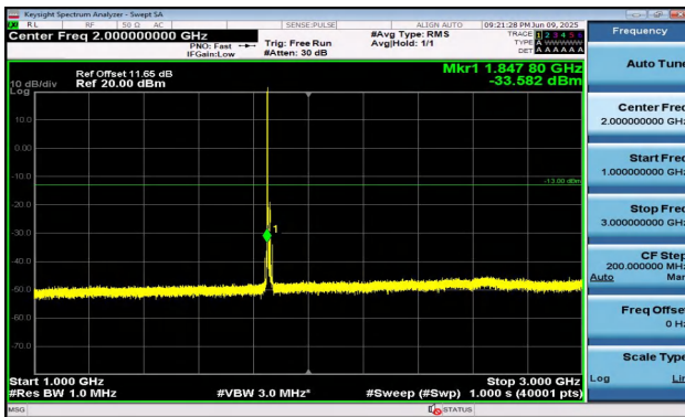
Band2-10MHz-16QAM-18650-1RB#0-1000~3000-PASS
