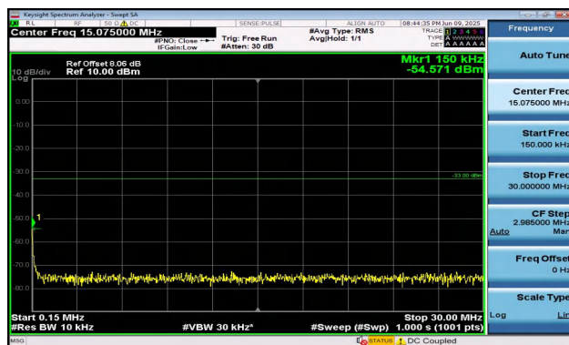
Band2-5MHz-16QAM-19175-1RB#24-0.15~30-PASS
