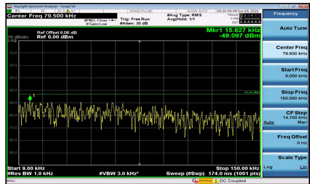
Band2-10MHz-16QAM-18650-1RB#0-0.009~0.15-PASS
