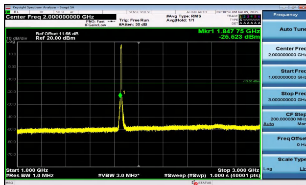
Band2-10MHz-QPSK-18650-50RB#0-1000~3000-PASS
