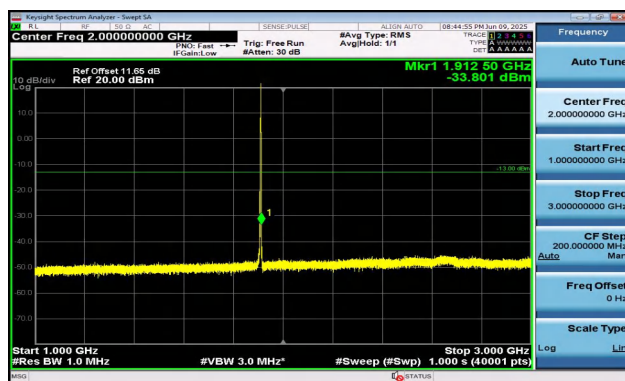
Band2-5MHz-16QAM-19175-1RB#24-1000~3000-PASS
