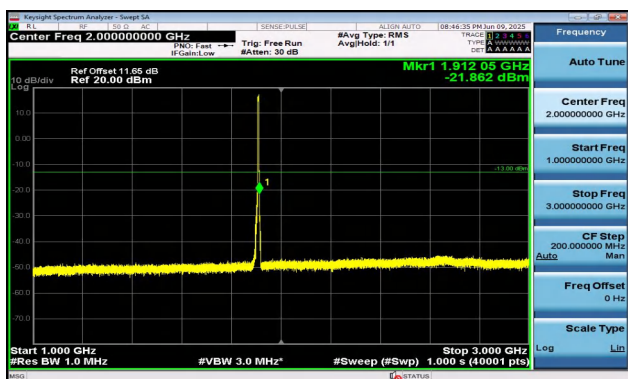
Band2-5MHz-16QAM-19175-25RB#0-1000~3000-PASS
