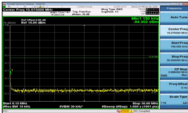
Band2-10MHz-QPSK-18650-1RB#49-0.15~30-PASS
