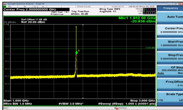
Band2-5MHz-QPSK-19175-25RB#0-1000~3000-PASS
