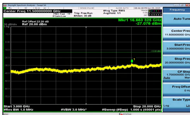
Band2-5MHz-16QAM-19175-25RB#0-3000~20000-PASS
