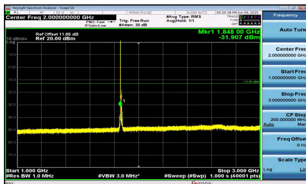
Band2-10MHz-QPSK-18650-1RB#0-1000~3000-PASS
