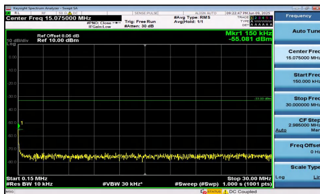
Band2-10MHz-16QAM-18650-1RB#49-0.15~30-PASS
