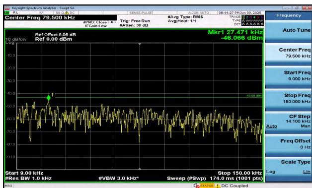
Band2-5MHz-16QAM-19175-1RB#24-0.009~0.15-PASS
