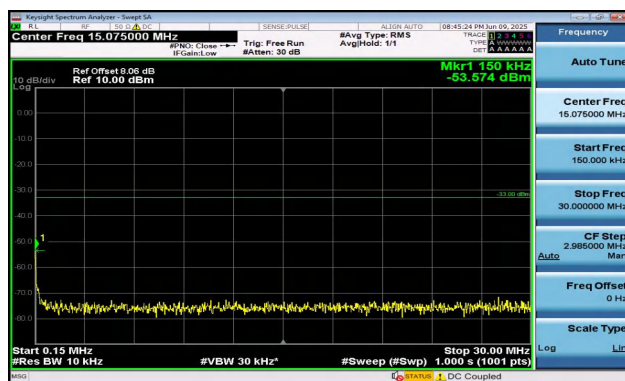
Band2-5MHz-QPSK-19175-25RB#0-0.15~30-PASS
