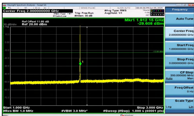
Band2-5MHz-QPSK-19175-1RB#24-1000~3000-PASS
