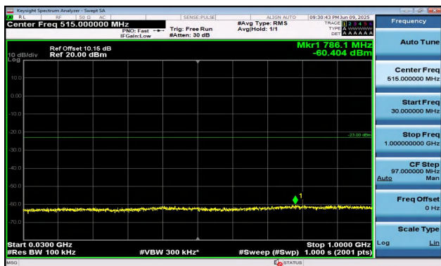
Band2-10MHz-QPSK-18650-50RB#0-30~1000-PASS
