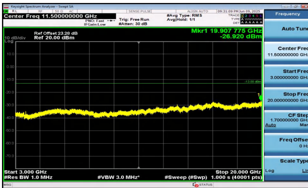
Band2-10MHz-QPSK-18650-50RB#0-3000~20000-PASS
