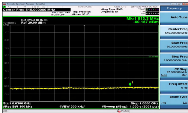
Band2-5MHz-QPSK-19175-25RB#0-30~1000-PASS
