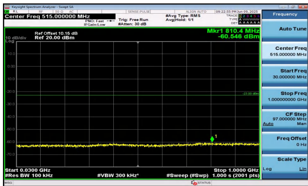
Band2-10MHz-16QAM-18650-1RB#49-30~1000-PASS
