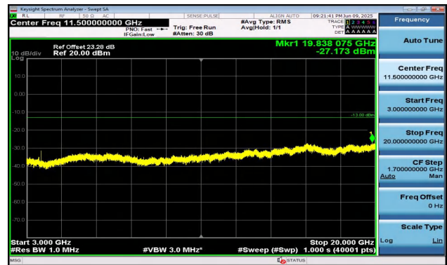
Band2-10MHz-16QAM-18650-1RB#0-3000~20000-PASS
