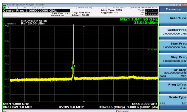
Band2-10MHz-QPSK-18650-1RB#49-1000~3000-PASS
