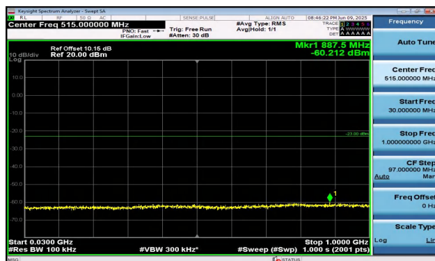
Band2-5MHz-16QAM-19175-25RB#0-30~1000-PASS
