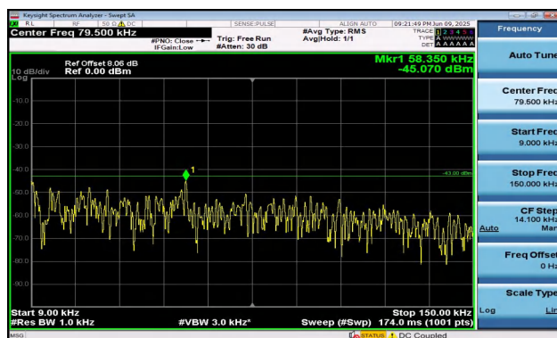
Band2-10MHz-QPSK-18650-1RB#49-0.009~0.15-PASS
