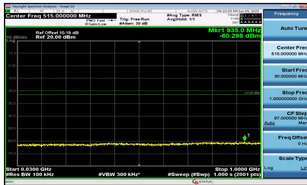
Band2-10MHz-QPSK-18650-1RB#49-30~1000-PASS
