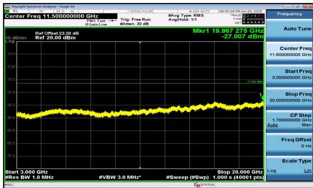
Band2-5MHz-16QAM-19175-1RB#24-3000~20000-PASS
