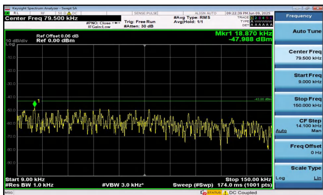
Band2-10MHz-16QAM-18650-1RB#49-0.009~0.15-PASS
