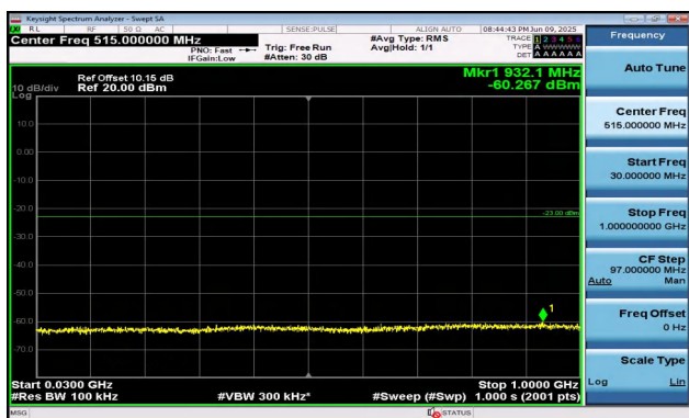
Band2-5MHz-16QAM-19175-1RB#24-30~1000-PASS
