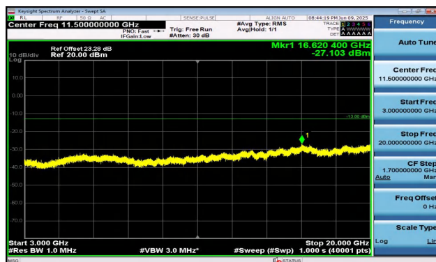
Band2-5MHz-QPSK-19175-1RB#24-3000~20000-PASS
