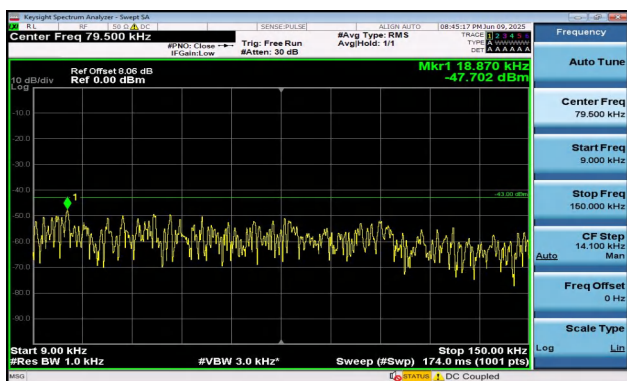
Band2-5MHz-QPSK-19175-25RB#0-0.009~0.15-PASS
