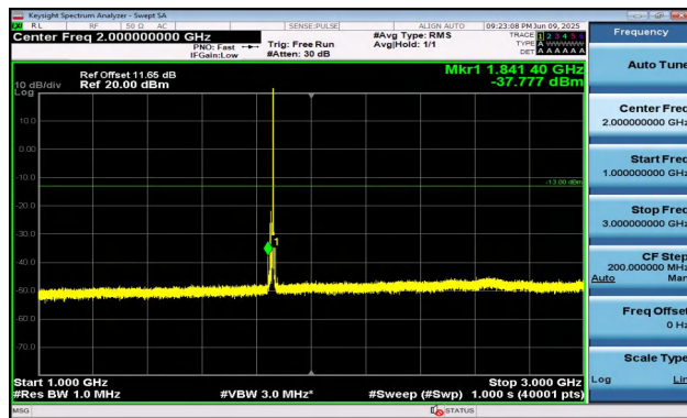
Band2-10MHz-16QAM-18650-1RB#49-1000~3000-PASS
