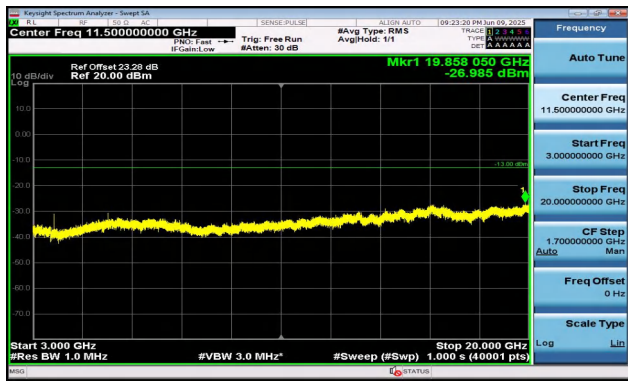
Band2-10MHz-16QAM-18650-1RB#49-3000~20000-PASS
