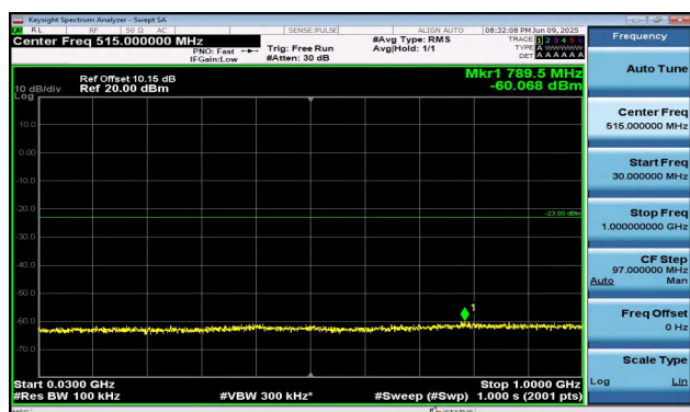
Band2-5MHz-QPSK-18625-1RB#0-30~1000-PASS
