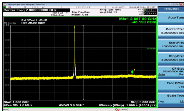
Band2-5MHz-QPSK-18900-25RB#0-1000~3000-PASS
