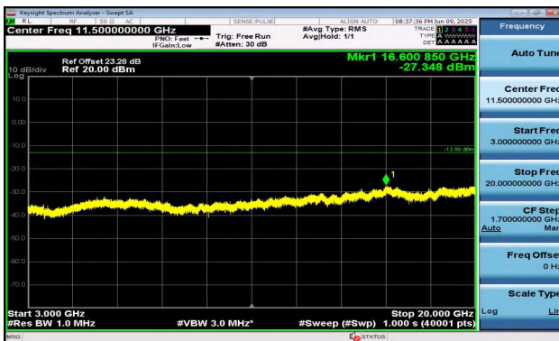
Band2-5MHz-QPSK-18900-1RB#0-3000~20000-PASS
