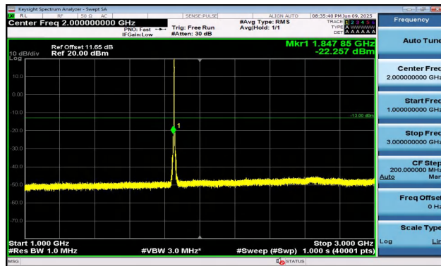
Band2-5MHz-QPSK-18625-25RB#0-1000~3000-PASS
