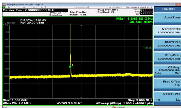
Band2-5MHz-QPSK-18625-1RB#24-1000~3000-PASS
