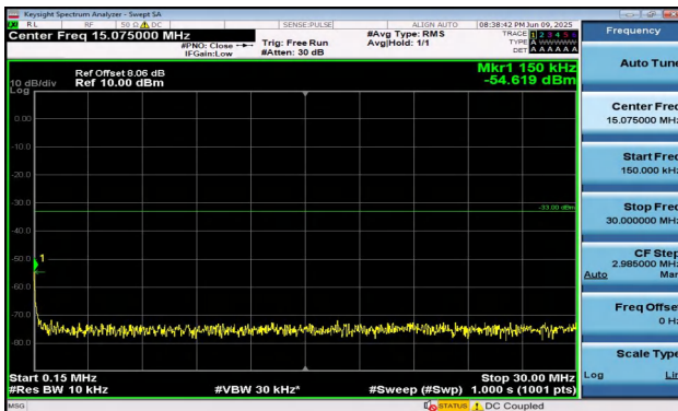
Band2-5MHz-QPSK-18900-1RB#24-0.15~30-PASS
