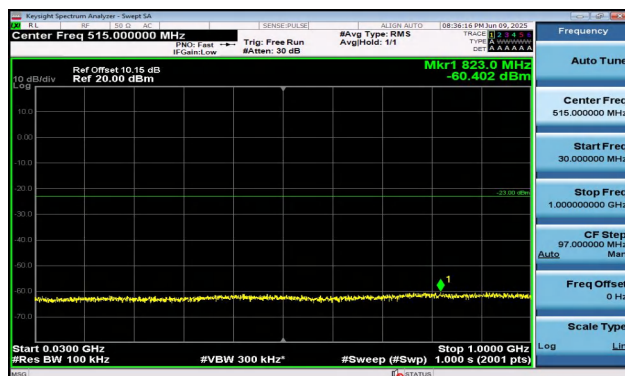
Band2-5MHz-16QAM-18625-25RB#0-30~1000-PASS
