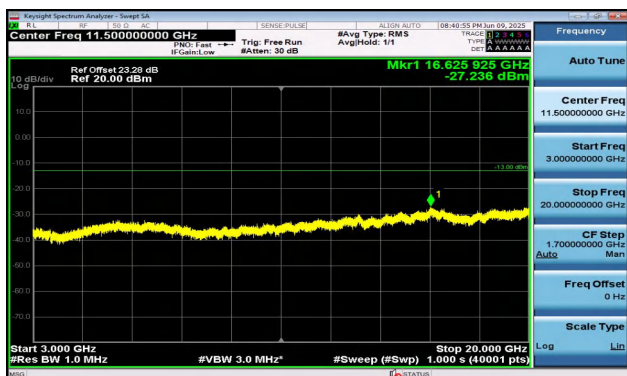
Band2-5MHz-QPSK-18900-25RB#0-3000~20000-PASS
