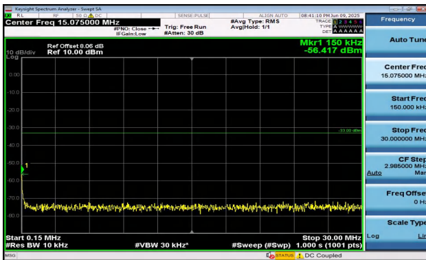
Band2-5MHz-16QAM-18900-25RB#0-0.15~30-PASS
