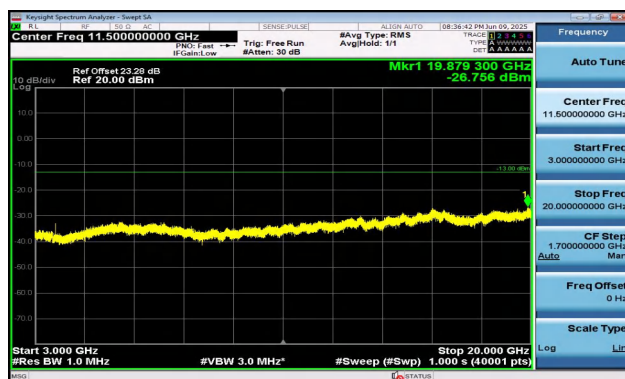
Band2-5MHz-16QAM-18625-25RB#0-3000~20000-PASS
