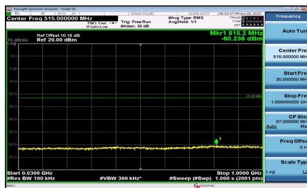
Band2-5MHz-QPSK-18625-1RB#24-30~1000-PASS
