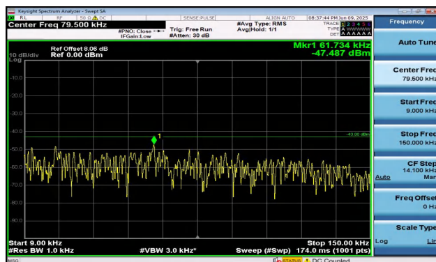
Band2-5MHz-16QAM-18900-1RB#0-0.009~0.15-PASS
