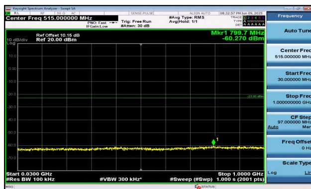
Band2-5MHz-16QAM-18625-1RB#0-30~1000-PASS
