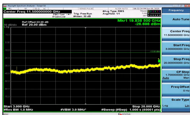
Band2-5MHz-QPSK-18625-1RB#0-3000~20000-PASS
