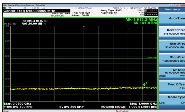
Band2-5MHz-16QAM-18900-1RB#0-30~1000-PASS
