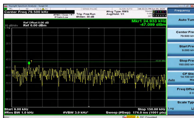
Band2-5MHz-QPSK-18625-1RB#24-0.009~0.15-PASS
