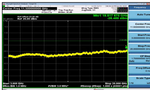
Band2-5MHz-QPSK-18900-1RB#24-3000~20000-PASS
