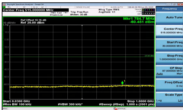
Band2-5MHz-QPSK-18900-25RB#0-30~1000-PASS
