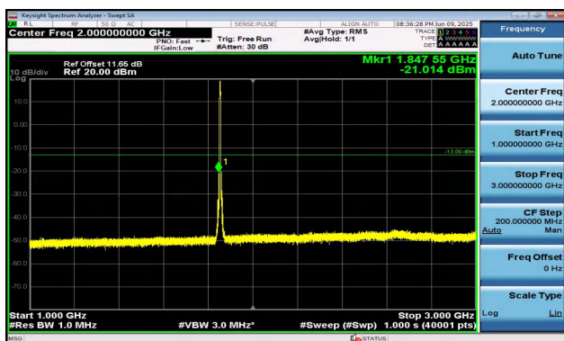
Band2-5MHz-16QAM-18625-25RB#0-1000~3000-PASS
