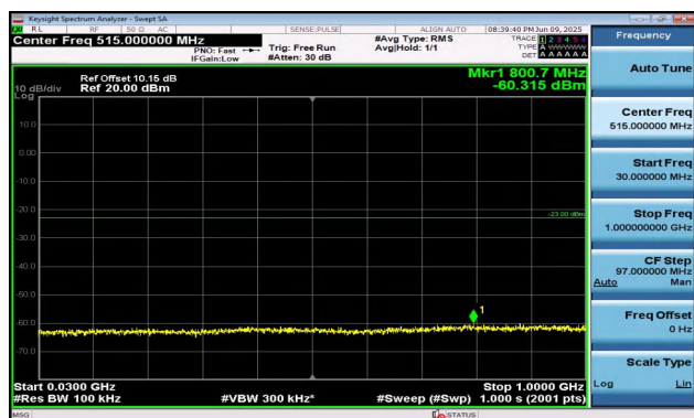
Band2-5MHz-16QAM-18900-1RB#24-30~1000-PASS
