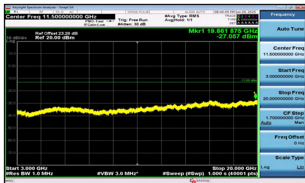
Band2-5MHz-16QAM-18900-1RB#24-3000~20000-PASS
