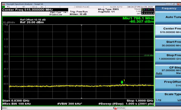
Band2-5MHz-16QAM-18625-1RB#24-30~1000-PASS
