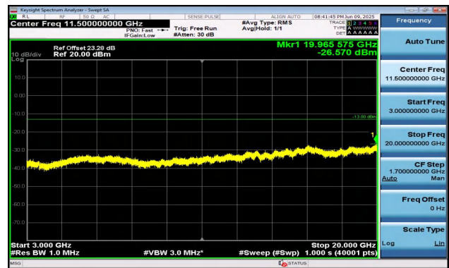
Band2-5MHz-16QAM-18900-25RB#0-3000~20000-PASS
