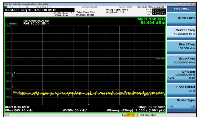
Band2-5MHz-16QAM-18625-1RB#24-0.15~30-PASS
