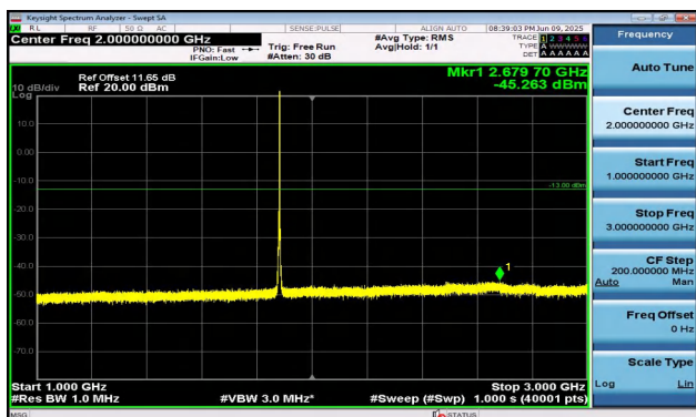
Band2-5MHz-QPSK-18900-1RB#24-1000~3000-PASS
