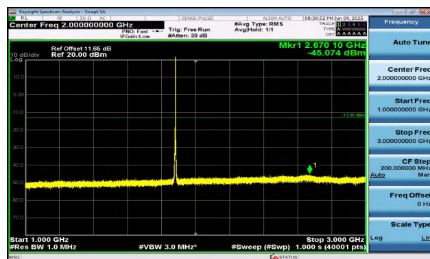
Band2-5MHz-16QAM-18900-1RB#24-1000~3000-PASS
