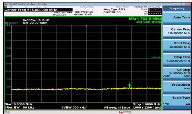
Band2-5MHz-16QAM-18900-25RB#0-30~1000-PASS
