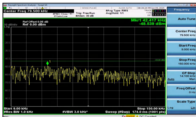
Band2-5MHz-16QAM-18900-1RB#24-0.009~0.15-PASS
