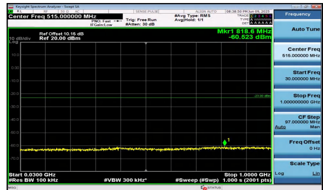
Band2-5MHz-QPSK-18900-1RB#24-30~1000-PASS
