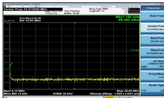
Band2-5MHz-16QAM-18900-1RB#24-0.15~30-PASS
