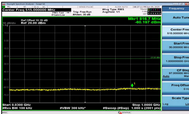
Band2-5MHz-QPSK-18900-1RB#0-30~1000-PASS
