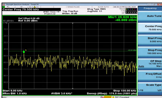
Band2-5MHz-QPSK-18625-25RB#0-0.009~0.15-PASS
