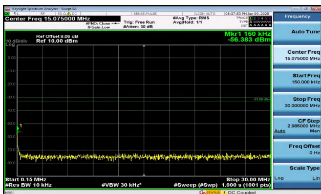
Band2-5MHz-16QAM-18900-1RB#0-0.15~30-PASS
