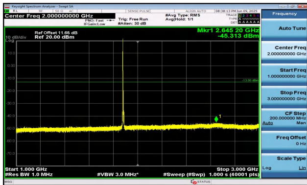
Band2-5MHz-16QAM-18900-1RB#0-1000~3000-PASS
