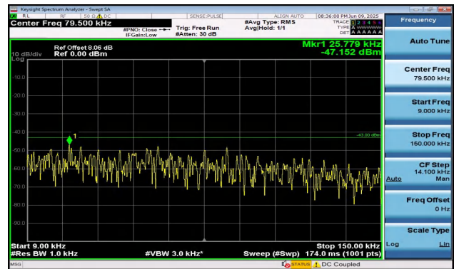
Band2-5MHz-16QAM-18625-25RB#0-0.009~0.15-PASS
