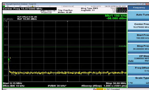
Band2-5MHz-QPSK-18625-25RB#0-0.15~30-PASS
