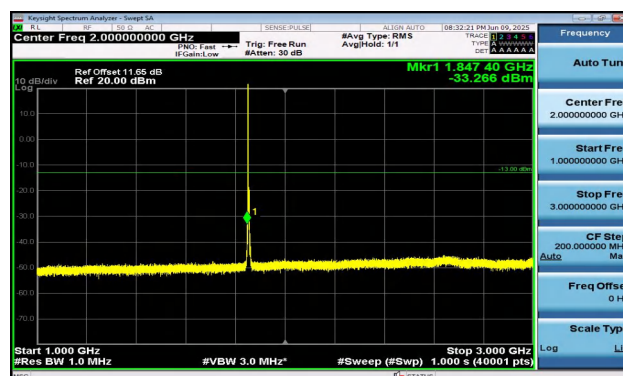
Band2-5MHz-QPSK-18625-1RB#0-1000~3000-PASS
