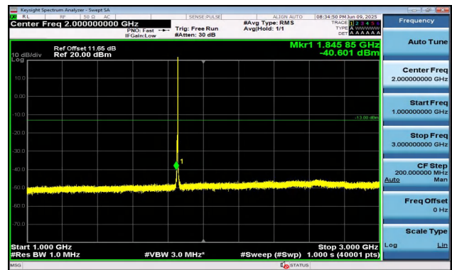
Band2-5MHz-16QAM-18625-1RB#24-1000~3000-PASS
