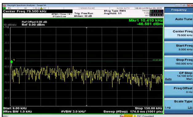
Band2-5MHz-QPSK-18900-25RB#0-0.009~0.15-PASS
