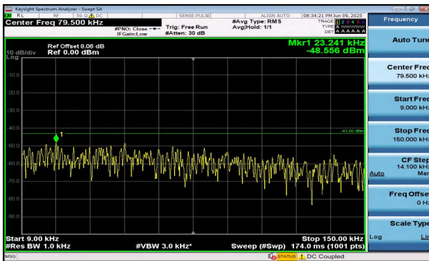
Band2-5MHz-16QAM-18625-1RB#24-0.009~0.15-PASS
