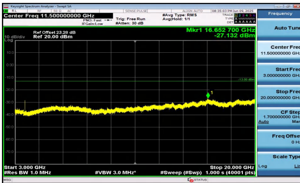
Band2-5MHz-16QAM-18625-1RB#24-3000~20000-PASS
