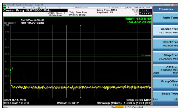
Band2-5MHz-QPSK-18900-25RB#0-0.15~30-PASS
