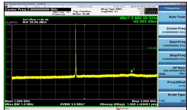
Band2-5MHz-QPSK-18900-1RB#0-1000~3000-PASS
