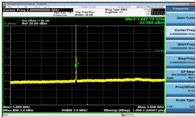
Band2-5MHz-16QAM-18625-1RB#0-1000~3000-PASS
