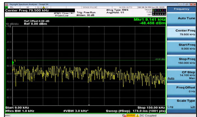
Band2-5MHz-QPSK-18900-1RB#24-0.009~0.15-PASS
