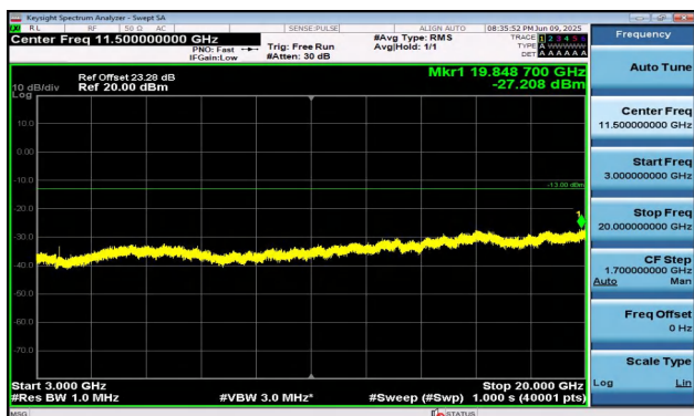
Band2-5MHz-QPSK-18625-25RB#0-3000~20000-PASS
