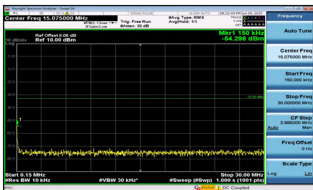
Band2-5MHz-16QAM-18625-1RB#0-0.15~30-PASS
