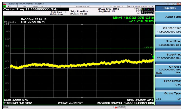
Band2-5MHz-16QAM-18625-1RB#0-3000~20000-PASS
