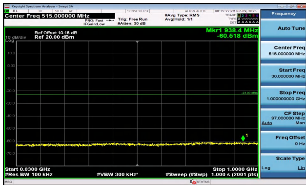
Band2-5MHz-QPSK-18625-25RB#0-30~1000-PASS
