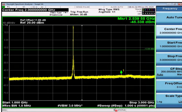
Band2-5MHz-16QAM-18900-25RB#0-1000~3000-PASS
