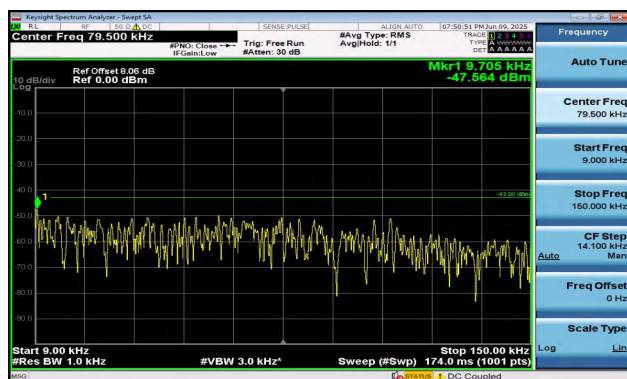
Band2-3MHz-QPSK-18900-15RB#0-0.009~0.15-PASS
