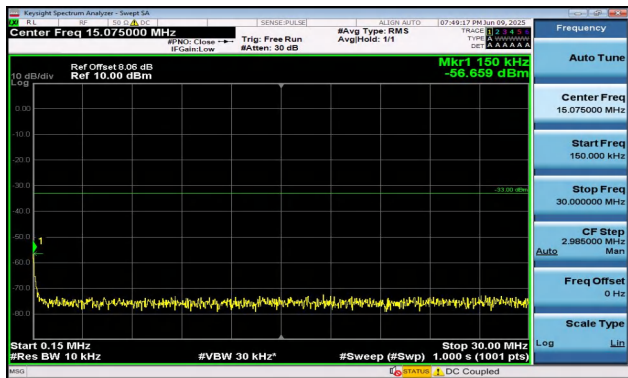
Band2-3MHz-QPSK-18900-1RB#14-0.15~30-PASS
