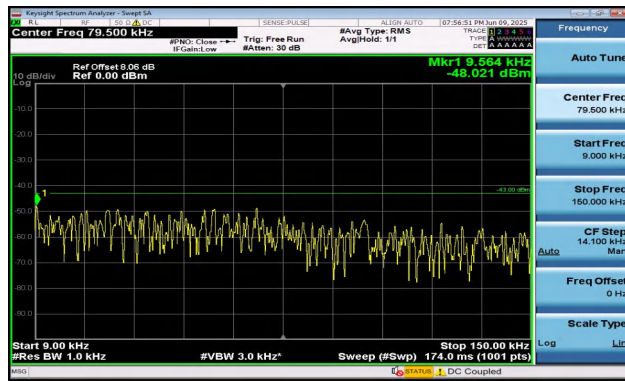
Band2-3MHz-16QAM-19185-15RB#0-0.009~0.15-PASS
