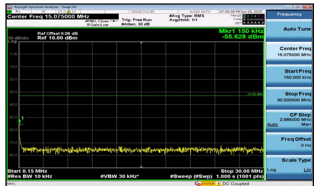
Band2-3MHz-QPSK-19185-15RB#0-0.15~30-PASS
