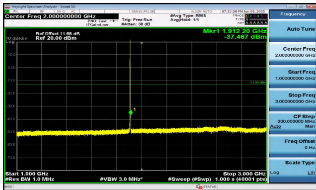
Band2-3MHz-16QAM-19185-1RB#0-1000~3000-PASS
