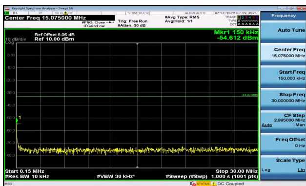
Band2-3MHz-16QAM-19185-1RB#0-0.15~30-PASS
