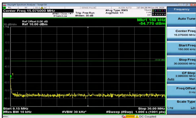
Band2-3MHz-QPSK-19185-1RB#14-0.15~30-PASS
