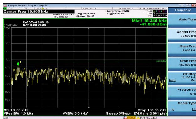
Band2-3MHz-QPSK-19185-1RB#14-0.009~0.15-PASS
