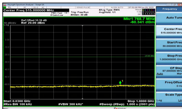
Band2-3MHz-16QAM-18900-15RB#0-30~1000-PASS
