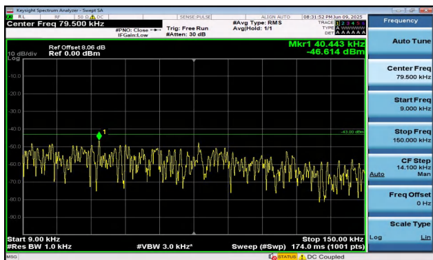
Band2-5MHz-QPSK-18625-1RB#0-0.009~0.15-PASS
