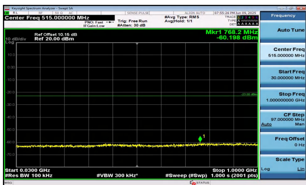
Band2-3MHz-16QAM-19185-1RB#14-30~1000-PASS
