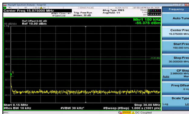
Band2-3MHz-16QAM-19185-1RB#14-0.15~30-PASS
