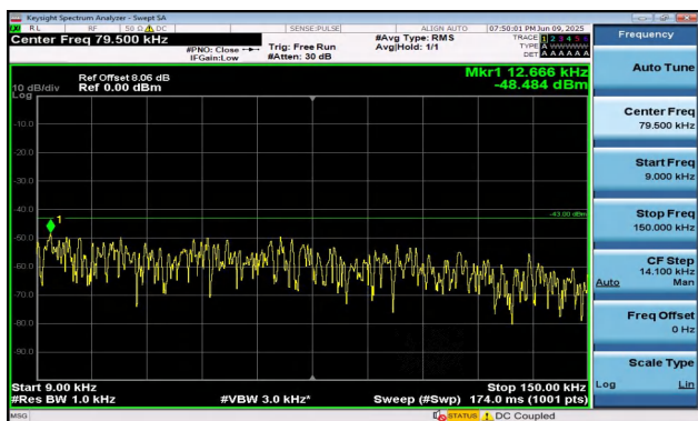
Band2-3MHz-16QAM-18900-1RB#14-0.009~0.15-PASS
