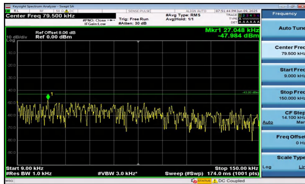
Band2-3MHz-16QAM-18900-15RB#0-0.009~0.15-PASS
