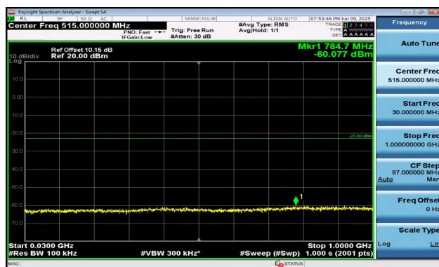
Band2-3MHz-16QAM-19185-1RB#0-30~1000-PASS
