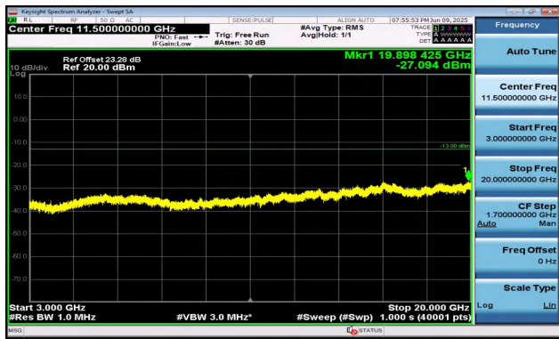
Band2-3MHz-16QAM-19185-1RB#14-3000~20000-PASS
