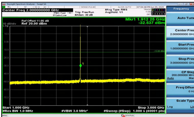
Band2-3MHz-QPSK-19185-1RB#14-1000~3000-PASS
