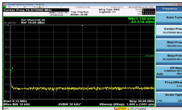
Band2-5MHz-QPSK-18625-1RB#0-0.15~30-PASS
