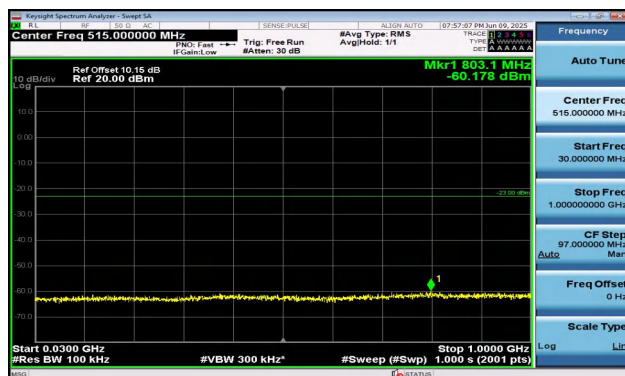
Band2-3MHz-16QAM-19185-15RB#0-30~1000-PASS
