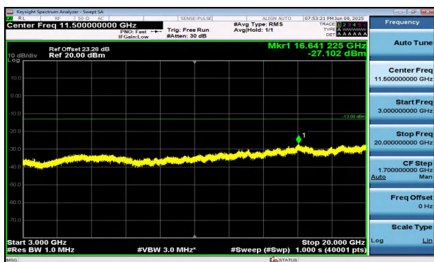
Band2-3MHz-QPSK-19185-1RB#0-3000~20000-PASS
