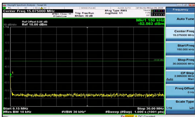
Band2-3MHz-16QAM-18900-15RB#0-0.15~30-PASS
