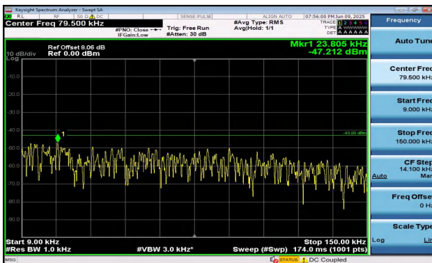
Band2-3MHz-QPSK-19185-15RB#0-0.009~0.15-PASS
