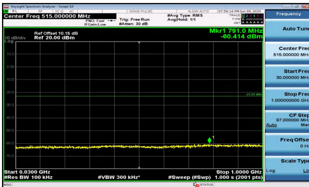
Band2-3MHz-QPSK-19185-15RB#0-30~1000-PASS
