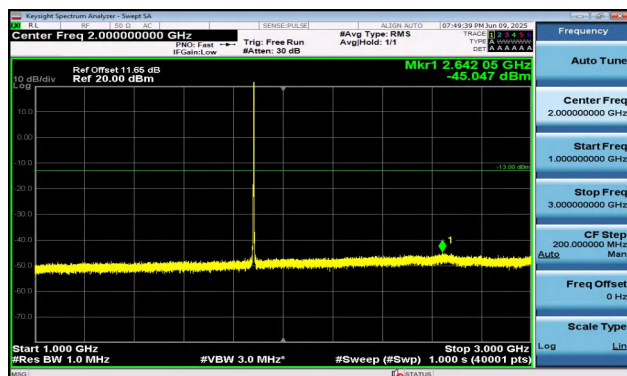
Band2-3MHz-QPSK-18900-1RB#14-1000~3000-PASS
