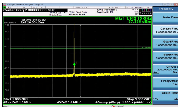
Band2-3MHz-QPSK-19185-1RB#0-1000~3000-PASS
