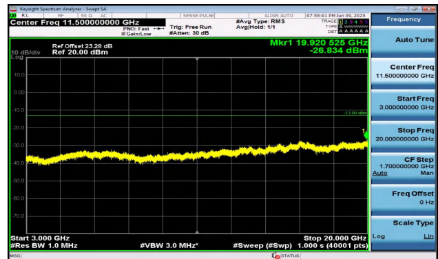
Band2-3MHz-QPSK-19185-1RB#14-3000~20000-PASS
