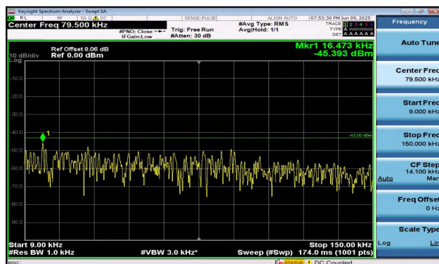
Band2-3MHz-16QAM-19185-1RB#0-0.009~0.15-PASS
