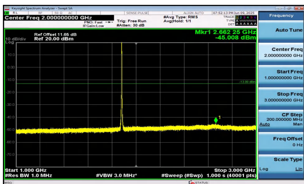
Band2-3MHz-16QAM-18900-15RB#0-1000~3000-PASS
