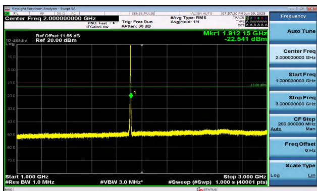
Band2-3MHz-16QAM-19185-15RB#0-1000~3000-PASS
