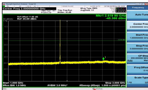
Band2-3MHz-16QAM-18900-1RB#14-1000~3000-PASS
