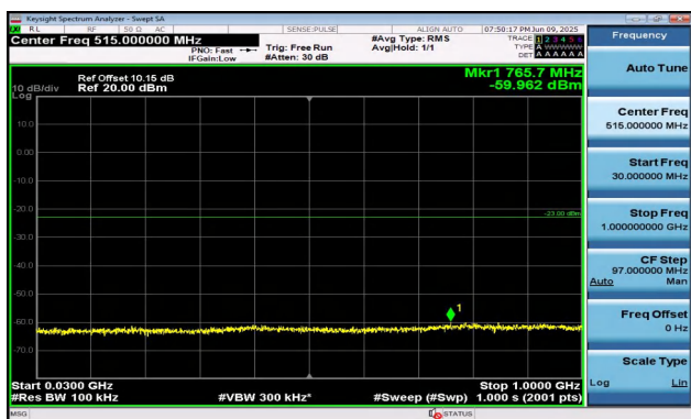
Band2-3MHz-16QAM-18900-1RB#14-30~1000-PASS
