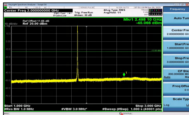
Band2-3MHz-QPSK-18900-15RB#0-1000~3000-PASS
