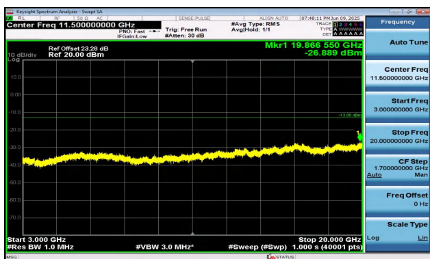
Band2-3MHz-QPSK-18900-1RB#0-3000~20000-PASS
