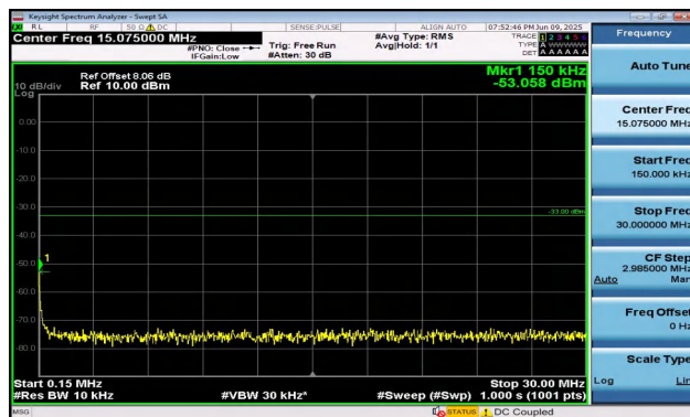
Band2-3MHz-QPSK-19185-1RB#0-0.15~30-PASS
