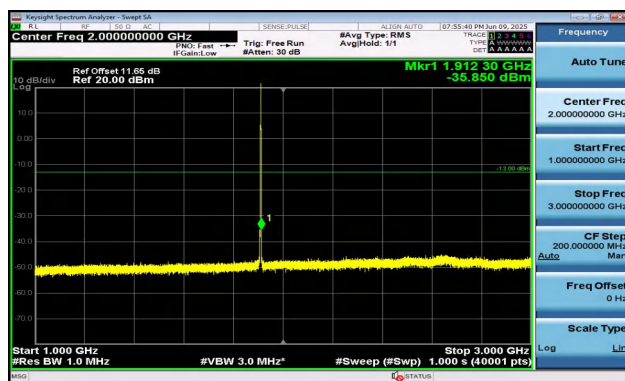
Band2-3MHz-16QAM-19185-1RB#14-1000~3000-PASS
