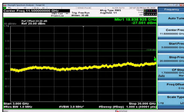
Band2-3MHz-16QAM-19185-15RB#0-3000~20000-PASS
