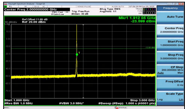
Band2-3MHz-QPSK-19185-15RB#0-1000~3000-PASS
