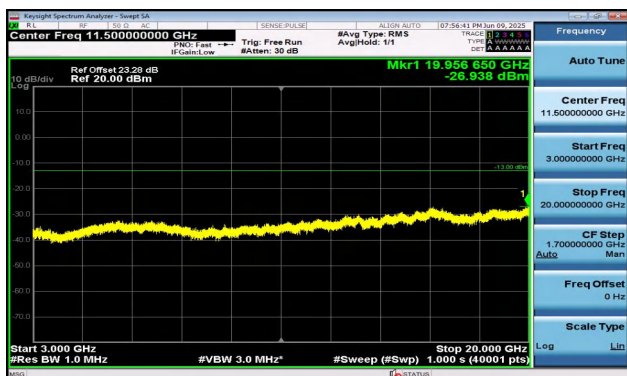
Band2-3MHz-QPSK-19185-15RB#0-3000~20000-PASS
