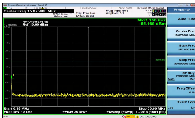
Band2-3MHz-16QAM-18900-1RB#14-0.15~30-PASS
