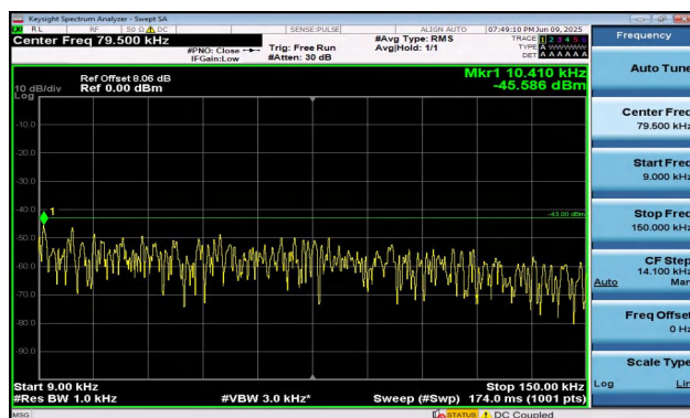
Band2-3MHz-QPSK-18900-1RB#14-0.009~0.15-PASS
