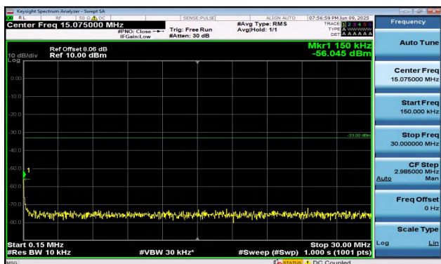
Band2-3MHz-16QAM-19185-15RB#0-0.15~30-PASS
