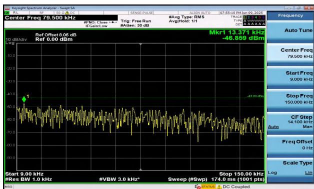
Band2-3MHz-16QAM-19185-1RB#14-0.009~0.15-PASS
