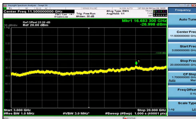
Band2-3MHz-16QAM-18900-15RB#0-3000~20000-PASS
