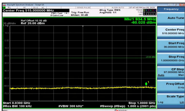
Band2-3MHz-QPSK-18900-1RB#0-30~1000-PASS
