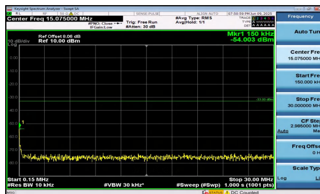
Band2-3MHz-QPSK-18900-15RB#0-0.15~30-PASS
