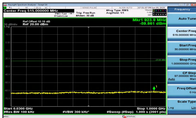
Band2-3MHz-QPSK-18900-15RB#0-30~1000-PASS
