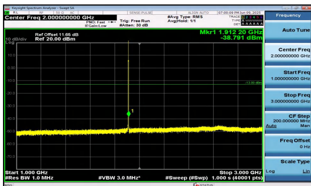
Band2-1.4MHz-QPSK-19193-1RB#5-1000~3000-PASS
