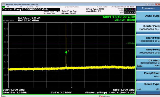
Band2-1.4MHz-16QAM-19193-6RB#0-1000~3000-PASS
