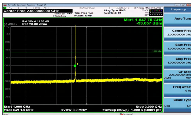
Band2-3MHz-QPSK-18615-1RB#0-1000~3000-PASS
