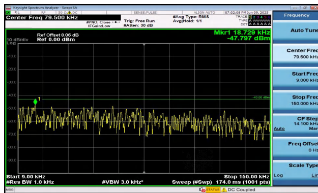
Band2-1.4MHz-16QAM-19193-6RB#0-0.009~0.15-PASS
