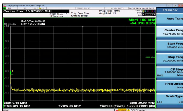
Band2-1.4MHz-16QAM-19193-1RB#0-0.15~30-PASS
