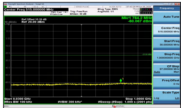
Band2-3MHz-16QAM-18615-1RB#0-30~1000-PASS
