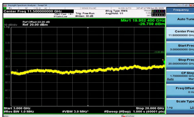
Band2-3MHz-16QAM-18615-15RB#0-3000~20000-PASS
