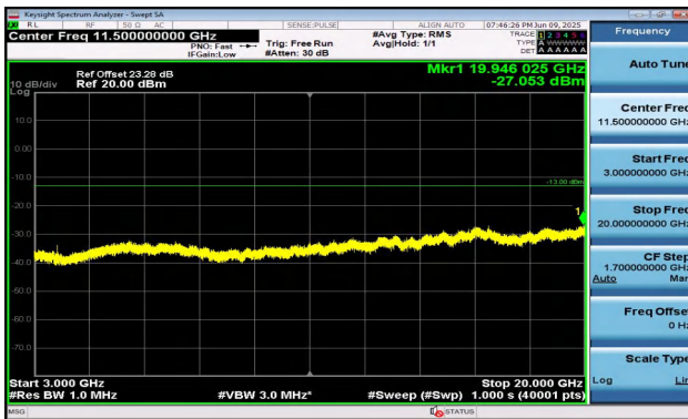
Band2-3MHz-QPSK-18615-15RB#0-3000~20000-PASS
