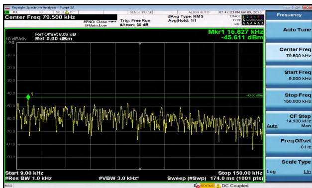
Band2-3MHz-QPSK-18615-1RB#0-0.009~0.15-PASS
