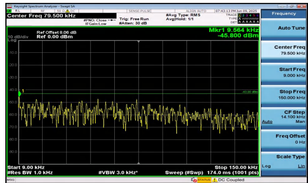
Band2-3MHz-16QAM-18615-1RB#0-0.009~0.15-PASS
