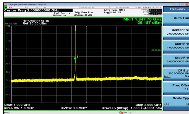
Band2-3MHz-QPSK-18615-15RB#0-1000~3000-PASS
