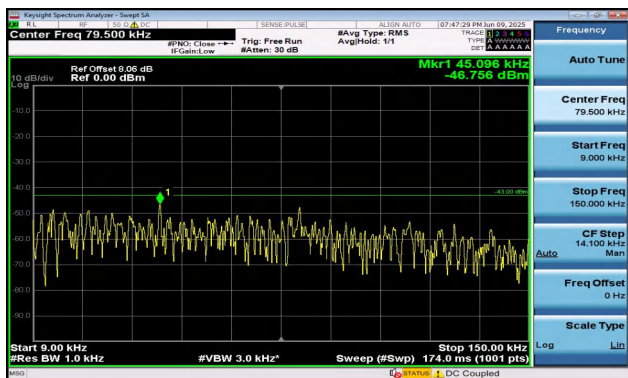
Band2-3MHz-QPSK-18900-1RB#0-0.009~0.15-PASS
