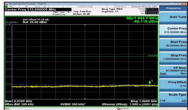
Band2-1.4MHz-QPSK-19193-1RB#5-30~1000-PASS
