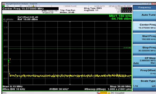
Band2-3MHz-QPSK-18615-1RB#14-0.15~30-PASS
