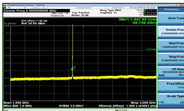
Band2-3MHz-16QAM-18615-1RB#14-1000~3000-PASS
