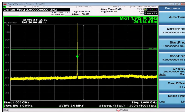
Band2-1.4MHz-QPSK-19193-6RB#0-1000~3000-PASS
