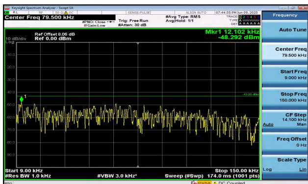
Band2-3MHz-16QAM-18615-1RB#14-0.009~0.15-PASS
