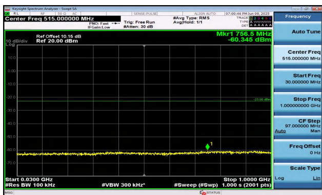
Band2-1.4MHz-16QAM-19193-1RB#5-30~1000-PASS
