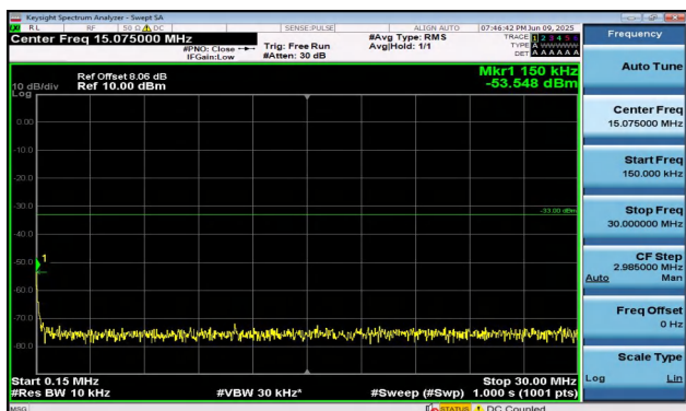
Band2-3MHz-16QAM-18615-15RB#0-0.15~30-PASS
