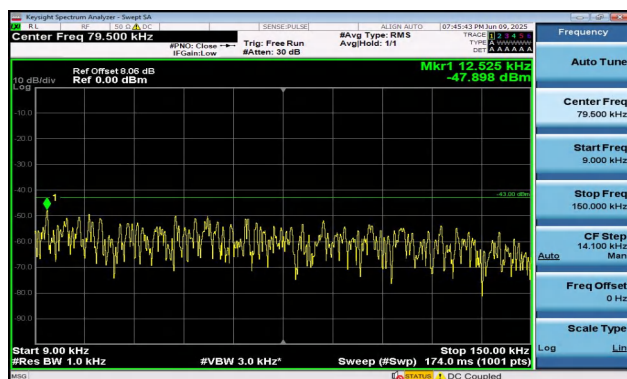
Band2-3MHz-QPSK-18615-15RB#0-0.009~0.15-PASS
