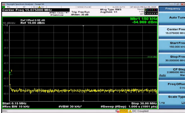
Band2-3MHz-16QAM-18615-1RB#0-0.15~30-PASS
