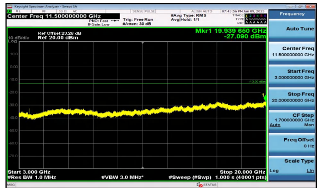
Band2-3MHz-16QAM-18615-1RB#0-3000~20000-PASS
