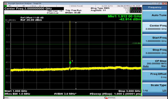
Band2-1.4MHz-QPSK-19193-1RB#0-1000~3000-PASS
