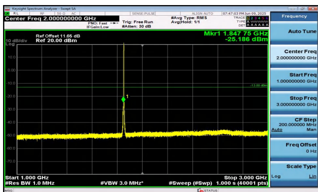
Band2-3MHz-16QAM-18615-15RB#0-1000~3000-PASS
