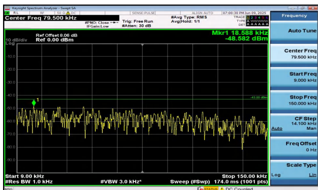
Band2-1.4MHz-16QAM-19193-1RB#5-0.009~0.15-PASS
