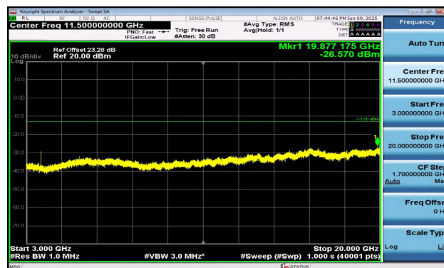
Band2-3MHz-QPSK-18615-1RB#14-3000~20000-PASS
