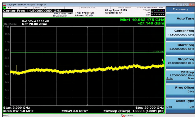
Band2-3MHz-16QAM-18615-1RB#14-3000~20000-PASS
