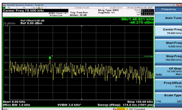
Band2-1.4MHz-QPSK-19193-6RB#0-0.009~0.15-PASS
