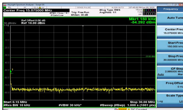
Band2-3MHz-16QAM-18615-1RB#14-0.15~30-PASS
