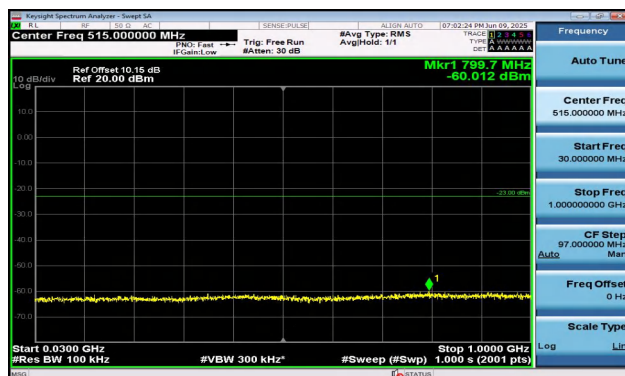
Band2-1.4MHz-16QAM-19193-6RB#0-30~1000-PASS
