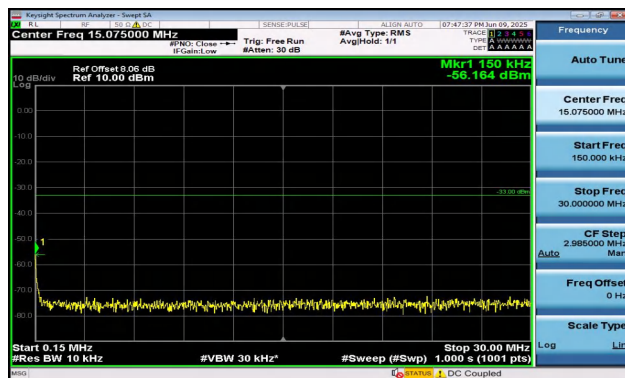
Band2-3MHz-QPSK-18900-1RB#0-0.15~30-PASS
