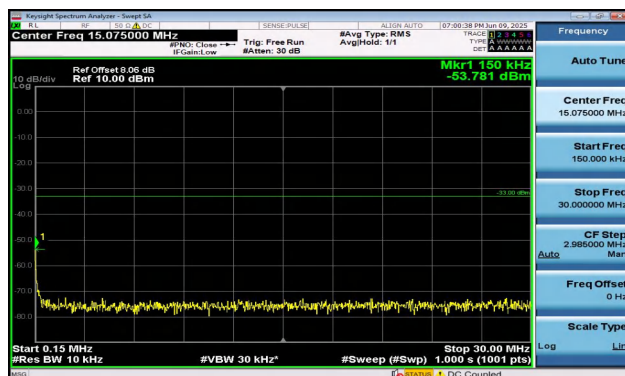
Band2-1.4MHz-16QAM-19193-1RB#5-0.15~30-PASS
