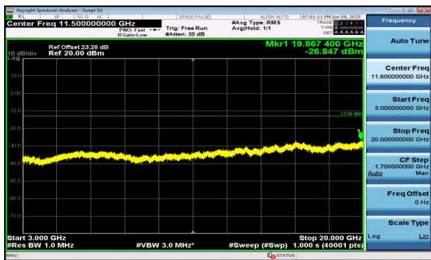
Band2-1.4MHz-16QAM-19193-1RB#5-3000~20000-PASS
