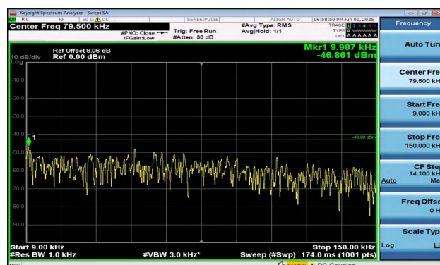
Band2-1.4MHz-16QAM-19193-1RB#0-0.009~0.15-PASS
