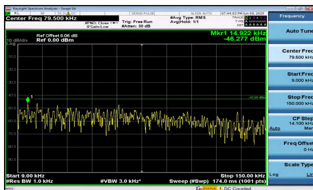
Band2-3MHz-QPSK-18615-1RB#14-0.009~0.15-PASS
