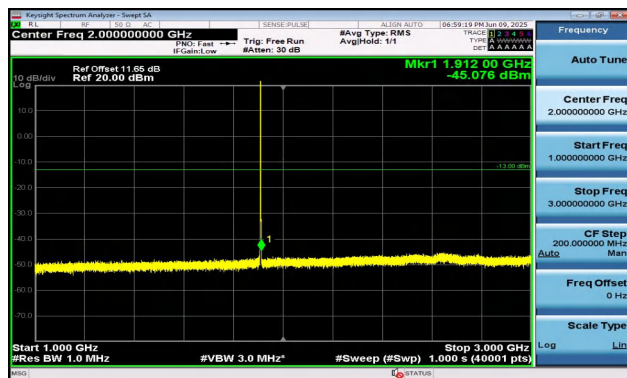
Band2-1.4MHz-16QAM-19193-1RB#0-1000~3000-PASS
