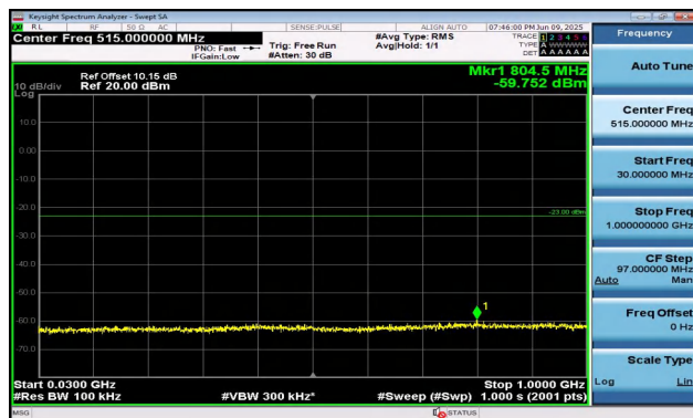
Band2-3MHz-QPSK-18615-15RB#0-30~1000-PASS
