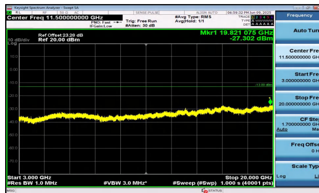
Band2-1.4MHz-16QAM-19193-1RB#0-3000~20000-PASS
