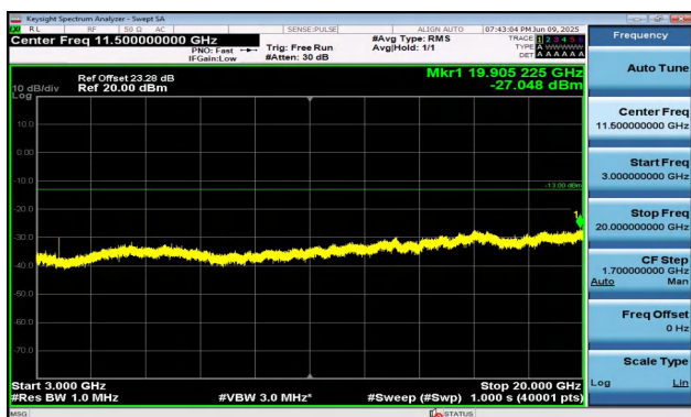
Band2-3MHz-QPSK-18615-1RB#0-3000~20000-PASS
