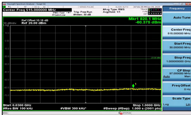
Band2-1.4MHz-QPSK-19193-6RB#0-30~1000-PASS
