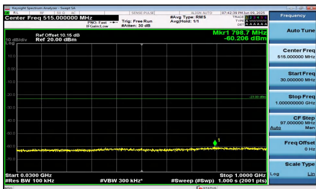
Band2-3MHz-QPSK-18615-1RB#0-30~1000-PASS
