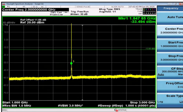
Band2-3MHz-16QAM-18615-1RB#0-1000~3000-PASS
