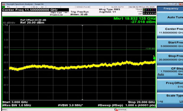
Band2-1.4MHz-QPSK-19193-1RB#0-3000~20000-PASS
