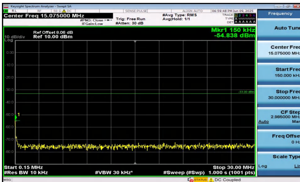
Band2-1.4MHz-QPSK-19193-1RB#5-0.15~30-PASS
