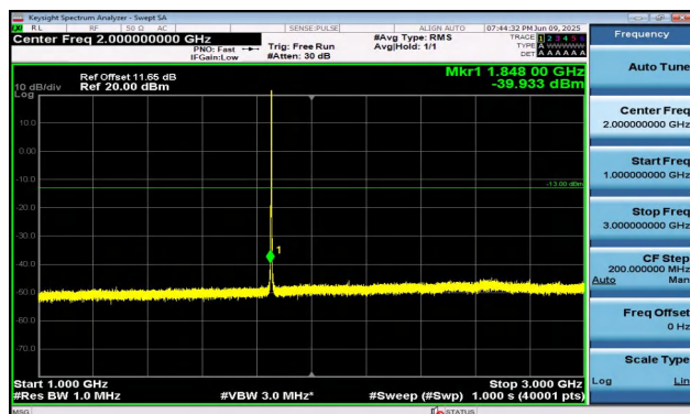
Band2-3MHz-QPSK-18615-1RB#14-1000~3000-PASS
