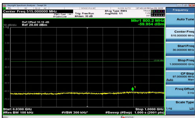
Band2-3MHz-16QAM-18615-1RB#14-30~1000-PASS
