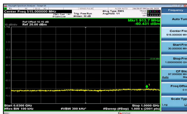
Band2-1.4MHz-16QAM-19193-1RB#0-30~1000-PASS
