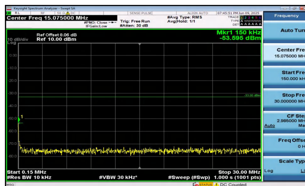
Band2-3MHz-QPSK-18615-15RB#0-0.15~30-PASS
