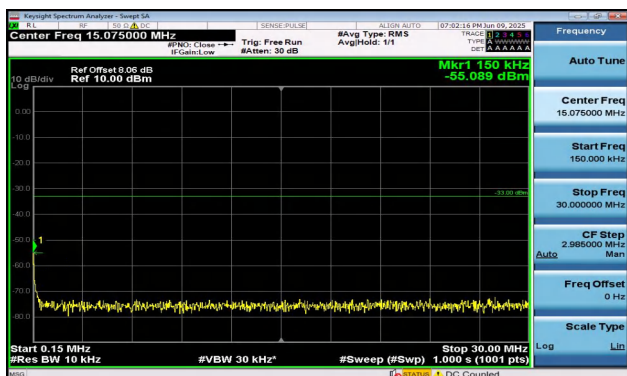
Band2-1.4MHz-16QAM-19193-6RB#0-0.15~30-PASS
