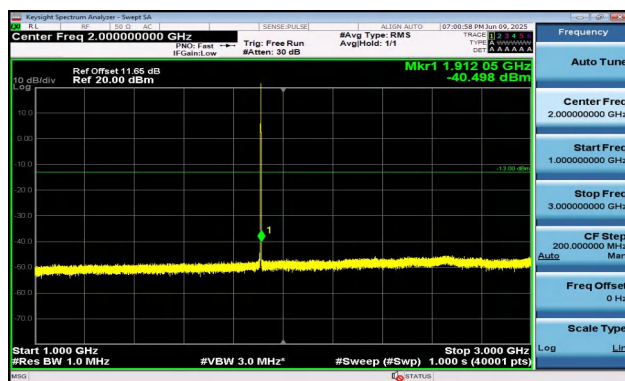
Band2-1.4MHz-16QAM-19193-1RB#5-1000~3000-PASS
