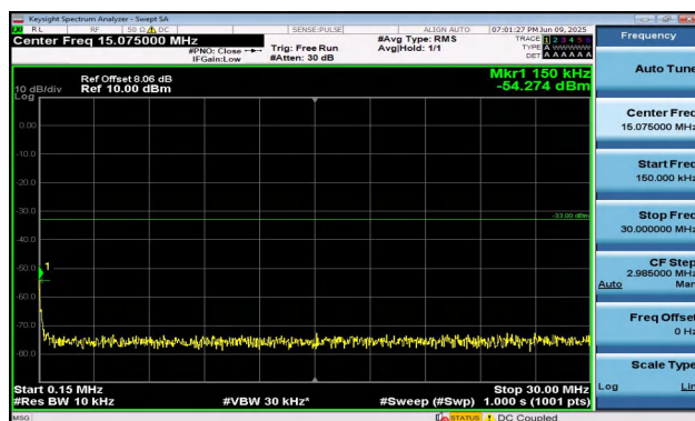
Band2-1.4MHz-QPSK-19193-6RB#0-0.15~30-PASS
