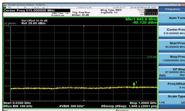
Band2-3MHz-16QAM-18615-15RB#0-30~1000-PASS
