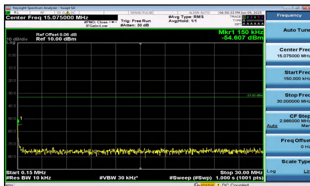
Band2-1.4MHz-16QAM-18607-1RB#5-0.15~30-PASS
