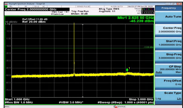
Band2-1.4MHz-QPSK-18900-1RB#0-1000~3000-PASS
