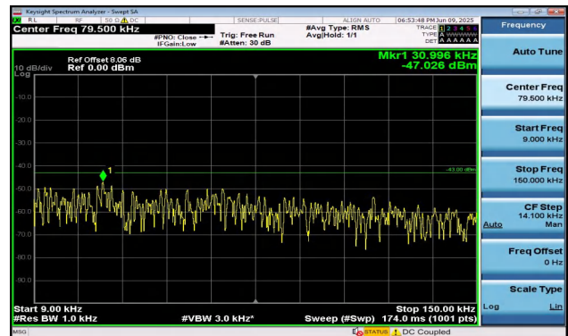
Band2-1.4MHz-16QAM-18900-1RB#0-0.009~0.15-PASS
