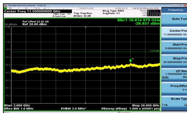
Band2-1.4MHz-QPSK-18900-1RB#5-3000~20000-PASS
