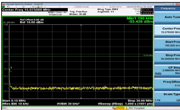
Band2-1.4MHz-16QAM-18900-1RB#0-0.15~30-PASS
