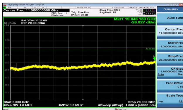
Band2-1.4MHz-QPSK-18607-1RB#5-3000~20000-PASS
