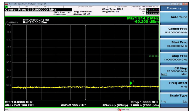
Band2-1.4MHz-QPSK-18900-1RB#5-30~1000-PASS
