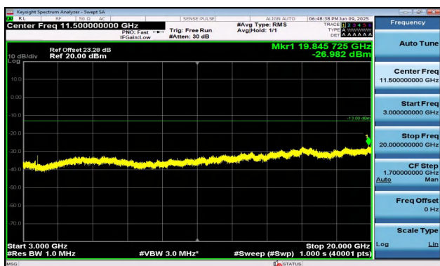
Band2-1.4MHz-QPSK-18607-1RB#0-3000~20000-PASS
