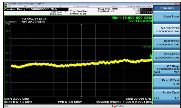
Band2-1.4MHz-16QAM-18900-1RB#0-3000~20000-PASS
