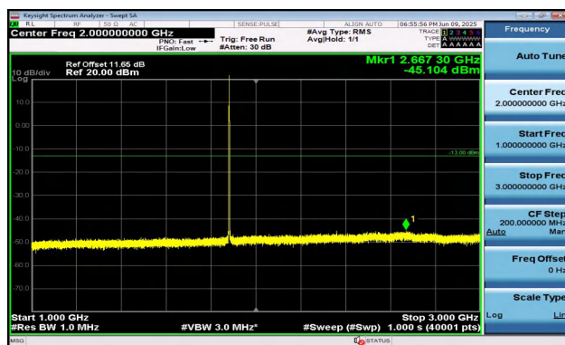
Band2-1.4MHz-16QAM-18900-1RB#5-1000~3000-PASS
