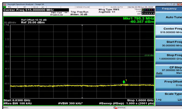
Band2-1.4MHz-QPSK-18900-6RB#0-30~1000-PASS
