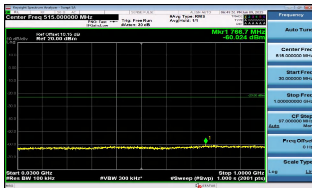
Band2-1.4MHz-QPSK-18607-1RB#5-30~1000-PASS
