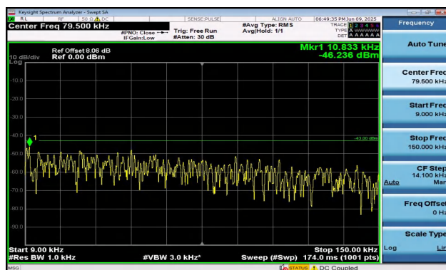
Band2-1.4MHz-QPSK-18607-1RB#5-0.009~0.15-PASS
