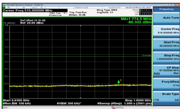
Band2-1.4MHz-16QAM-18900-1RB#5-30~1000-PASS
