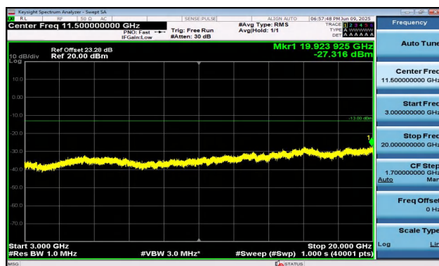
Band2-1.4MHz-16QAM-18900-6RB#0-3000~20000-PASS
