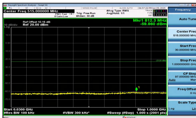
Band2-1.4MHz-16QAM-18900-6RB#0-30~1000-PASS
