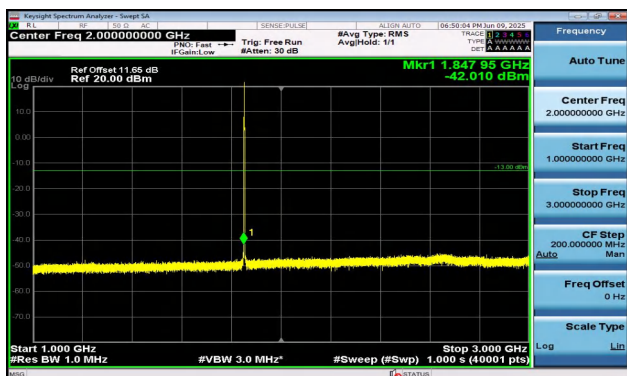
Band2-1.4MHz-QPSK-18607-1RB#5-1000~3000-PASS
