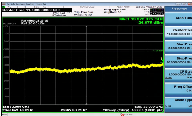
Band2-1.4MHz-QPSK-18900-6RB#0-3000~20000-PASS
