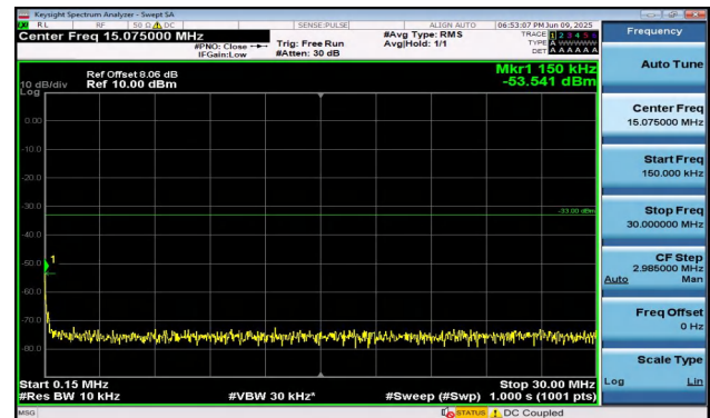
Band2-1.4MHz-QPSK-18900-1RB#0-0.15~30-PASS
