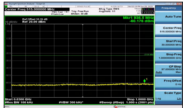
Band2-1.4MHz-16QAM-18607-6RB#0-30~1000-PASS
