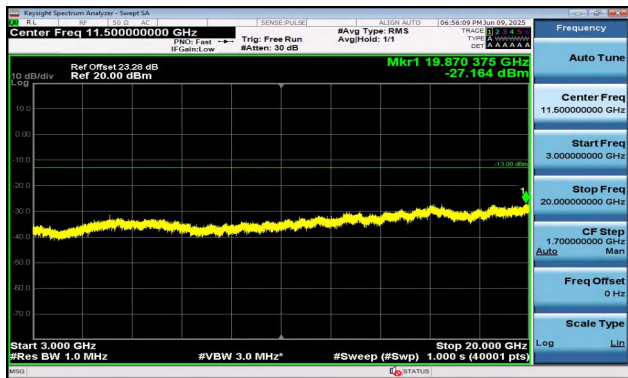
Band2-1.4MHz-16QAM-18900-1RB#5-3000~20000-PASS
