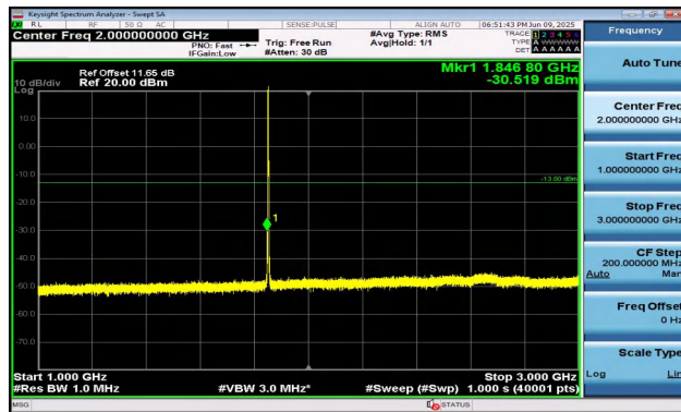
Band2-1.4MHz-QPSK-18607-6RB#0-1000~3000-PASS
