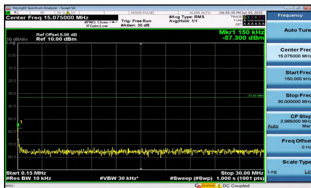
Band2-1.4MHz-16QAM-18900-1RB#5-0.15~30-PASS
