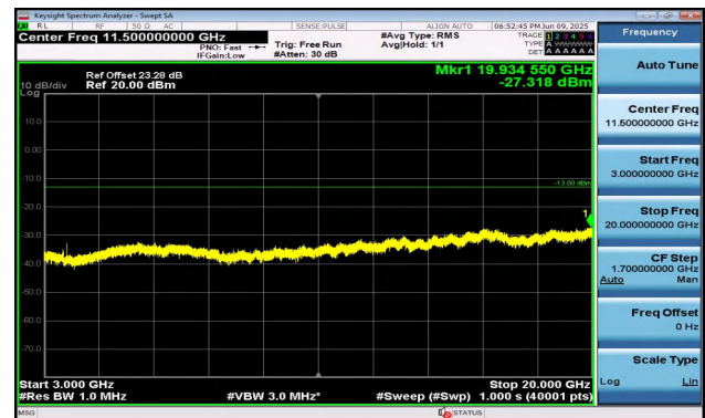
Band2-1.4MHz-16QAM-18607-6RB#0-3000~20000-PASS
