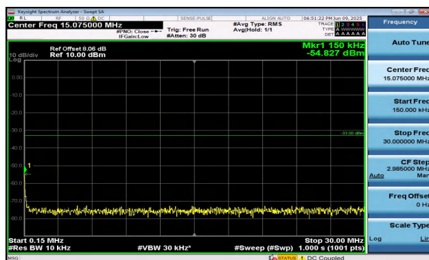
Band2-1.4MHz-QPSK-18607-6RB#0-0.15~30-PASS
