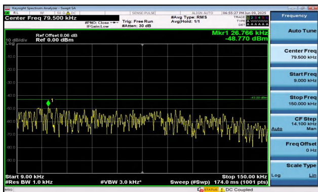
Band2-1.4MHz-16QAM-18900-1RB#5-0.009~0.15-PASS
