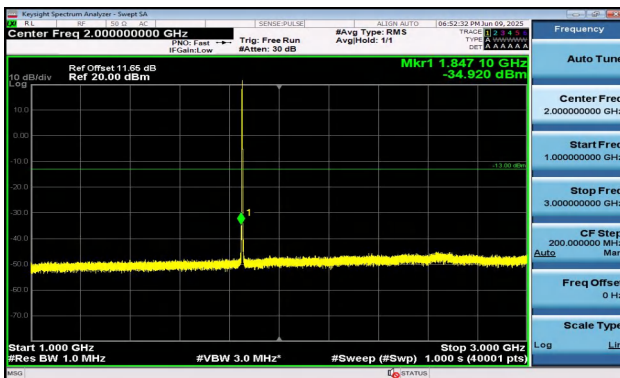
Band2-1.4MHz-16QAM-18607-6RB#0-1000~3000-PASS
