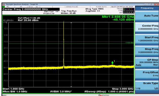
Band2-1.4MHz-16QAM-18900-6RB#0-1000~3000-PASS
