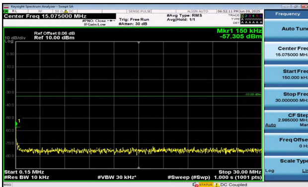
Band2-1.4MHz-16QAM-18607-6RB#0-0.15~30-PASS
