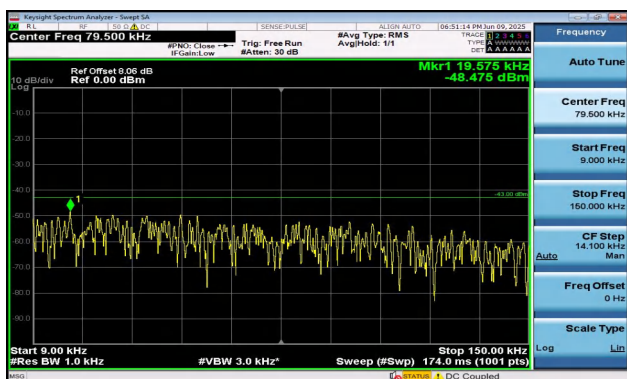
Band2-1.4MHz-QPSK-18607-6RB#0-0.009~0.15-PASS
