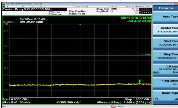
Band2-1.4MHz-QPSK-18900-1RB#0-30~1000-PASS
