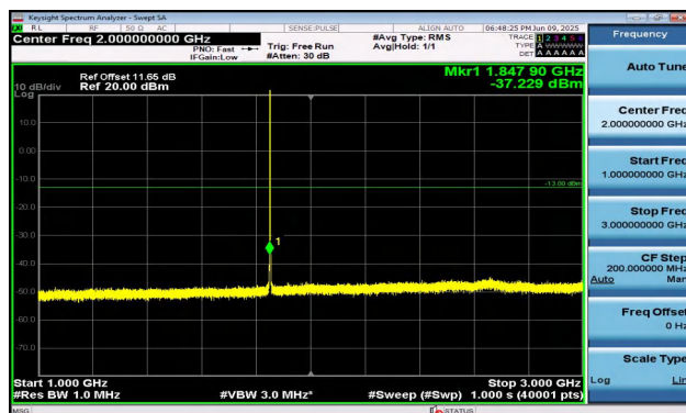
Band2-1.4MHz-QPSK-18607-1RB#0-1000~3000-PASS
