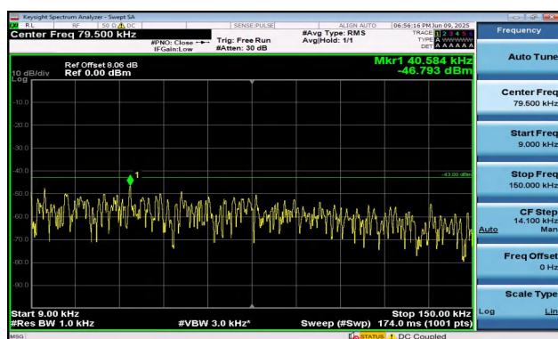
Band2-1.4MHz-QPSK-18900-6RB#0-0.009~0.15-PASS
