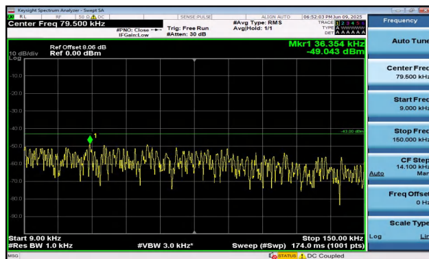
Band2-1.4MHz-16QAM-18607-6RB#0-0.009~0.15-PASS
