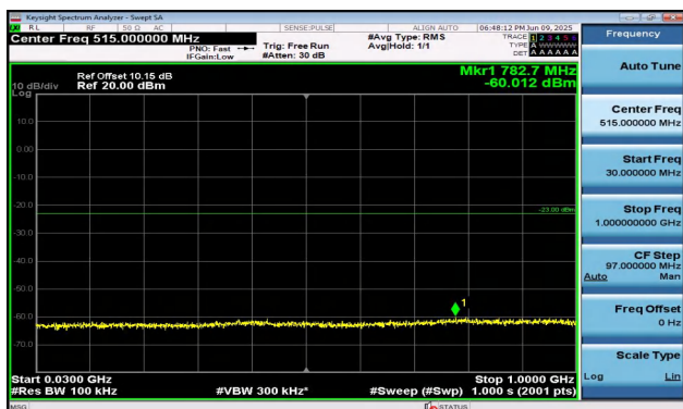
Band2-1.4MHz-QPSK-18607-1RB#0-30~1000-PASS
