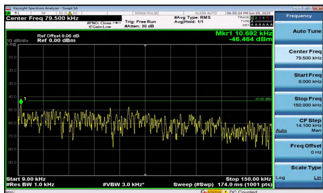
Band2-1.4MHz-16QAM-18607-1RB#5-0.009~0.15-PASS
