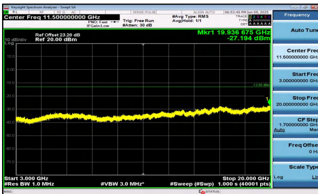
Band2-1.4MHz-QPSK-18900-1RB#0-3000~20000-PASS
