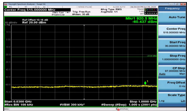
Band2-1.4MHz-16QAM-18900-1RB#0-30~1000-PASS
