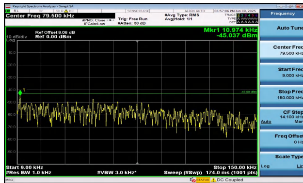
Band2-1.4MHz-16QAM-18900-6RB#0-0.009~0.15-PASS
