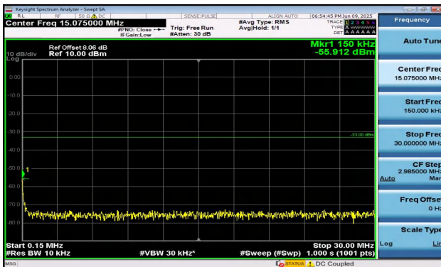
Band2-1.4MHz-QPSK-18900-1RB#5-0.15~30-PASS
