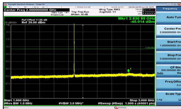
Band2-1.4MHz-QPSK-18900-6RB#0-1000~3000-PASS
