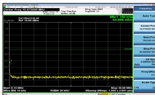
Band2-1.4MHz-QPSK-18900-6RB#0-0.15~30-PASS
