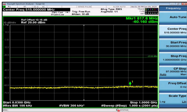
Band2-1.4MHz-QPSK-18607-6RB#0-30~1000-PASS
