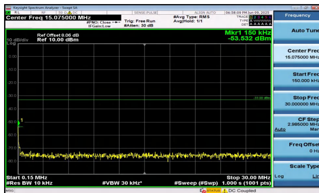
Band2-1.4MHz-QPSK-19193-1RB#0-0.15~30-PASS
