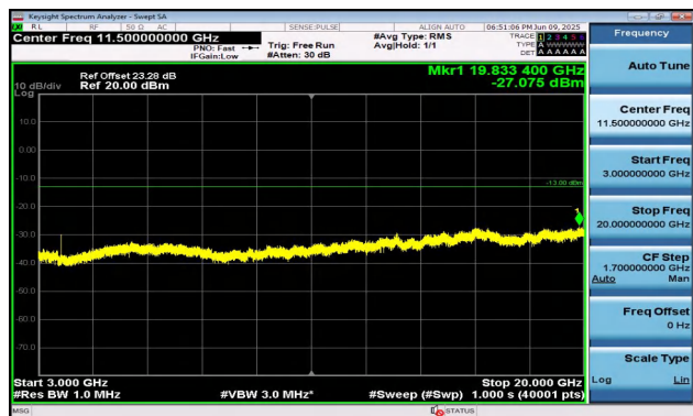
Band2-1.4MHz-16QAM-18607-1RB#5-3000~20000-PASS
