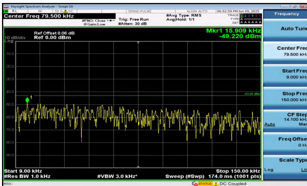
Band2-1.4MHz-QPSK-18900-1RB#0-0.009~0.15-PASS
