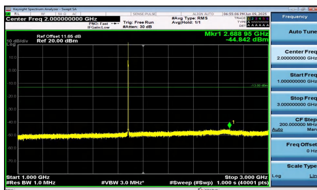
Band2-1.4MHz-QPSK-18900-1RB#5-1000~3000-PASS
