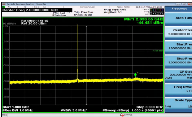
Band2-1.4MHz-16QAM-18900-1RB#0-1000~3000-PASS
