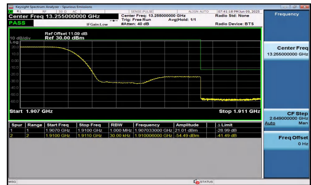
Band2-3MHz-16QAM-19185-1RB#0-PASS
