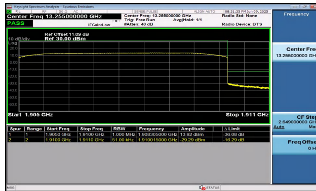
Band2-5MHz-16QAM-19175-25RB#0-PASS
