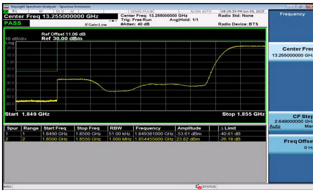
Band2-5MHz-16QAM-18625-1RB#24-PASS
