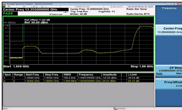
Band2-10MHz-16QAM-18650-1RB#49-PASS
