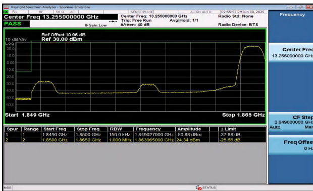
Band2-15MHz-16QAM-18675-1RB#74-PASS
