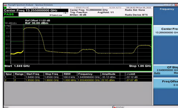
Band2-10MHz-16QAM-18650-1RB#0-PASS
