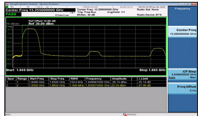
Band2-15MHz-16QAM-18675-1RB#0-PASS
