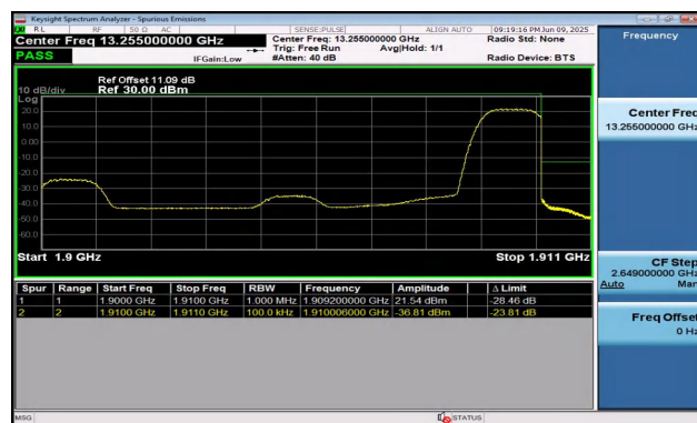
Band2-10MHz-16QAM-19150-1RB#49-PASS
