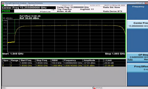
Band2-15MHz-QPSK-18675-75RB#0-PASS
