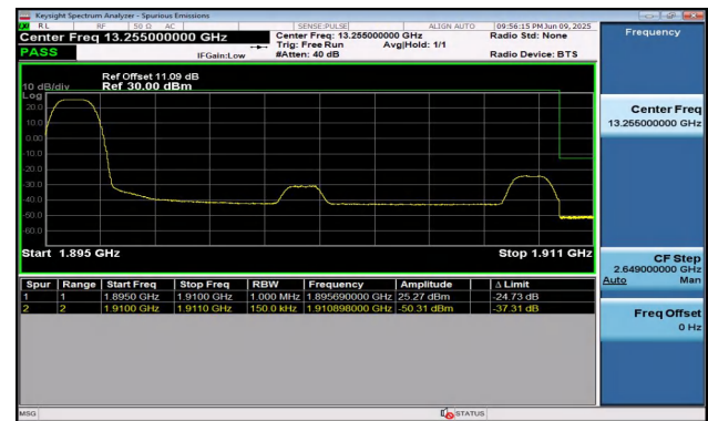
Band2-15MHz-QPSK-19125-1RB#0-PASS
