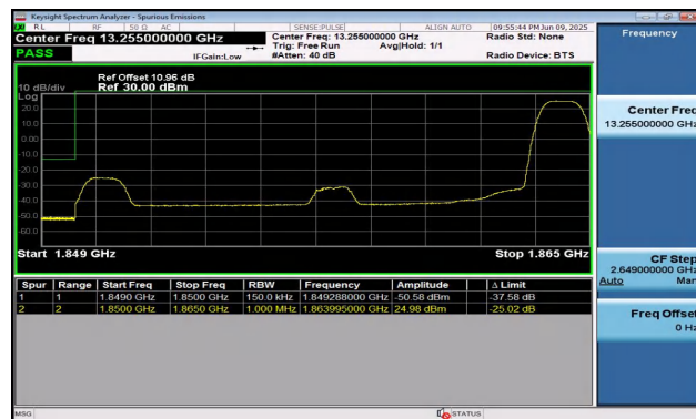
Band2-15MHz-QPSK-18675-1RB#74-PASS
