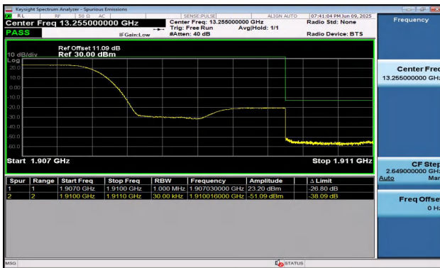
Band2-3MHz-QPSK-19185-1RB#0-PASS
