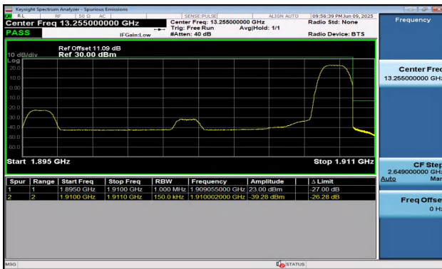
Band2-15MHz-QPSK-19125-1RB#74-PASS
