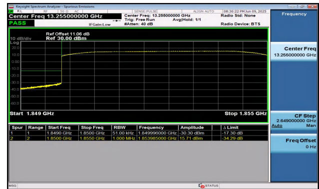
Band2-5MHz-16QAM-18625-25RB#0-PASS
