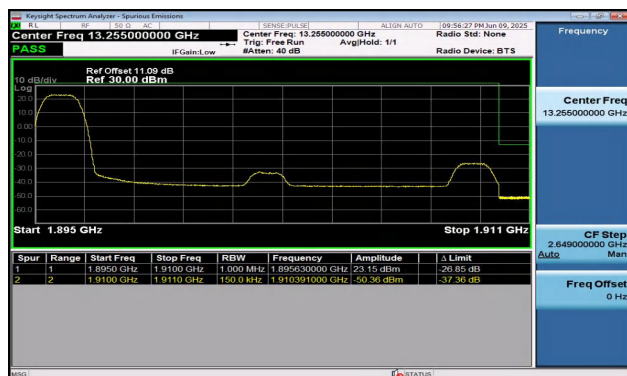
Band2-15MHz-16QAM-19125-1RB#0-PASS
