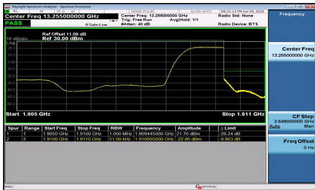
Band2-5MHz-16QAM-19175-1RB#24-PASS
