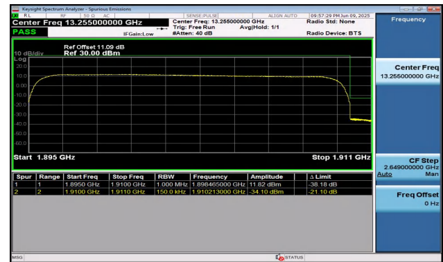
Band2-15MHz-QPSK-19125-75RB#0-PASS
