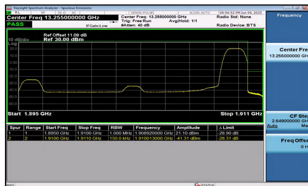
Band2-15MHz-16QAM-19125-1RB#74-PASS
