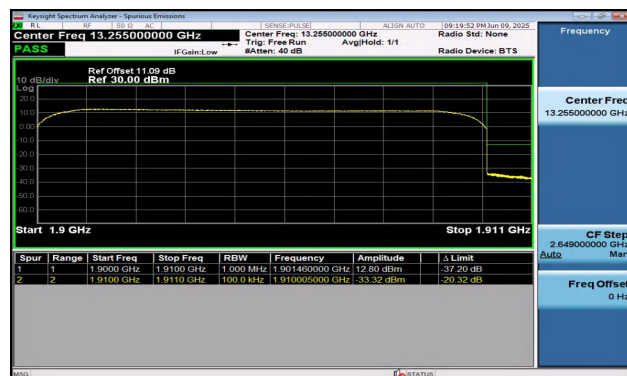
Band2-10MHz-QPSK-19150-50RB#0-PASS
