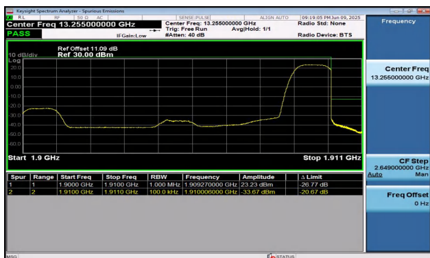
Band2-10MHz-QPSK-19150-1RB#49-PASS
