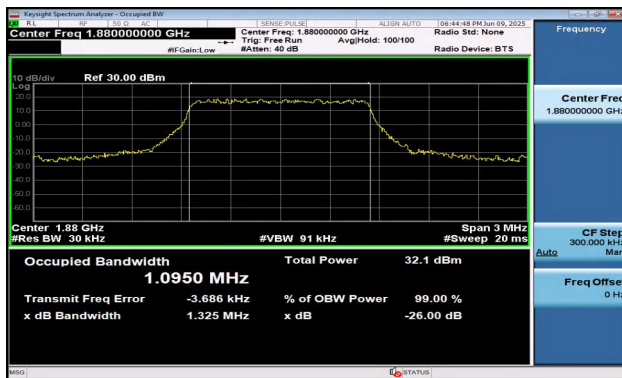
Band2-1.4MHz-QPSK-18900-6RB#0-PASS
