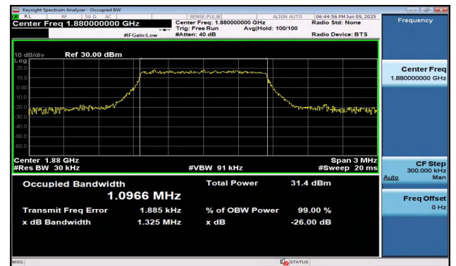
Band2-1.4MHz-16QAM-18900-6RB#0-PASS
