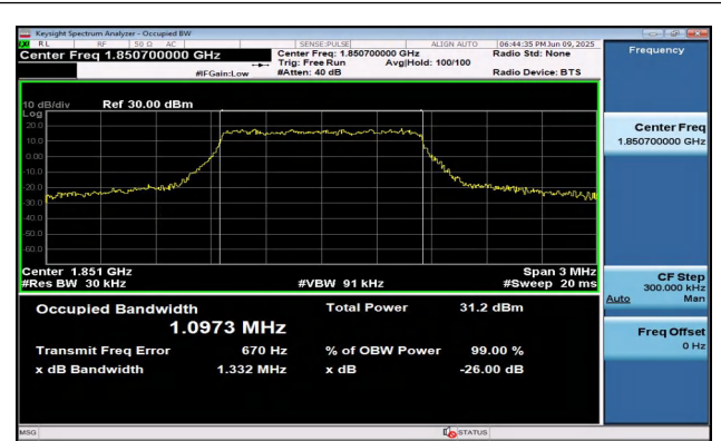
Band2-1.4MHz-16QAM-18607-6RB#0-PASS
