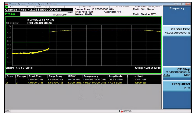
Band2-3MHz-16QAM-18615-15RB#0-PASS
