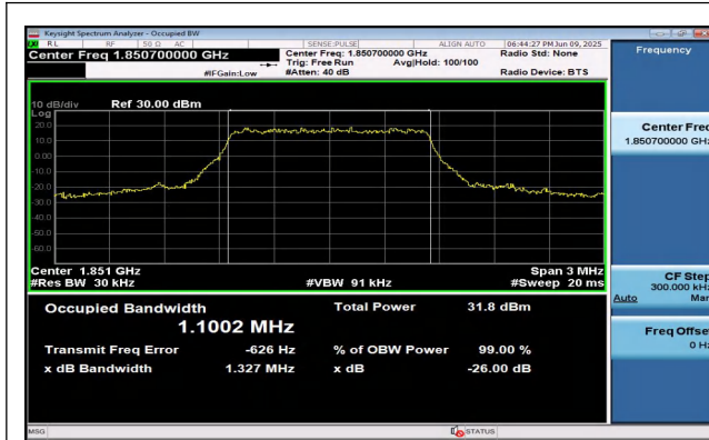
Band2-1.4MHz-QPSK-18607-6RB#0-PASS
