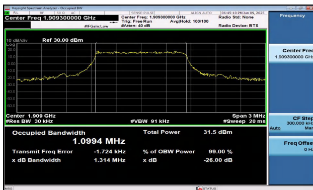
Band2-1.4MHz-QPSK-19193-6RB#0-PASS
